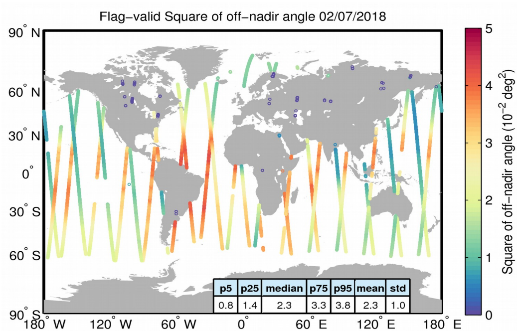
Figure 37. Geographical distribution of flag-valid mispointing data over oceans and lakes for 02/07/2018. The statistical values shown in the table refer to the mispointing in 10^{-2} \text{ deg}^2 and are calculated over all measurements shown in the figure.
