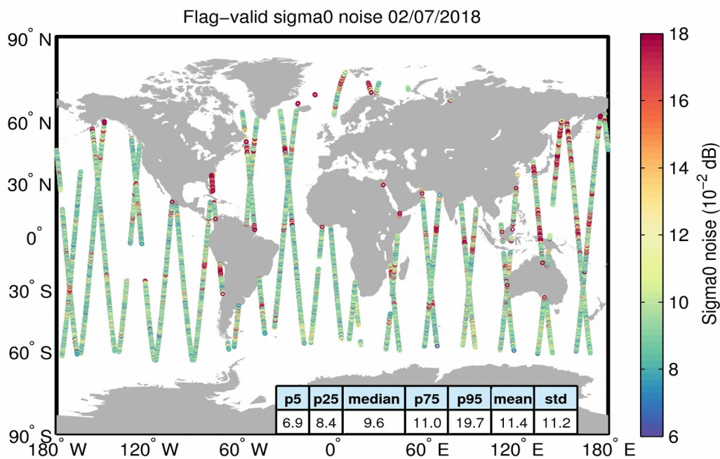
Figure 26. Geographical distribution of flag-valid 20-Hz sigma0 measurement noise over oceans and lakes for 02/07/2018. The statistical values shown in the table refer to the sigma0 noise and are calculated over all measurements shown in the figure.
