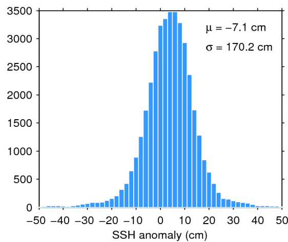
Figure 7. Histogram of flag-valid SSH anomaly over oceans and lakes for 02/07/2018. The mean ( \mu ) and standard deviation ( \sigma ) are also shown. Note that values outside [-50 50] cm are excluded from the histogram for the sake of readability but not from the computation of \mu and \sigma .
