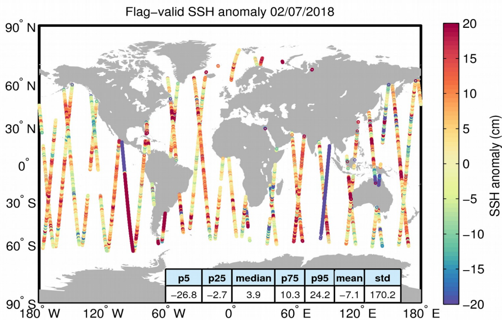
Figure 5. Geographical distribution of flag-valid 1-Hz SSH anomaly data over oceans and lakes for 02/07/2018. The statistical values shown in the table refer to the SSH anomaly in cm and are calculated over all measurements shown in the figure.
