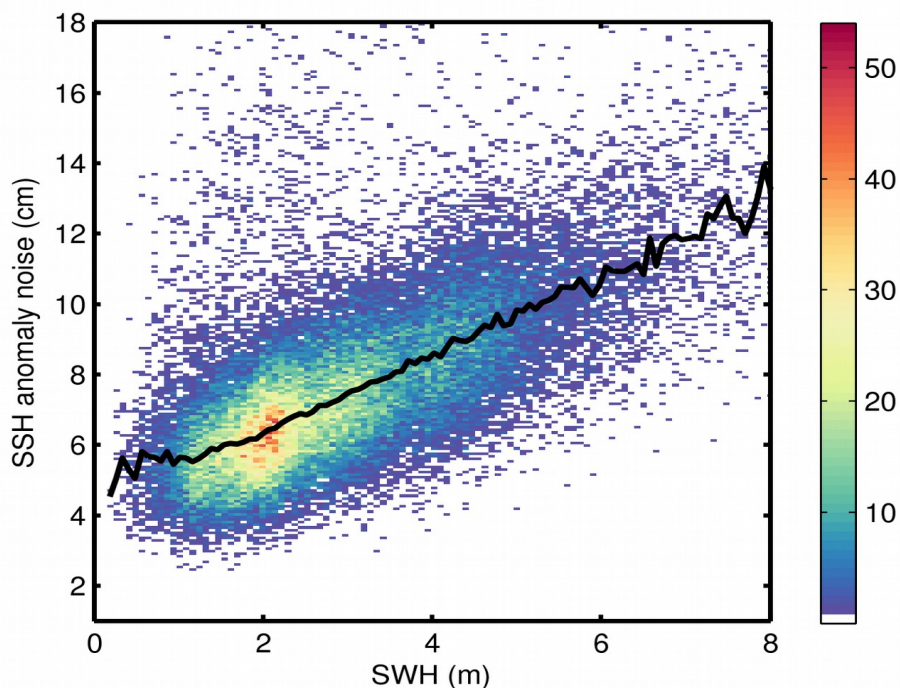
Figure 9. 2D histogram showing flag-valid SSH anomaly noise as a function of SWH for 02/07/2018. The black line denotes the median SSH anomaly noise as a function of SWH.
