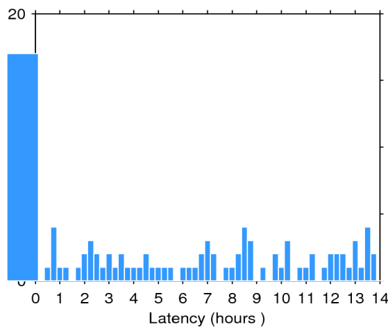
Figure 2. Histogram of the data latency for 02/07/2018. The y-axis denotes the number of files that are made available with a delay of x-hours with respect to the mean time of the records stored in the file.
