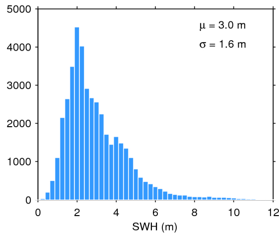
Figure 17. Histogram of flag-valid SWH over oceans and lakes for 02/07/2018. The mean ( \mu ) and standard deviation ( \sigma ) are also shown. Note that values larger than 12 m are excluded from the histogram for the sake of readability but not from the computation of \mu and \sigma .
