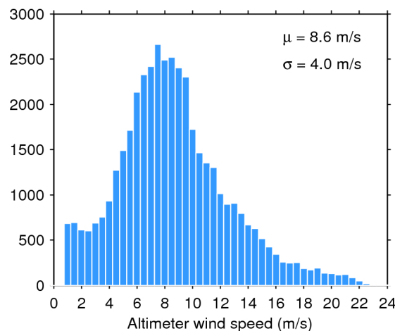
Figure 35. Histogram of science-valid wind over oceans and lakes for 02/07/2018. The mean ( \mu ) and standard deviation ( \sigma ) are also shown. Note that values larger than 24 m/s are excluded from the histogram for the sake of readability but not from the computation of \mu and \sigma .
