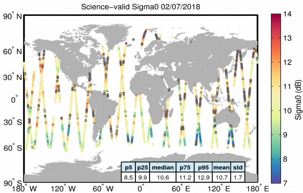
Figure 27. Geographical distribution of science-valid sigma0 data over oceans and lakes for 02/07/2018. The statistical values shown in the table refer to the sigma0 in dB and are calculated over all measurements shown in the figure. Gray circles denote records that have been rejected based on the editing criteria described in Table 4.
