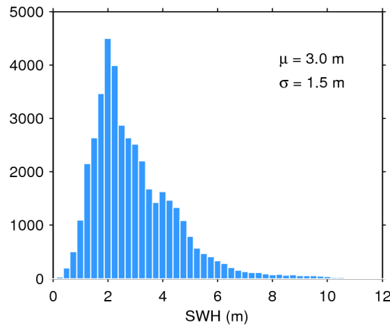
Figure 20. Histogram of science-valid SWH over oceans and lakes for 02/07/2018. The mean ( \mu ) and standard deviation ( \sigma ) are also shown. Note that values larger than 12 m are excluded from the histogram for the sake of readability but not from the computation of \mu and \sigma .
