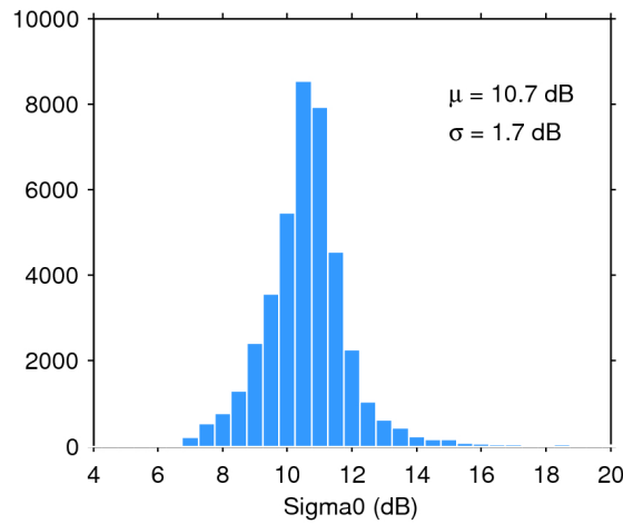
Figure 28. Histogram of science-valid sigma0 over oceans and lakes for 02/07/2018. The mean ( \mu ) and standard deviation ( \sigma ) are also shown. Note that values outside [4 20] dB are excluded from the histogram for the sake of readability but not from the computation of \mu and \sigma .
