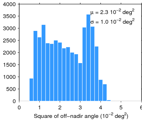
Figure 39. Histogram of flag-valid mispointing over oceans and lakes for 02/07/2018. The mean ( \mu ) and standard deviation ( \sigma ) are also shown. Note that values larger than 6 \cdot 10^{-2} \text{ deg}^2 are excluded from the histogram for the sake of readability but not from the computation of \mu and \sigma .
