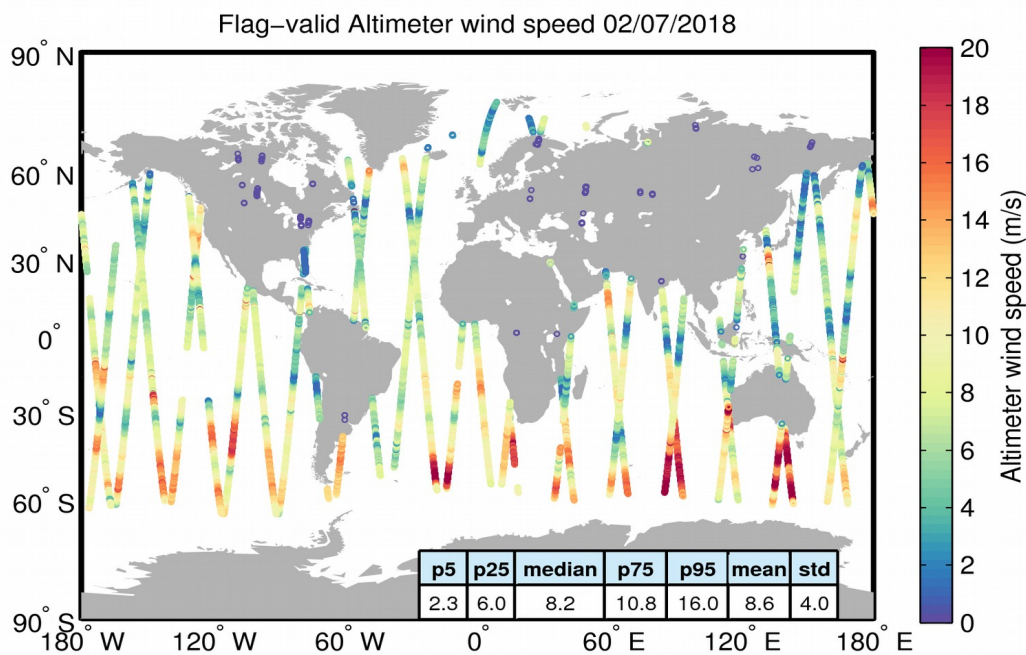
Figure 31. Geographical distribution of flag-valid wind data over oceans and lakes for 02/07/2018. The statistical values shown in the table refer to the wind in m/s and are calculated over all measurements shown in the figure.
