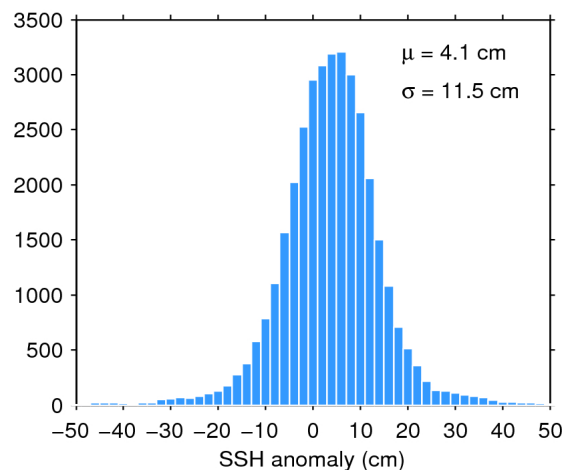
Figure 11. Histogram of science-valid SSH anomaly over oceans and lakes for 02/07/2018. The mean ( \mu ) and standard deviation ( \sigma ) are also shown. Note that values outside [-50 50] cm are excluded from the histogram for the sake of readability but not from the computation of \mu and \sigma .
