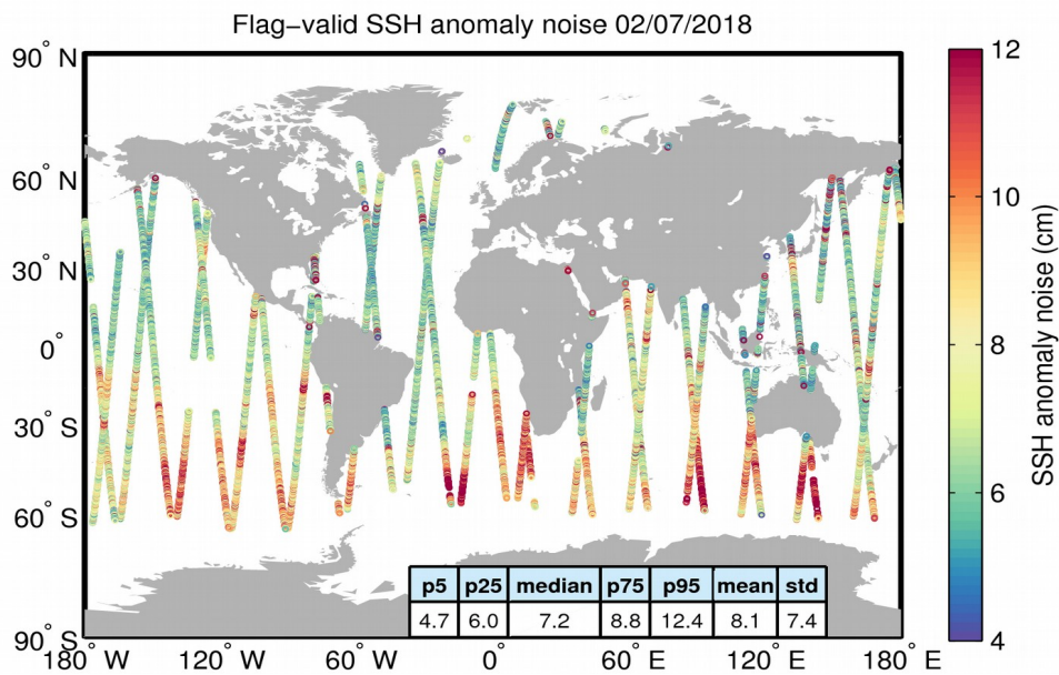
Figure 8. Geographical distribution of flag-valid 20-Hz SSH anomaly measurement noise over oceans and lakes for 02/07/2018. The statistical values shown in the table refer to the SSH anomaly noise and are calculated over all measurements shown in the figure.
