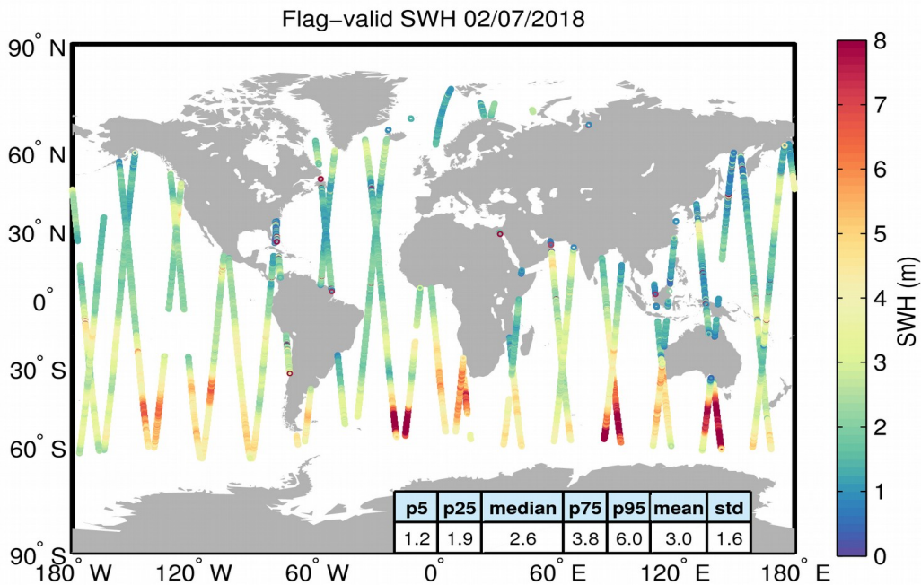
Figure 15. Geographical distribution of flag-valid SWH data over oceans and lakes for 02/07/2018. The statistical values shown in the table refer to the SWH in m and are calculated over all measurements shown in the figure.
