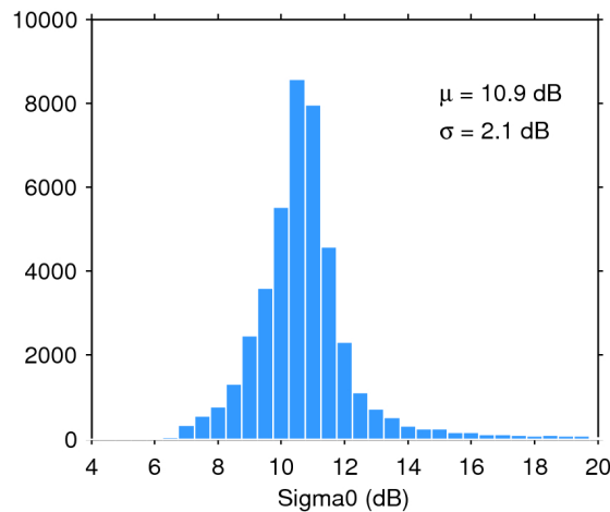
Figure 25. Histogram of flag-valid sigma0 over oceans and lakes for 02/07/2018. The mean ( \mu ) and standard deviation ( \sigma ) are also shown. Note that values outside [4 20] dB are excluded from the histogram for the sake of readability but not from the computation of \mu and \sigma .
