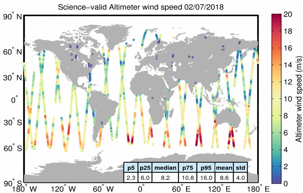
Figure 34. Geographical distribution of science-valid wind data over oceans and lakes for 02/07/2018. The statistical values shown in the table refer to the wind in m/s and are calculated over all measurements shown in the figure. Gray circles denote records that have been rejected based on the editing criteria described in Table 5.
