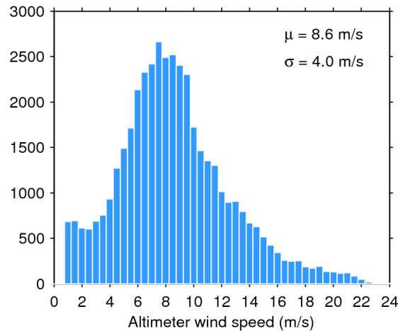
Figure 33. Histogram of flag-valid wind over oceans and lakes for 02/07/2018. The mean ( \mu ) and standard deviation ( \sigma ) are also shown. Note that values larger than 24 m/s are excluded from the histogram for the sake of readability but not from the computation of \mu and \sigma .
