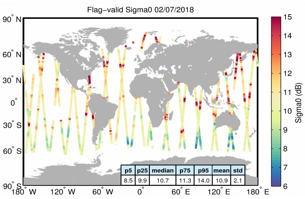
Figure 23. Geographical distribution of flag-valid sigma0 data over oceans and lakes for 02/07/2018. The statistical values shown in the table refer to the sigma0 in dB and are calculated over all measurements shown in the figure.
