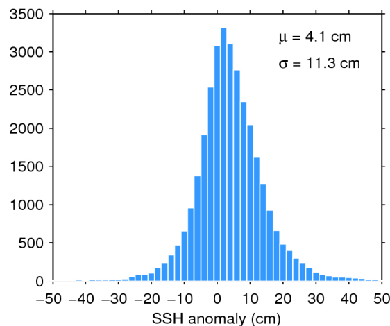
Figure 11. Histogram of science-valid SSH anomaly over oceans and lakes for 01/07/2018. The mean ( \mu ) and standard deviation ( \sigma ) are also shown. Note that values outside [-50 50] cm are excluded from the histogram for the sake of readability but not from the computation of \mu and \sigma .
