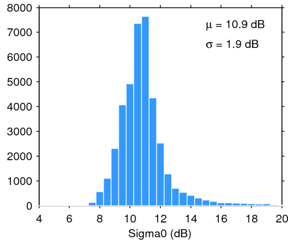
Figure 25. Histogram of flag-valid sigma0 over oceans and lakes for 01/07/2018. The mean ( \mu ) and standard deviation ( \sigma ) are also shown. Note that values outside [4 20] dB are excluded from the histogram for the sake of readability but not from the computation of \mu and \sigma .
