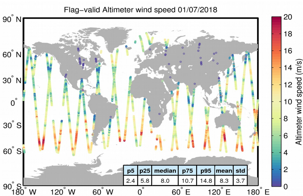
Figure 31. Geographical distribution of flag-valid wind data over oceans and lakes for 01/07/2018. The statistical values shown in the table refer to the wind in m/s and are calculated over all measurements shown in the figure.
