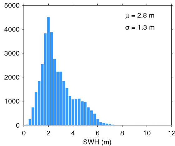
Figure 20. Histogram of science-valid SWH over oceans and lakes for 01/07/2018. The mean ( \mu ) and standard deviation ( \sigma ) are also shown. Note that values larger than 12 m are excluded from the histogram for the sake of readability but not from the computation of \mu and \sigma .
