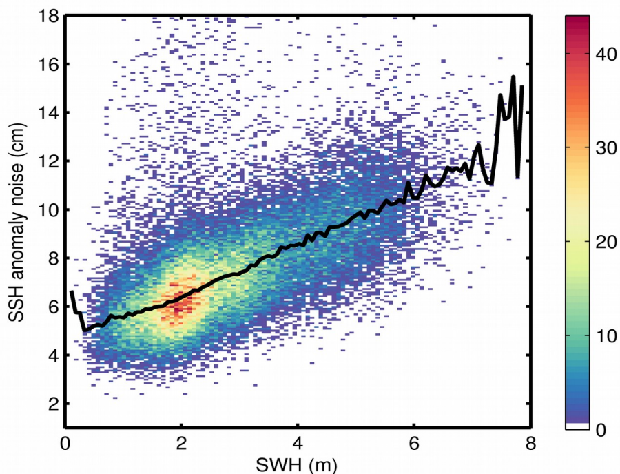
Figure 9. 2D histogram showing flag-valid SSH anomaly noise as a function of SWH for 01/07/2018. The black line denotes the median SSH anomaly noise as a function of SWH.
