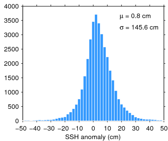
Figure 7. Histogram of flag-valid SSH anomaly over oceans and lakes for 01/07/2018. The mean ( \mu ) and standard deviation ( \sigma ) are also shown. Note that values outside [-50\ 50] cm are excluded from the histogram for the sake of readability but not from the computation of \mu and \sigma .
