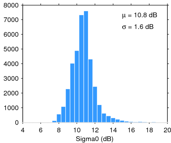
Figure 28. Histogram of science-valid sigma0 over oceans and lakes for 01/07/2018. The mean ( \mu ) and standard deviation ( \sigma ) are also shown. Note that values outside [4 20] dB are excluded from the histogram for the sake of readability but not from the computation of \mu and \sigma .
