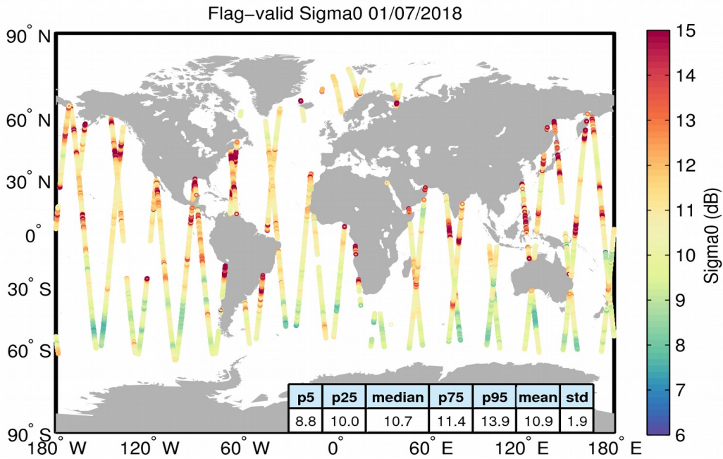
Figure 23. Geographical distribution of flag-valid sigma0 data over oceans and lakes for 01/07/2018. The statistical values shown in the table refer to the sigma0 in dB and are calculated over all measurements shown in the figure.
