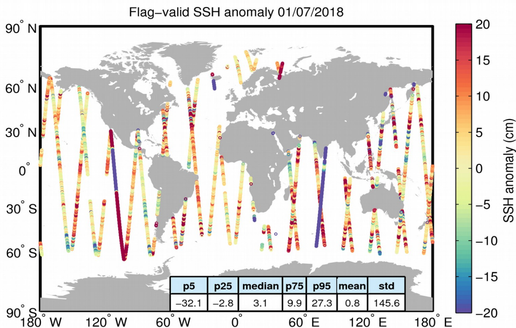
Figure 5. Geographical distribution of flag-valid 1-Hz SSH anomaly data over oceans and lakes for 01/07/2018. The statistical values shown in the table refer to the SSH anomaly in cm and are calculated over all measurements shown in the figure.
