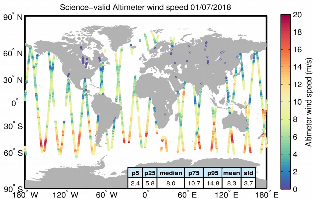
Figure 34. Geographical distribution of science-valid wind data over oceans and lakes for 01/07/2018. The statistical values shown in the table refer to the wind in m/s and are calculated over all measurements shown in the figure. Gray circles denote records that have been rejected based on the editing criteria described in Table 5.
