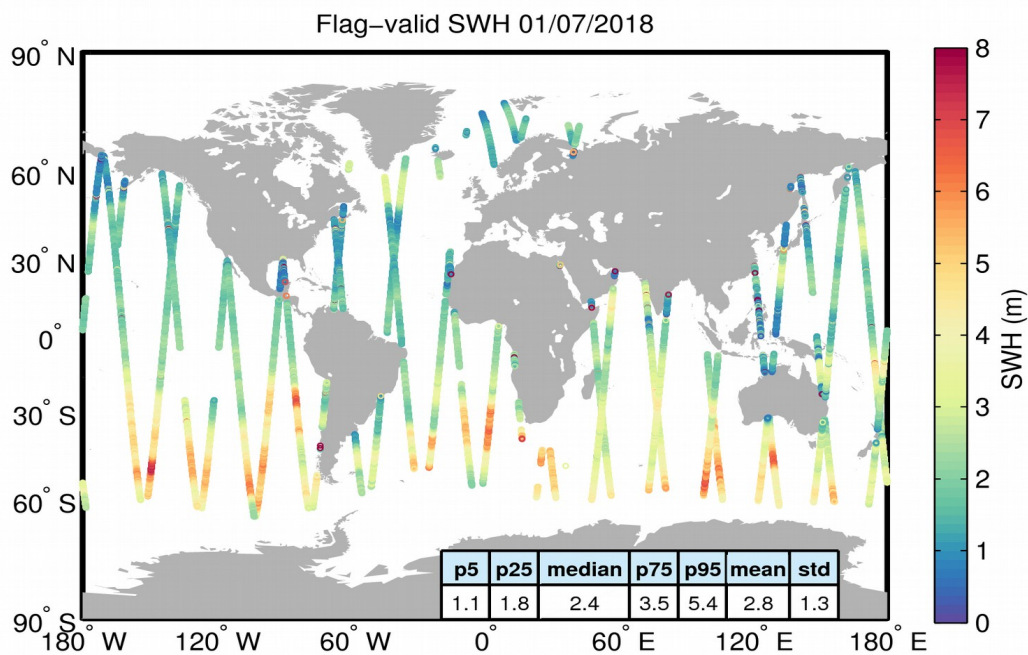
Figure 15. Geographical distribution of flag-valid SWH data over oceans and lakes for 01/07/2018. The statistical values shown in the table refer to the SWH in m and are calculated over all measurements shown in the figure.
