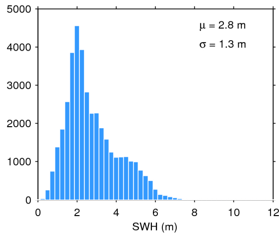
Figure 17. Histogram of flag-valid SWH over oceans and lakes for 01/07/2018. The mean ( \mu ) and standard deviation ( \sigma ) are also shown. Note that values larger than 12 m are excluded from the histogram for the sake of readability but not from the computation of \mu and \sigma .
