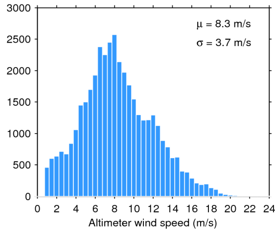
Figure 33. Histogram of flag-valid wind over oceans and lakes for 01/07/2018. The mean ( \mu ) and standard deviation ( \sigma ) are also shown. Note that values larger than 24 m/s are excluded from the histogram for the sake of readability but not from the computation of \mu and \sigma .
