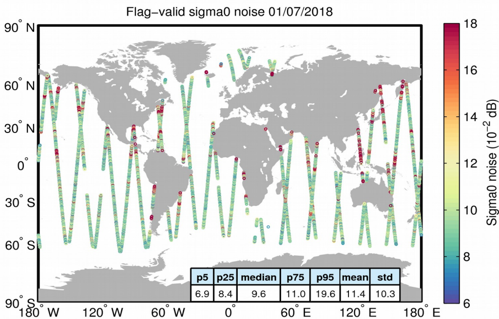
Figure 26. Geographical distribution of flag-valid 20-Hz sigma0 measurement noise over oceans and lakes for 01/07/2018. The statistical values shown in the table refer to the sigma0 noise and are calculated over all measurements shown in the figure.
