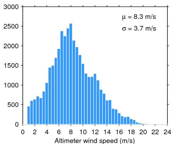
Figure 35. Histogram of science-valid wind over oceans and lakes for 01/07/2018. The mean ( \mu ) and standard deviation ( \sigma ) are also shown. Note that values larger than 24 m/s are excluded from the histogram for the sake of readability but not from the computation of \mu and \sigma .
