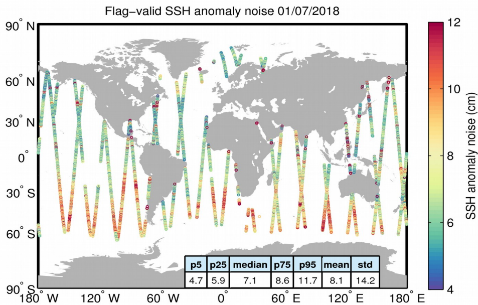
Figure 8. Geographical distribution of flag-valid 20-Hz SSH anomaly measurement noise over oceans and lakes for 01/07/2018. The statistical values shown in the table refer to the SSH anomaly noise and are calculated over all measurements shown in the figure.
