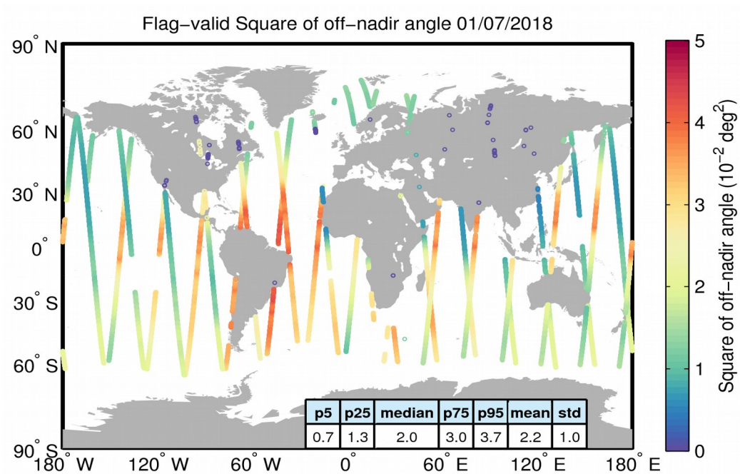
Figure 37. Geographical distribution of flag-valid mispointing data over oceans and lakes for 01/07/2018. The statistical values shown in the table refer to the mispointing in 10^{-2} \text{ deg}^2 and are calculated over all measurements shown in the figure.
