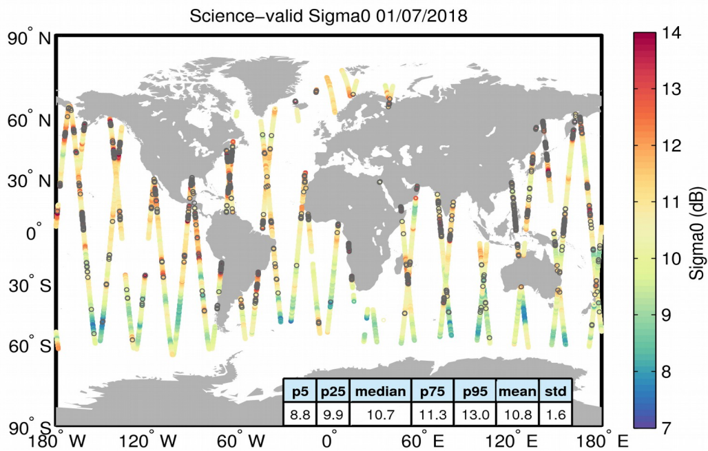
Figure 27. Geographical distribution of science-valid sigma0 data over oceans and lakes for 01/07/2018. The statistical values shown in the table refer to the sigma0 in dB and are calculated over all measurements shown in the figure. Gray circles denote records that have been rejected based on the editing criteria described in Table 4.
