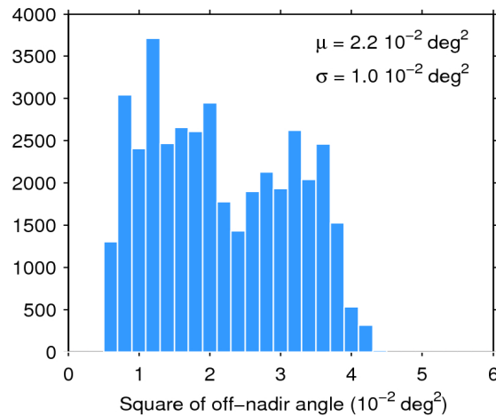
Figure 39. Histogram of flag-valid mispointing over oceans and lakes for 01/07/2018. The mean ( \mu ) and standard deviation ( \sigma ) are also shown. Note that values larger than 6 \cdot 10^{-2} \text{ deg}^2 are excluded from the histogram for the sake of readability but not from the computation of \mu and \sigma .
