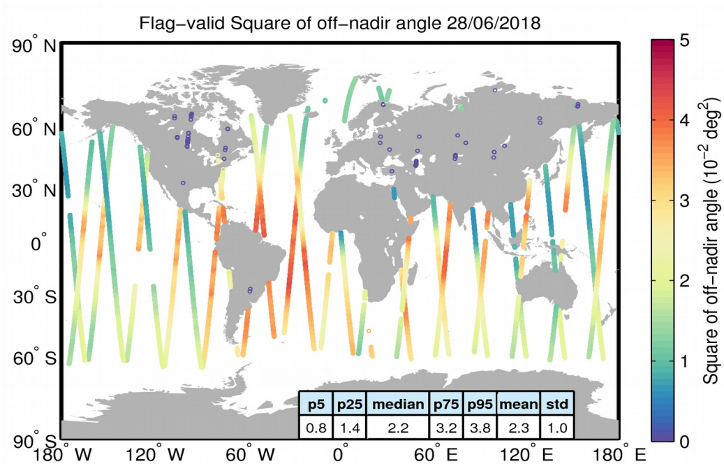
Figure 37. Geographical distribution of flag-valid mispointing data over oceans and lakes for 28/06/2018. The statistical values shown in the table refer to the mispointing in 10^{-2} \text{deg}^2 and are calculated over all measurements shown in the figure.
