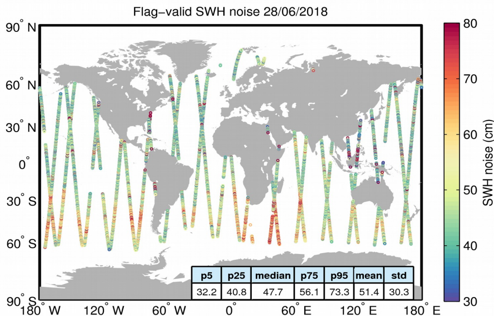
Figure 18. Geographical distribution of flag-valid 20-Hz SWH measurement noise over oceans and lakes for 28/06/2018. The statistical values shown in the figure refer to the SWH noise and are calculated over all measurements shown in the figure.
