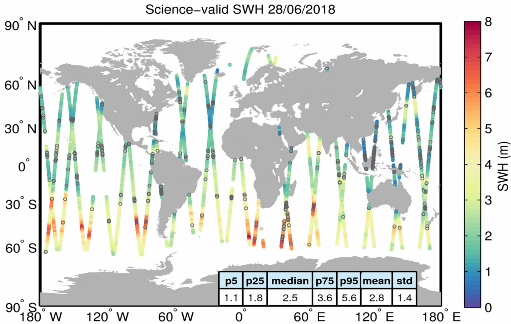
Figure 19. Geographical distribution of science-valid SWH data over oceans and lakes for 28/06/2018. The statistical values shown in the table refer to the SWH in m and are calculated over all measurements shown in the figure. Gray circles denote records that have been rejected based on the editing criteria described in Table 3.
