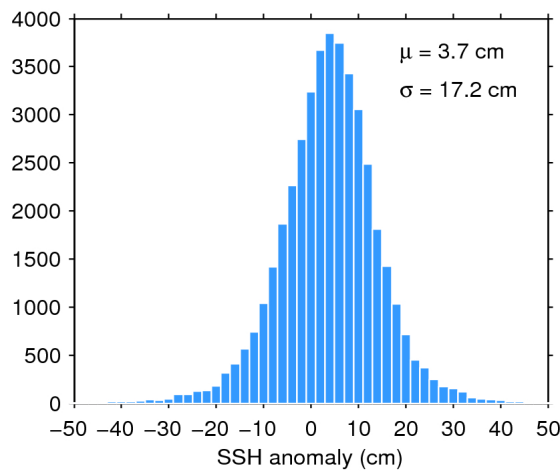
Figure 7. Histogram of flag-valid SSH anomaly over oceans and lakes for 28/06/2018. The mean ( \mu ) and standard deviation ( \sigma ) are also shown. Note that values outside [-50 50] cm are excluded from the histogram for the sake of readability but not from the computation of \mu and \sigma .
