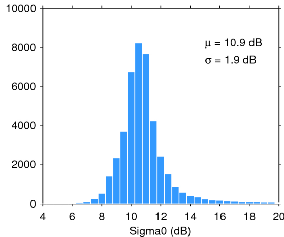
Figure 25. Histogram of flag-valid sigma0 over oceans and lakes for 28/06/2018. The mean ( \mu ) and standard deviation ( \sigma ) are also shown. Note that values outside [4 20] dB are excluded from the histogram for the sake of readability but not from the computation of \mu and \sigma .
