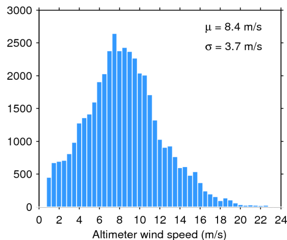
Figure 35. Histogram of science-valid wind over oceans and lakes for 28/06/2018. The mean ( \mu ) and standard deviation ( \sigma ) are also shown. Note that values larger than 24 m/s are excluded from the histogram for the sake of readability but not from the computation of \mu and \sigma .
