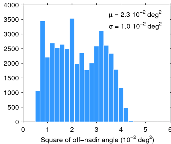
Figure 39. Histogram of flag-valid mispointing over oceans and lakes for 28/06/2018. The mean ( \mu ) and standard deviation ( \sigma ) are also shown. Note that values larger than 6 \cdot 10^{-2} \text{ deg}^2 are excluded from the histogram for the sake of readability but not from the computation of \mu and \sigma .
