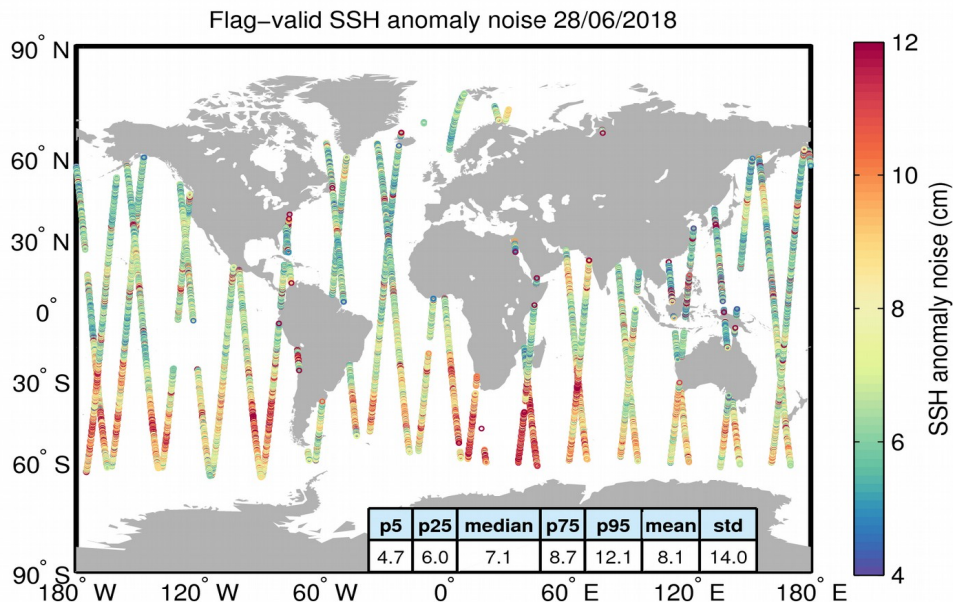
Figure 8. Geographical distribution of flag-valid 20-Hz SSH anomaly measurement noise over oceans and lakes for 28/06/2018. The statistical values shown in the table refer to the SSH anomaly noise and are calculated over all measurements shown in the figure.
