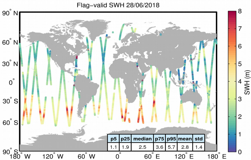
Figure 15. Geographical distribution of flag-valid SWH data over oceans and lakes for 28/06/2018. The statistical values shown in the table refer to the SWH in m and are calculated over all measurements shown in the figure.
