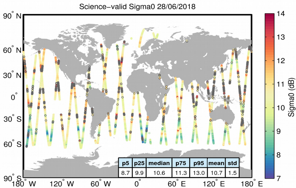
Figure 27. Geographical distribution of science-valid sigma0 data over oceans and lakes for 28/06/2018. The statistical values shown in the table refer to the sigma0 in dB and are calculated over all measurements shown in the figure. Gray circles denote records that have been rejected based on the editing criteria described in Table 4.
