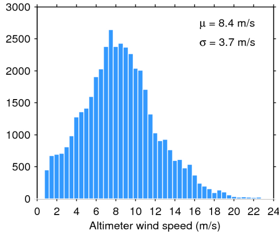
Figure 33. Histogram of flag-valid wind over oceans and lakes for 28/06/2018. The mean ( \mu ) and standard deviation ( \sigma ) are also shown. Note that values larger than 24 m/s are excluded from the histogram for the sake of readability but not from the computation of \mu and \sigma .
