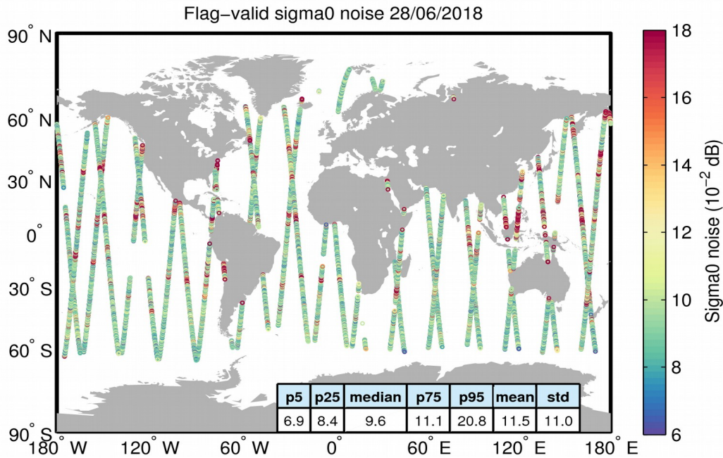
Figure 26. Geographical distribution of flag-valid 20-Hz sigma0 measurement noise over oceans and lakes for 28/06/2018. The statistical values shown in the table refer to the sigma0 noise and are calculated over all measurements shown in the figure.
