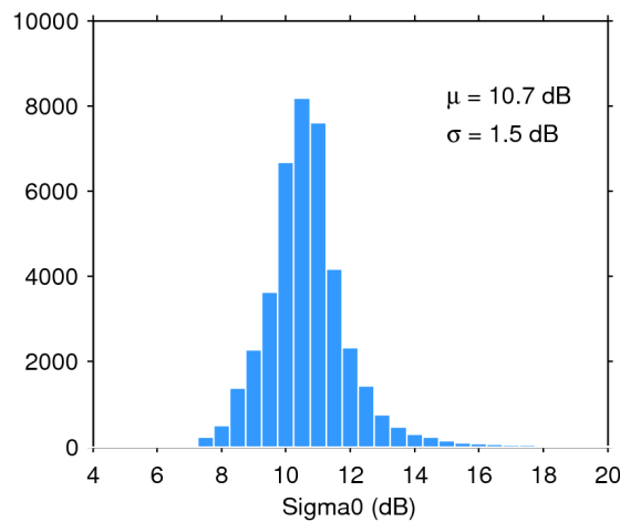
Figure 28. Histogram of science-valid sigma0 over oceans and lakes for 28/06/2018. The mean ( \mu ) and standard deviation ( \sigma ) are also shown. Note that values outside [4 20] dB are excluded from the histogram for the sake of readability but not from the computation of \mu and \sigma .
