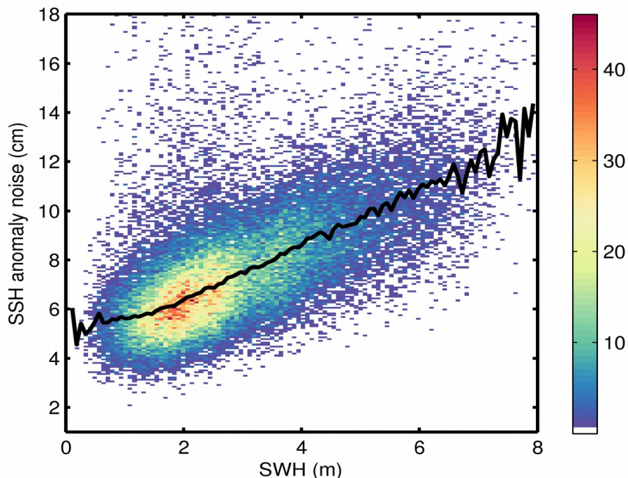
Figure 9. 2D histogram showing flag-valid SSH anomaly noise as a function of SWH for 28/06/2018. The black line denotes the median SSH anomaly noise as a function of SWH.
