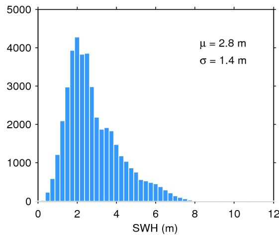
Figure 17. Histogram of flag-valid SWH over oceans and lakes for 28/06/2018. The mean ( \mu ) and standard deviation ( \sigma ) are also shown. Note that values larger than 12 m are excluded from the histogram for the sake of readability but not from the computation of \mu and \sigma .
