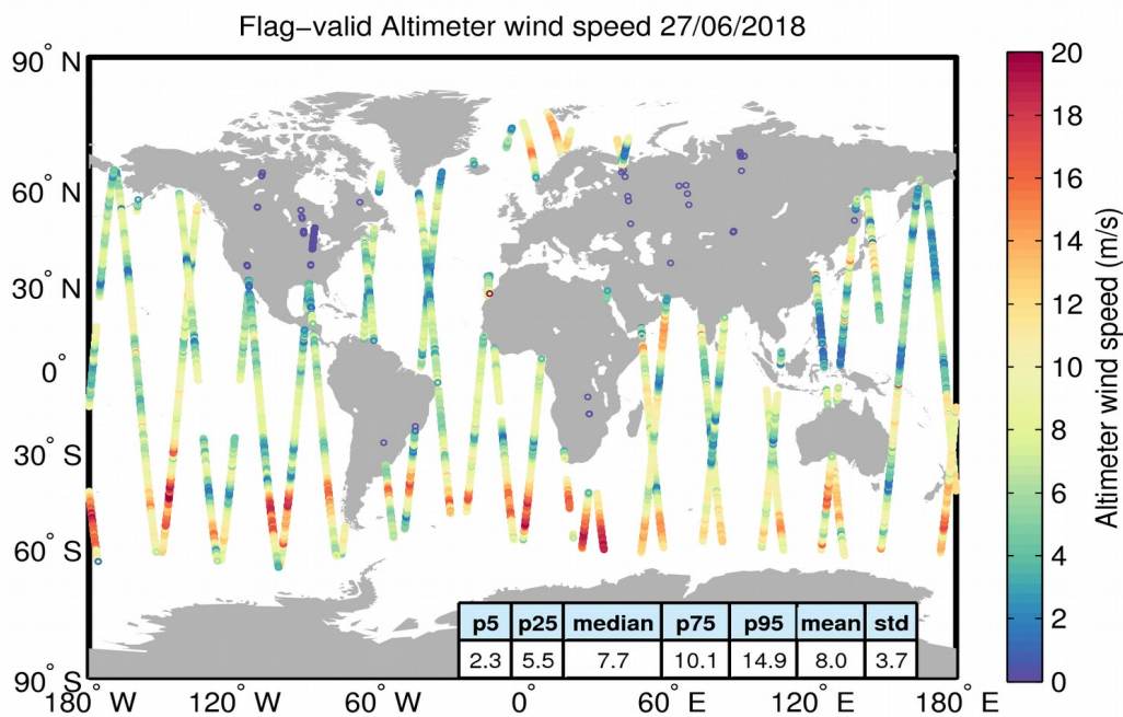
Figure 31. Geographical distribution of flag-valid wind data over oceans and lakes for 27/06/2018. The statistical values shown in the table refer to the wind in m/s and are calculated over all measurements shown in the figure.
