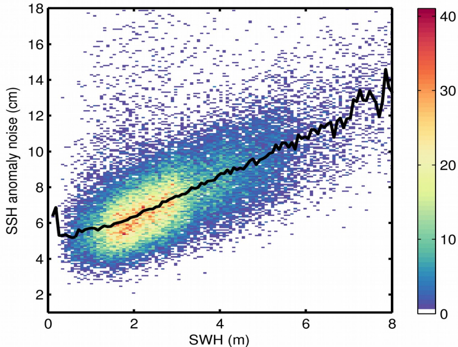
Figure 9. 2D histogram showing flag-valid SSH anomaly noise as a function of SWH for 27/06/2018. The black line denotes the median SSH anomaly noise as a function of SWH.
