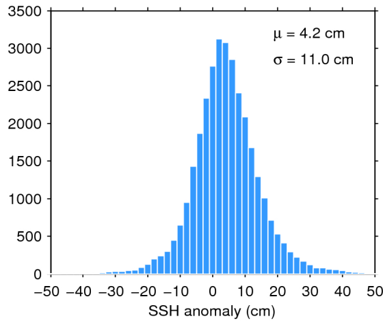
Figure 11. Histogram of science-valid SSH anomaly over oceans and lakes for 27/06/2018. The mean ( \mu ) and standard deviation ( \sigma ) are also shown. Note that values outside [-50 50] cm are excluded from the histogram for the sake of readability but not from the computation of \mu and \sigma .
