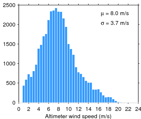
Figure 35. Histogram of science-valid wind over oceans and lakes for 27/06/2018. The mean ( \mu ) and standard deviation ( \sigma ) are also shown. Note that values larger than 24 m/s are excluded from the histogram for the sake of readability but not from the computation of \mu and \sigma .
