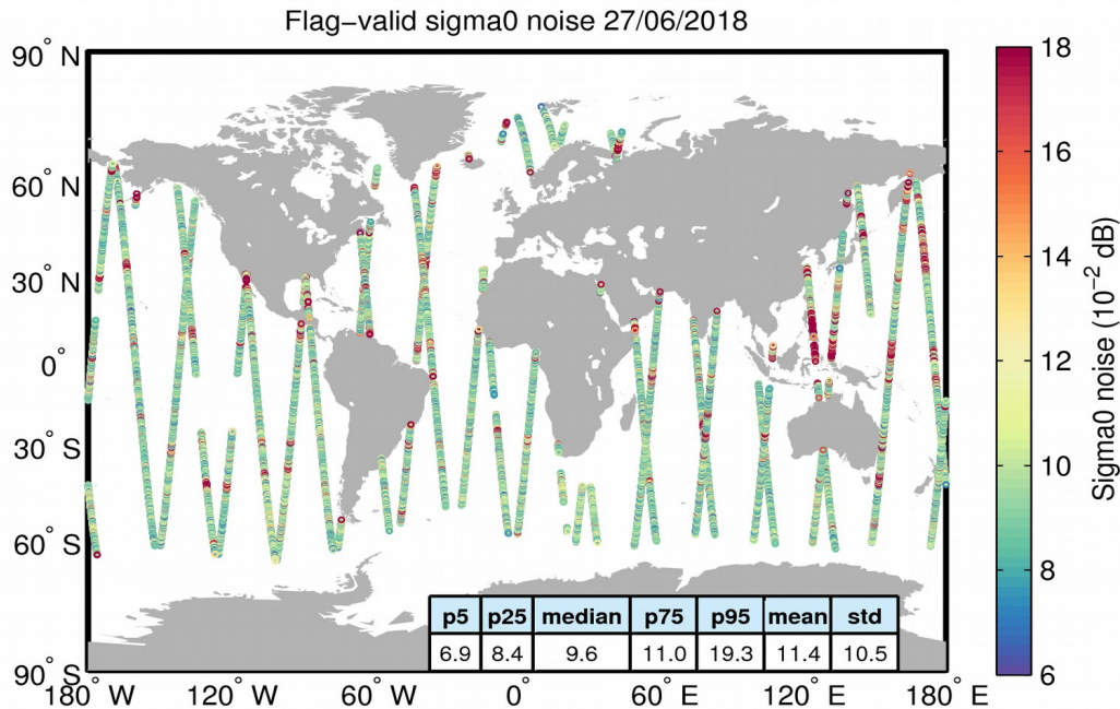
Figure 26. Geographical distribution of flag-valid 20-Hz sigma0 measurement noise over oceans and lakes for 27/06/2018. The statistical values shown in the table refer to the sigma0 noise and are calculated over all measurements shown in the figure.
