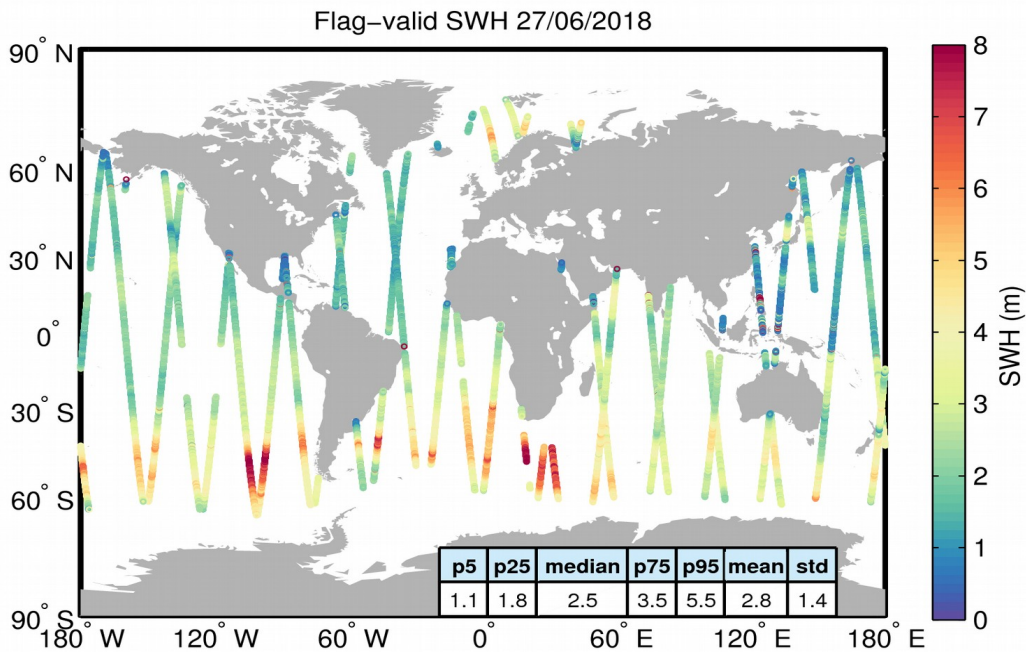
Figure 15. Geographical distribution of flag-valid SWH data over oceans and lakes for 27/06/2018. The statistical values shown in the table refer to the SWH in m and are calculated over all measurements shown in the figure.
