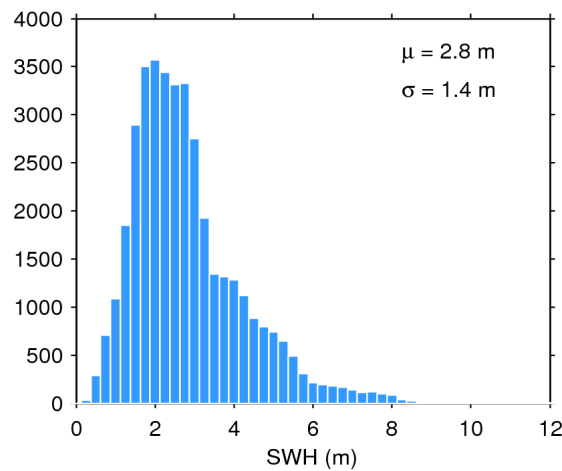
Figure 17. Histogram of flag-valid SWH over oceans and lakes for 27/06/2018. The mean ( \mu ) and standard deviation ( \sigma ) are also shown. Note that values larger than 12 m are excluded from the histogram for the sake of readability but not from the computation of \mu and \sigma .
