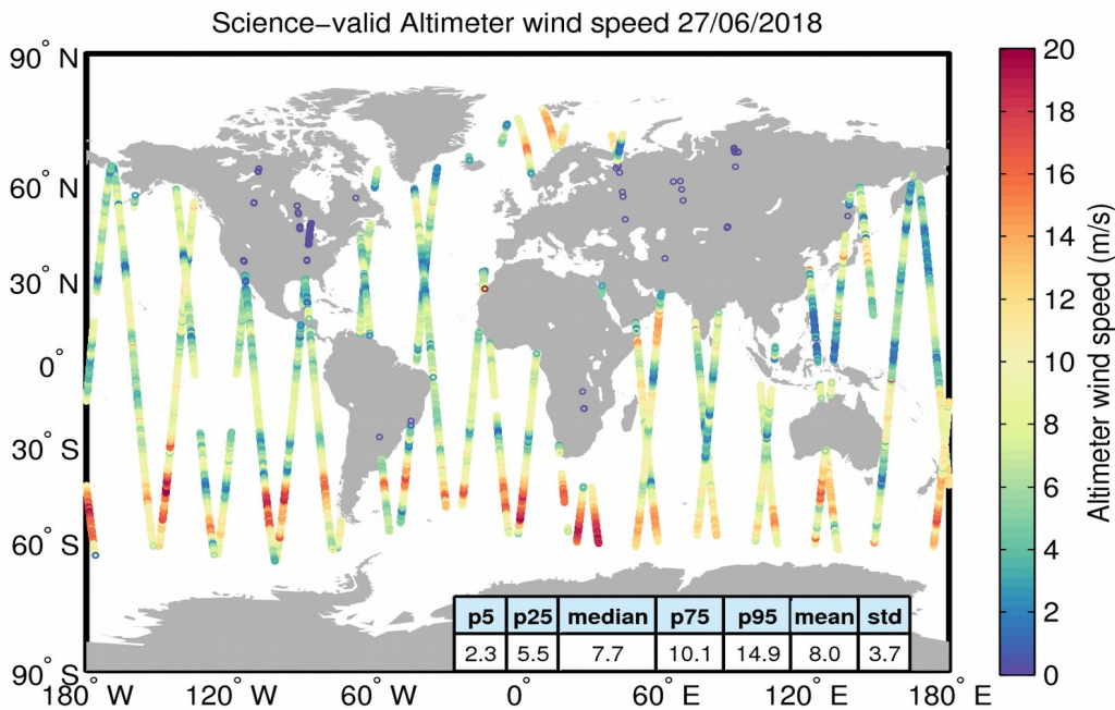
Figure 34. Geographical distribution of science-valid wind data over oceans and lakes for 27/06/2018. The statistical values shown in the table refer to the wind in m/s and are calculated over all measurements shown in the figure. Gray circles denote records that have been rejected based on the editing criteria described in Table 5.
