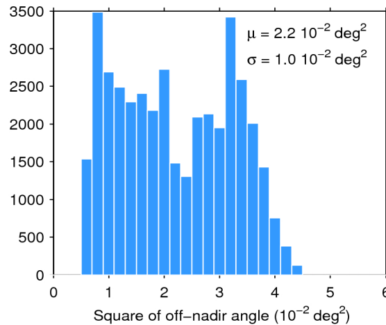
Figure 39. Histogram of flag-valid mispointing over oceans and lakes for 27/06/2018. The mean ( \mu ) and standard deviation ( \sigma ) are also shown. Note that values larger than 6 \times 10^{-2} \text{ deg}^2 are excluded from the histogram for the sake of readability but not from the computation of \mu and \sigma .
