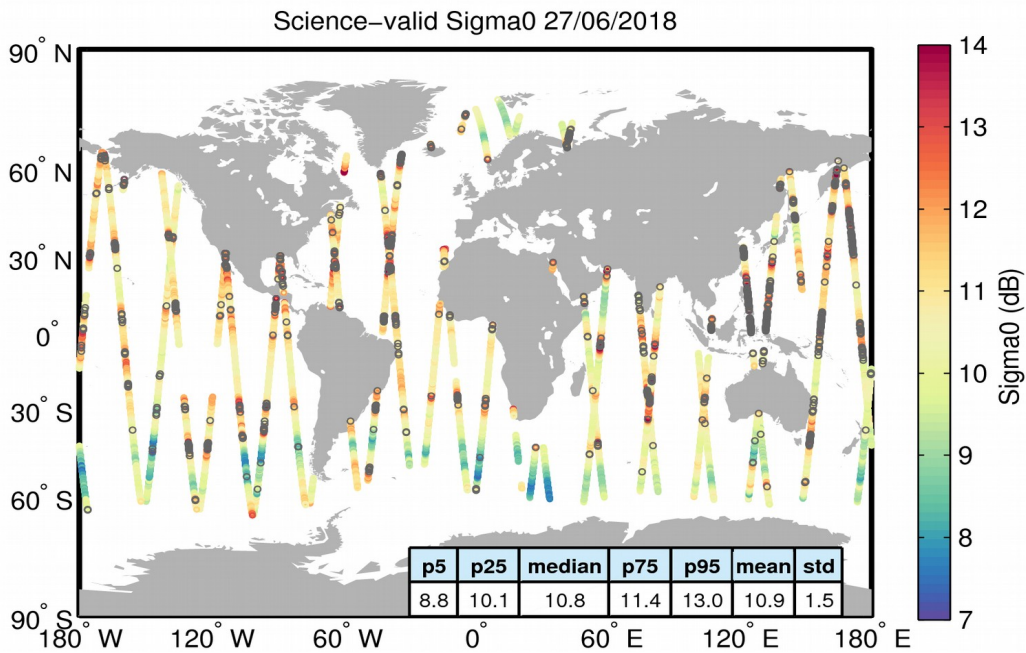
Figure 27. Geographical distribution of science-valid sigma0 data over oceans and lakes for 27/06/2018. The statistical values shown in the table refer to the sigma0 in dB and are calculated over all measurements shown in the figure. Gray circles denote records that have been rejected based on the editing criteria described in Table 4.
