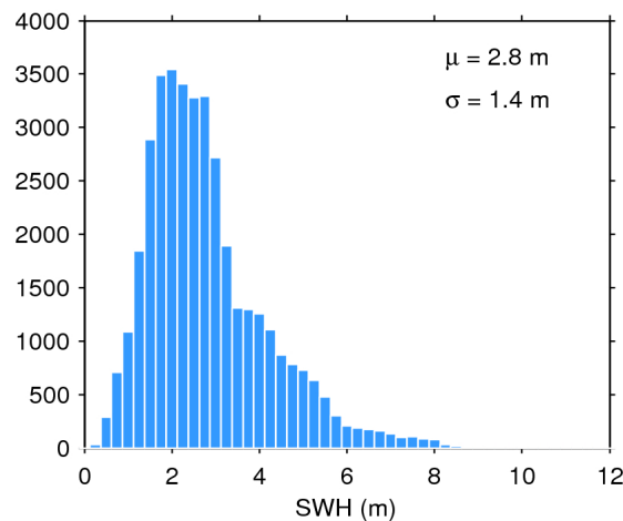
Figure 20. Histogram of science-valid SWH over oceans and lakes for 27/06/2018. The mean ( \mu ) and standard deviation ( \sigma ) are also shown. Note that values larger than 12 m are excluded from the histogram for the sake of readability but not from the computation of \mu and \sigma .
