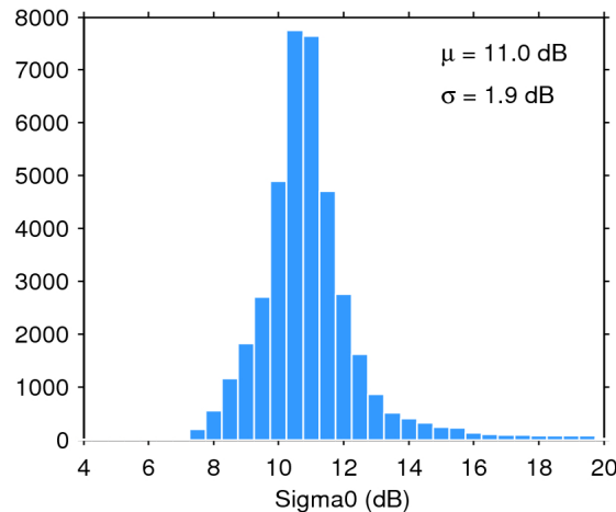
Figure 25. Histogram of flag-valid sigma0 over oceans and lakes for 27/06/2018. The mean ( \mu ) and standard deviation ( \sigma ) are also shown. Note that values outside [4 20] dB are excluded from the histogram for the sake of readability but not from the computation of \mu and \sigma .
