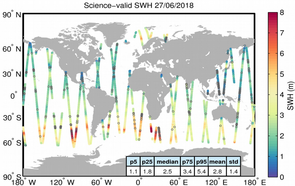
Figure 19. Geographical distribution of science-valid SWH data over oceans and lakes for 27/06/2018. The statistical values shown in the table refer to the SWH in m and are calculated over all measurements shown in the figure. Gray circles denote records that have been rejected based on the editing criteria described in Table 3.
