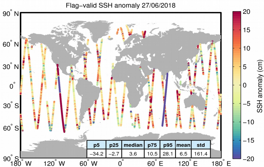
Figure 5. Geographical distribution of flag-valid 1-Hz SSH anomaly data over oceans and lakes for 27/06/2018. The statistical values shown in the table refer to the SSH anomaly in cm and are calculated over all measurements shown in the figure.
