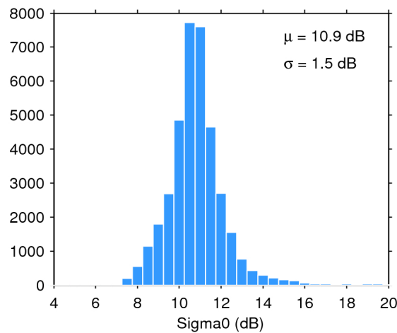
Figure 28. Histogram of science-valid sigma0 over oceans and lakes for 27/06/2018. The mean ( \mu ) and standard deviation ( \sigma ) are also shown. Note that values outside [4 20] dB are excluded from the histogram for the sake of readability but not from the computation of \mu and \sigma .
