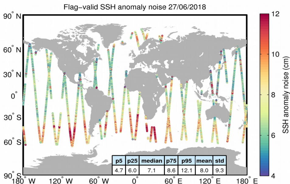
Figure 8. Geographical distribution of flag-valid 20-Hz SSH anomaly measurement noise over oceans and lakes for 27/06/2018. The statistical values shown in the table refer to the SSH anomaly noise and are calculated over all measurements shown in the figure.
