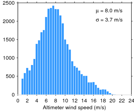
Figure 33. Histogram of flag-valid wind over oceans and lakes for 27/06/2018. The mean ( \mu ) and standard deviation ( \sigma ) are also shown. Note that values larger than 24 m/s are excluded from the histogram for the sake of readability but not from the computation of \mu and \sigma .
