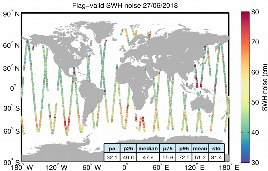
Figure 18. Geographical distribution of flag-valid 20-Hz SWH measurement noise over oceans and lakes for 27/06/2018. The statistical values shown in the figure refer to the SWH noise and are calculated over all measurements shown in the figure.
