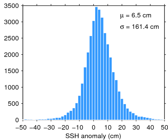
Figure 7. Histogram of flag-valid SSH anomaly over oceans and lakes for 27/06/2018. The mean ( \mu ) and standard deviation ( \sigma ) are also shown. Note that values outside [-50 50] cm are excluded from the histogram for the sake of readability but not from the computation of \mu and \sigma .
