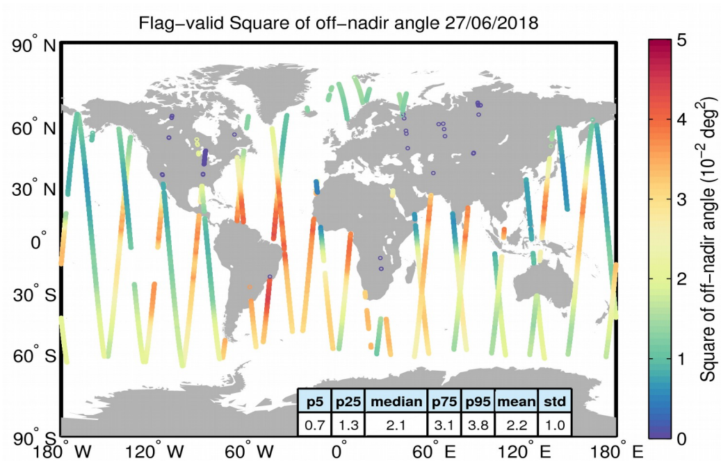
Figure 37. Geographical distribution of flag-valid mispointing data over oceans and lakes for 27/06/2018. The statistical values shown in the table refer to the mispointing in 10^{-2} \text{ deg}^2 and are calculated over all measurements shown in the figure.
