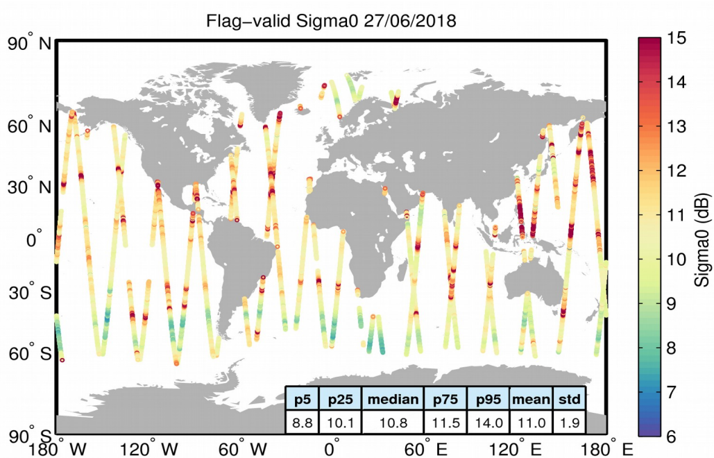
Figure 23. Geographical distribution of flag-valid sigma0 data over oceans and lakes for 27/06/2018. The statistical values shown in the table refer to the sigma0 in dB and are calculated over all measurements shown in the figure.
