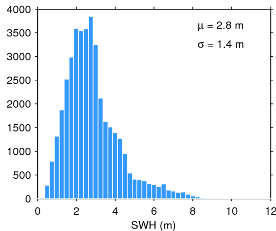
Figure 17. Histogram of flag-valid SWH over oceans and lakes for 25/06/2018. The mean ( \mu ) and standard deviation ( \sigma ) are also shown. Note that values larger than 12 m are excluded from the histogram for the sake of readability but not from the computation of \mu and \sigma .
