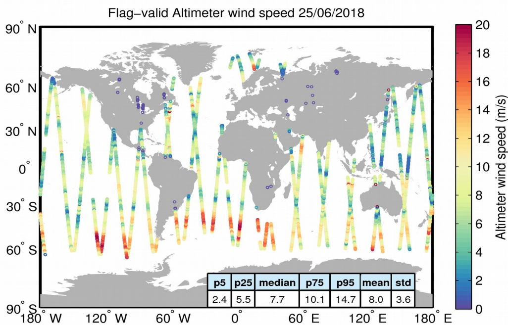
Figure 31. Geographical distribution of flag-valid wind data over oceans and lakes for 25/06/2018. The statistical values shown in the table refer to the wind in m/s and are calculated over all measurements shown in the figure.
