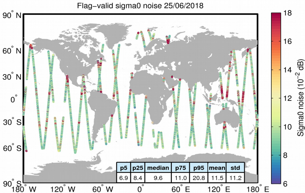
Figure 26. Geographical distribution of flag-valid 20-Hz sigma0 measurement noise over oceans and lakes for 25/06/2018. The statistical values shown in the table refer to the sigma0 noise and are calculated over all measurements shown in the figure.
