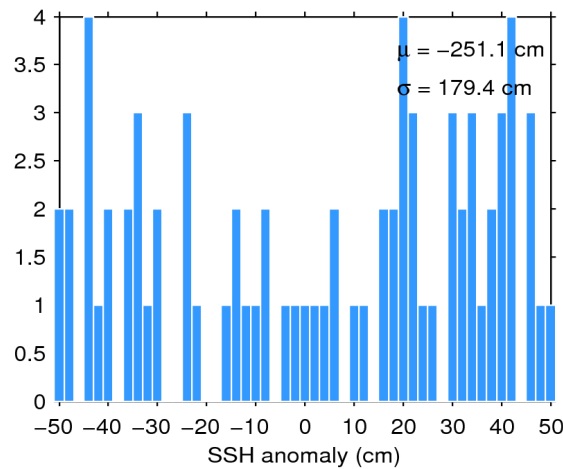
Figure 7. Histogram of flag-valid SSH anomaly over oceans and lakes for 25/06/2018. The mean ( \mu ) and standard deviation ( \sigma ) are also shown. Note that values outside [-50\ 50] cm are excluded from the histogram for the sake of readability but not from the computation of \mu and \sigma .
