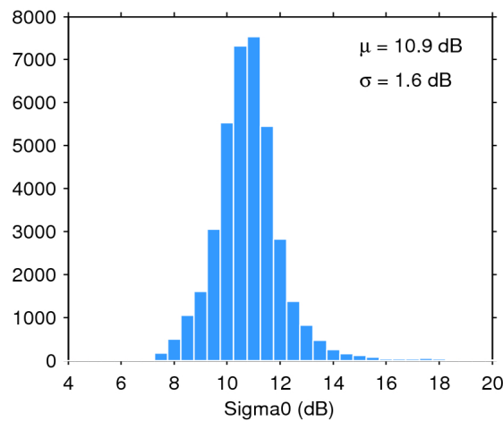
Figure 28. Histogram of science-valid sigma0 over oceans and lakes for 25/06/2018. The mean ( \mu ) and standard deviation ( \sigma ) are also shown. Note that values outside [4 20] dB are excluded from the histogram for the sake of readability but not from the computation of \mu and \sigma .
