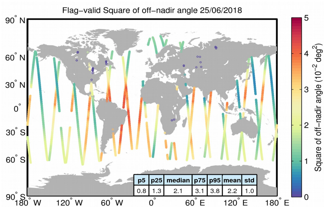
Figure 37. Geographical distribution of flag-valid mispointing data over oceans and lakes for 25/06/2018. The statistical values shown in the table refer to the mispointing in 10^{-2} \text{ deg}^2 and are calculated over all measurements shown in the figure.
