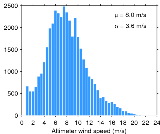
Figure 35. Histogram of science-valid wind over oceans and lakes for 25/06/2018. The mean ( \mu ) and standard deviation ( \sigma ) are also shown. Note that values larger than 24 m/s are excluded from the histogram for the sake of readability but not from the computation of \mu and \sigma .
