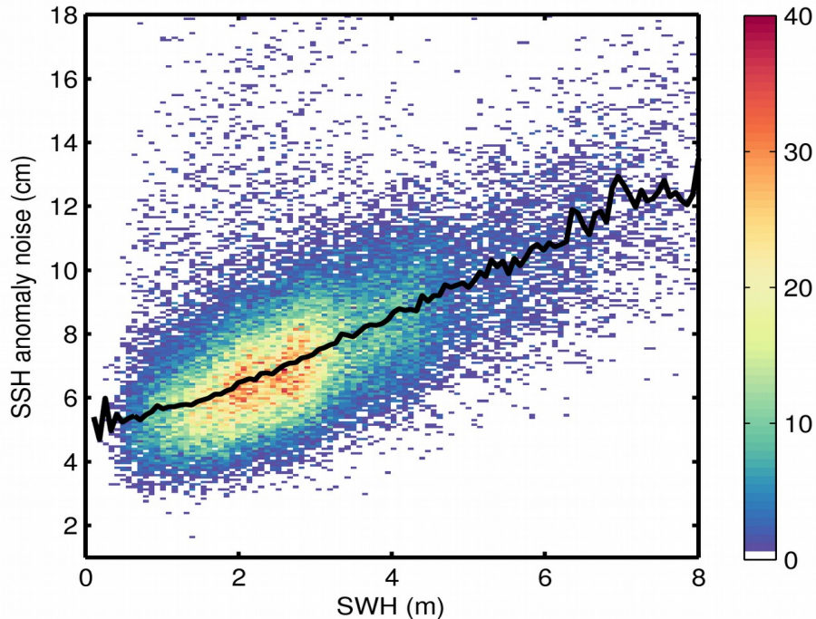
Figure 9. 2D histogram showing flag-valid SSH anomaly noise as a function of SWH for 25/06/2018. The black line denotes the median SSH anomaly noise as a function of SWH.
