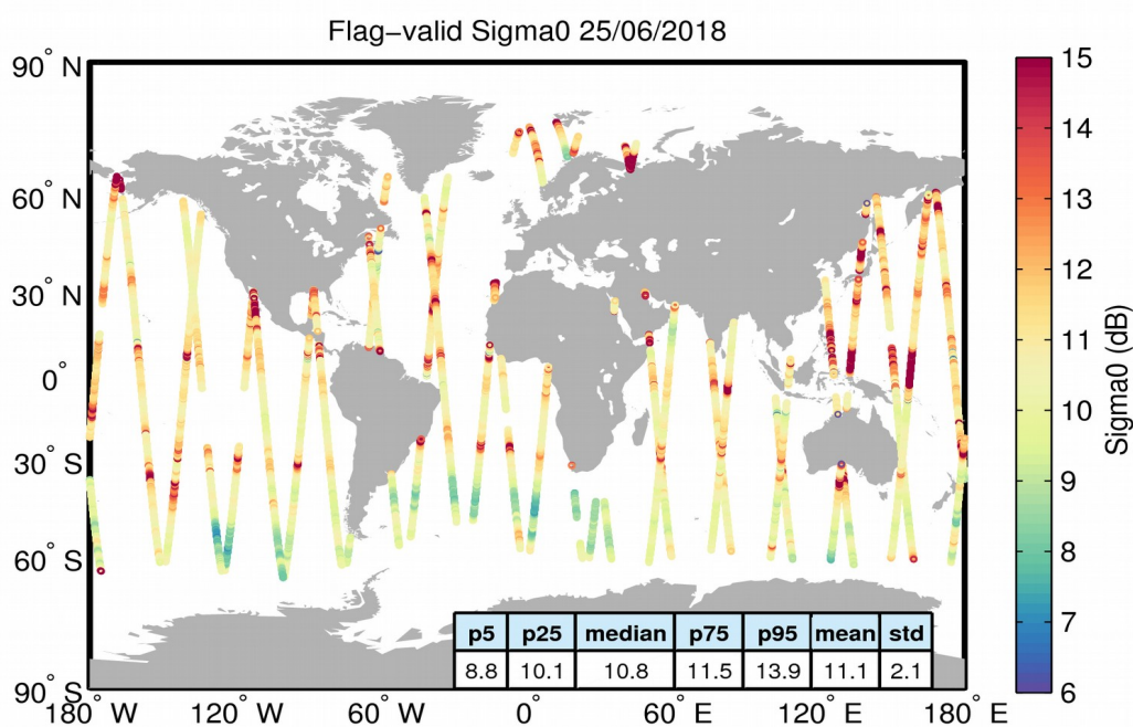
Figure 23. Geographical distribution of flag-valid sigma0 data over oceans and lakes for 25/06/2018. The statistical values shown in the table refer to the sigma0 in dB and are calculated over all measurements shown in the figure.
