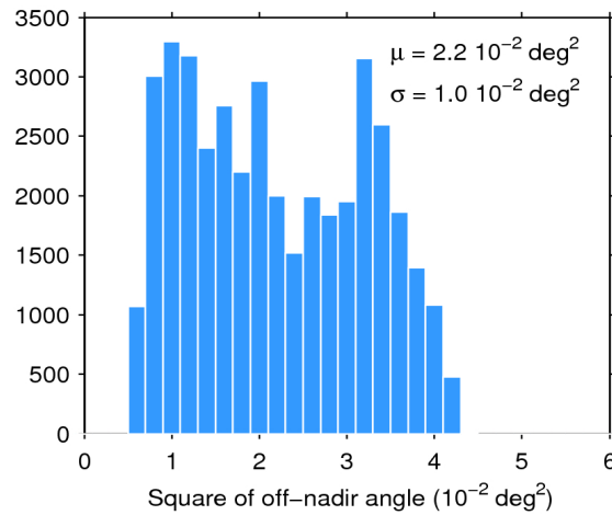
Figure 39. Histogram of flag-valid mispointing over oceans and lakes for 25/06/2018. The mean ( \mu ) and standard deviation ( \sigma ) are also shown. Note that values larger than 6 \cdot 10^{-2} \text{ deg}^2 are excluded from the histogram for the sake of readability but not from the computation of \mu and \sigma .
