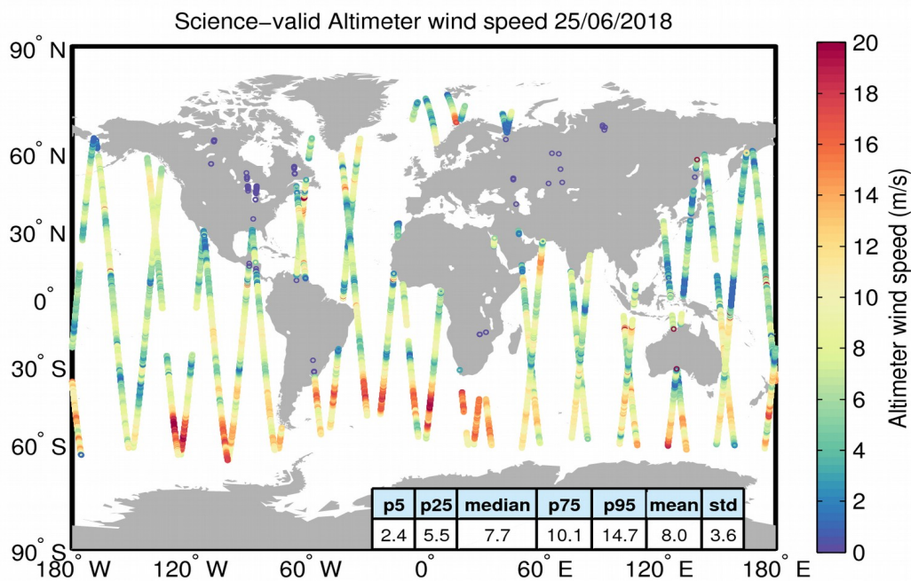
Figure 34. Geographical distribution of science-valid wind data over oceans and lakes for 25/06/2018. The statistical values shown in the table refer to the wind in m/s and are calculated over all measurements shown in the figure. Gray circles denote records that have been rejected based on the editing criteria described in Table 5.
