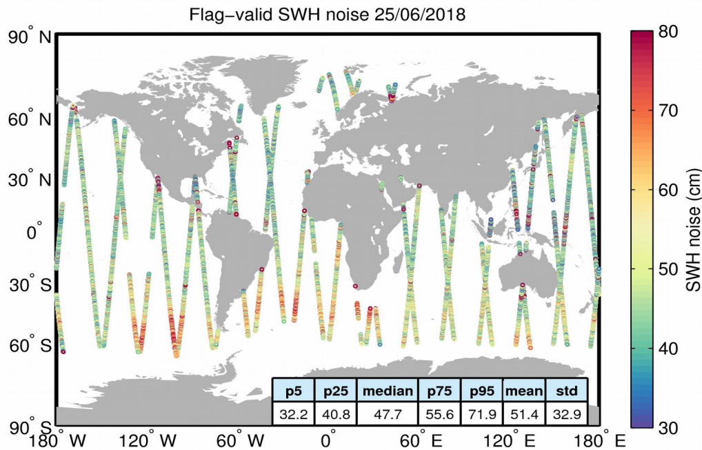
Figure 18. Geographical distribution of flag-valid 20-Hz SWH measurement noise over oceans and lakes for 25/06/2018. The statistical values shown in the figure refer to the SWH noise and are calculated over all measurements shown in the figure.
