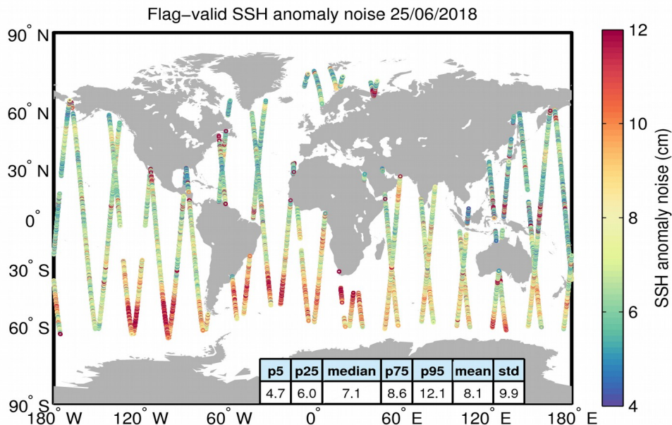
Figure 8. Geographical distribution of flag-valid 20-Hz SSH anomaly measurement noise over oceans and lakes for 25/06/2018. The statistical values shown in the table refer to the SSH anomaly noise and are calculated over all measurements shown in the figure.
