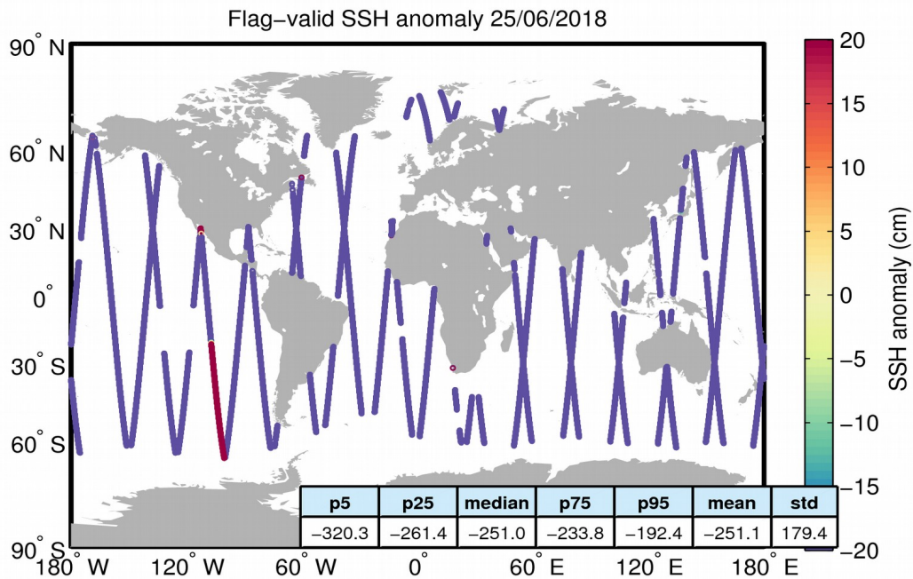
Figure 5. Geographical distribution of flag-valid 1-Hz SSH anomaly data over oceans and lakes for 25/06/2018. The statistical values shown in the table refer to the SSH anomaly in cm and are calculated over all measurements shown in the figure.
