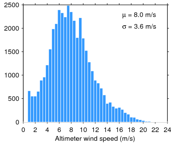
Figure 33. Histogram of flag-valid wind over oceans and lakes for 25/06/2018. The mean ( \mu ) and standard deviation ( \sigma ) are also shown. Note that values larger than 24 m/s are excluded from the histogram for the sake of readability but not from the computation of \mu and \sigma .
