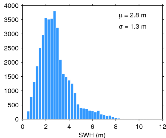
Figure 20. Histogram of science-valid SWH over oceans and lakes for 25/06/2018. The mean ( \mu ) and standard deviation ( \sigma ) are also shown. Note that values larger than 12 m are excluded from the histogram for the sake of readability but not from the computation of \mu and \sigma .
