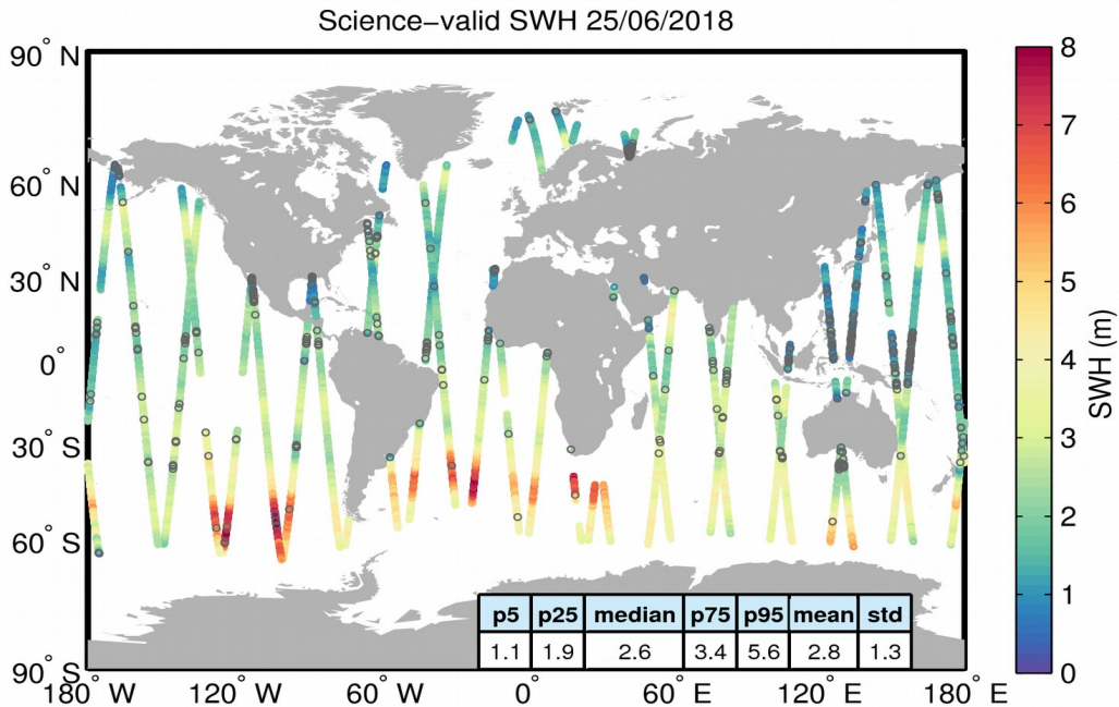
Figure 19. Geographical distribution of science-valid SWH data over oceans and lakes for 25/06/2018. The statistical values shown in the table refer to the SWH in m and are calculated over all measurements shown in the figure. Gray circles denote records that have been rejected based on the editing criteria described in Table 3.
