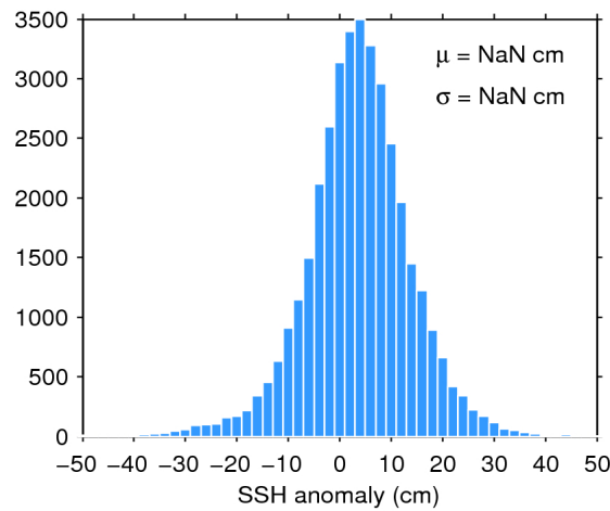
Figure 11. Histogram of science-valid SSH anomaly over oceans and lakes for 25/06/2018. The mean ( \mu ) and standard deviation ( \sigma ) are also shown. Note that values outside [-50 50] cm are excluded from the histogram for the sake of readability but not from the computation of \mu and \sigma .
