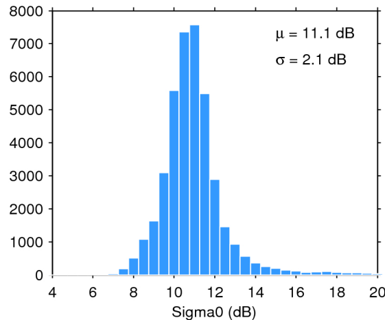
Figure 25. Histogram of flag-valid sigma0 over oceans and lakes for 25/06/2018. The mean ( \mu ) and standard deviation ( \sigma ) are also shown. Note that values outside [4 20] dB are excluded from the histogram for the sake of readability but not from the computation of \mu and \sigma .
