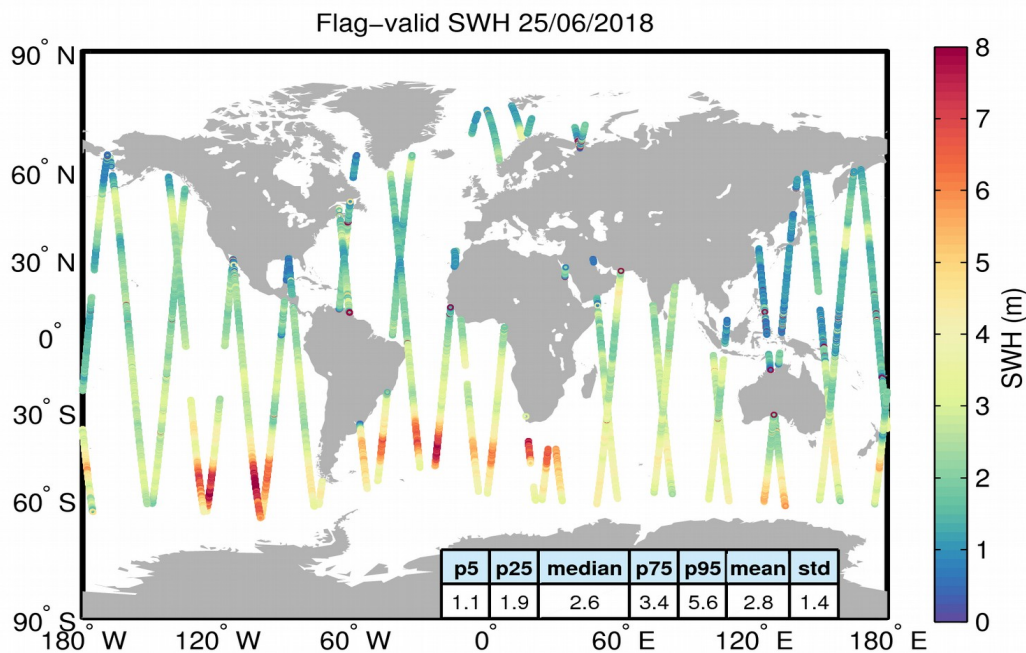
Figure 15. Geographical distribution of flag-valid SWH data over oceans and lakes for 25/06/2018. The statistical values shown in the table refer to the SWH in m and are calculated over all measurements shown in the figure.
