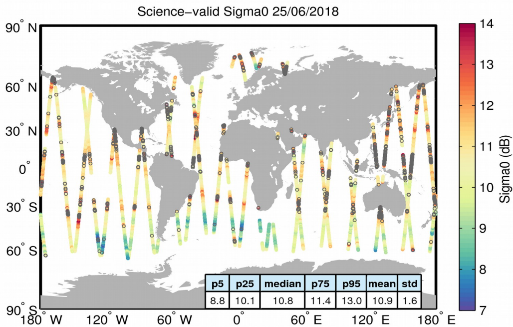
Figure 27. Geographical distribution of science-valid sigma0 data over oceans and lakes for 25/06/2018. The statistical values shown in the table refer to the sigma0 in dB and are calculated over all measurements shown in the figure. Gray circles denote records that have been rejected based on the editing criteria described in Table 4.
