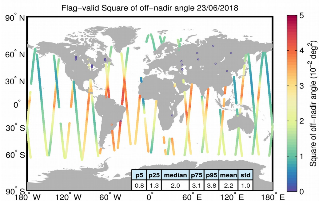
Figure 37. Geographical distribution of flag-valid mispointing data over oceans and lakes for 23/06/2018. The statistical values shown in the table refer to the mispointing in 10^{-2} \text{ deg}^2 and are calculated over all measurements shown in the figure.
