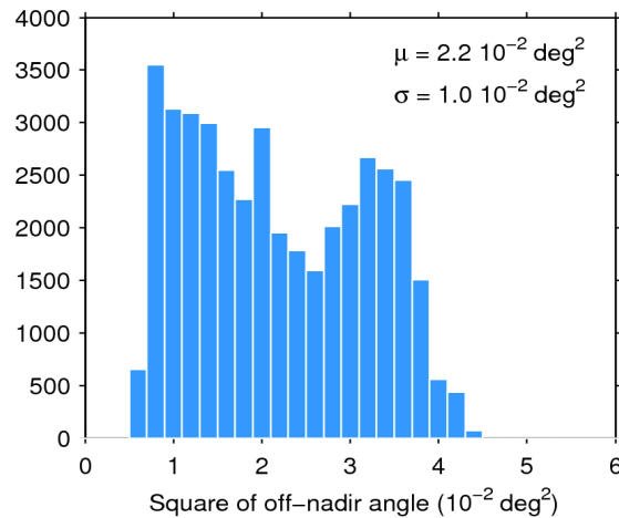
Figure 39. Histogram of flag-valid mispointing over oceans and lakes for 23/06/2018. The mean ( \mu ) and standard deviation ( \sigma ) are also shown. Note that values larger than 6 \cdot 10^{-2} \text{ deg}^2 are excluded from the histogram for the sake of readability but not from the computation of \mu and \sigma .
