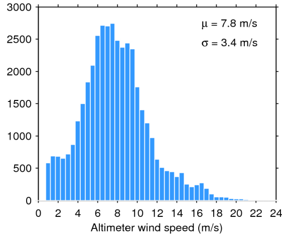
Figure 33. Histogram of flag-valid wind over oceans and lakes for 23/06/2018. The mean ( \mu ) and standard deviation ( \sigma ) are also shown. Note that values larger than 24 m/s are excluded from the histogram for the sake of readability but not from the computation of \mu and \sigma .
