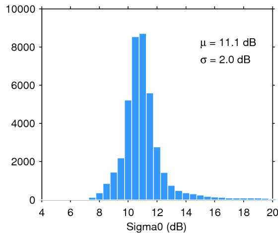
Figure 25. Histogram of flag-valid sigma0 over oceans and lakes for 23/06/2018. The mean ( \mu ) and standard deviation ( \sigma ) are also shown. Note that values outside [4 20] dB are excluded from the histogram for the sake of readability but not from the computation of \mu and \sigma .
