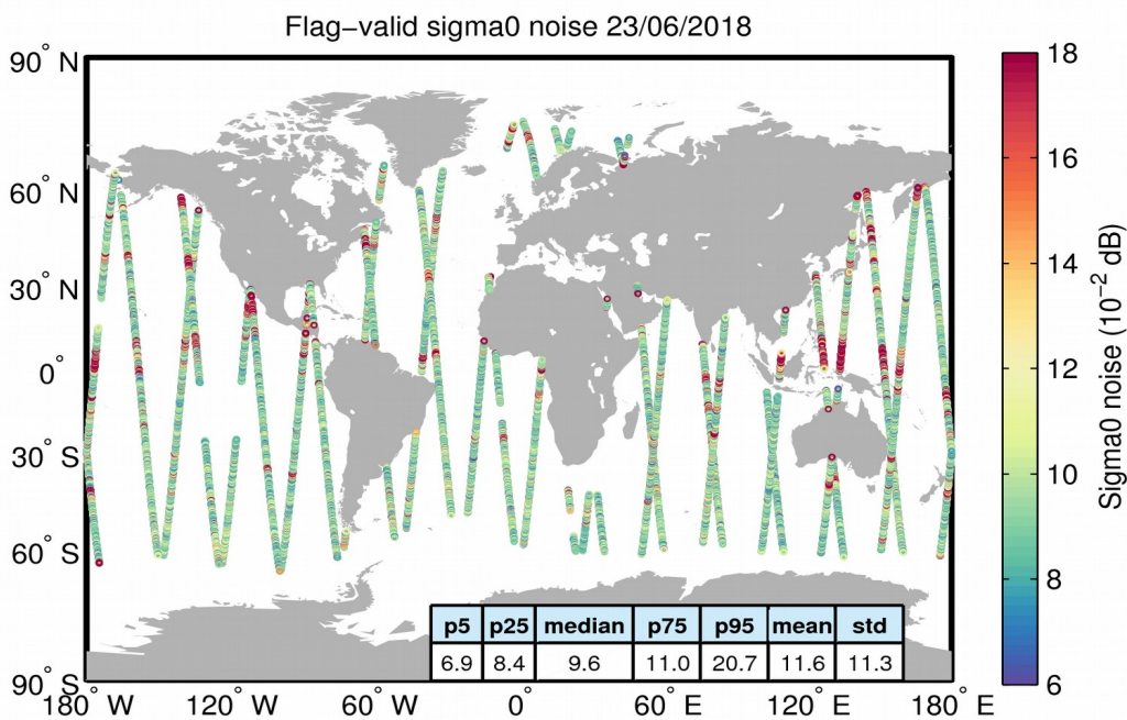
Figure 26. Geographical distribution of flag-valid 20-Hz sigma0 measurement noise over oceans and lakes for 23/06/2018. The statistical values shown in the table refer to the sigma0 noise and are calculated over all measurements shown in the figure.
