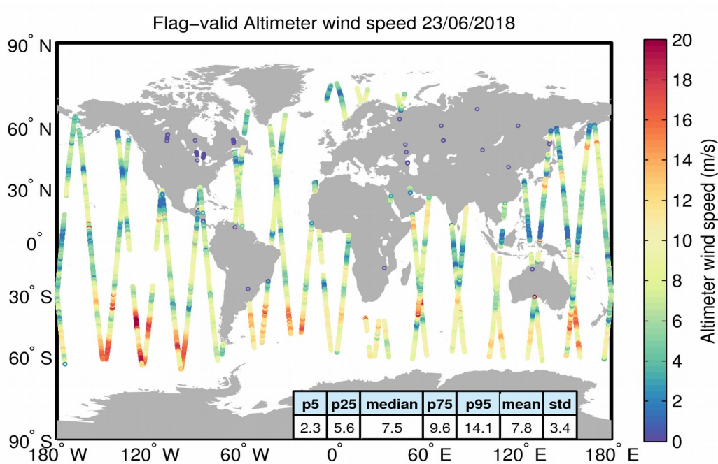
Figure 31. Geographical distribution of flag-valid wind data over oceans and lakes for 23/06/2018. The statistical values shown in the table refer to the wind in m/s and are calculated over all measurements shown in the figure.
