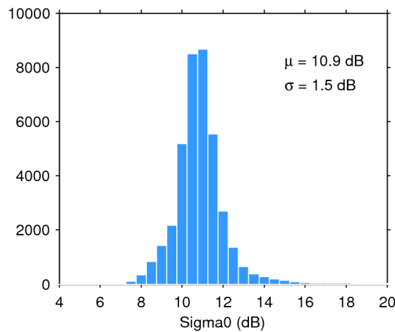
Figure 28. Histogram of science-valid sigma0 over oceans and lakes for 23/06/2018. The mean ( \mu ) and standard deviation ( \sigma ) are also shown. Note that values outside [4 20] dB are excluded from the histogram for the sake of readability but not from the computation of \mu and \sigma .
