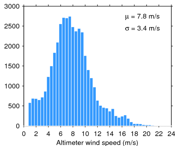
Figure 35. Histogram of science-valid wind over oceans and lakes for 23/06/2018. The mean ( \mu ) and standard deviation ( \sigma ) are also shown. Note that values larger than 24 m/s are excluded from the histogram for the sake of readability but not from the computation of \mu and \sigma .
