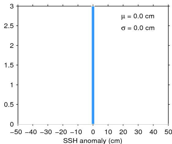
Figure 11. Histogram of science-valid SSH anomaly over oceans and lakes for 23/06/2018. The mean ( \mu ) and standard deviation ( \sigma ) are also shown. Note that values outside [-50 50] cm are excluded from the histogram for the sake of readability but not from the computation of \mu and \sigma .
