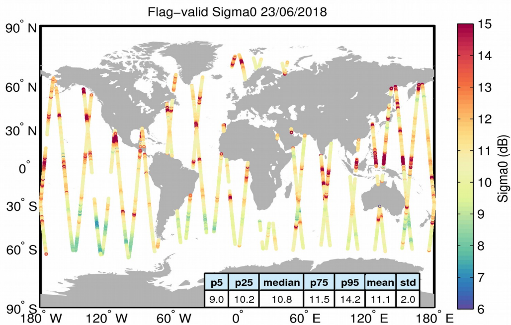
Figure 23. Geographical distribution of flag-valid sigma0 data over oceans and lakes for 23/06/2018. The statistical values shown in the table refer to the sigma0 in dB and are calculated over all measurements shown in the figure.
