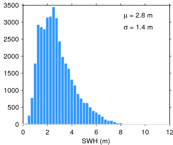
Figure 20. Histogram of science-valid SWH over oceans and lakes for 23/06/2018. The mean ( \mu ) and standard deviation ( \sigma ) are also shown. Note that values larger than 12 m are excluded from the histogram for the sake of readability but not from the computation of \mu and \sigma .
