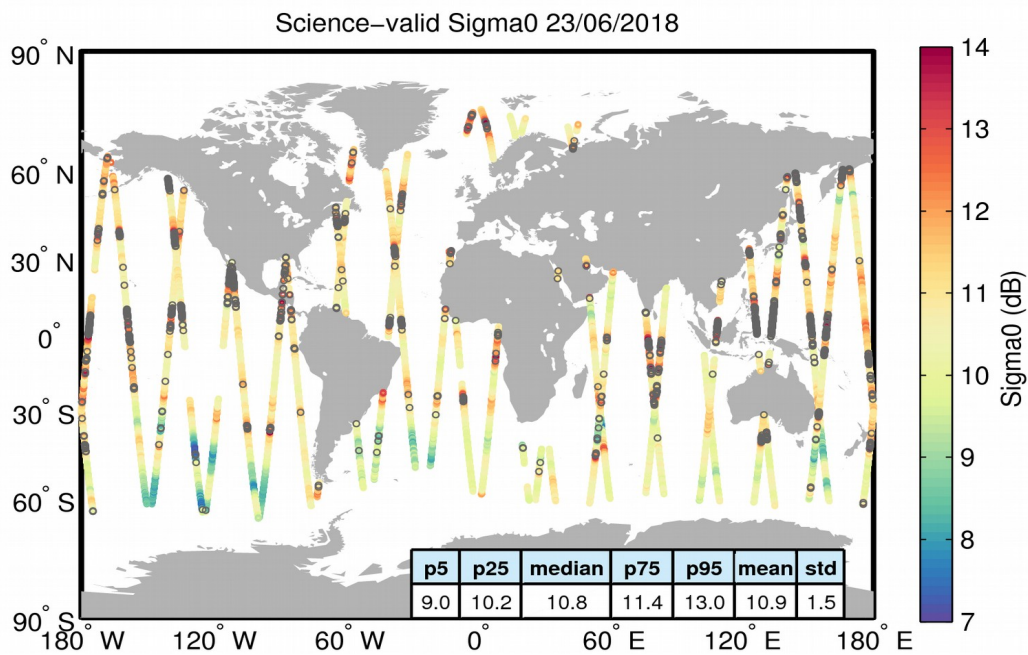
Figure 27. Geographical distribution of science-valid sigma0 data over oceans and lakes for 23/06/2018. The statistical values shown in the table refer to the sigma0 in dB and are calculated over all measurements shown in the figure. Gray circles denote records that have been rejected based on the editing criteria described in Table 4.
