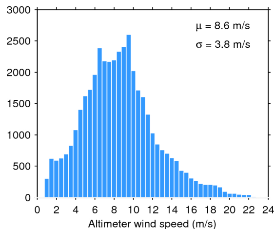
Figure 35. Histogram of science-valid wind over oceans and lakes for 22/06/2018. The mean ( \mu ) and standard deviation ( \sigma ) are also shown. Note that values larger than 24 m/s are excluded from the histogram for the sake of readability but not from the computation of \mu and \sigma .
