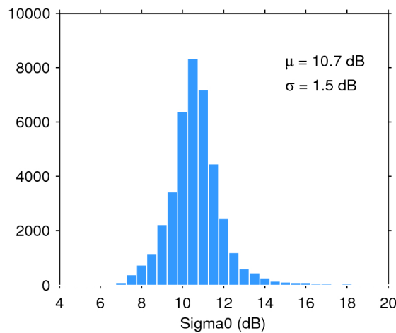
Figure 28. Histogram of science-valid sigma0 over oceans and lakes for 22/06/2018. The mean ( \mu ) and standard deviation ( \sigma ) are also shown. Note that values outside [4 20] dB are excluded from the histogram for the sake of readability but not from the computation of \mu and \sigma .
