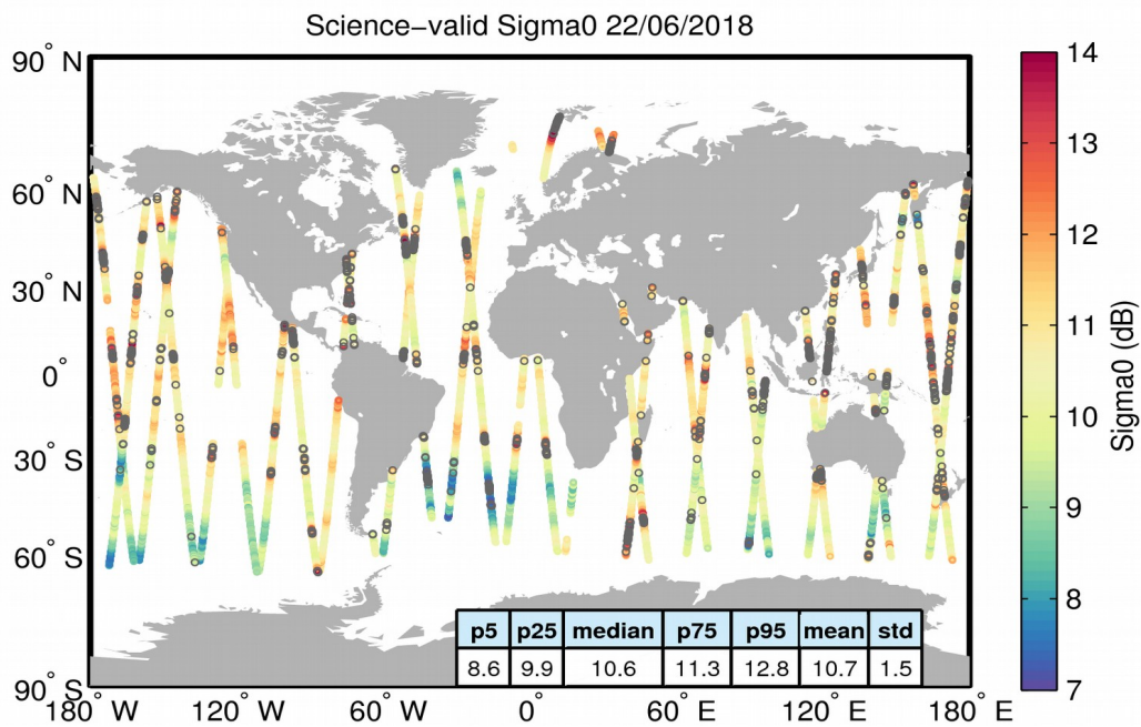
Figure 27. Geographical distribution of science-valid sigma0 data over oceans and lakes for 22/06/2018. The statistical values shown in the table refer to the sigma0 in dB and are calculated over all measurements shown in the figure. Gray circles denote records that have been rejected based on the editing criteria described in Table 4.
