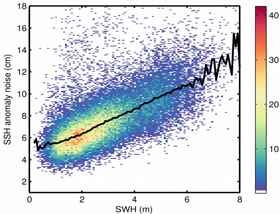
Figure 9. 2D histogram showing flag-valid SSH anomaly noise as a function of SWH for 22/06/2018. The black line denotes the median SSH anomaly noise as a function of SWH.
