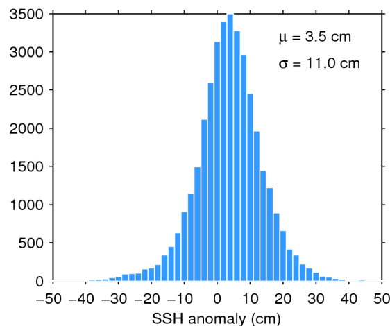
Figure 11. Histogram of science-valid SSH anomaly over oceans and lakes for 22/06/2018. The mean ( \mu ) and standard deviation ( \sigma ) are also shown. Note that values outside [-50 50] cm are excluded from the histogram for the sake of readability but not from the computation of \mu and \sigma .
