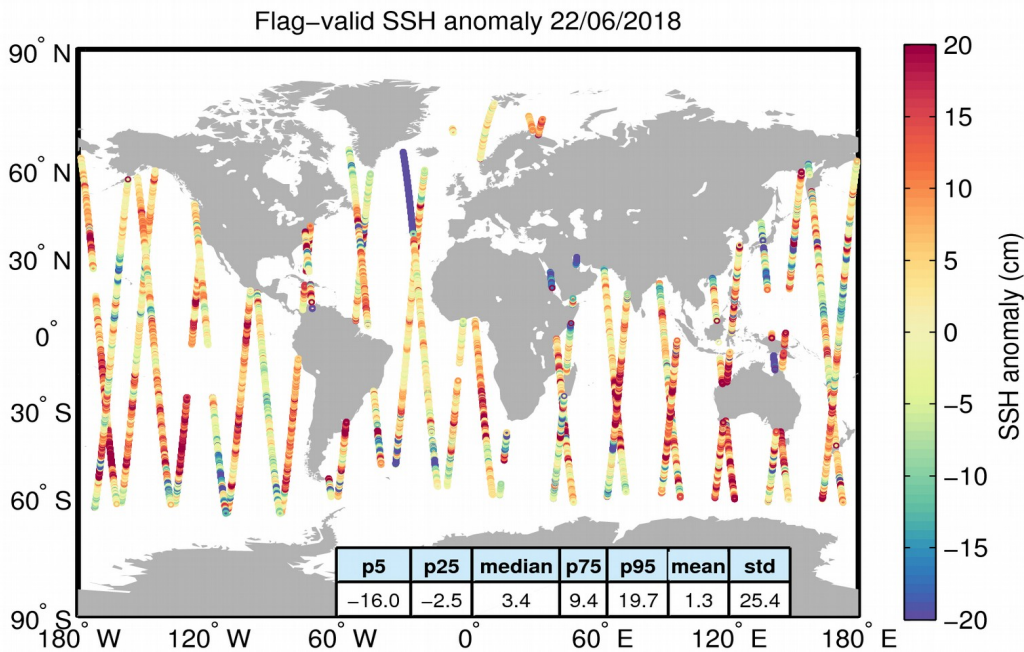
Figure 5. Geographical distribution of flag-valid 1-Hz SSH anomaly data over oceans and lakes for 22/06/2018. The statistical values shown in the table refer to the SSH anomaly in cm and are calculated over all measurements shown in the figure.
