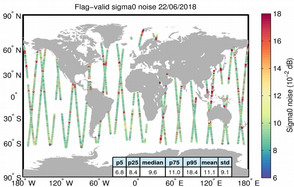
Figure 26. Geographical distribution of flag-valid 20-Hz sigma0 measurement noise over oceans and lakes for 22/06/2018. The statistical values shown in the table refer to the sigma0 noise and are calculated over all measurements shown in the figure.
