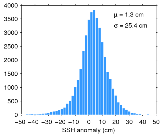
Figure 7. Histogram of flag-valid SSH anomaly over oceans and lakes for 22/06/2018. The mean ( \mu ) and standard deviation ( \sigma ) are also shown. Note that values outside [-50 50] cm are excluded from the histogram for the sake of readability but not from the computation of \mu and \sigma .
