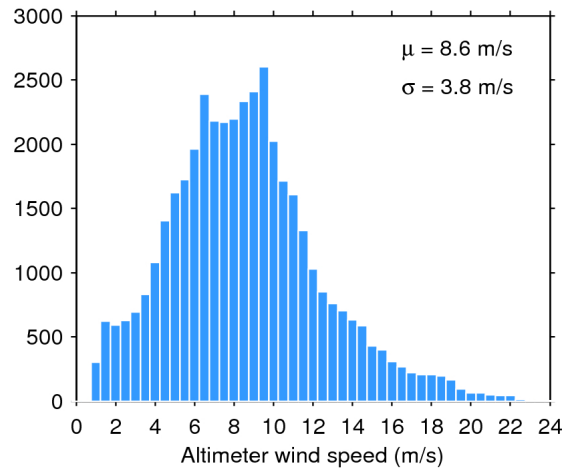
Figure 33. Histogram of flag-valid wind over oceans and lakes for 22/06/2018. The mean ( \mu ) and standard deviation ( \sigma ) are also shown. Note that values larger than 24 m/s are excluded from the histogram for the sake of readability but not from the computation of \mu and \sigma .
