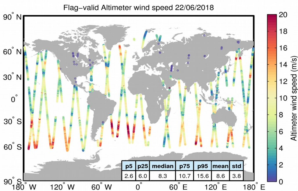
Figure 31. Geographical distribution of flag-valid wind data over oceans and lakes for 22/06/2018. The statistical values shown in the table refer to the wind in m/s and are calculated over all measurements shown in the figure.
