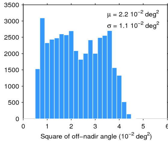
Figure 39. Histogram of flag-valid mispointing over oceans and lakes for 22/06/2018. The mean ( \mu ) and standard deviation ( \sigma ) are also shown. Note that values larger than 6 \cdot 10^{-2} \text{ deg}^2 are excluded from the histogram for the sake of readability but not from the computation of \mu and \sigma .
