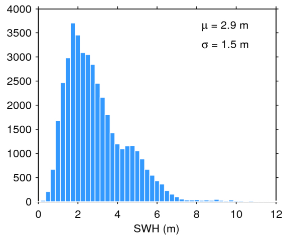
Figure 17. Histogram of flag-valid SWH over oceans and lakes for 22/06/2018. The mean ( \mu ) and standard deviation ( \sigma ) are also shown. Note that values larger than 12 m are excluded from the histogram for the sake of readability but not from the computation of \mu and \sigma .
