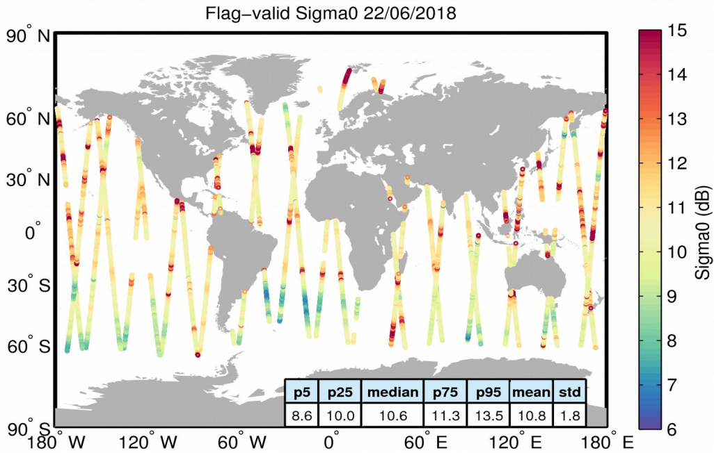
Figure 23. Geographical distribution of flag-valid sigma0 data over oceans and lakes for 22/06/2018. The statistical values shown in the table refer to the sigma0 in dB and are calculated over all measurements shown in the figure.
