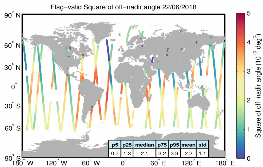
Figure 37. Geographical distribution of flag-valid mispointing data over oceans and lakes for 22/06/2018. The statistical values shown in the table refer to the mispointing in 10^{-2} deg 2 and are calculated over all measurements shown in the figure.
