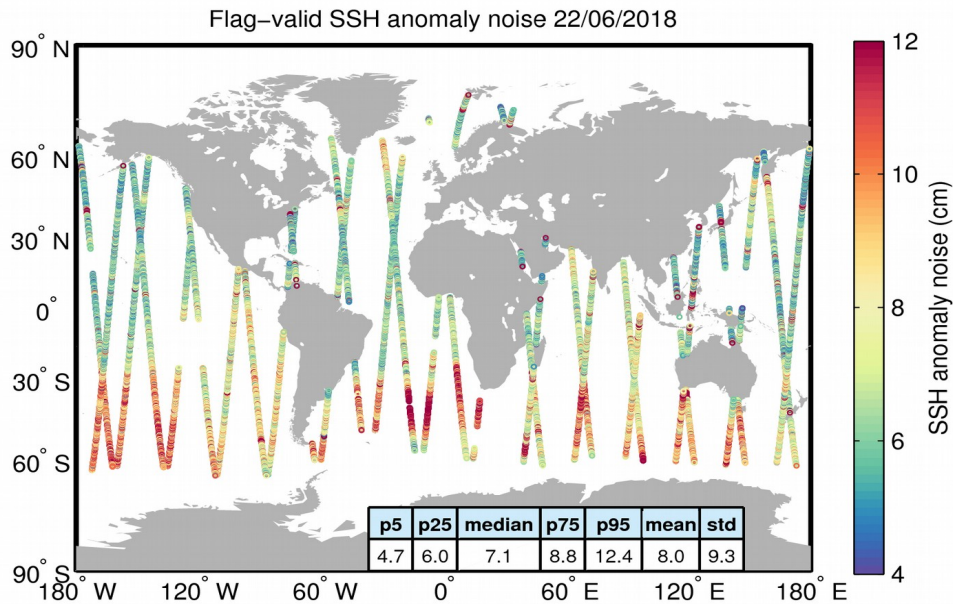
Figure 8. Geographical distribution of flag-valid 20-Hz SSH anomaly measurement noise over oceans and lakes for 22/06/2018. The statistical values shown in the table refer to the SSH anomaly noise and are calculated over all measurements shown in the figure.
