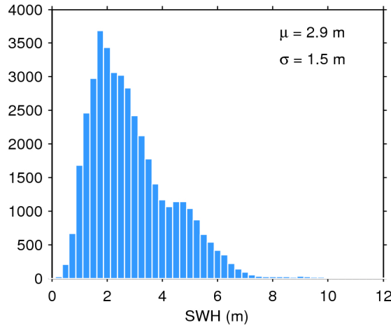
Figure 20. Histogram of science-valid SWH over oceans and lakes for 22/06/2018. The mean ( \mu ) and standard deviation ( \sigma ) are also shown. Note that values larger than 12 m are excluded from the histogram for the sake of readability but not from the computation of \mu and \sigma .
