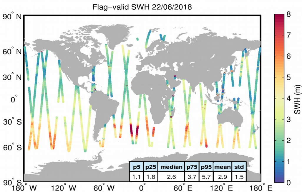
Figure 15. Geographical distribution of flag-valid SWH data over oceans and lakes for 22/06/2018. The statistical values shown in the table refer to the SWH in m and are calculated over all measurements shown in the figure.
