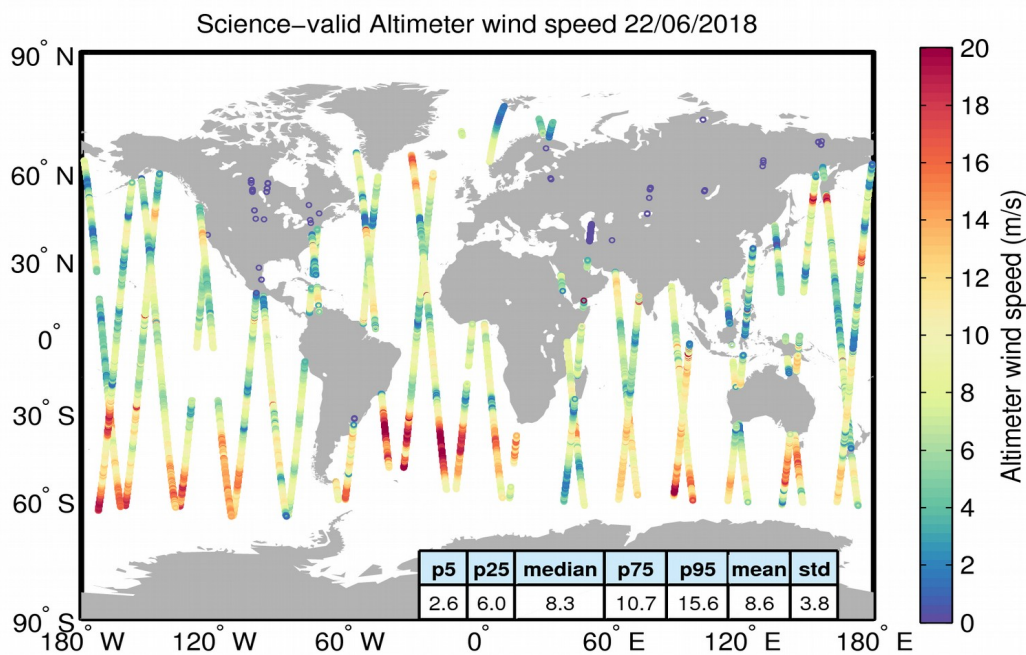
Figure 34. Geographical distribution of science-valid wind data over oceans and lakes for 22/06/2018. The statistical values shown in the table refer to the wind in m/s and are calculated over all measurements shown in the figure. Gray circles denote records that have been rejected based on the editing criteria described in Table 5.
