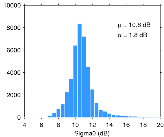
Figure 25. Histogram of flag-valid sigma0 over oceans and lakes for 22/06/2018. The mean ( \mu ) and standard deviation ( \sigma ) are also shown. Note that values outside [4 20] dB are excluded from the histogram for the sake of readability but not from the computation of \mu and \sigma .
