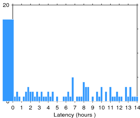
Figure 2. Histogram of the data latency for 22/06/2018. The y-axis denotes the number of files that are made available with a delay of x-hours with respect to the mean time of the records stored in the file.
