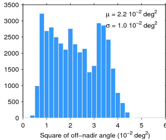
Figure 39. Histogram of flag-valid mispointing over oceans and lakes for 21/06/2018. The mean ( \mu ) and standard deviation ( \sigma ) are also shown. Note that values larger than 6 \cdot 10^{-2} \text{ deg}^2 are excluded from the histogram for the sake of readability but not from the computation of \mu and \sigma .
