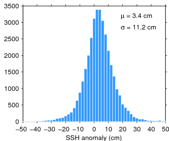
Figure 11. Histogram of science-valid SSH anomaly over oceans and lakes for 21/06/2018. The mean ( \mu ) and standard deviation ( \sigma ) are also shown. Note that values outside [-50 50] cm are excluded from the histogram for the sake of readability but not from the computation of \mu and \sigma .
