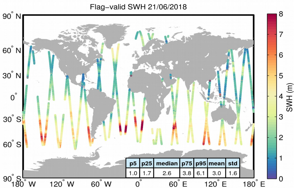
Figure 15. Geographical distribution of flag-valid SWH data over oceans and lakes for 21/06/2018. The statistical values shown in the table refer to the SWH in m and are calculated over all measurements shown in the figure.
