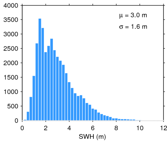
Figure 17. Histogram of flag-valid SWH over oceans and lakes for 21/06/2018. The mean ( \mu ) and standard deviation ( \sigma ) are also shown. Note that values larger than 12 m are excluded from the histogram for the sake of readability but not from the computation of \mu and \sigma .
