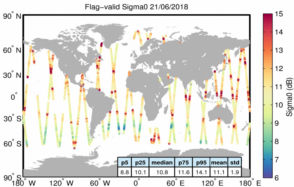
Figure 23. Geographical distribution of flag-valid sigma0 data over oceans and lakes for 21/06/2018. The statistical values shown in the table refer to the sigma0 in dB and are calculated over all measurements shown in the figure.
