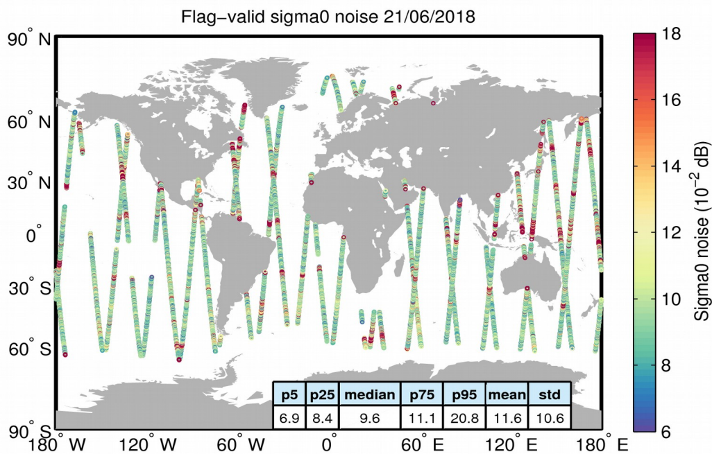
Figure 26. Geographical distribution of flag-valid 20-Hz sigma0 measurement noise over oceans and lakes for 21/06/2018. The statistical values shown in the table refer to the sigma0 noise and are calculated over all measurements shown in the figure.
