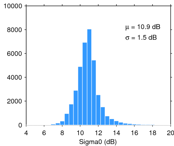
Figure 28. Histogram of science-valid sigma0 over oceans and lakes for 21/06/2018. The mean ( \mu ) and standard deviation ( \sigma ) are also shown. Note that values outside [4 20] dB are excluded from the histogram for the sake of readability but not from the computation of \mu and \sigma .
