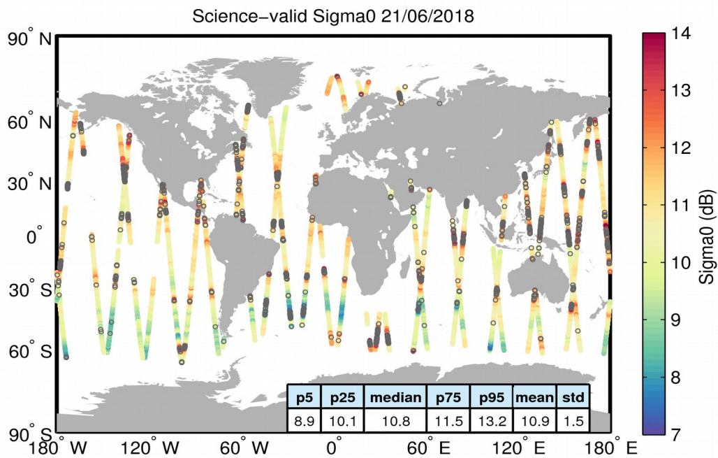
Figure 27. Geographical distribution of science-valid sigma0 data over oceans and lakes for 21/06/2018. The statistical values shown in the table refer to the sigma0 in dB and are calculated over all measurements shown in the figure. Gray circles denote records that have been rejected based on the editing criteria described in Table 4.
