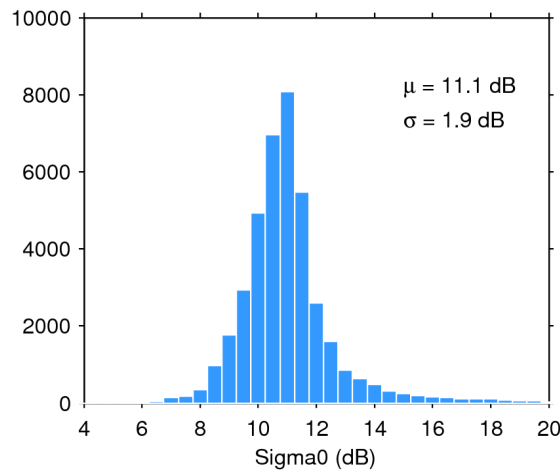
Figure 25. Histogram of flag-valid sigma0 over oceans and lakes for 21/06/2018. The mean ( \mu ) and standard deviation ( \sigma ) are also shown. Note that values outside [4 20] dB are excluded from the histogram for the sake of readability but not from the computation of \mu and \sigma .
