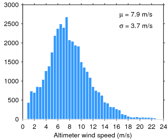
Figure 33. Histogram of flag-valid wind over oceans and lakes for 21/06/2018. The mean ( \mu ) and standard deviation ( \sigma ) are also shown. Note that values larger than 24 m/s are excluded from the histogram for the sake of readability but not from the computation of \mu and \sigma .
