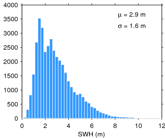
Figure 20. Histogram of science-valid SWH over oceans and lakes for 21/06/2018. The mean ( \mu ) and standard deviation ( \sigma ) are also shown. Note that values larger than 12 m are excluded from the histogram for the sake of readability but not from the computation of \mu and \sigma .
