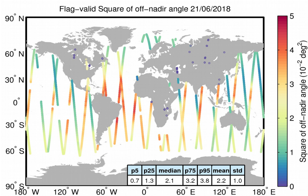
Figure 37. Geographical distribution of flag-valid mispointing data over oceans and lakes for 21/06/2018. The statistical values shown in the table refer to the mispointing in 10^{-2} \text{ deg}^2 and are calculated over all measurements shown in the figure.
