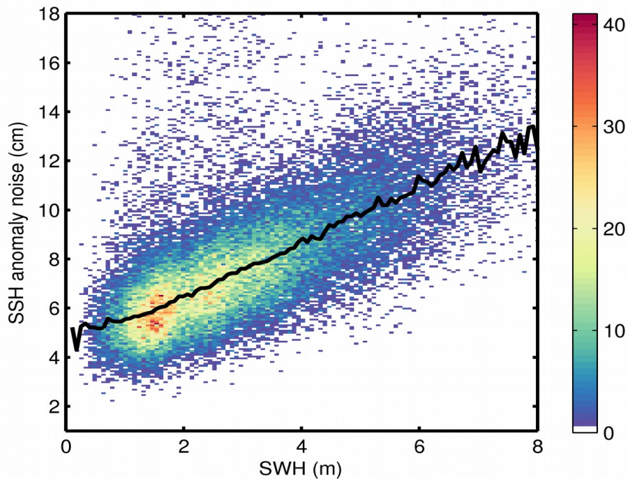
Figure 9. 2D histogram showing flag-valid SSH anomaly noise as a function of SWH for 21/06/2018. The black line denotes the median SSH anomaly noise as a function of SWH.
