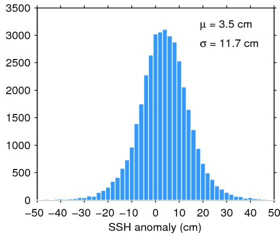
Figure 11. Histogram of science-valid SSH anomaly over oceans and lakes for 19/06/2018. The mean ( \mu ) and standard deviation ( \sigma ) are also shown. Note that values outside [-50 50] cm are excluded from the histogram for the sake of readability but not from the computation of \mu and \sigma .
