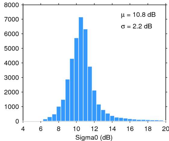
Figure 25. Histogram of flag-valid sigma0 over oceans and lakes for 19/06/2018. The mean ( \mu ) and standard deviation ( \sigma ) are also shown. Note that values outside [4 20] dB are excluded from the histogram for the sake of readability but not from the computation of \mu and \sigma .
