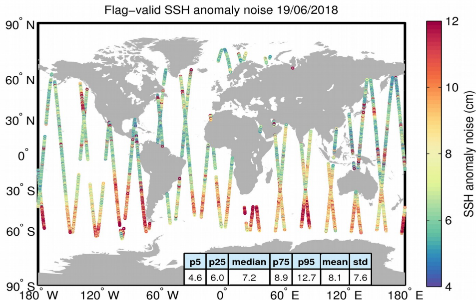
Figure 8. Geographical distribution of flag-valid 20-Hz SSH anomaly measurement noise over oceans and lakes for 19/06/2018. The statistical values shown in the table refer to the SSH anomaly noise and are calculated over all measurements shown in the figure.
