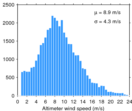
Figure 35. Histogram of science-valid wind over oceans and lakes for 19/06/2018. The mean ( \mu ) and standard deviation ( \sigma ) are also shown. Note that values larger than 24 m/s are excluded from the histogram for the sake of readability but not from the computation of \mu and \sigma .
