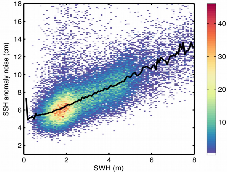
Figure 9. 2D histogram showing flag-valid SSH anomaly noise as a function of SWH for 19/06/2018. The black line denotes the median SSH anomaly noise as a function of SWH.
