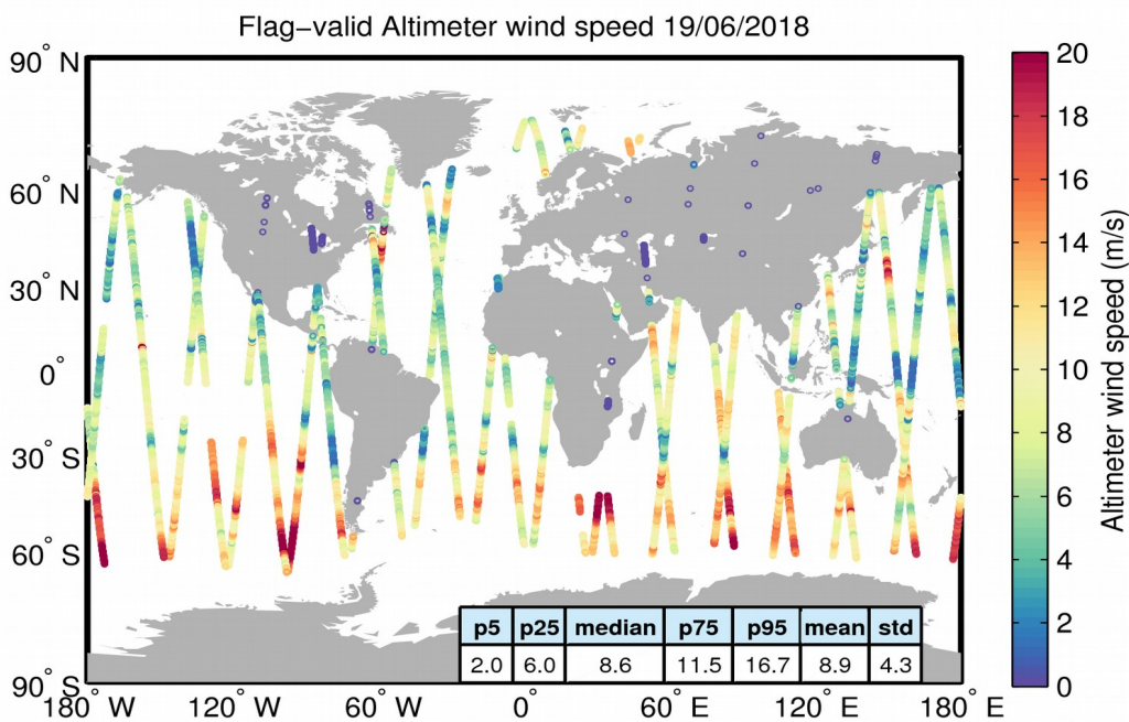
Figure 31. Geographical distribution of flag-valid wind data over oceans and lakes for 19/06/2018. The statistical values shown in the table refer to the wind in m/s and are calculated over all measurements shown in the figure.
