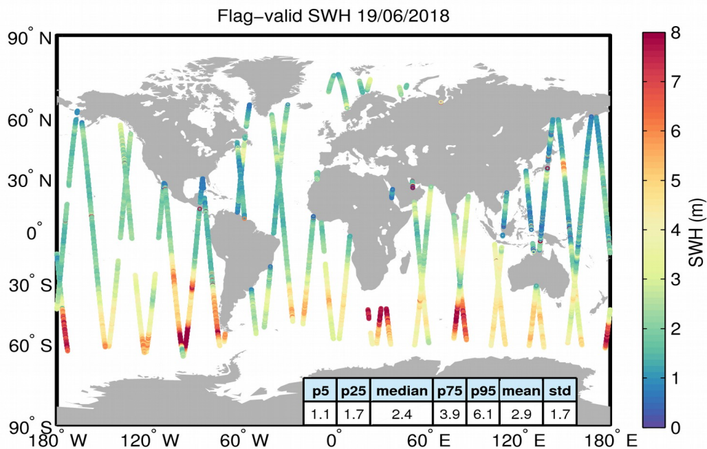
Figure 15. Geographical distribution of flag-valid SWH data over oceans and lakes for 19/06/2018. The statistical values shown in the table refer to the SWH in m and are calculated over all measurements shown in the figure.
