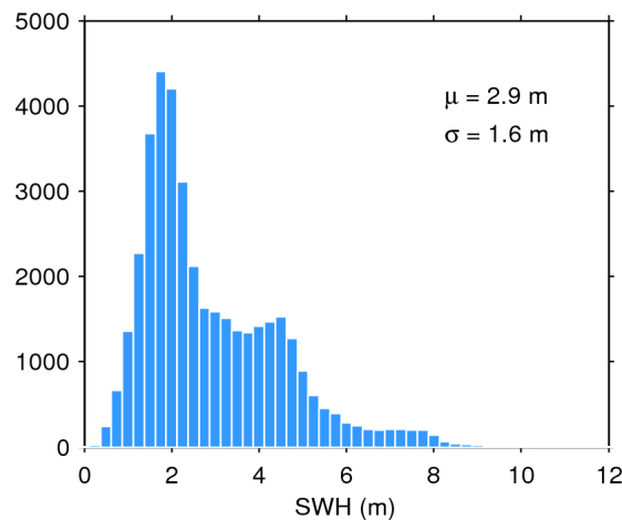
Figure 20. Histogram of science-valid SWH over oceans and lakes for 19/06/2018. The mean ( \mu ) and standard deviation ( \sigma ) are also shown. Note that values larger than 12 m are excluded from the histogram for the sake of readability but not from the computation of \mu and \sigma .
