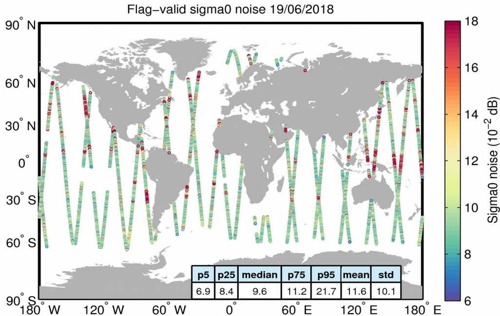
Figure 26. Geographical distribution of flag-valid 20-Hz sigma0 measurement noise over oceans and lakes for 19/06/2018. The statistical values shown in the table refer to the sigma0 noise and are calculated over all measurements shown in the figure.
