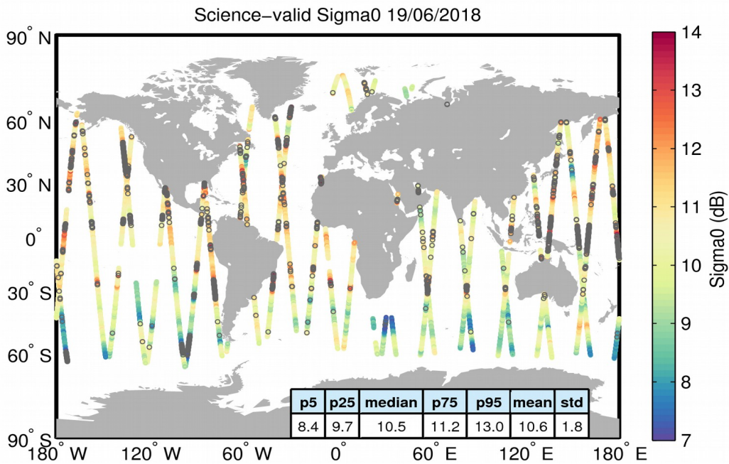
Figure 27. Geographical distribution of science-valid sigma0 data over oceans and lakes for 19/06/2018. The statistical values shown in the table refer to the sigma0 in dB and are calculated over all measurements shown in the figure. Gray circles denote records that have been rejected based on the editing criteria described in Table 4.
