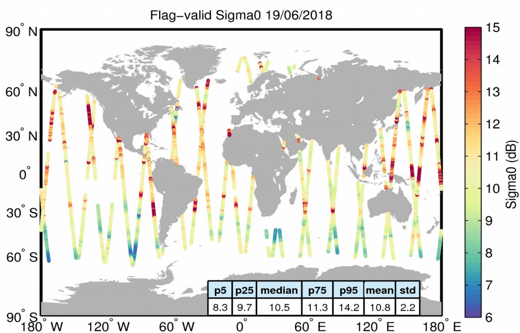
Figure 23. Geographical distribution of flag-valid sigma0 data over oceans and lakes for 19/06/2018. The statistical values shown in the table refer to the sigma0 in dB and are calculated over all measurements shown in the figure.
