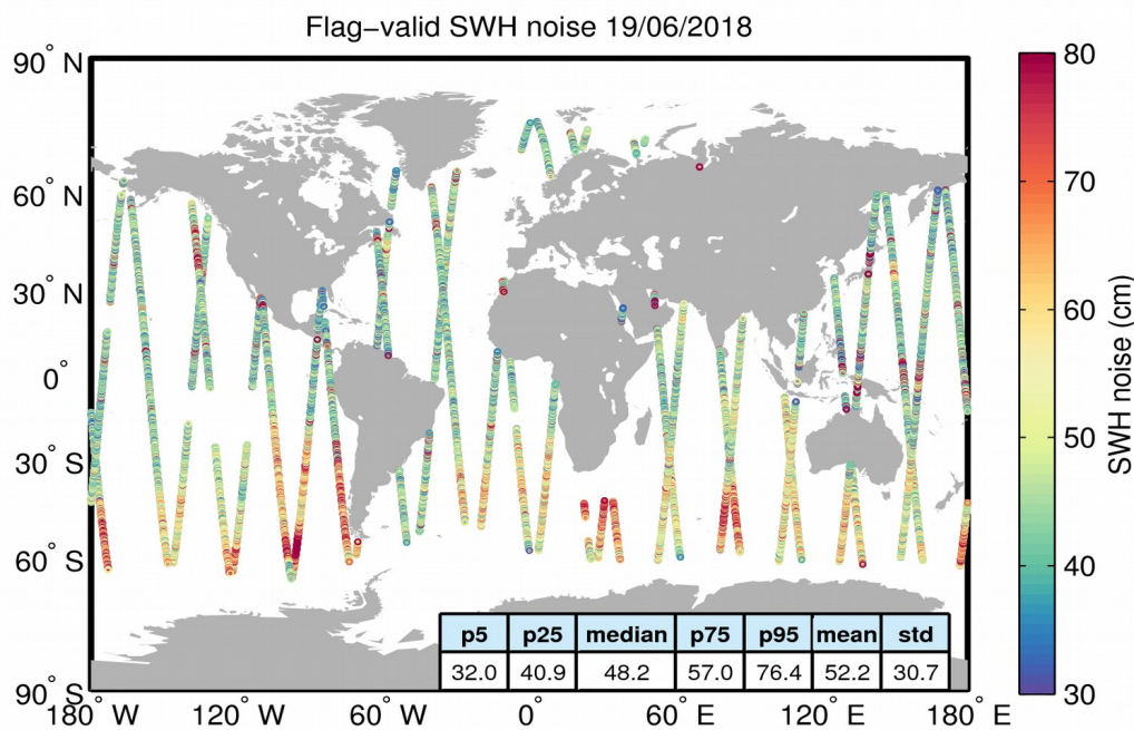
Figure 18. Geographical distribution of flag-valid 20-Hz SWH measurement noise over oceans and lakes for 19/06/2018. The statistical values shown in the table refer to the SWH noise and are calculated over all measurements shown in the figure.
