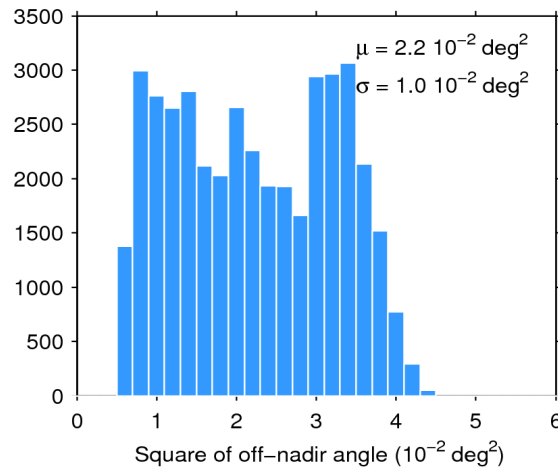
Figure 39. Histogram of flag-valid mispointing over oceans and lakes for 19/06/2018. The mean ( \mu ) and standard deviation ( \sigma ) are also shown. Note that values larger than 6 \cdot 10^{-2} \text{ deg}^2 are excluded from the histogram for the sake of readability but not from the computation of \mu and \sigma .
