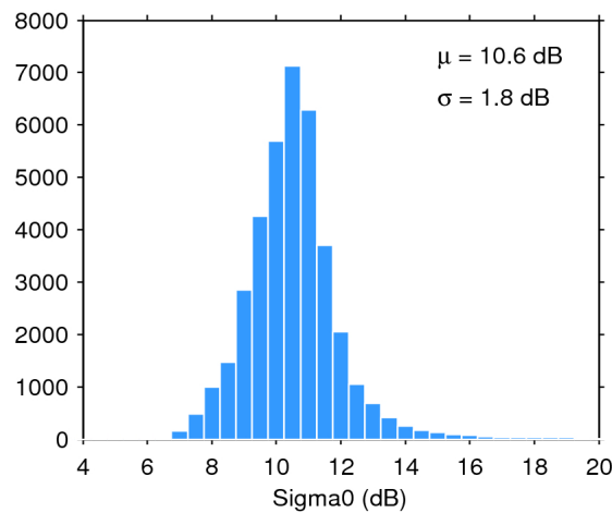
Figure 28. Histogram of science-valid sigma0 over oceans and lakes for 19/06/2018. The mean ( \mu ) and standard deviation ( \sigma ) are also shown. Note that values outside [4 20] dB are excluded from the histogram for the sake of readability but not from the computation of \mu and \sigma .
