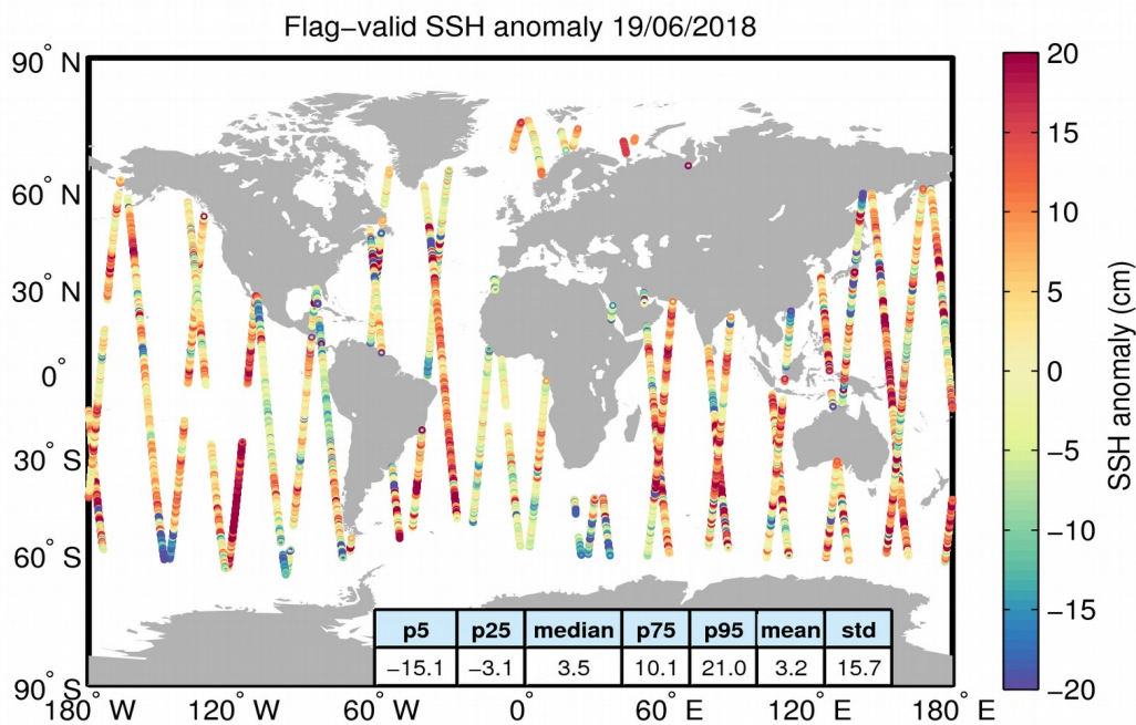
Figure 5. Geographical distribution of flag-valid 1-Hz SSH anomaly data over oceans and lakes for 19/06/2018. The statistical values shown in the table refer to the SSH anomaly in cm and are calculated over all measurements shown in the figure.
