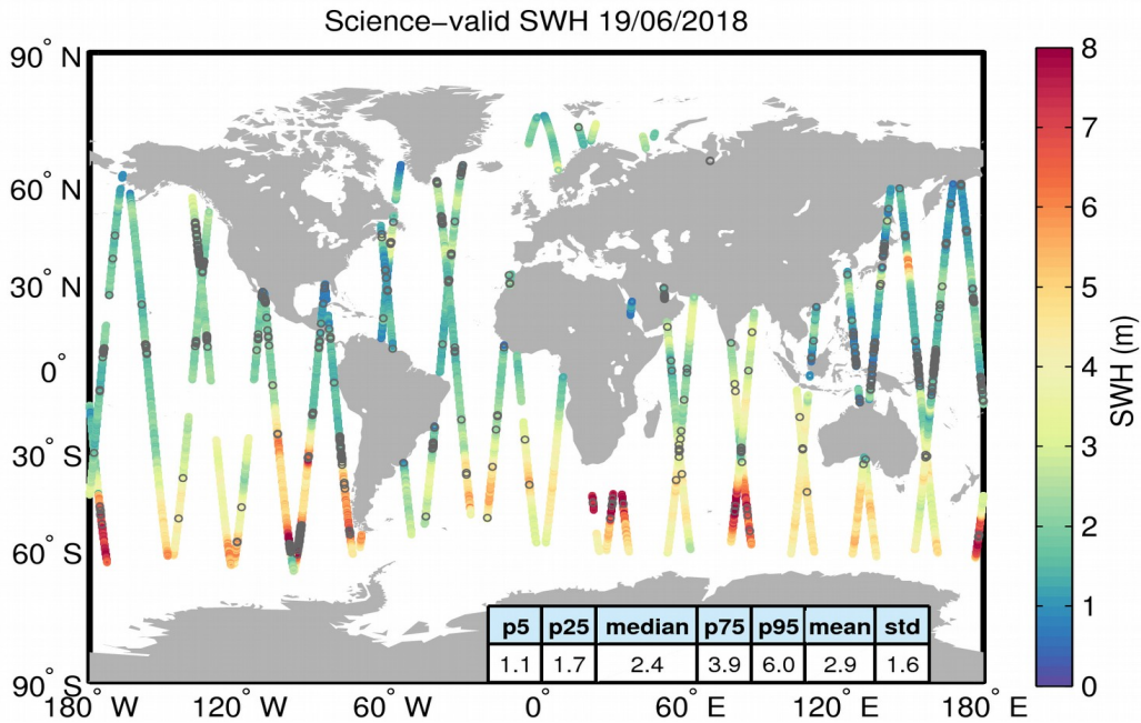
Figure 19. Geographical distribution of science-valid SWH data over oceans and lakes for 19/06/2018. The statistical values shown in the table refer to the SWH in m and are calculated over all measurements shown in the figure. Gray circles denote records that have been rejected based on the editing criteria described in Table 3.
