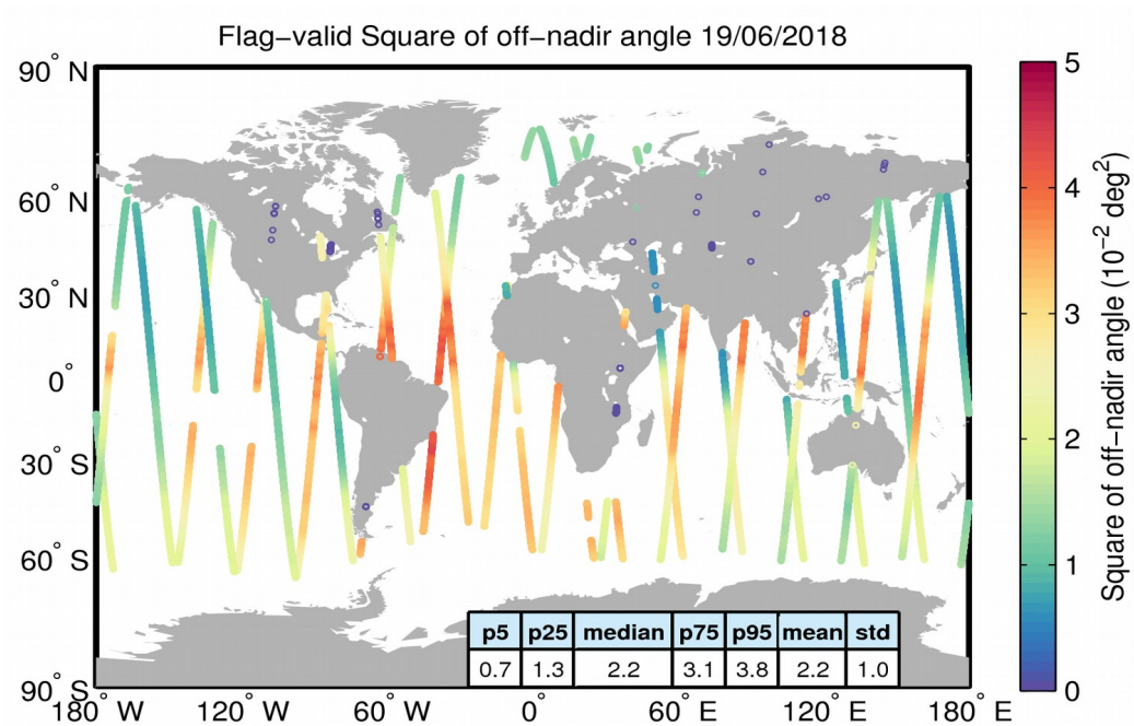
Figure 37. Geographical distribution of flag-valid mispointing data over oceans and lakes for 19/06/2018. The statistical values shown in the table refer to the mispointing in 10^{-2} \text{deg}^2 and are calculated over all measurements shown in the figure.
