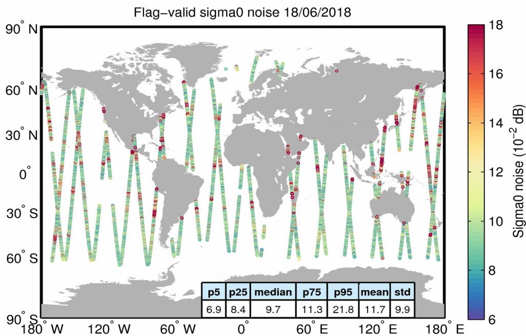
Figure 26. Geographical distribution of flag-valid 20-Hz sigma0 measurement noise over oceans and lakes for 18/06/2018. The statistical values shown in the table refer to the sigma0 noise and are calculated over all measurements shown in the figure.
