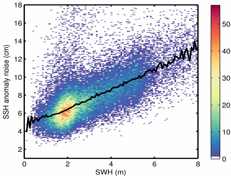
Figure 9. 2D histogram showing flag-valid SSH anomaly noise as a function of SWH for 18/06/2018. The black line denotes the median SSH anomaly noise as a function of SWH.
