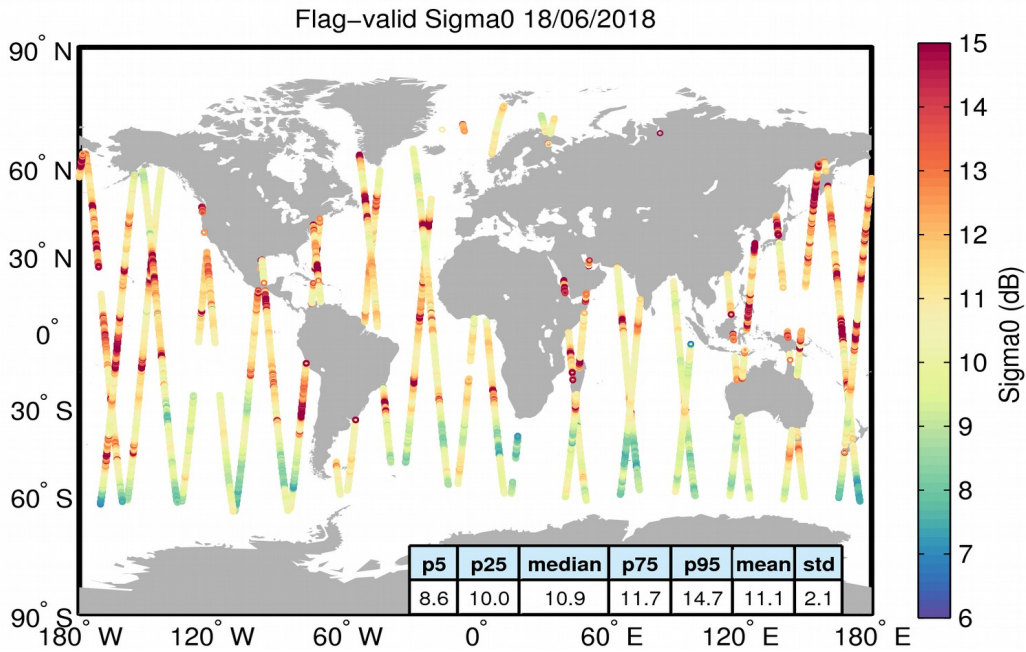
Figure 23. Geographical distribution of flag-valid sigma0 data over oceans and lakes for 18/06/2018. The statistical values shown in the table refer to the sigma0 in dB and are calculated over all measurements shown in the figure.
