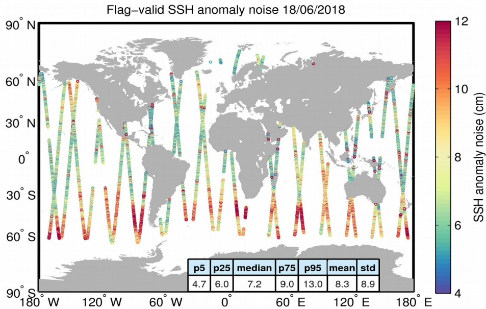
Figure 8. Geographical distribution of flag-valid 20-Hz SSH anomaly measurement noise over oceans and lakes for 18/06/2018. The statistical values shown in the table refer to the SSH anomaly noise and are calculated over all measurements shown in the figure.
