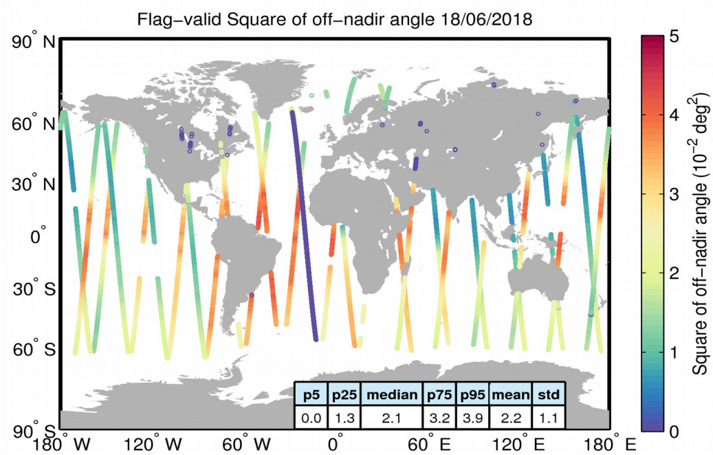
Figure 37. Geographical distribution of flag-valid mispointing data over oceans and lakes for 18/06/2018. The statistical values shown in the table refer to the mispointing in 10^{-2} \text{ deg}^2 and are calculated over all measurements shown in the figure.
