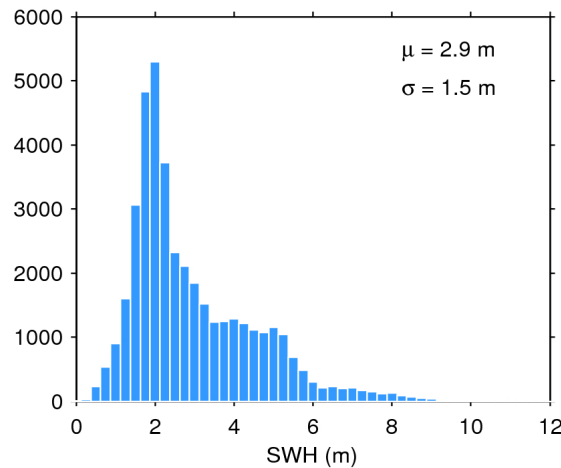
Figure 20. Histogram of science-valid SWH over oceans and lakes for 18/06/2018. The mean ( \mu ) and standard deviation ( \sigma ) are also shown. Note that values larger than 12 m are excluded from the histogram for the sake of readability but not from the computation of \mu and \sigma .
