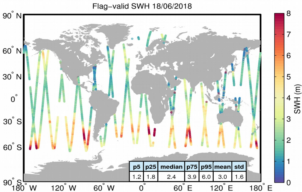
Figure 15. Geographical distribution of flag-valid SWH data over oceans and lakes for 18/06/2018. The statistical values shown in the table refer to the SWH in m and are calculated over all measurements shown in the figure.
