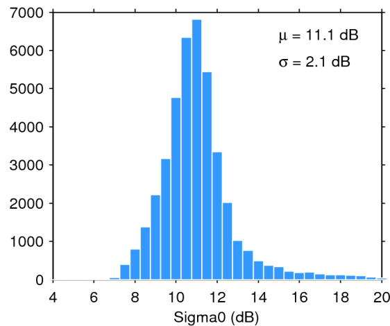
Figure 25. Histogram of flag-valid sigma0 over oceans and lakes for 18/06/2018. The mean ( \mu ) and standard deviation ( \sigma ) are also shown. Note that values outside [4 20] dB are excluded from the histogram for the sake of readability but not from the computation of \mu and \sigma .
