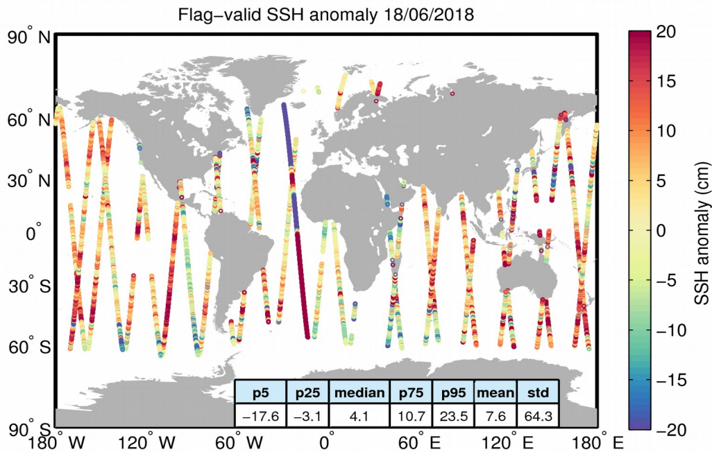
Figure 5. Geographical distribution of flag-valid 1-Hz SSH anomaly data over oceans and lakes for 18/06/2018. The statistical values shown in the table refer to the SSH anomaly in cm and are calculated over all measurements shown in the figure.
