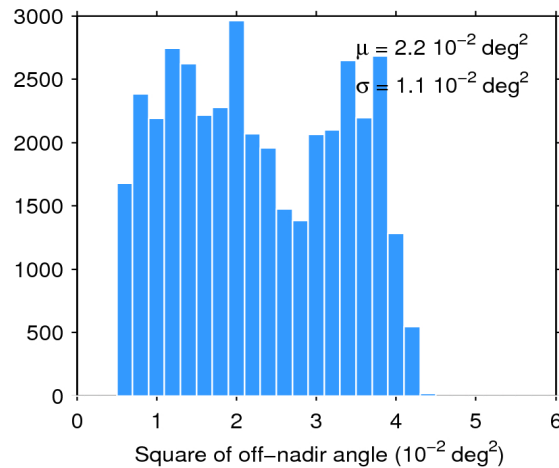
Figure 39. Histogram of flag-valid mispointing over oceans and lakes for 18/06/2018. The mean ( \mu ) and standard deviation ( \sigma ) are also shown. Note that values larger than 6 \cdot 10^{-2} \text{ deg}^2 are excluded from the histogram for the sake of readability but not from the computation of \mu and \sigma .
