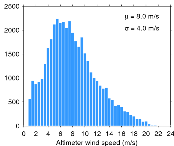
Figure 35. Histogram of science-valid wind over oceans and lakes for 18/06/2018. The mean ( \mu ) and standard deviation ( \sigma ) are also shown. Note that values larger than 24 m/s are excluded from the histogram for the sake of readability but not from the computation of \mu and \sigma .
