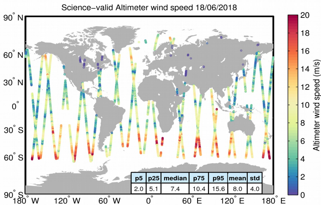
Figure 34. Geographical distribution of science-valid wind data over oceans and lakes for 18/06/2018. The statistical values shown in the table refer to the wind in m/s and are calculated over all measurements shown in the figure. Gray circles denote records that have been rejected based on the editing criteria described in Table 5.
