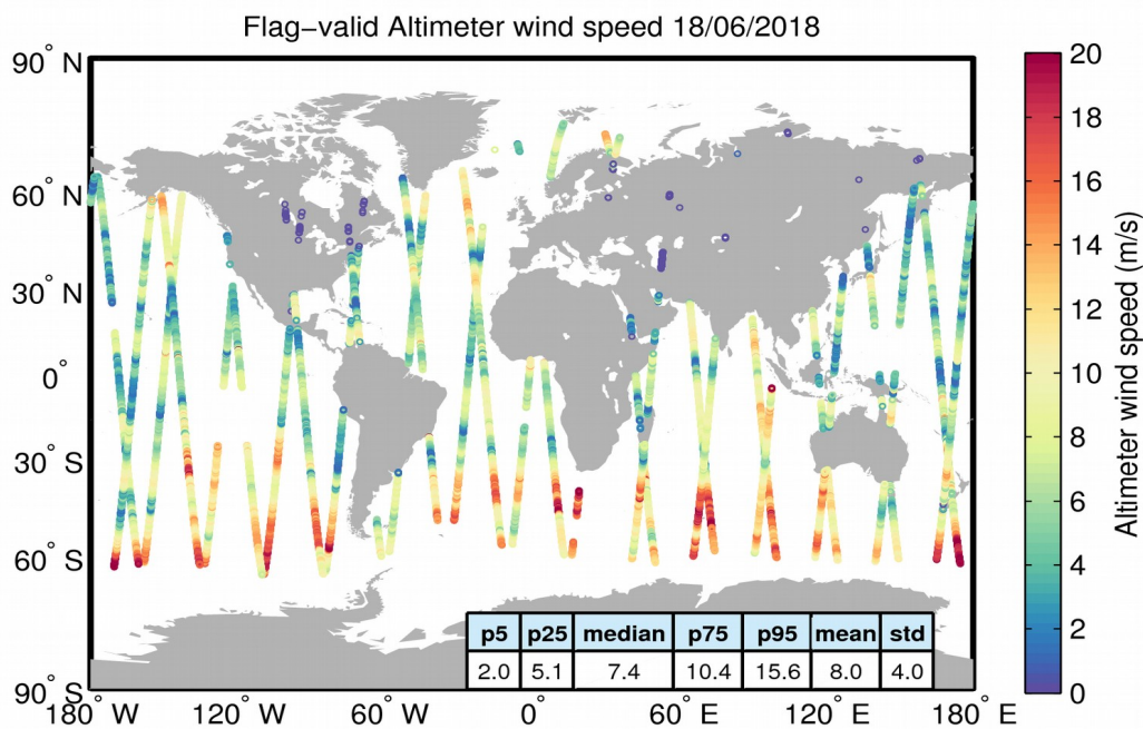
Figure 31. Geographical distribution of flag-valid wind data over oceans and lakes for 18/06/2018. The statistical values shown in the table refer to the wind in m/s and are calculated over all measurements shown in the figure.
