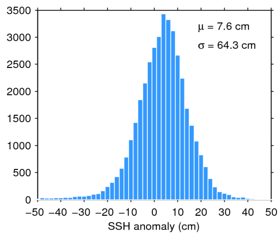
Figure 7. Histogram of flag-valid SSH anomaly over oceans and lakes for 18/06/2018. The mean ( \mu ) and standard deviation ( \sigma ) are also shown. Note that values outside [-50\ 50] cm are excluded from the histogram for the sake of readability but not from the computation of \mu and \sigma .
