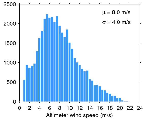
Figure 33. Histogram of flag-valid wind over oceans and lakes for 18/06/2018. The mean ( \mu ) and standard deviation ( \sigma ) are also shown. Note that values larger than 24 m/s are excluded from the histogram for the sake of readability but not from the computation of \mu and \sigma .
