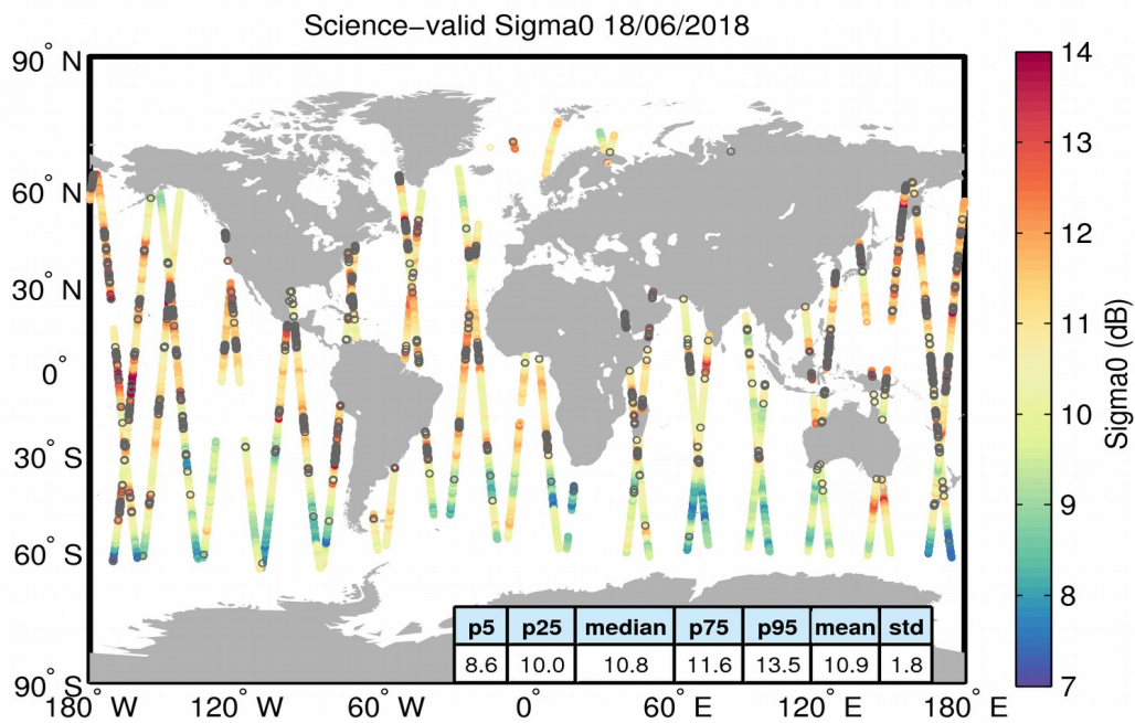
Figure 27. Geographical distribution of science-valid sigma0 data over oceans and lakes for 18/06/2018. The statistical values shown in the table refer to the sigma0 in dB and are calculated over all measurements shown in the figure. Gray circles denote records that have been rejected based on the editing criteria described in Table 4.
