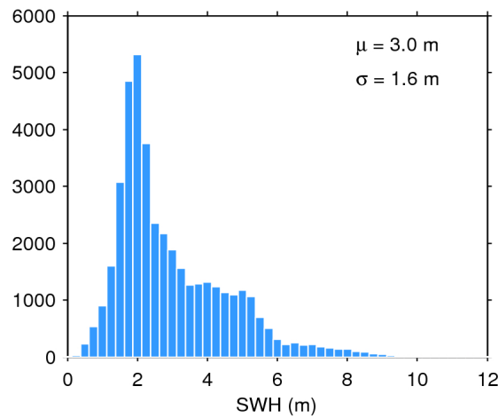
Figure 17. Histogram of flag-valid SWH over oceans and lakes for 18/06/2018. The mean ( \mu ) and standard deviation ( \sigma ) are also shown. Note that values larger than 12 m are excluded from the histogram for the sake of readability but not from the computation of \mu and \sigma .
