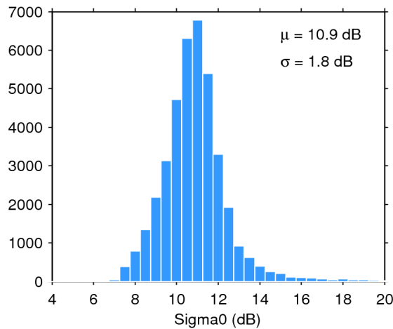
Figure 28. Histogram of science-valid sigma0 over oceans and lakes for 18/06/2018. The mean ( \mu ) and standard deviation ( \sigma ) are also shown. Note that values outside [4 20] dB are excluded from the histogram for the sake of readability but not from the computation of \mu and \sigma .
