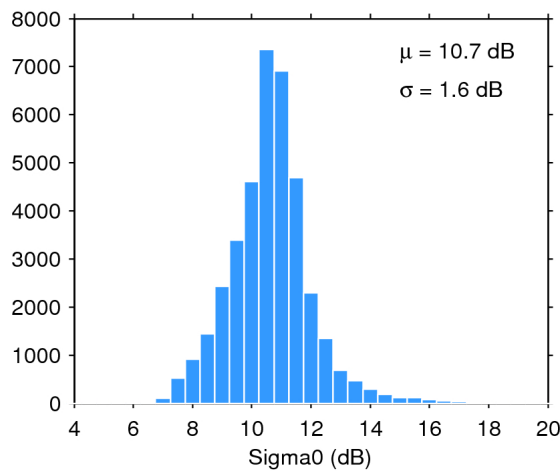
Figure 28. Histogram of science-valid sigma0 over oceans and lakes for 17/06/2018. The mean ( \mu ) and standard deviation ( \sigma ) are also shown. Note that values outside [4 20] dB are excluded from the histogram for the sake of readability but not from the computation of \mu and \sigma .
