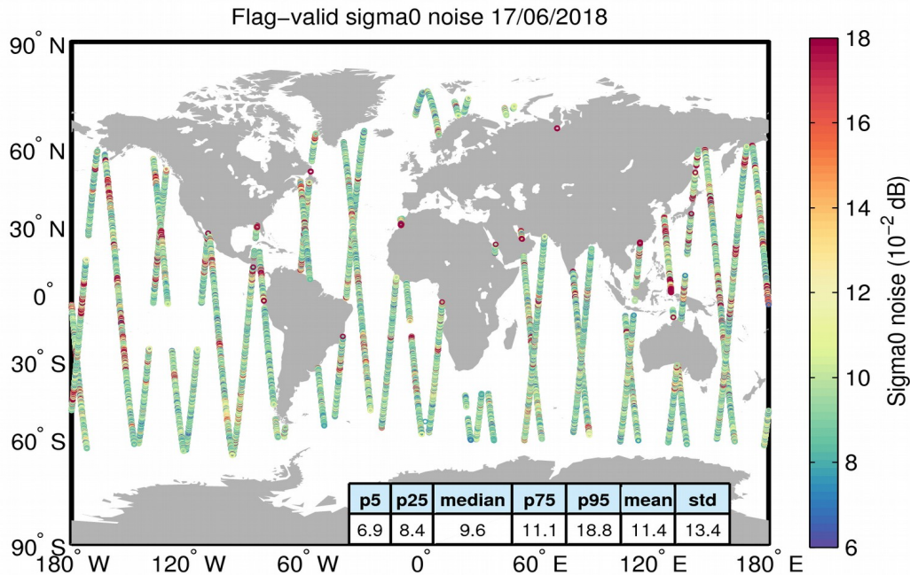
Figure 26. Geographical distribution of flag-valid 20-Hz sigma0 measurement noise over oceans and lakes for 17/06/2018. The statistical values shown in the table refer to the sigma0 noise and are calculated over all measurements shown in the figure.
