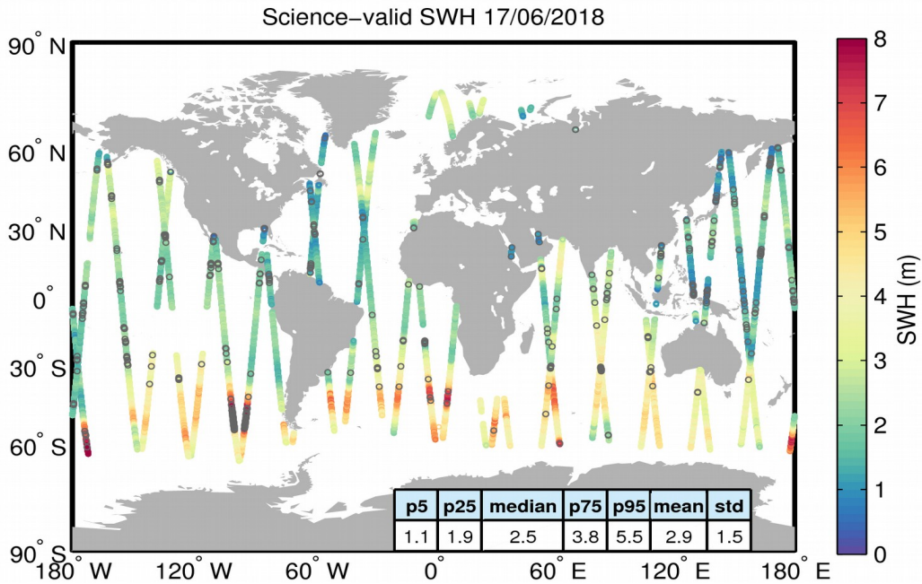
Figure 19. Geographical distribution of science-valid SWH data over oceans and lakes for 17/06/2018. The statistical values shown in the table refer to the SWH in m and are calculated over all measurements shown in the figure. Gray circles denote records that have been rejected based on the editing criteria described in Table 3.
