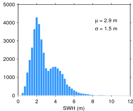
Figure 20. Histogram of science-valid SWH over oceans and lakes for 17/06/2018. The mean ( \mu ) and standard deviation ( \sigma ) are also shown. Note that values larger than 12 m are excluded from the histogram for the sake of readability but not from the computation of \mu and \sigma .
