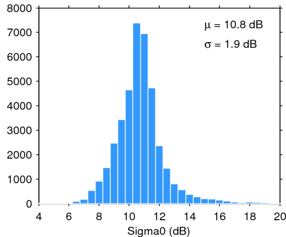
Figure 25. Histogram of flag-valid sigma0 over oceans and lakes for 17/06/2018. The mean ( \mu ) and standard deviation ( \sigma ) are also shown. Note that values outside [4 20] dB are excluded from the histogram for the sake of readability but not from the computation of \mu and \sigma .
