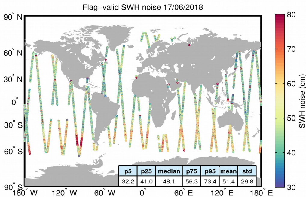
Figure 18. Geographical distribution of flag-valid 20-Hz SWH measurement noise over oceans and lakes for 17/06/2018. The statistical values shown in the figure refer to the SWH noise and are calculated over all measurements shown in the figure.
