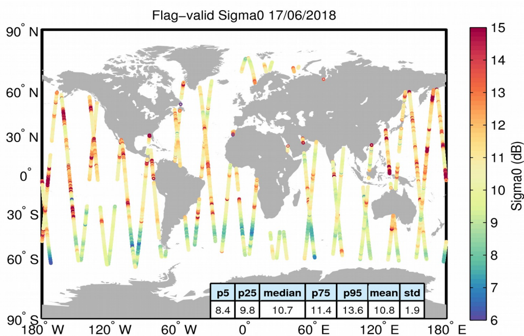
Figure 23. Geographical distribution of flag-valid sigma0 data over oceans and lakes for 17/06/2018. The statistical values shown in the table refer to the sigma0 in dB and are calculated over all measurements shown in the figure.
