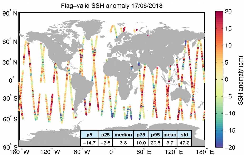
Figure 5. Geographical distribution of flag-valid 1-Hz SSH anomaly data over oceans and lakes for 17/06/2018. The statistical values shown in the table refer to the SSH anomaly in cm and are calculated over all measurements shown in the figure.
