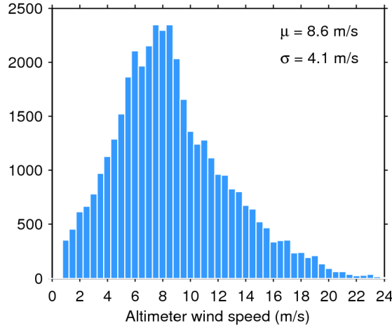
Figure 33. Histogram of flag-valid wind over oceans and lakes for 17/06/2018. The mean ( \mu ) and standard deviation ( \sigma ) are also shown. Note that values larger than 24 m/s are excluded from the histogram for the sake of readability but not from the computation of \mu and \sigma .
