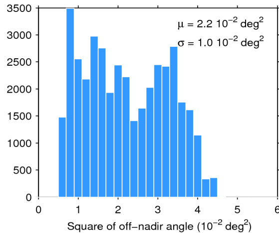
Figure 39. Histogram of flag-valid mispointing over oceans and lakes for 17/06/2018. The mean ( \mu ) and standard deviation ( \sigma ) are also shown. Note that values larger than 6 \cdot 10^{-2} \text{ deg}^2 are excluded from the histogram for the sake of readability but not from the computation of \mu and \sigma .
