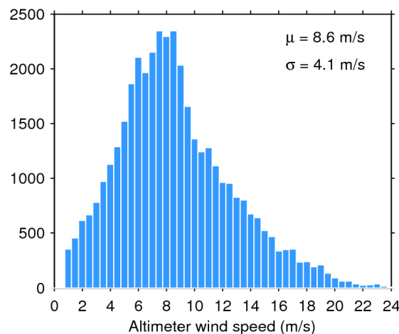
Figure 35. Histogram of science-valid wind over oceans and lakes for 17/06/2018. The mean ( \mu ) and standard deviation ( \sigma ) are also shown. Note that values larger than 24 m/s are excluded from the histogram for the sake of readability but not from the computation of \mu and \sigma .
