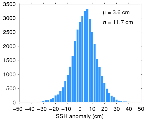
Figure 11. Histogram of science-valid SSH anomaly over oceans and lakes for 17/06/2018. The mean ( \mu ) and standard deviation ( \sigma ) are also shown. Note that values outside [-50 50] cm are excluded from the histogram for the sake of readability but not from the computation of \mu and \sigma .
