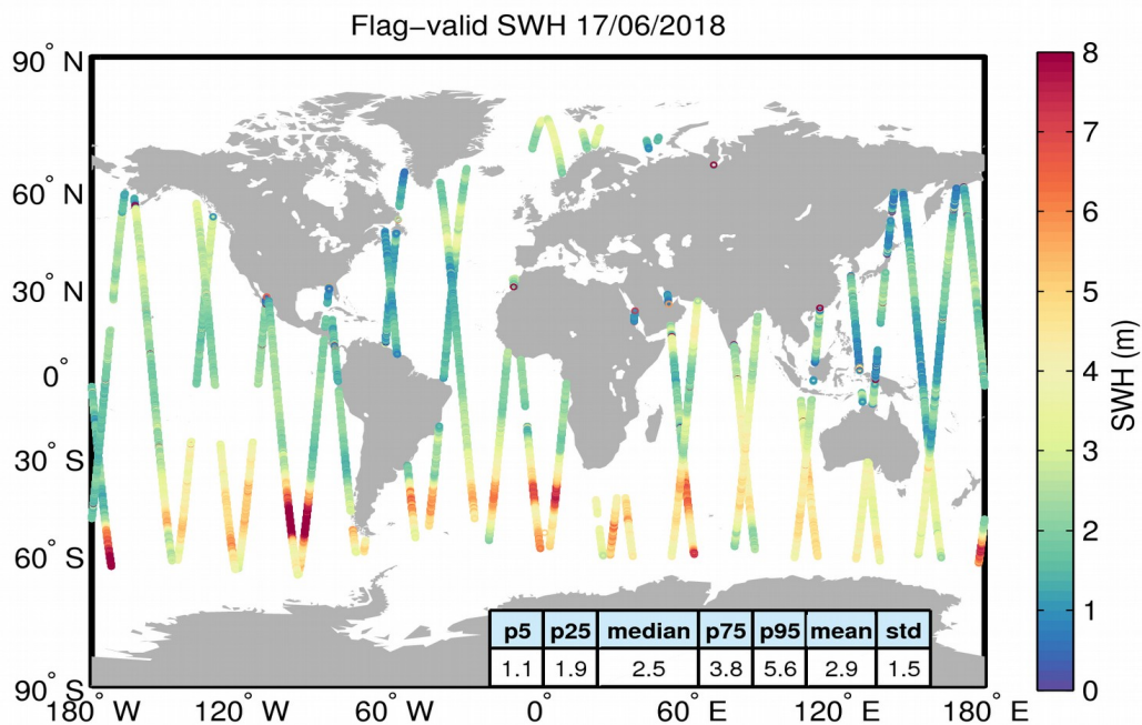
Figure 15. Geographical distribution of flag-valid SWH data over oceans and lakes for 17/06/2018. The statistical values shown in the table refer to the SWH in m and are calculated over all measurements shown in the figure.
