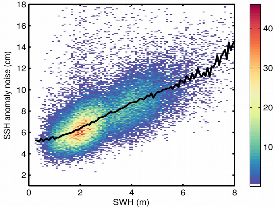
Figure 9. 2D histogram showing flag-valid SSH anomaly noise as a function of SWH for 17/06/2018. The black line denotes the median SSH anomaly noise as a function of SWH.
