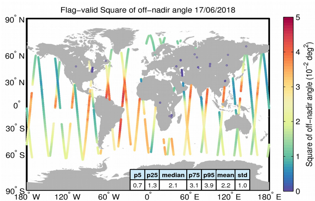
Figure 37. Geographical distribution of flag-valid mispointing data over oceans and lakes for 17/06/2018. The statistical values shown in the table refer to the mispointing in 10^{-2} \text{ deg}^2 and are calculated over all measurements shown in the figure.
