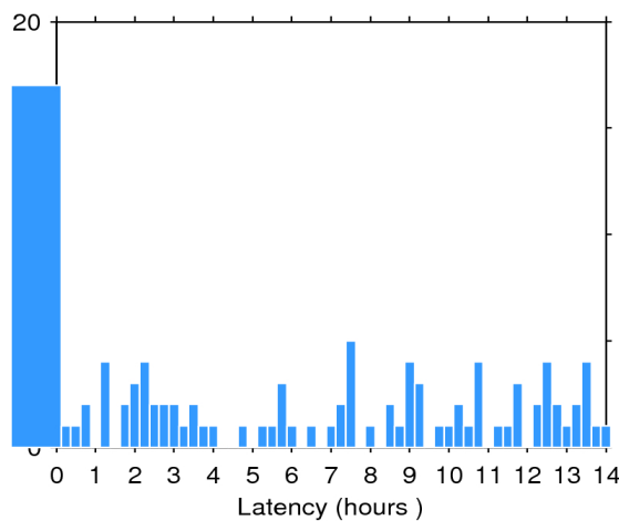
Figure 2. Histogram of the data latency for 17/06/2018. The y-axis denotes the number of files that are made available with a delay of x-hours with respect to the mean time of the records stored in the file.
