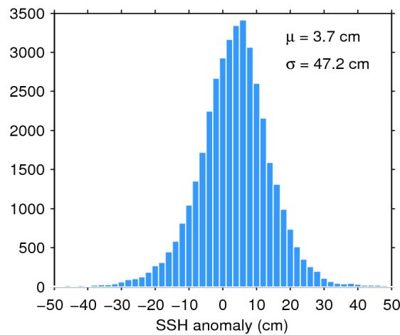
Figure 7. Histogram of flag-valid SSH anomaly over oceans and lakes for 17/06/2018. The mean ( \mu ) and standard deviation ( \sigma ) are also shown. Note that values outside [-50 50] cm are excluded from the histogram for the sake of readability but not from the computation of \mu and \sigma .
