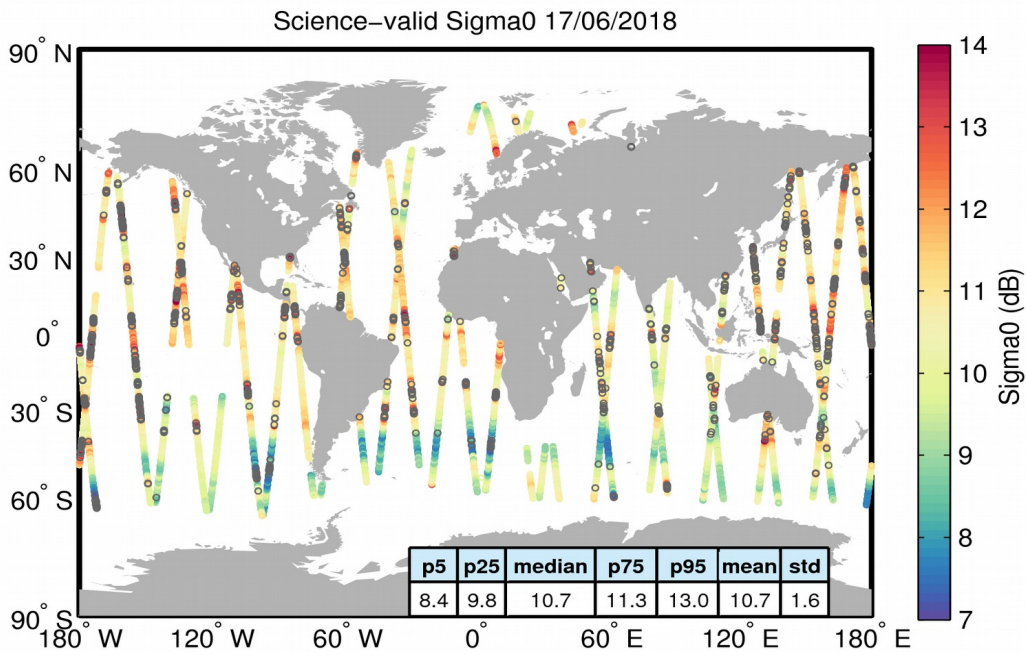
Figure 27. Geographical distribution of science-valid sigma0 data over oceans and lakes for 17/06/2018. The statistical values shown in the table refer to the sigma0 in dB and are calculated over all measurements shown in the figure. Gray circles denote records that have been rejected based on the editing criteria described in Table 4.
