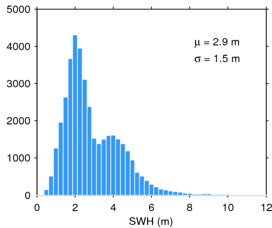
Figure 17. Histogram of flag-valid SWH over oceans and lakes for 17/06/2018. The mean ( \mu ) and standard deviation ( \sigma ) are also shown. Note that values larger than 12 m are excluded from the histogram for the sake of readability but not from the computation of \mu and \sigma .
