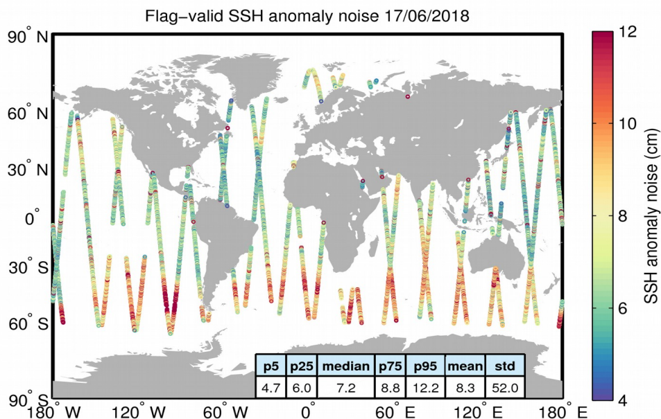
Figure 8. Geographical distribution of flag-valid 20-Hz SSH anomaly measurement noise over oceans and lakes for 17/06/2018. The statistical values shown in the table refer to the SSH anomaly noise and are calculated over all measurements shown in the figure.
