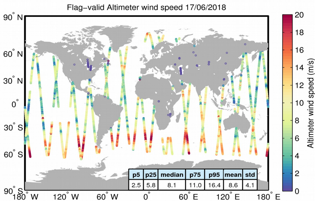
Figure 31. Geographical distribution of flag-valid wind data over oceans and lakes for 17/06/2018. The statistical values shown in the table refer to the wind in m/s and are calculated over all measurements shown in the figure.
