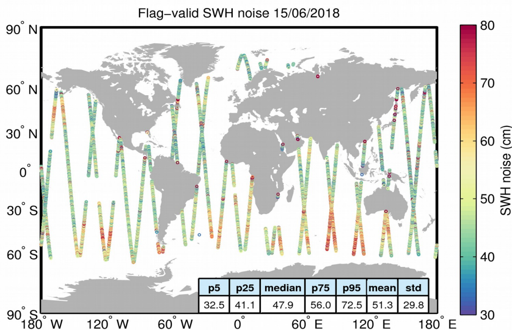
Figure 18. Geographical distribution of flag-valid 20-Hz SWH measurement noise over oceans and lakes for 15/06/2018. The statistical values shown in the table refer to the SWH noise and are calculated over all measurements shown in the figure.
