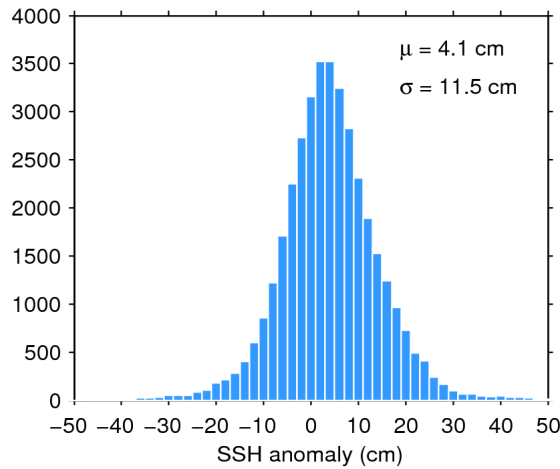
Figure 11. Histogram of science-valid SSH anomaly over oceans and lakes for 15/06/2018. The mean ( \mu ) and standard deviation ( \sigma ) are also shown. Note that values outside [-50 50] cm are excluded from the histogram for the sake of readability but not from the computation of \mu and \sigma .
