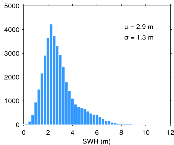
Figure 20. Histogram of science-valid SWH over oceans and lakes for 15/06/2018. The mean ( \mu ) and standard deviation ( \sigma ) are also shown. Note that values larger than 12 m are excluded from the histogram for the sake of readability but not from the computation of \mu and \sigma .
