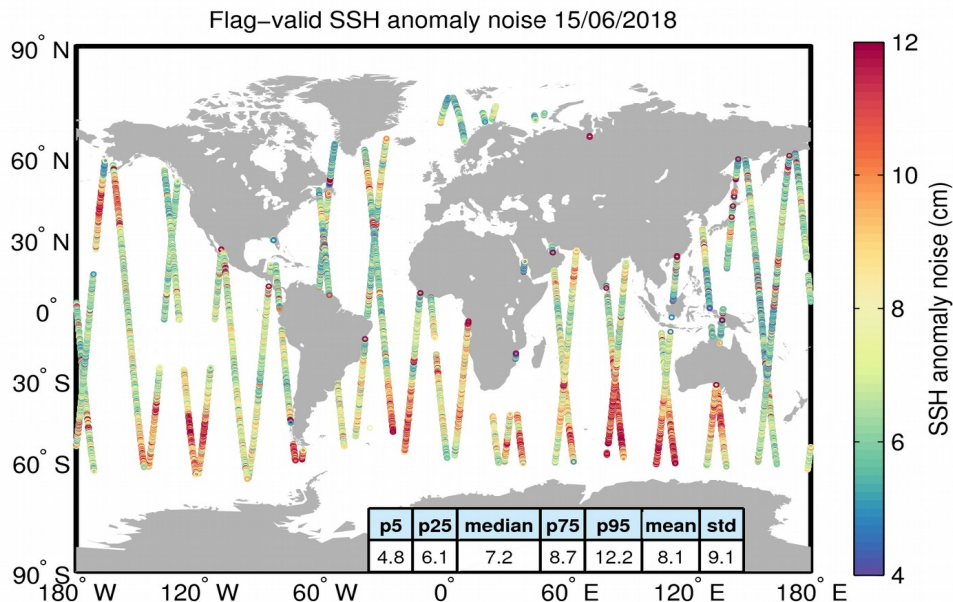
Figure 8. Geographical distribution of flag-valid 20-Hz SSH anomaly measurement noise over oceans and lakes for 15/06/2018. The statistical values shown in the table refer to the SSH anomaly noise and are calculated over all measurements shown in the figure.
