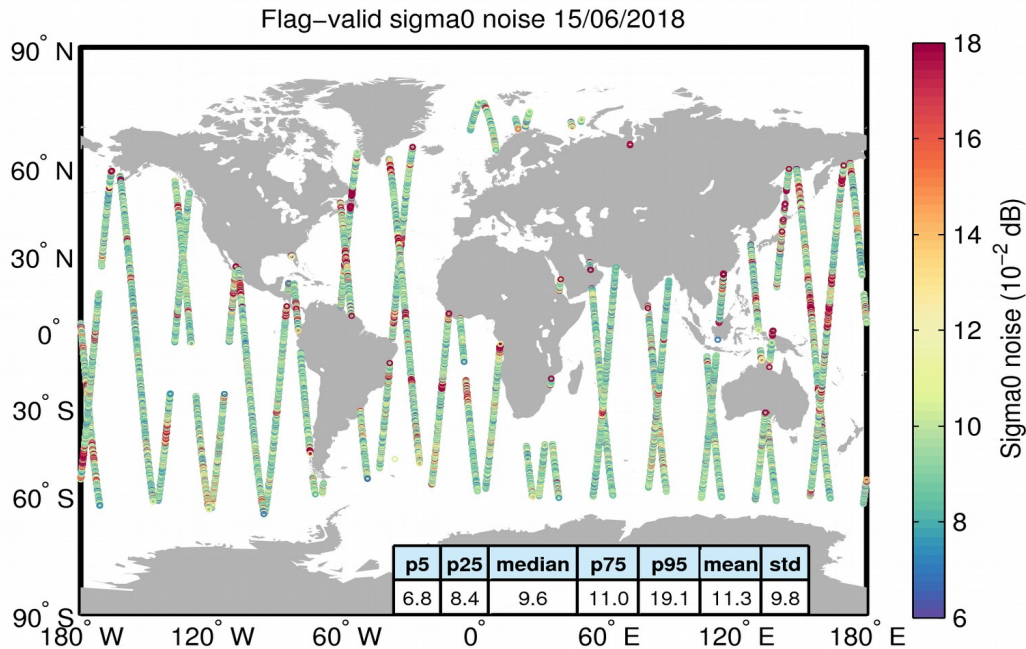
Figure 26. Geographical distribution of flag-valid 20-Hz sigma0 measurement noise over oceans and lakes for 15/06/2018. The statistical values shown in the table refer to the sigma0 noise and are calculated over all measurements shown in the figure.
