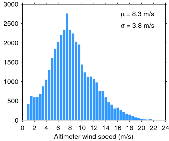
Figure 33. Histogram of flag-valid wind over oceans and lakes for 15/06/2018. The mean ( \mu ) and standard deviation ( \sigma ) are also shown. Note that values larger than 24 m/s are excluded from the histogram for the sake of readability but not from the computation of \mu and \sigma .
