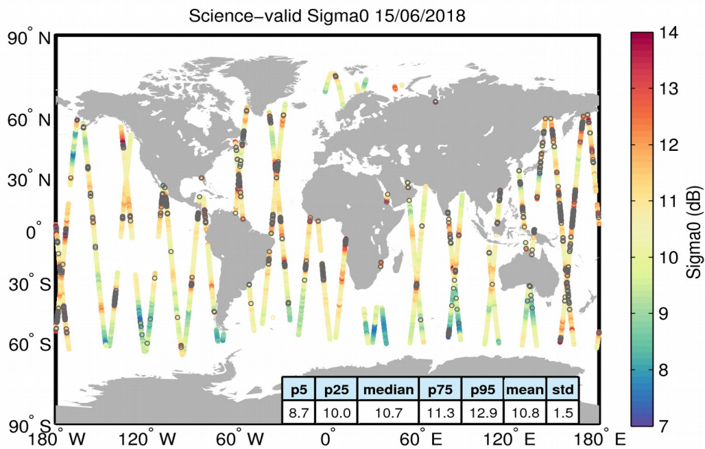
Figure 27. Geographical distribution of science-valid sigma0 data over oceans and lakes for 15/06/2018. The statistical values shown in the table refer to the sigma0 in dB and are calculated over all measurements shown in the figure. Gray circles denote records that have been rejected based on the editing criteria described in Table 4.
