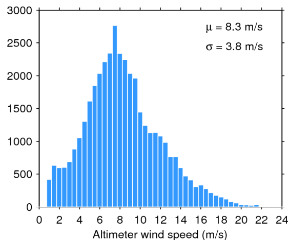
Figure 35. Histogram of science-valid wind over oceans and lakes for 15/06/2018. The mean ( \mu ) and standard deviation ( \sigma ) are also shown. Note that values larger than 24 m/s are excluded from the histogram for the sake of readability but not from the computation of \mu and \sigma .
