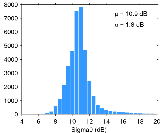
Figure 25. Histogram of flag-valid sigma0 over oceans and lakes for 15/06/2018. The mean ( \mu ) and standard deviation ( \sigma ) are also shown. Note that values outside [4 20] dB are excluded from the histogram for the sake of readability but not from the computation of \mu and \sigma .
