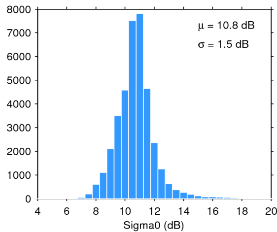
Figure 28. Histogram of science-valid sigma0 over oceans and lakes for 15/06/2018. The mean ( \mu ) and standard deviation ( \sigma ) are also shown. Note that values outside [4 20] dB are excluded from the histogram for the sake of readability but not from the computation of \mu and \sigma .
