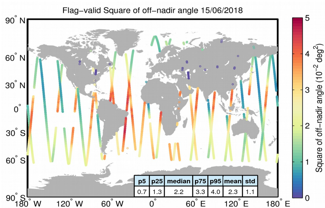
Figure 37. Geographical distribution of flag-valid mispointing data over oceans and lakes for 15/06/2018. The statistical values shown in the table refer to the mispointing in 10^{-2} deg 2 and are calculated over all measurements shown in the figure.
