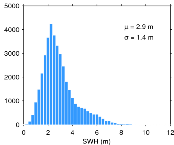
Figure 17. Histogram of flag-valid SWH over oceans and lakes for 15/06/2018. The mean ( \mu ) and standard deviation ( \sigma ) are also shown. Note that values larger than 12 m are excluded from the histogram for the sake of readability but not from the computation of \mu and \sigma .
