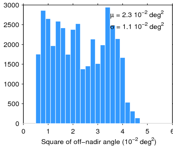
Figure 39. Histogram of flag-valid mispointing over oceans and lakes for 15/06/2018. The mean ( \mu ) and standard deviation ( \sigma ) are also shown. Note that values larger than 6 \cdot 10^{-2} \text{ deg}^2 are excluded from the histogram for the sake of readability but not from the computation of \mu and \sigma .
