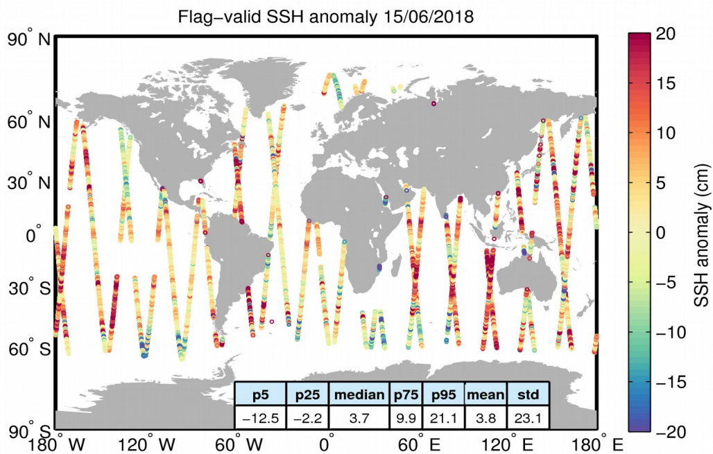
Figure 5. Geographical distribution of flag-valid 1-Hz SSH anomaly data over oceans and lakes for 15/06/2018. The statistical values shown in the table refer to the SSH anomaly in cm and are calculated over all measurements shown in the figure.
