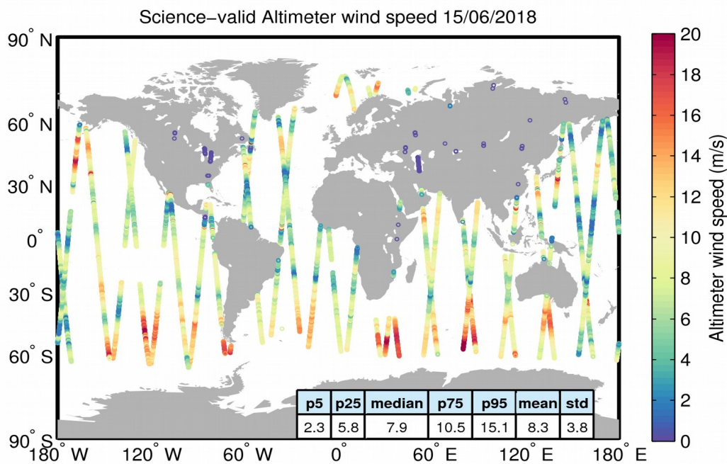
Figure 34. Geographical distribution of science-valid wind data over oceans and lakes for 15/06/2018. The statistical values shown in the table refer to the wind in m/s and are calculated over all measurements shown in the figure. Gray circles denote records that have been rejected based on the editing criteria described in Table 5.
