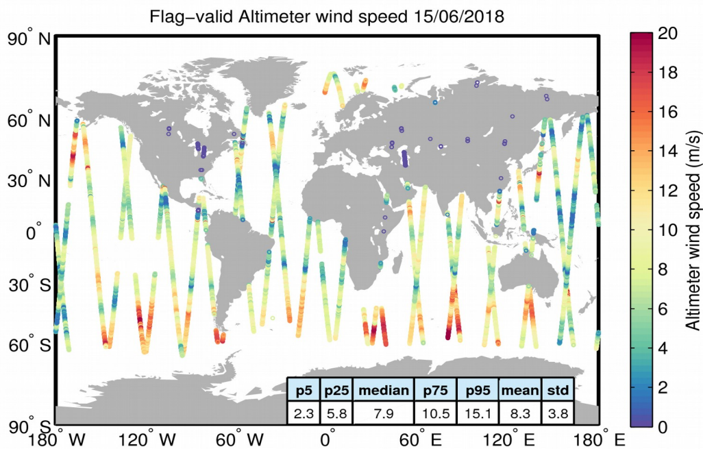
Figure 31. Geographical distribution of flag-valid wind data over oceans and lakes for 15/06/2018. The statistical values shown in the table refer to the wind in m/s and are calculated over all measurements shown in the figure.
