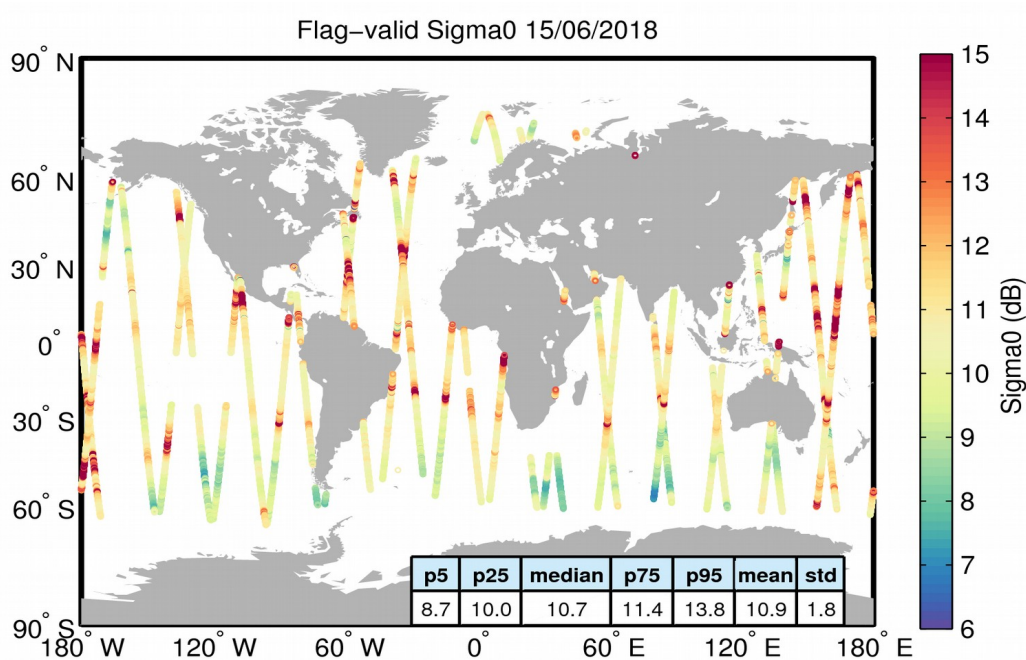
Figure 23. Geographical distribution of flag-valid sigma0 data over oceans and lakes for 15/06/2018. The statistical values shown in the table refer to the sigma0 in dB and are calculated over all measurements shown in the figure.
