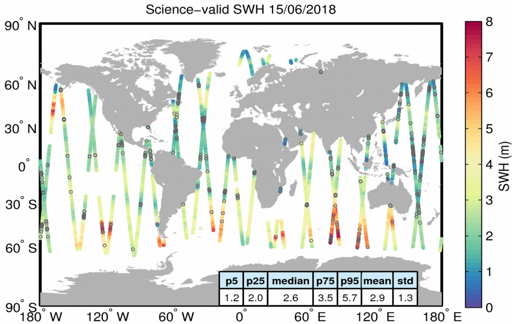
Figure 19. Geographical distribution of science-valid SWH data over oceans and lakes for 15/06/2018. The statistical values shown in the table refer to the SWH in m and are calculated over all measurements shown in the figure. Gray circles denote records that have been rejected based on the editing criteria described in Table 3.
