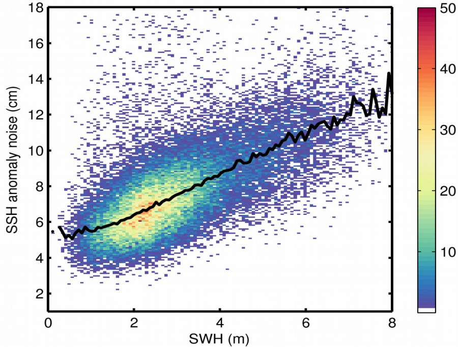
Figure 9. 2D histogram showing flag-valid SSH anomaly noise as a function of SWH for 15/06/2018. The black line denotes the median SSH anomaly noise as a function of SWH.
