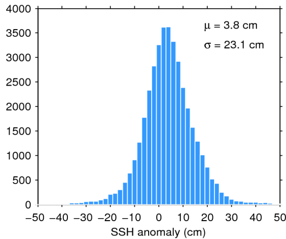
Figure 7. Histogram of flag-valid SSH anomaly over oceans and lakes for 15/06/2018. The mean ( \mu ) and standard deviation ( \sigma ) are also shown. Note that values outside [-50 50] cm are excluded from the histogram for the sake of readability but not from the computation of \mu and \sigma .
