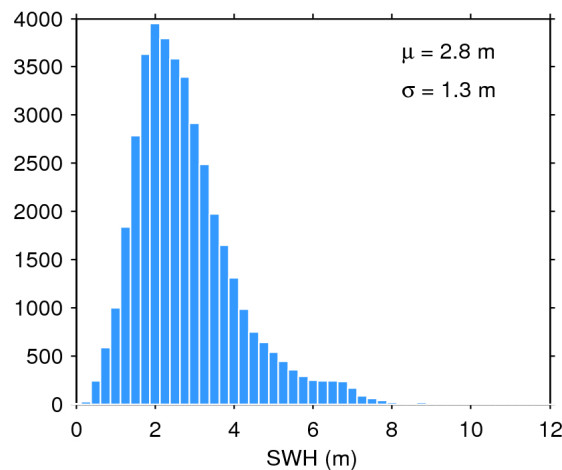
Figure 20. Histogram of science-valid SWH over oceans and lakes for 14/06/2018. The mean ( \mu ) and standard deviation ( \sigma ) are also shown. Note that values larger than 12 m are excluded from the histogram for the sake of readability but not from the computation of \mu and \sigma .
