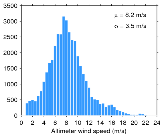
Figure 35. Histogram of science-valid wind over oceans and lakes for 14/06/2018. The mean ( \mu ) and standard deviation ( \sigma ) are also shown. Note that values larger than 24 m/s are excluded from the histogram for the sake of readability but not from the computation of \mu and \sigma .
