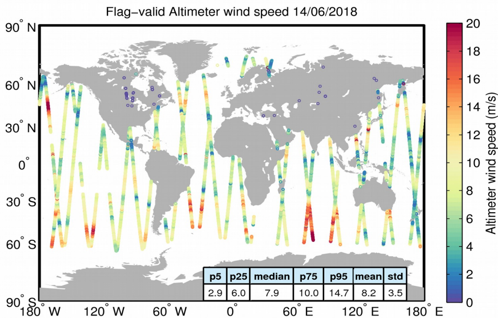
Figure 31. Geographical distribution of flag-valid wind data over oceans and lakes for 14/06/2018. The statistical values shown in the table refer to the wind in m/s and are calculated over all measurements shown in the figure.
