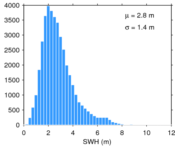
Figure 17. Histogram of flag-valid SWH over oceans and lakes for 14/06/2018. The mean ( \mu ) and standard deviation ( \sigma ) are also shown. Note that values larger than 12 m are excluded from the histogram for the sake of readability but not from the computation of \mu and \sigma .
