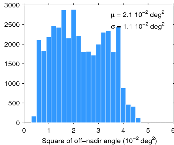
Figure 39. Histogram of flag-valid mispointing over oceans and lakes for 14/06/2018. The mean ( \mu ) and standard deviation ( \sigma ) are also shown. Note that values larger than 6 \cdot 10^{-2} \text{ deg}^2 are excluded from the histogram for the sake of readability but not from the computation of \mu and \sigma .
