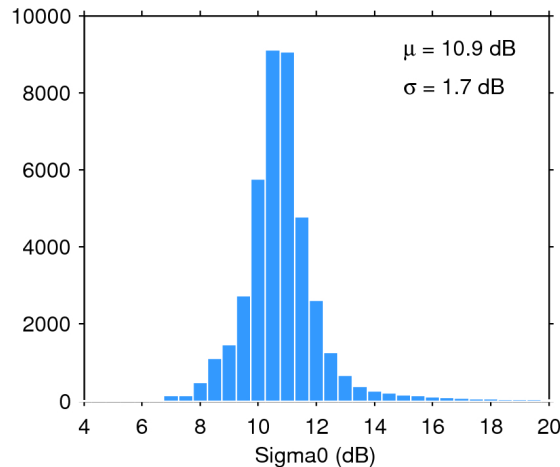
Figure 25. Histogram of flag-valid sigma0 over oceans and lakes for 14/06/2018. The mean ( \mu ) and standard deviation ( \sigma ) are also shown. Note that values outside [4 20] dB are excluded from the histogram for the sake of readability but not from the computation of \mu and \sigma .
