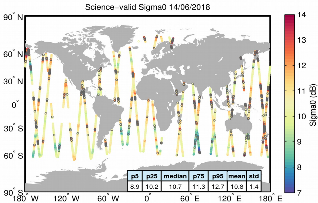
Figure 27. Geographical distribution of science-valid sigma0 data over oceans and lakes for 14/06/2018. The statistical values shown in the table refer to the sigma0 in dB and are calculated over all measurements shown in the figure. Gray circles denote records that have been rejected based on the editing criteria described in Table 4.
