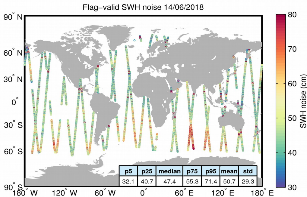
Figure 18. Geographical distribution of flag-valid 20-Hz SWH measurement noise over oceans and lakes for 14/06/2018. The statistical values shown in the figure refer to the SWH noise and are calculated over all measurements shown in the figure.
