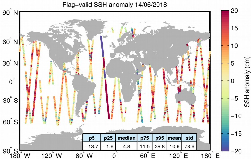
Figure 5. Geographical distribution of flag-valid 1-Hz SSH anomaly data over oceans and lakes for 14/06/2018. The statistical values shown in the table refer to the SSH anomaly in cm and are calculated over all measurements shown in the figure.
