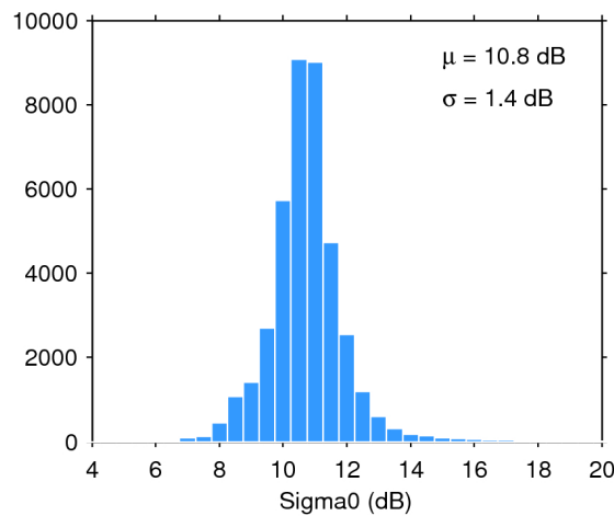
Figure 28. Histogram of science-valid sigma0 over oceans and lakes for 14/06/2018. The mean ( \mu ) and standard deviation ( \sigma ) are also shown. Note that values outside [4 20] dB are excluded from the histogram for the sake of readability but not from the computation of \mu and \sigma .
