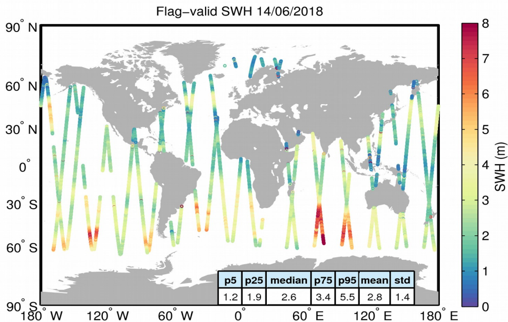
Figure 15. Geographical distribution of flag-valid SWH data over oceans and lakes for 14/06/2018. The statistical values shown in the table refer to the SWH in m and are calculated over all measurements shown in the figure.
