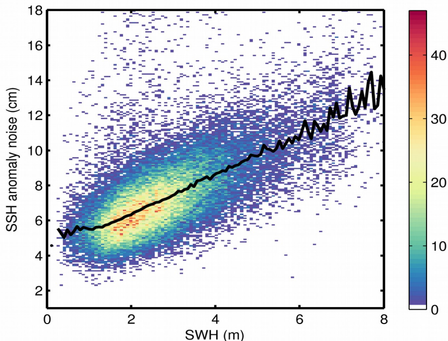
Figure 9. 2D histogram showing flag-valid SSH anomaly noise as a function of SWH for 14/06/2018. The black line denotes the median SSH anomaly noise as a function of SWH.
