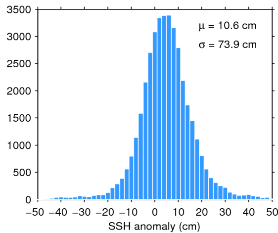
Figure 7. Histogram of flag-valid SSH anomaly over oceans and lakes for 14/06/2018. The mean ( \mu ) and standard deviation ( \sigma ) are also shown. Note that values outside [-50\ 50] cm are excluded from the histogram for the sake of readability but not from the computation of \mu and \sigma .
