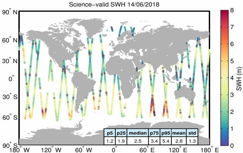
Figure 19. Geographical distribution of science-valid SWH data over oceans and lakes for 14/06/2018. The statistical values shown in the table refer to the SWH in m and are calculated over all measurements shown in the figure. Gray circles denote records that have been rejected based on the editing criteria described in Table 3.
