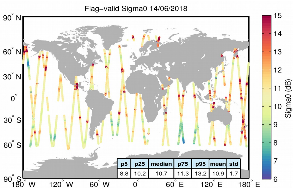
Figure 23. Geographical distribution of flag-valid sigma0 data over oceans and lakes for 14/06/2018. The statistical values shown in the table refer to the sigma0 in dB and are calculated over all measurements shown in the figure.
