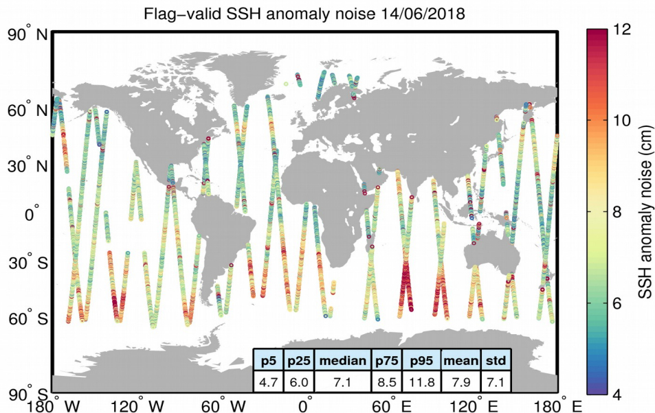
Figure 8. Geographical distribution of flag-valid 20-Hz SSH anomaly measurement noise over oceans and lakes for 14/06/2018. The statistical values shown in the table refer to the SSH anomaly noise and are calculated over all measurements shown in the figure.
