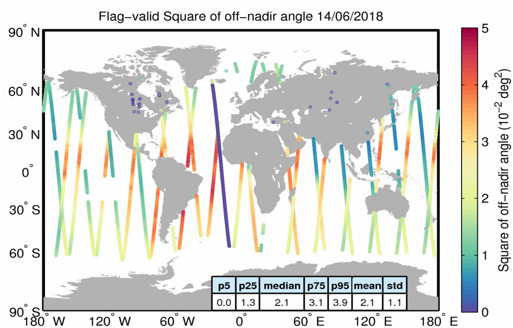
Figure 37. Geographical distribution of flag-valid mispointing data over oceans and lakes for 14/06/2018. The statistical values shown in the table refer to the mispointing in 10^{-2} deg 2 and are calculated over all measurements shown in the figure.
