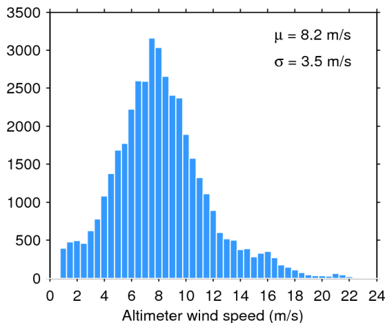
Figure 33. Histogram of flag-valid wind over oceans and lakes for 14/06/2018. The mean ( \mu ) and standard deviation ( \sigma ) are also shown. Note that values larger than 24 m/s are excluded from the histogram for the sake of readability but not from the computation of \mu and \sigma .
