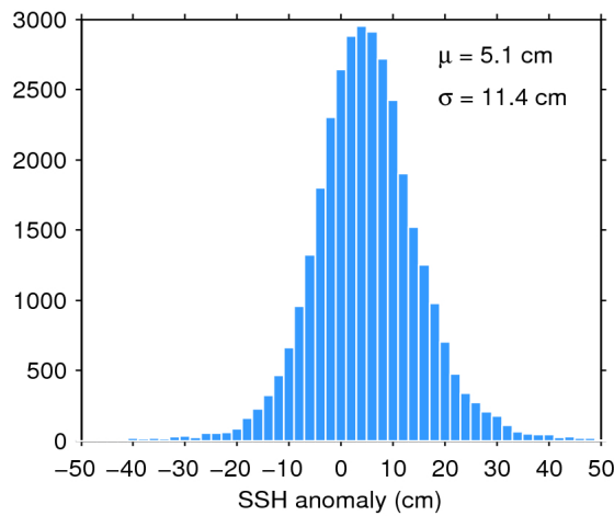
Figure 11. Histogram of science-valid SSH anomaly over oceans and lakes for 14/06/2018. The mean ( \mu ) and standard deviation ( \sigma ) are also shown. Note that values outside [-50 50] cm are excluded from the histogram for the sake of readability but not from the computation of \mu and \sigma .
