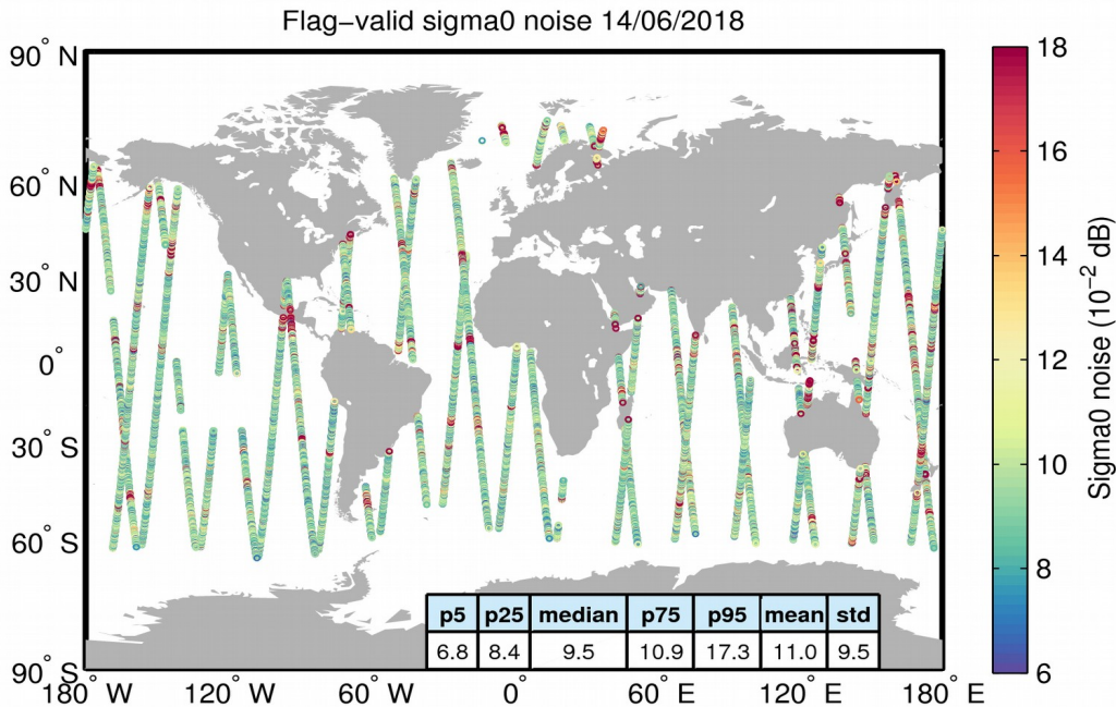
Figure 26. Geographical distribution of flag-valid 20-Hz sigma0 measurement noise over oceans and lakes for 14/06/2018. The statistical values shown in the table refer to the sigma0 noise and are calculated over all measurements shown in the figure.
