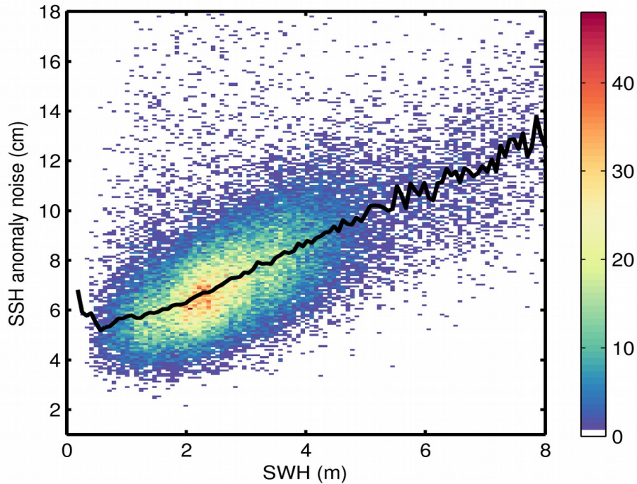
Figure 9. 2D histogram showing flag-valid SSH anomaly noise as a function of SWH for 13/06/2018. The black line denotes the median SSH anomaly noise as a function of SWH.
