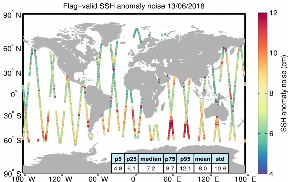
Figure 8. Geographical distribution of flag-valid 20-Hz SSH anomaly measurement noise over oceans and lakes for 13/06/2018. The statistical values shown in the table refer to the SSH anomaly noise and are calculated over all measurements shown in the figure.
