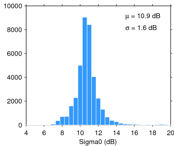
Figure 28. Histogram of science-valid sigma0 over oceans and lakes for 13/06/2018. The mean ( \mu ) and standard deviation ( \sigma ) are also shown. Note that values outside [4 20] dB are excluded from the histogram for the sake of readability but not from the computation of \mu and \sigma .
