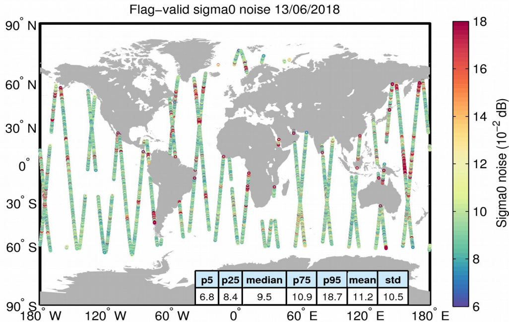
Figure 26. Geographical distribution of flag-valid 20-Hz sigma0 measurement noise over oceans and lakes for 13/06/2018. The statistical values shown in the table refer to the sigma0 noise and are calculated over all measurements shown in the figure.
