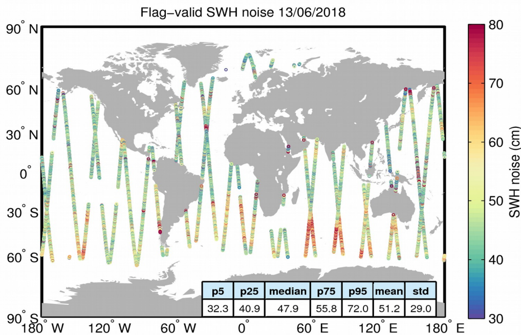
Figure 18. Geographical distribution of flag-valid 20-Hz SWH measurement noise over oceans and lakes for 13/06/2018. The statistical values shown in the table refer to the SWH noise and are calculated over all measurements shown in the figure.
