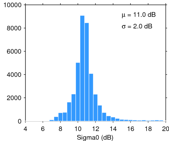
Figure 25. Histogram of flag-valid sigma0 over oceans and lakes for 13/06/2018. The mean ( \mu ) and standard deviation ( \sigma ) are also shown. Note that values outside [4 20] dB are excluded from the histogram for the sake of readability but not from the computation of \mu and \sigma .
