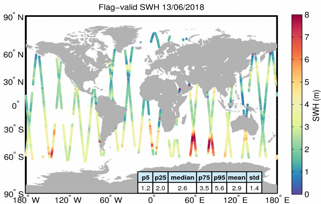
Figure 15. Geographical distribution of flag-valid SWH data over oceans and lakes for 13/06/2018. The statistical values shown in the table refer to the SWH in m and are calculated over all measurements shown in the figure.
