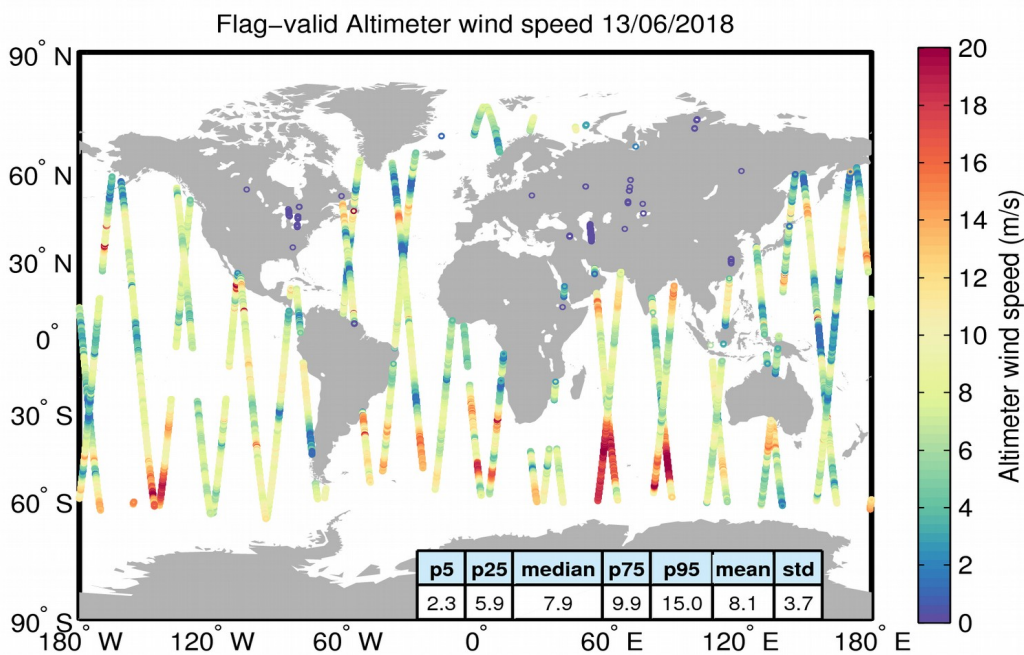
Figure 31. Geographical distribution of flag-valid wind data over oceans and lakes for 13/06/2018. The statistical values shown in the table refer to the wind in m/s and are calculated over all measurements shown in the figure.
