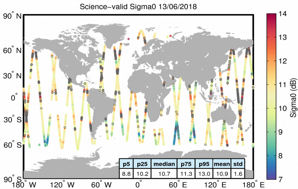
Figure 27. Geographical distribution of science-valid sigma0 data over oceans and lakes for 13/06/2018. The statistical values shown in the table refer to the sigma0 in dB and are calculated over all measurements shown in the figure. Gray circles denote records that have been rejected based on the editing criteria described in Table 4.
