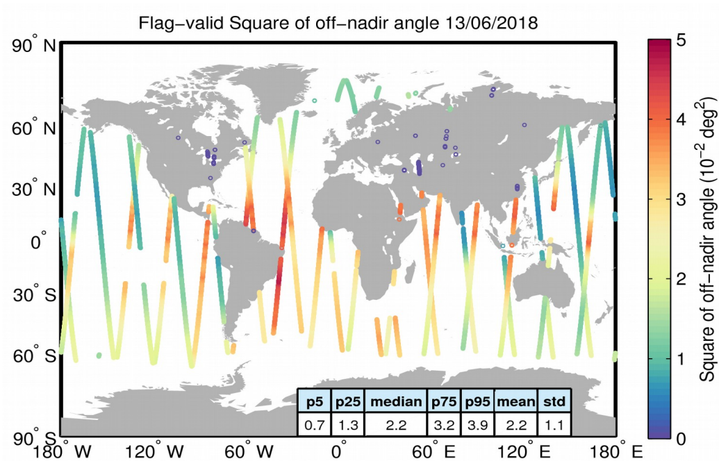
Figure 37. Geographical distribution of flag-valid mispointing data over oceans and lakes for 13/06/2018. The statistical values shown in the table refer to the mispointing in 10^{-2} \text{ deg}^2 and are calculated over all measurements shown in the figure.
