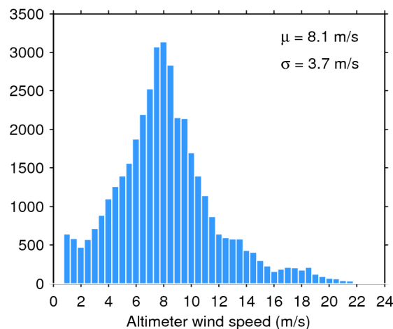
Figure 35. Histogram of science-valid wind over oceans and lakes for 13/06/2018. The mean ( \mu ) and standard deviation ( \sigma ) are also shown. Note that values larger than 24 m/s are excluded from the histogram for the sake of readability but not from the computation of \mu and \sigma .
