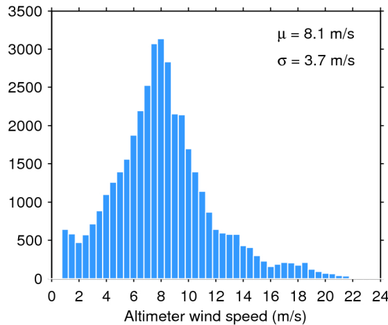
Figure 33. Histogram of flag-valid wind over oceans and lakes for 13/06/2018. The mean ( \mu ) and standard deviation ( \sigma ) are also shown. Note that values larger than 24 m/s are excluded from the histogram for the sake of readability but not from the computation of \mu and \sigma .
