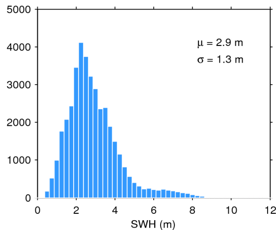
Figure 20. Histogram of science-valid SWH over oceans and lakes for 13/06/2018. The mean ( \mu ) and standard deviation ( \sigma ) are also shown. Note that values larger than 12 m are excluded from the histogram for the sake of readability but not from the computation of \mu and \sigma .
