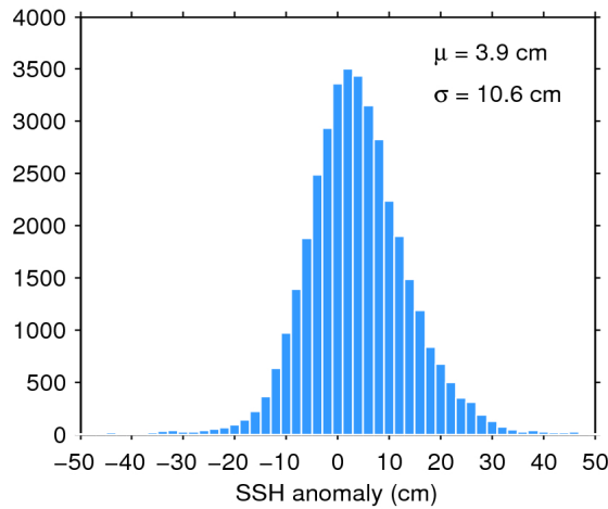
Figure 11. Histogram of science-valid SSH anomaly over oceans and lakes for 13/06/2018. The mean ( \mu ) and standard deviation ( \sigma ) are also shown. Note that values outside [-50 50] cm are excluded from the histogram for the sake of readability but not from the computation of \mu and \sigma .
