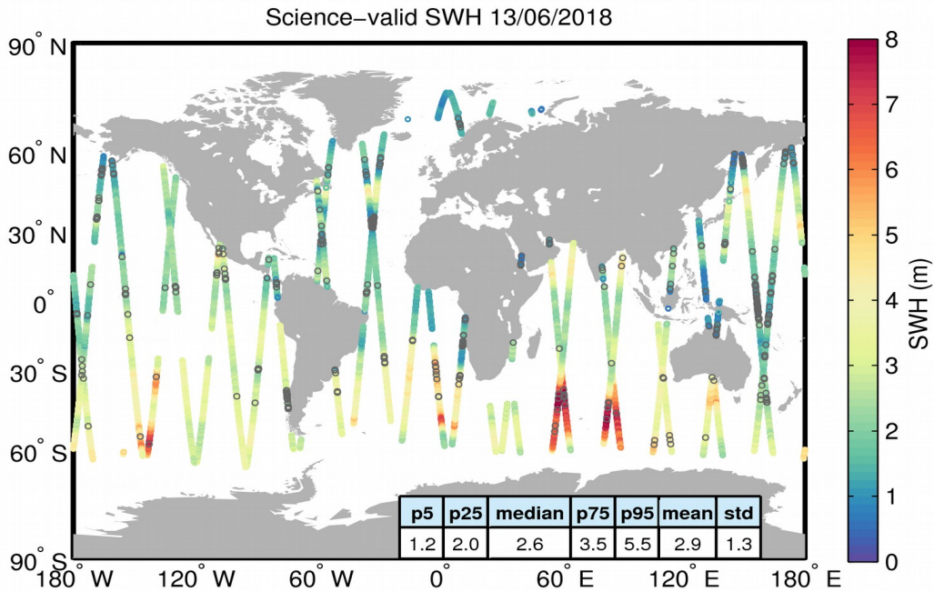
Figure 19. Geographical distribution of science-valid SWH data over oceans and lakes for 13/06/2018. The statistical values shown in the table refer to the SWH in m and are calculated over all measurements shown in the figure. Gray circles denote records that have been rejected based on the editing criteria described in Table 3.
