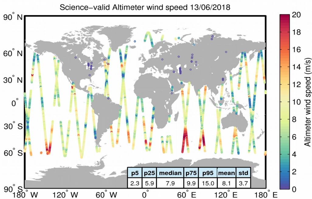
Figure 34. Geographical distribution of science-valid wind data over oceans and lakes for 13/06/2018. The statistical values shown in the table refer to the wind in m/s and are calculated over all measurements shown in the figure. Gray circles denote records that have been rejected based on the editing criteria described in Table 5.
