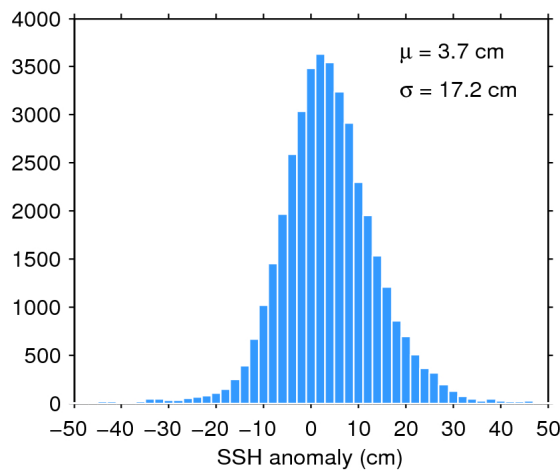
Figure 7. Histogram of flag-valid SSH anomaly over oceans and lakes for 13/06/2018. The mean ( \mu ) and standard deviation ( \sigma ) are also shown. Note that values outside [-50\ 50] cm are excluded from the histogram for the sake of readability but not from the computation of \mu and \sigma .
