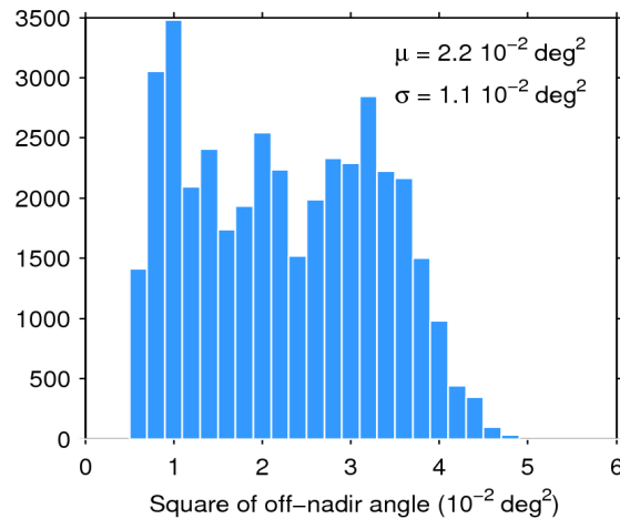
Figure 39. Histogram of flag-valid mispointing over oceans and lakes for 13/06/2018. The mean ( \mu ) and standard deviation ( \sigma ) are also shown. Note that values larger than 6 \cdot 10^{-2} \text{ deg}^2 are excluded from the histogram for the sake of readability but not from the computation of \mu and \sigma .
