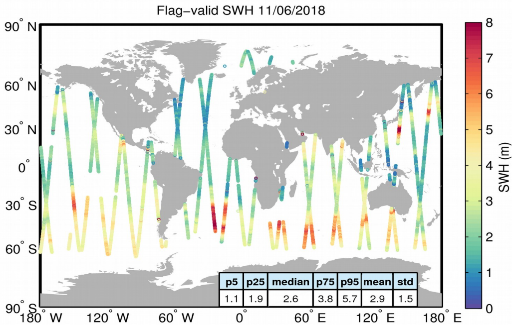
Figure 15. Geographical distribution of flag-valid SWH data over oceans and lakes for 11/06/2018. The statistical values shown in the table refer to the SWH in m and are calculated over all measurements shown in the figure.
