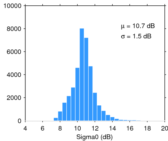
Figure 28. Histogram of science-valid sigma0 over oceans and lakes for 11/06/2018. The mean ( \mu ) and standard deviation ( \sigma ) are also shown. Note that values outside [4 20] dB are excluded from the histogram for the sake of readability but not from the computation of \mu and \sigma .
