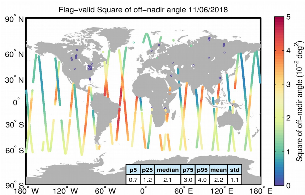
Figure 37. Geographical distribution of flag-valid mispointing data over oceans and lakes for 11/06/2018. The statistical values shown in the table refer to the mispointing in 10^{-2} deg 2 and are calculated over all measurements shown in the figure.
