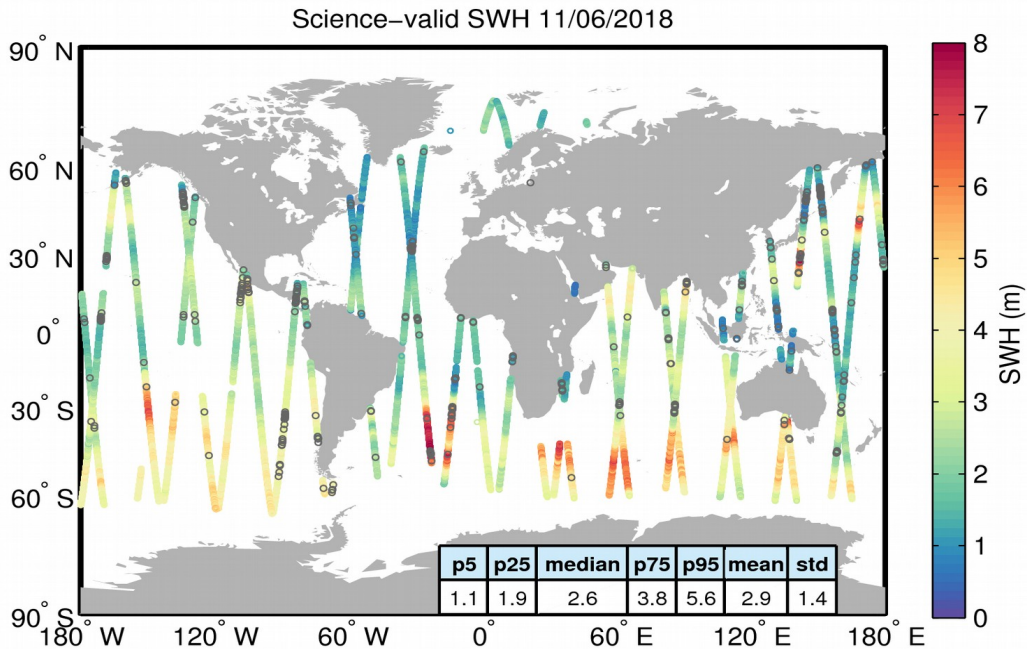
Figure 19. Geographical distribution of science-valid SWH data over oceans and lakes for 11/06/2018. The statistical values shown in the table refer to the SWH in m and are calculated over all measurements shown in the figure. Gray circles denote records that have been rejected based on the editing criteria described in Table 3.
