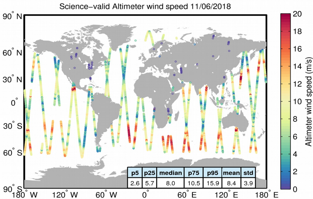
Figure 34. Geographical distribution of science-valid wind data over oceans and lakes for 11/06/2018. The statistical values shown in the table refer to the wind in m/s and are calculated over all measurements shown in the figure. Gray circles denote records that have been rejected based on the editing criteria described in Table 5.
