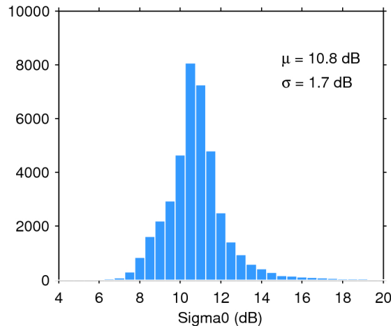
Figure 25. Histogram of flag-valid sigma0 over oceans and lakes for 11/06/2018. The mean ( \mu ) and standard deviation ( \sigma ) are also shown. Note that values outside [4 20] dB are excluded from the histogram for the sake of readability but not from the computation of \mu and \sigma .
