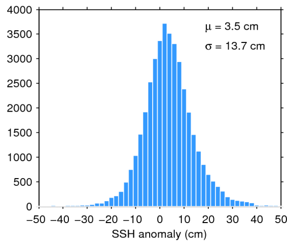
Figure 7. Histogram of flag-valid SSH anomaly over oceans and lakes for 11/06/2018. The mean ( \mu ) and standard deviation ( \sigma ) are also shown. Note that values outside [-50\ 50] cm are excluded from the histogram for the sake of readability but not from the computation of \mu and \sigma .
