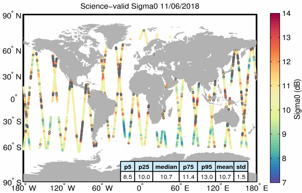
Figure 27. Geographical distribution of science-valid sigma0 data over oceans and lakes for 11/06/2018. The statistical values shown in the table refer to the sigma0 in dB and are calculated over all measurements shown in the figure. Gray circles denote records that have been rejected based on the editing criteria described in Table 4.
