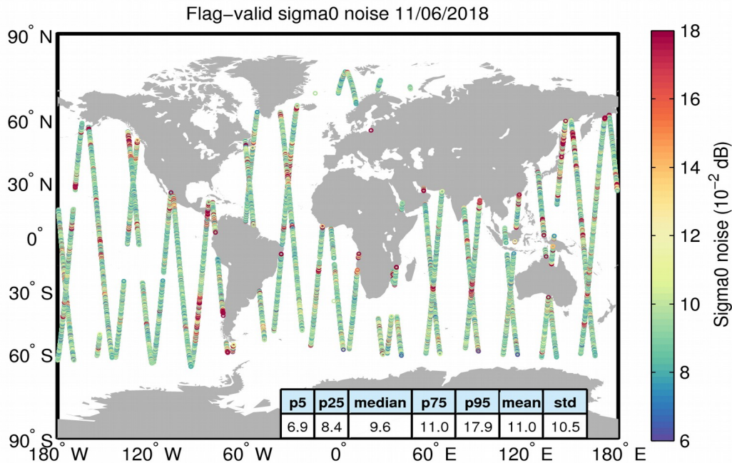
Figure 26. Geographical distribution of flag-valid 20-Hz sigma0 measurement noise over oceans and lakes for 11/06/2018. The statistical values shown in the table refer to the sigma0 noise and are calculated over all measurements shown in the figure.
