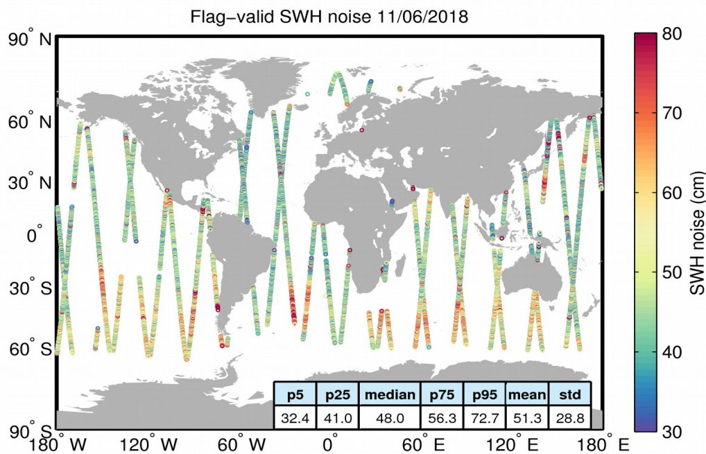
Figure 18. Geographical distribution of flag-valid 20-Hz SWH measurement noise over oceans and lakes for 11/06/2018. The statistical values shown in the figure refer to the SWH noise and are calculated over all measurements shown in the figure.
