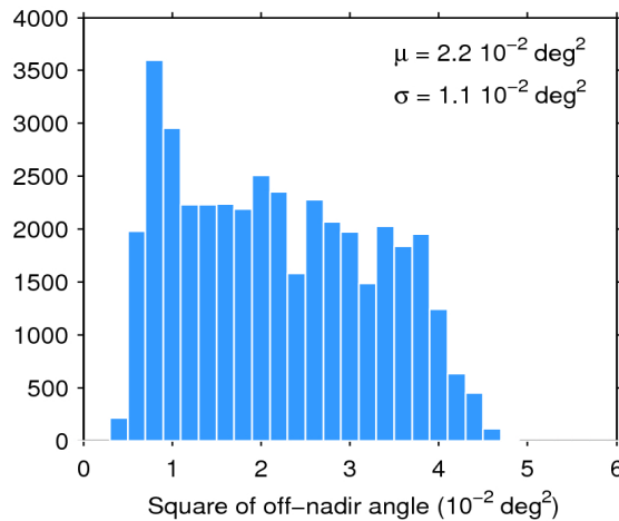
Figure 39. Histogram of flag-valid mispointing over oceans and lakes for 11/06/2018. The mean ( \mu ) and standard deviation ( \sigma ) are also shown. Note that values larger than 6 \cdot 10^{-2} \text{ deg}^2 are excluded from the histogram for the sake of readability but not from the computation of \mu and \sigma .
