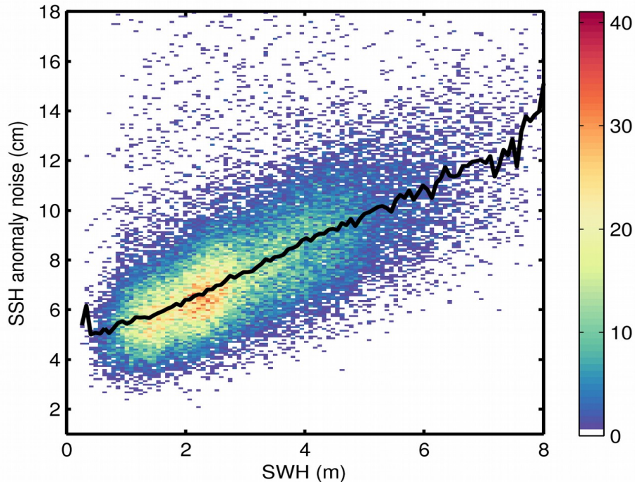
Figure 9. 2D histogram showing flag-valid SSH anomaly noise as a function of SWH for 11/06/2018. The black line denotes the median SSH anomaly noise as a function of SWH.
