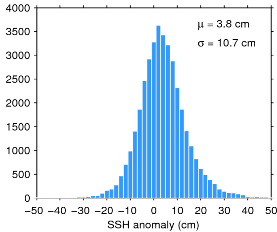
Figure 11. Histogram of science-valid SSH anomaly over oceans and lakes for 11/06/2018. The mean ( \mu ) and standard deviation ( \sigma ) are also shown. Note that values outside [-50 50] cm are excluded from the histogram for the sake of readability but not from the computation of \mu and \sigma .
