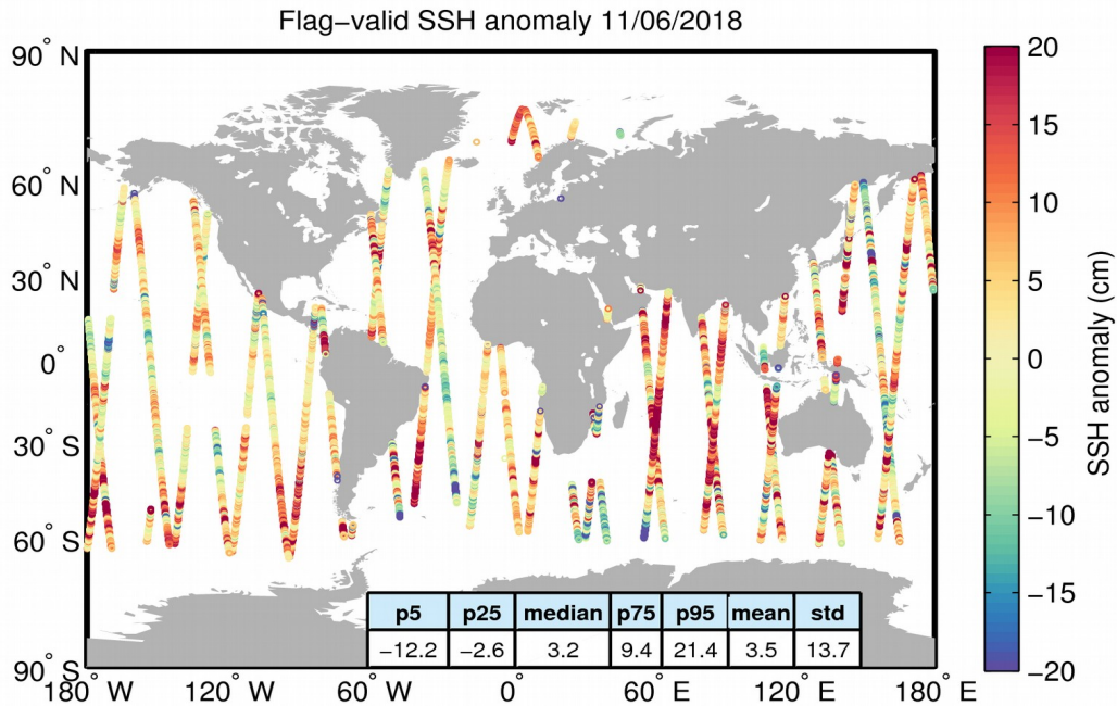
Figure 5. Geographical distribution of flag-valid 1-Hz SSH anomaly data over oceans and lakes for 11/06/2018. The statistical values shown in the table refer to the SSH anomaly in cm and are calculated over all measurements shown in the figure.
