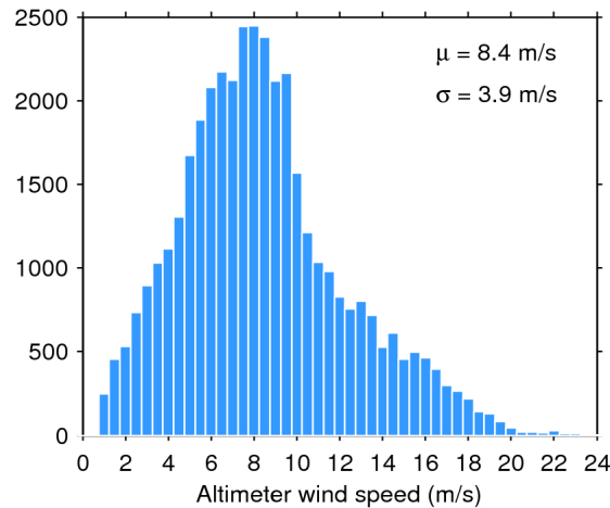
Figure 33. Histogram of flag-valid wind over oceans and lakes for 11/06/2018. The mean ( \mu ) and standard deviation ( \sigma ) are also shown. Note that values larger than 24 m/s are excluded from the histogram for the sake of readability but not from the computation of \mu and \sigma .
