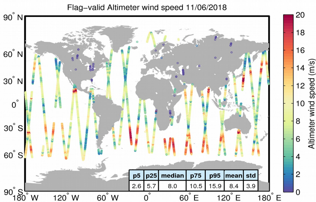
Figure 31. Geographical distribution of flag-valid wind data over oceans and lakes for 11/06/2018. The statistical values shown in the table refer to the wind in m/s and are calculated over all measurements shown in the figure.
