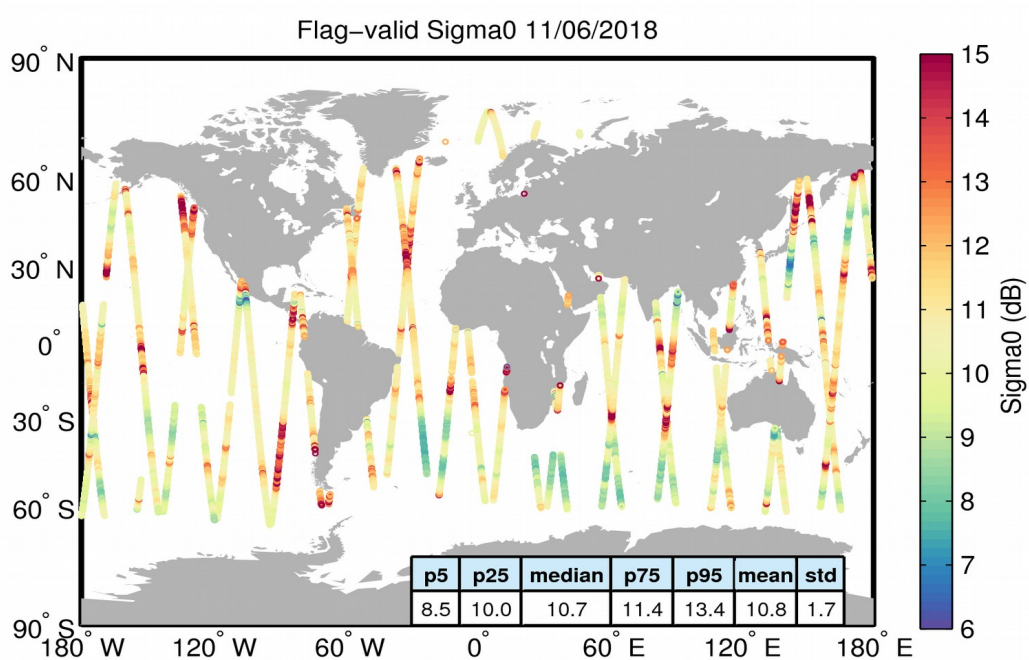
Figure 23. Geographical distribution of flag-valid sigma0 data over oceans and lakes for 11/06/2018. The statistical values shown in the table refer to the sigma0 in dB and are calculated over all measurements shown in the figure.
