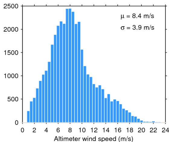
Figure 35. Histogram of science-valid wind over oceans and lakes for 11/06/2018. The mean ( \mu ) and standard deviation ( \sigma ) are also shown. Note that values larger than 24 m/s are excluded from the histogram for the sake of readability but not from the computation of \mu and \sigma .
