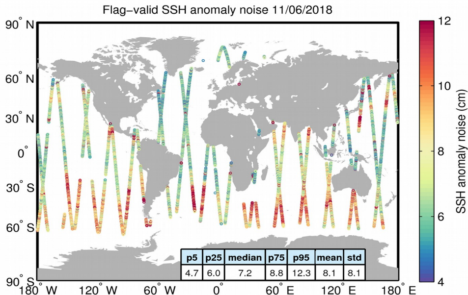
Figure 8. Geographical distribution of flag-valid 20-Hz SSH anomaly measurement noise over oceans and lakes for 11/06/2018. The statistical values shown in the table refer to the SSH anomaly noise and are calculated over all measurements shown in the figure.
