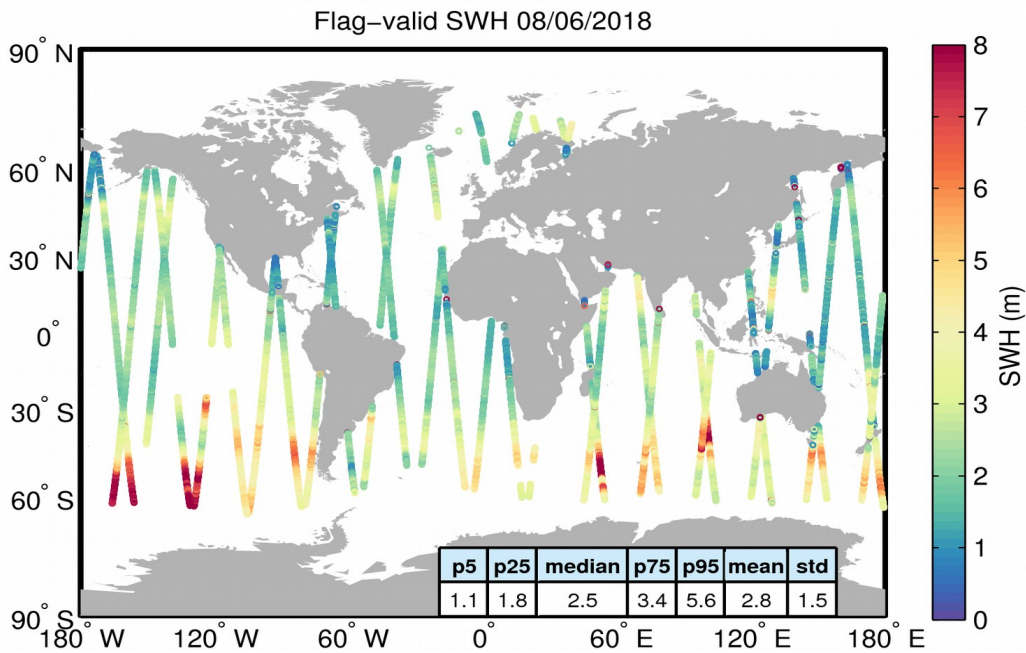
Figure 15. Geographical distribution of flag-valid SWH data over oceans and lakes for 08/06/2018. The statistical values shown in the table refer to the SWH in m and are calculated over all measurements shown in the figure.
