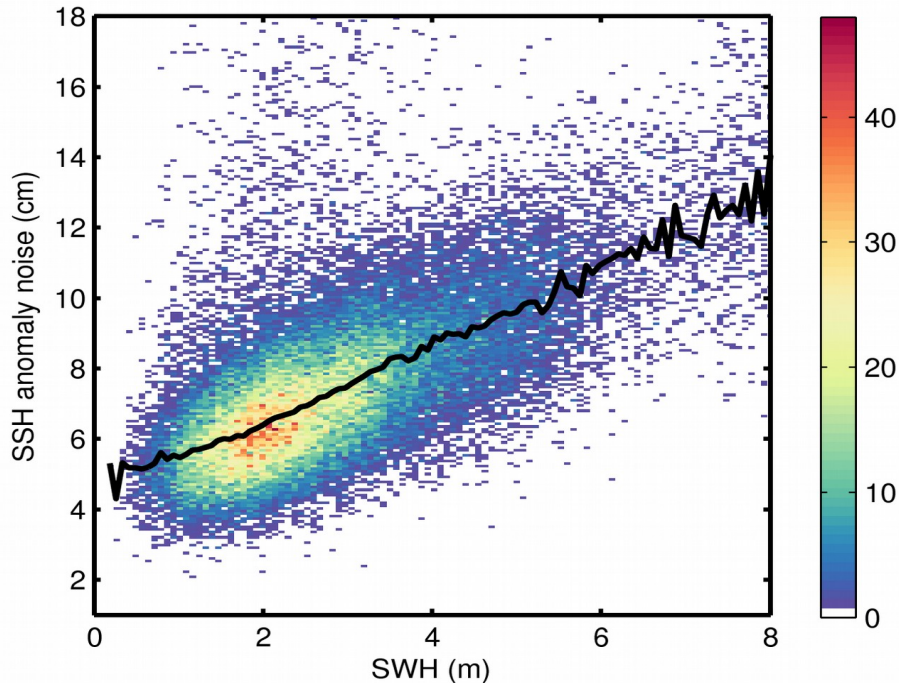
Figure 9. 2D histogram showing flag-valid SSH anomaly noise as a function of SWH for 08/06/2018. The black line denotes the median SSH anomaly noise as a function of SWH.
