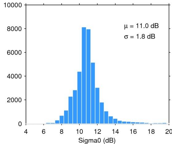
Figure 25. Histogram of flag-valid sigma0 over oceans and lakes for 08/06/2018. The mean ( \mu ) and standard deviation ( \sigma ) are also shown. Note that values outside [4 20] dB are excluded from the histogram for the sake of readability but not from the computation of \mu and \sigma .
