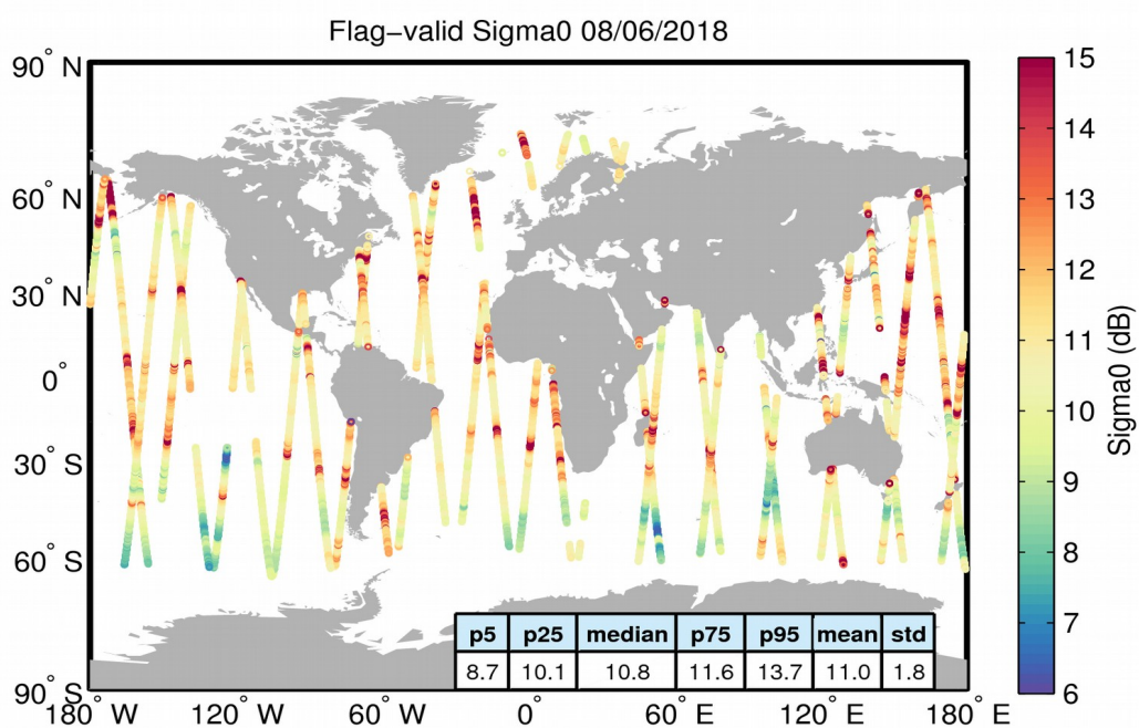
Figure 23. Geographical distribution of flag-valid sigma0 data over oceans and lakes for 08/06/2018. The statistical values shown in the table refer to the sigma0 in dB and are calculated over all measurements shown in the figure.
