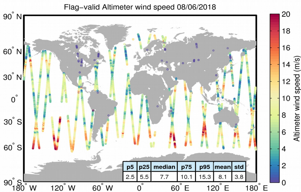
Figure 31. Geographical distribution of flag-valid wind data over oceans and lakes for 08/06/2018. The statistical values shown in the table refer to the wind in m/s and are calculated over all measurements shown in the figure.
