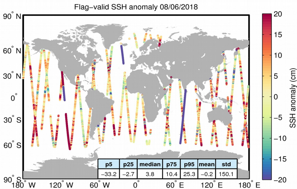
Figure 5. Geographical distribution of flag-valid 1-Hz SSH anomaly data over oceans and lakes for 08/06/2018. The statistical values shown in the table refer to the SSH anomaly in cm and are calculated over all measurements shown in the figure.
