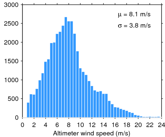
Figure 33. Histogram of flag-valid wind over oceans and lakes for 08/06/2018. The mean ( \mu ) and standard deviation ( \sigma ) are also shown. Note that values larger than 24 m/s are excluded from the histogram for the sake of readability but not from the computation of \mu and \sigma .
