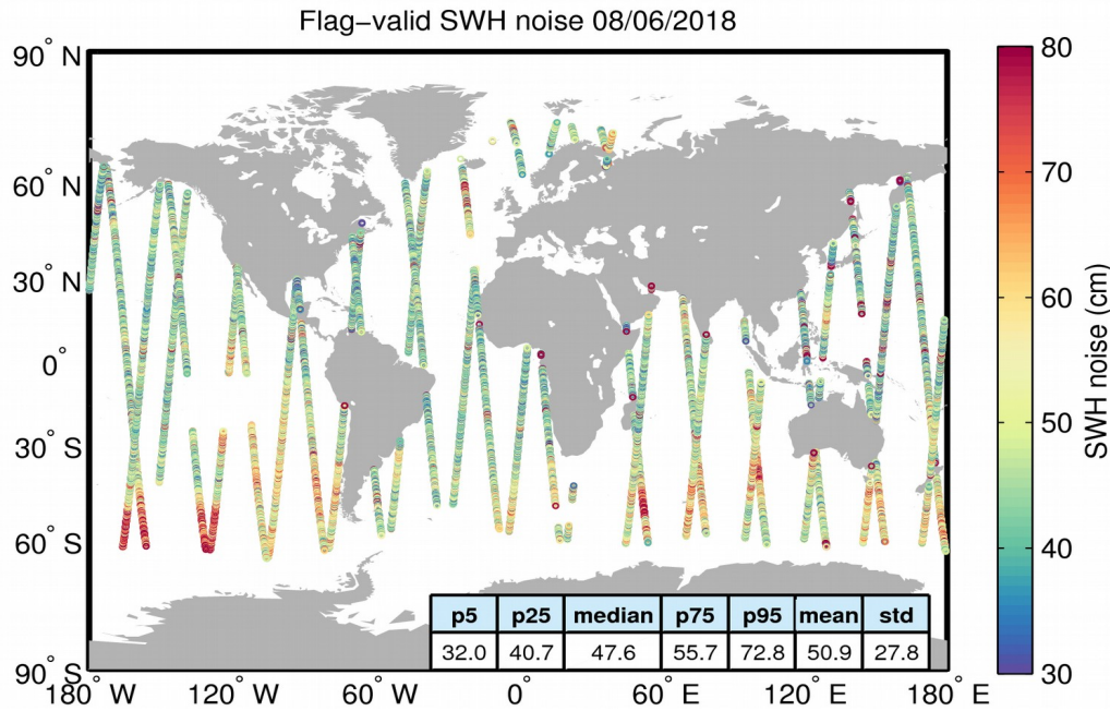
Figure 18. Geographical distribution of flag-valid 20-Hz SWH measurement noise over oceans and lakes for 08/06/2018. The statistical values shown in the table refer to the SWH noise and are calculated over all measurements shown in the figure.
