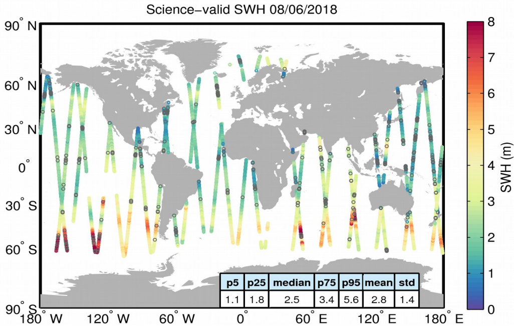
Figure 19. Geographical distribution of science-valid SWH data over oceans and lakes for 08/06/2018. The statistical values shown in the table refer to the SWH in m and are calculated over all measurements shown in the figure. Gray circles denote records that have been rejected based on the editing criteria described in Table 3.
