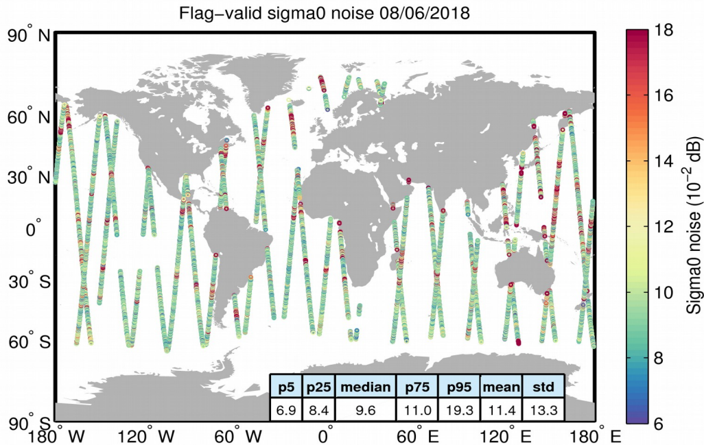
Figure 26. Geographical distribution of flag-valid 20-Hz sigma0 measurement noise over oceans and lakes for 08/06/2018. The statistical values shown in the table refer to the sigma0 noise and are calculated over all measurements shown in the figure.
