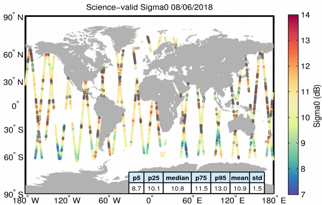
Figure 27. Geographical distribution of science-valid sigma0 data over oceans and lakes for 08/06/2018. The statistical values shown in the table refer to the sigma0 in dB and are calculated over all measurements shown in the figure. Gray circles denote records that have been rejected based on the editing criteria described in Table 4.
