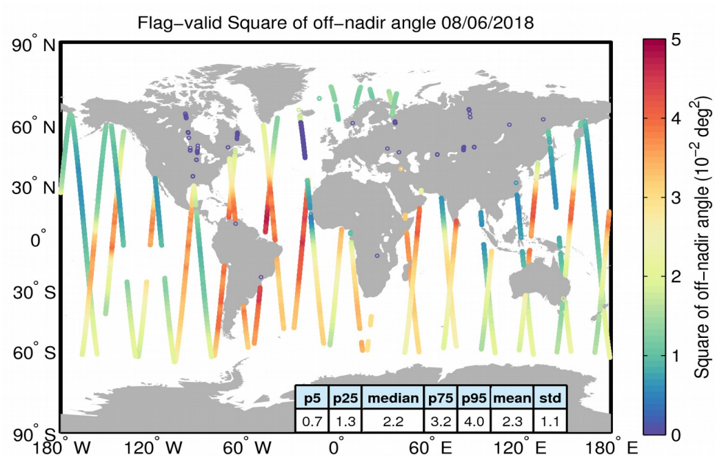
Figure 37. Geographical distribution of flag-valid mispointing data over oceans and lakes for 08/06/2018. The statistical values shown in the table refer to the mispointing in 10^{-2} deg 2 and are calculated over all measurements shown in the figure.
