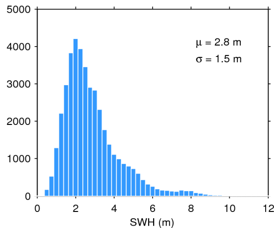
Figure 17. Histogram of flag-valid SWH over oceans and lakes for 08/06/2018. The mean ( \mu ) and standard deviation ( \sigma ) are also shown. Note that values larger than 12 m are excluded from the histogram for the sake of readability but not from the computation of \mu and \sigma .
