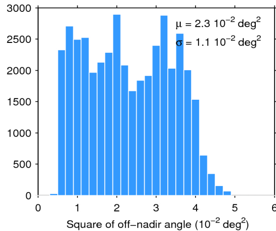
Figure 39. Histogram of flag-valid mispointing over oceans and lakes for 08/06/2018. The mean ( \mu ) and standard deviation ( \sigma ) are also shown. Note that values larger than 6 \cdot 10^{-2} \text{ deg}^2 are excluded from the histogram for the sake of readability but not from the computation of \mu and \sigma .
