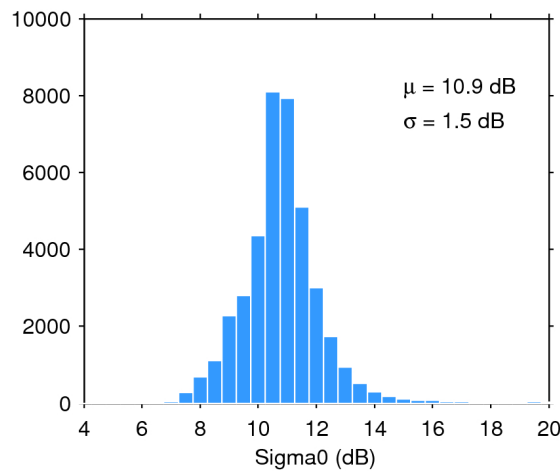
Figure 28. Histogram of science-valid sigma0 over oceans and lakes for 08/06/2018. The mean ( \mu ) and standard deviation ( \sigma ) are also shown. Note that values outside [4 20] dB are excluded from the histogram for the sake of readability but not from the computation of \mu and \sigma .
