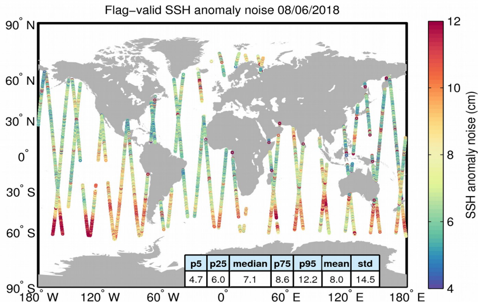
Figure 8. Geographical distribution of flag-valid 20-Hz SSH anomaly measurement noise over oceans and lakes for 08/06/2018. The statistical values shown in the table refer to the SSH anomaly noise and are calculated over all measurements shown in the figure.
