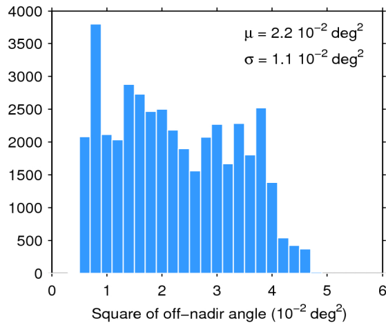
Figure 39. Histogram of flag-valid mispointing over oceans and lakes for 05/06/2018. The mean ( \mu ) and standard deviation ( \sigma ) are also shown. Note that values larger than 6 \cdot 10^{-2} \text{ deg}^2 are excluded from the histogram for the sake of readability but not from the computation of \mu and \sigma .
