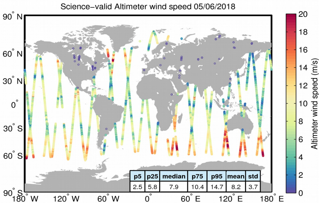
Figure 34. Geographical distribution of science-valid wind data over oceans and lakes for 05/06/2018. The statistical values shown in the table refer to the wind in m/s and are calculated over all measurements shown in the figure. Gray circles denote records that have been rejected based on the editing criteria described in Table 5.
