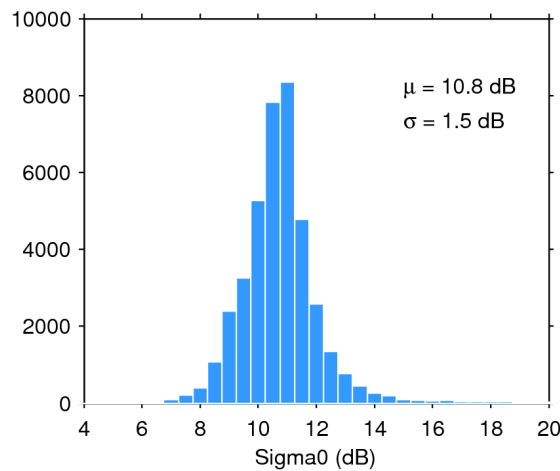
Figure 28. Histogram of science-valid sigma0 over oceans and lakes for 05/06/2018. The mean ( \mu ) and standard deviation ( \sigma ) are also shown. Note that values outside [4 20] dB are excluded from the histogram for the sake of readability but not from the computation of \mu and \sigma .
