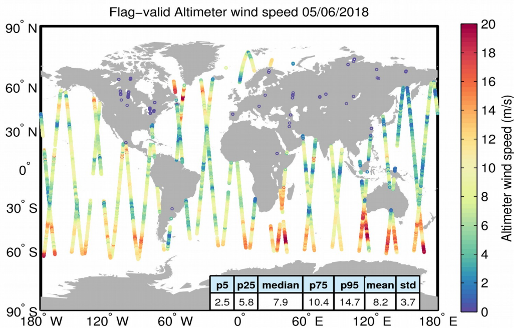
Figure 31. Geographical distribution of flag-valid wind data over oceans and lakes for 05/06/2018. The statistical values shown in the table refer to the wind in m/s and are calculated over all measurements shown in the figure.
