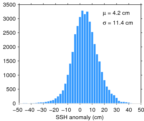
Figure 11. Histogram of science-valid SSH anomaly over oceans and lakes for 05/06/2018. The mean ( \mu ) and standard deviation ( \sigma ) are also shown. Note that values outside [-50 50] cm are excluded from the histogram for the sake of readability but not from the computation of \mu and \sigma .
