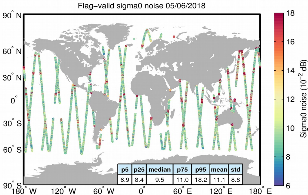
Figure 26. Geographical distribution of flag-valid 20-Hz sigma0 measurement noise over oceans and lakes for 05/06/2018. The statistical values shown in the table refer to the sigma0 noise and are calculated over all measurements shown in the figure.
