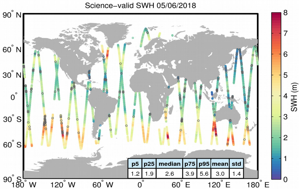
Figure 19. Geographical distribution of science-valid SWH data over oceans and lakes for 05/06/2018. The statistical values shown in the table refer to the SWH in m and are calculated over all measurements shown in the figure. Gray circles denote records that have been rejected based on the editing criteria described in Table 3.
