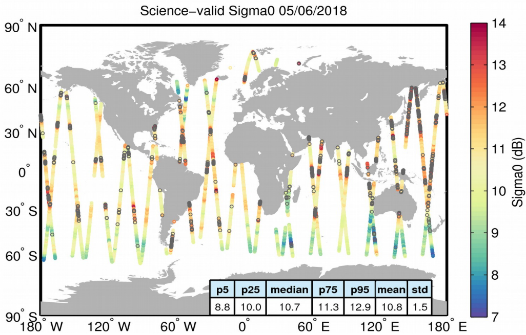
Figure 27. Geographical distribution of science-valid sigma0 data over oceans and lakes for 05/06/2018. The statistical values shown in the table refer to the sigma0 in dB and are calculated over all measurements shown in the figure. Gray circles denote records that have been rejected based on the editing criteria described in Table 4.
