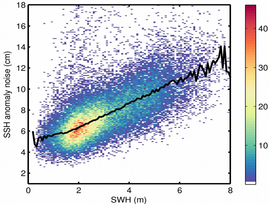
Figure 9. 2D histogram showing flag-valid SSH anomaly noise as a function of SWH for 05/06/2018. The black line denotes the median SSH anomaly noise as a function of SWH.
