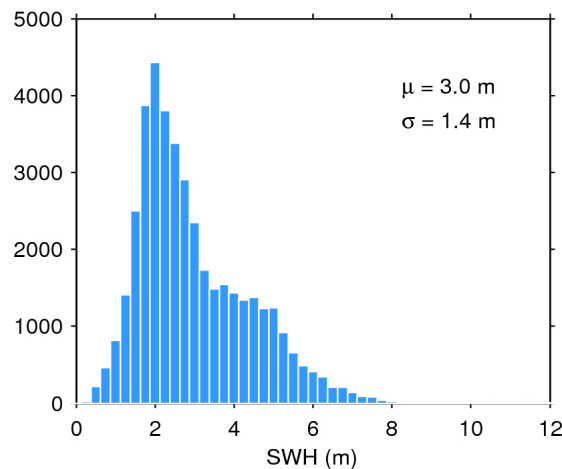
Figure 17. Histogram of flag-valid SWH over oceans and lakes for 05/06/2018. The mean ( \mu ) and standard deviation ( \sigma ) are also shown. Note that values larger than 12 m are excluded from the histogram for the sake of readability but not from the computation of \mu and \sigma .
