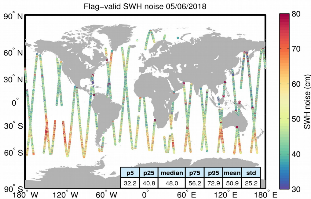
Figure 18. Geographical distribution of flag-valid 20-Hz SWH measurement noise over oceans and lakes for 05/06/2018. The statistical values shown in the figure refer to the SWH noise and are calculated over all measurements shown in the figure.
