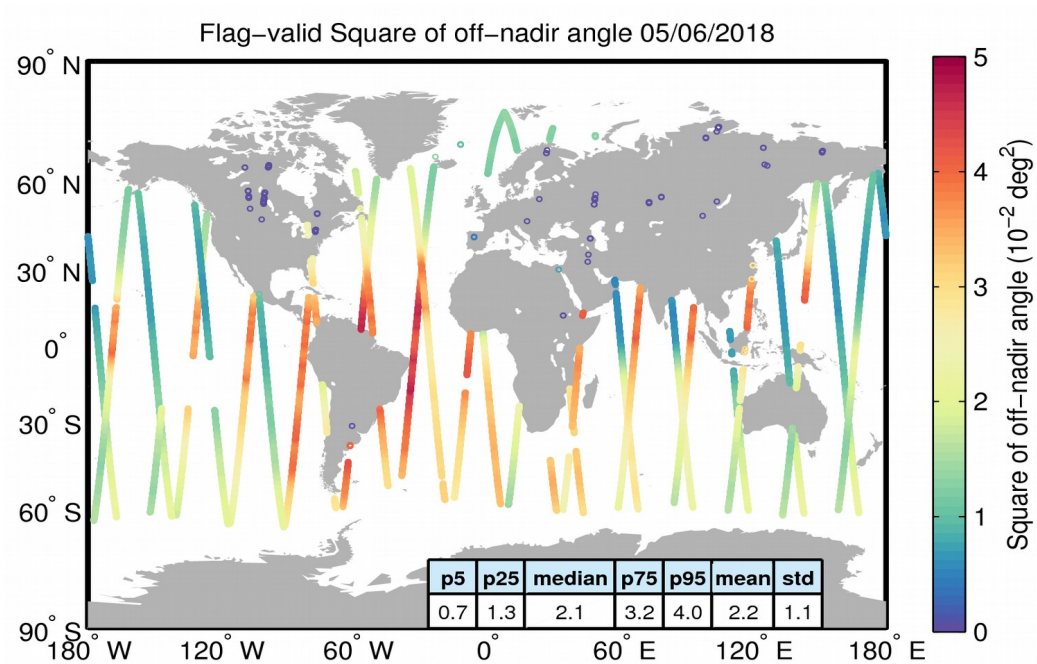
Figure 37. Geographical distribution of flag-valid mispointing data over oceans and lakes for 05/06/2018. The statistical values shown in the table refer to the mispointing in 10^{-2} deg 2 and are calculated over all measurements shown in the figure.
