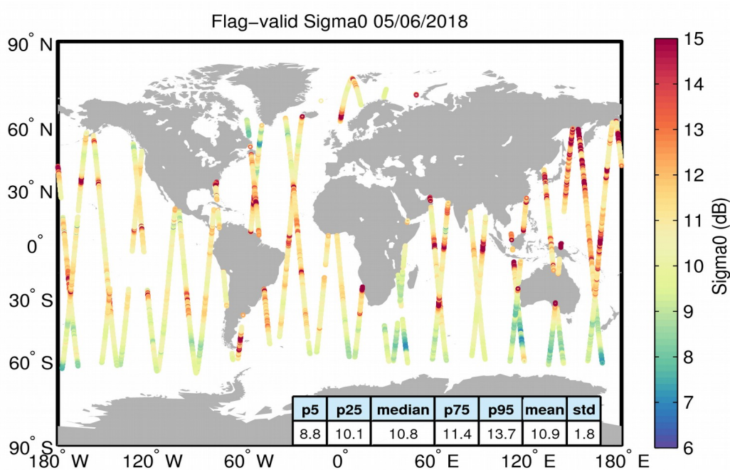
Figure 23. Geographical distribution of flag-valid sigma0 data over oceans and lakes for 05/06/2018. The statistical values shown in the table refer to the sigma0 in dB and are calculated over all measurements shown in the figure.
