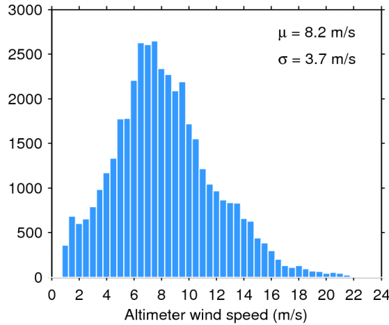
Figure 33. Histogram of flag-valid wind over oceans and lakes for 05/06/2018. The mean ( \mu ) and standard deviation ( \sigma ) are also shown. Note that values larger than 24 m/s are excluded from the histogram for the sake of readability but not from the computation of \mu and \sigma .
