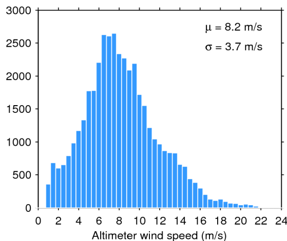
Figure 35. Histogram of science-valid wind over oceans and lakes for 05/06/2018. The mean ( \mu ) and standard deviation ( \sigma ) are also shown. Note that values larger than 24 m/s are excluded from the histogram for the sake of readability but not from the computation of \mu and \sigma .
