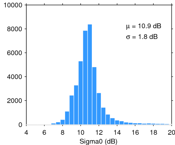
Figure 25. Histogram of flag-valid sigma0 over oceans and lakes for 05/06/2018. The mean ( \mu ) and standard deviation ( \sigma ) are also shown. Note that values outside [4 20] dB are excluded from the histogram for the sake of readability but not from the computation of \mu and \sigma .
