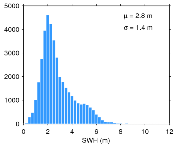
Figure 20. Histogram of science-valid SWH over oceans and lakes for 04/06/2018. The mean ( \mu ) and standard deviation ( \sigma ) are also shown. Note that values larger than 12 m are excluded from the histogram for the sake of readability but not from the computation of \mu and \sigma .
