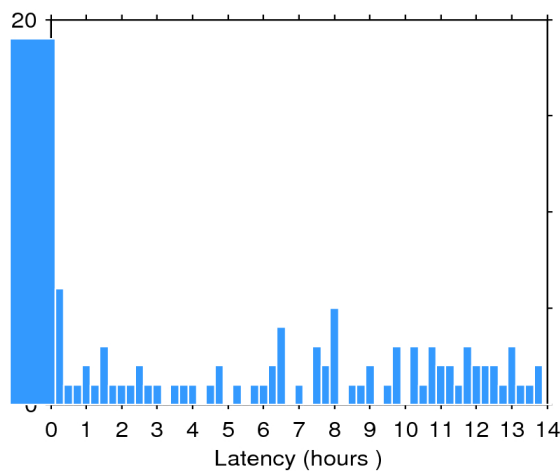
Figure 2. Histogram of the data latency for 04/06/2018. The y-axis denotes the number of files that are made available with a delay of x-hours with respect to the mean time of the records stored in the file.
