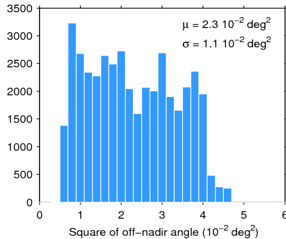
Figure 39. Histogram of flag-valid mispointing over oceans and lakes for 04/06/2018. The mean ( \mu ) and standard deviation ( \sigma ) are also shown. Note that values larger than 6 \cdot 10^{-2} \text{ deg}^2 are excluded from the histogram for the sake of readability but not from the computation of \mu and \sigma .
