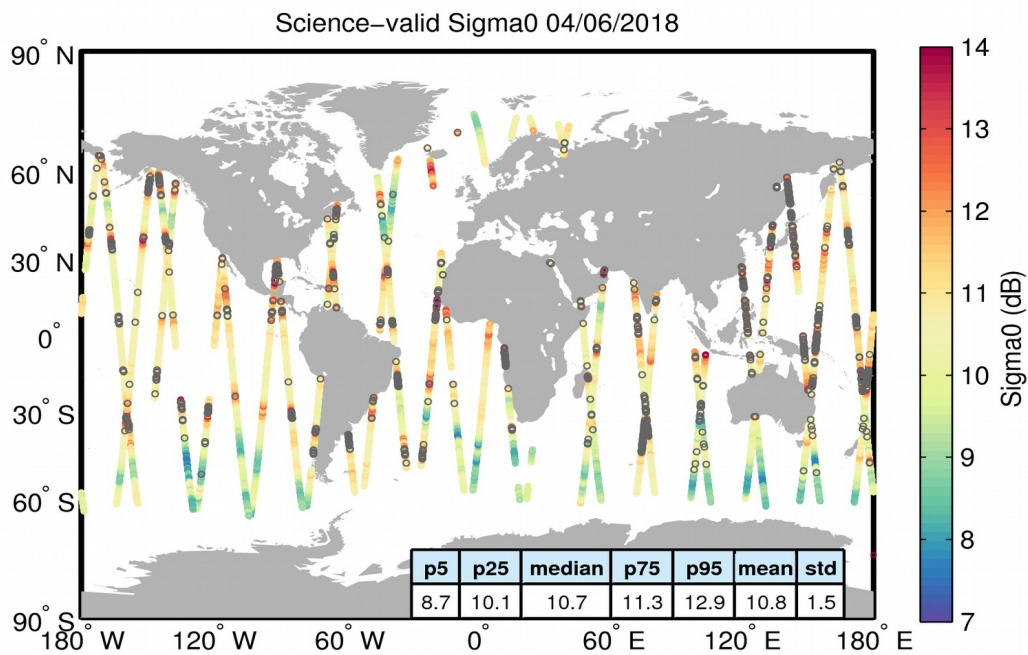
Figure 27. Geographical distribution of science-valid sigma0 data over oceans and lakes for 04/06/2018. The statistical values shown in the table refer to the sigma0 in dB and are calculated over all measurements shown in the figure. Gray circles denote records that have been rejected based on the editing criteria described in Table 4.
