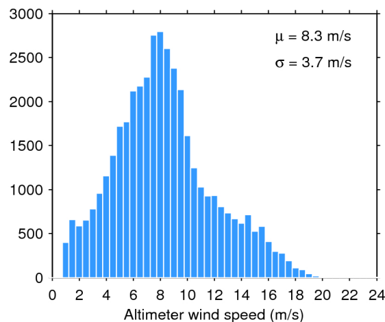
Figure 35. Histogram of science-valid wind over oceans and lakes for 04/06/2018. The mean ( \mu ) and standard deviation ( \sigma ) are also shown. Note that values larger than 24 m/s are excluded from the histogram for the sake of readability but not from the computation of \mu and \sigma .
