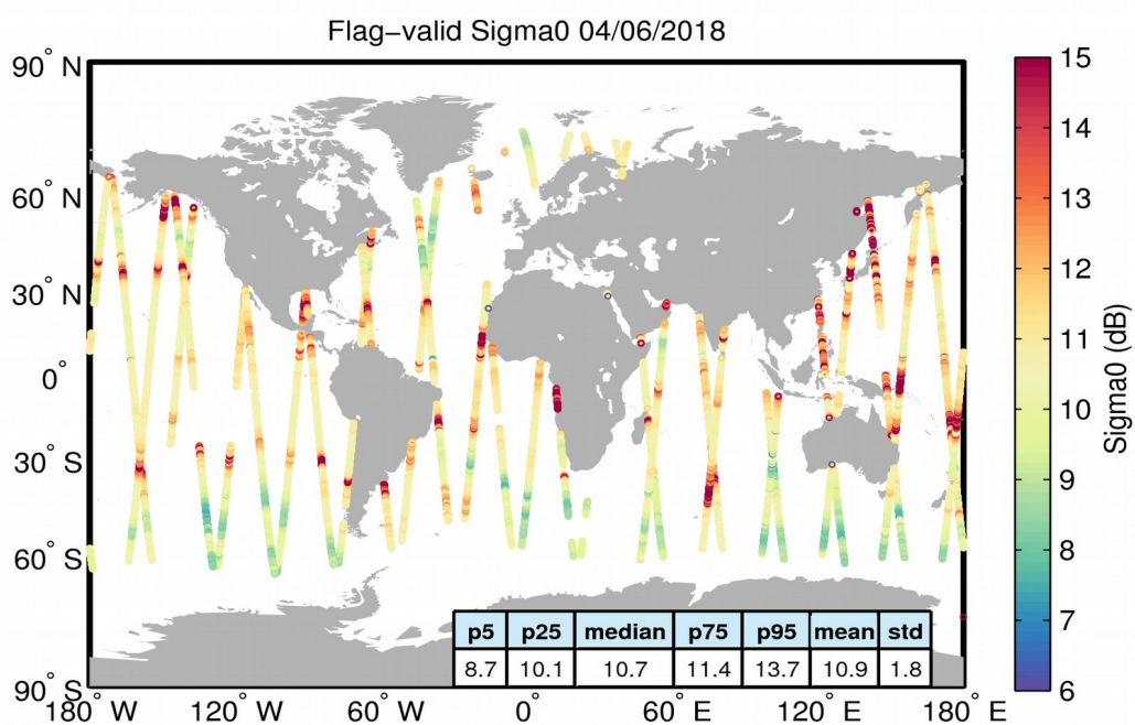
Figure 23. Geographical distribution of flag-valid sigma0 data over oceans and lakes for 04/06/2018. The statistical values shown in the table refer to the sigma0 in dB and are calculated over all measurements shown in the figure.
