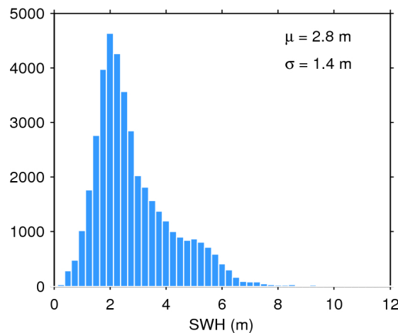
Figure 17. Histogram of flag-valid SWH over oceans and lakes for 04/06/2018. The mean ( \mu ) and standard deviation ( \sigma ) are also shown. Note that values larger than 12 m are excluded from the histogram for the sake of readability but not from the computation of \mu and \sigma .
