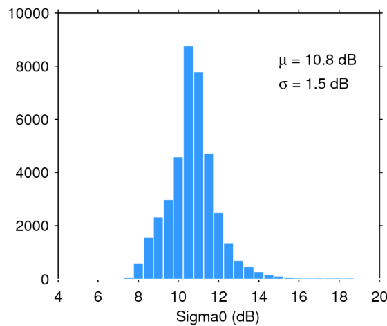
Figure 28. Histogram of science-valid sigma0 over oceans and lakes for 04/06/2018. The mean ( \mu ) and standard deviation ( \sigma ) are also shown. Note that values outside [4 20] dB are excluded from the histogram for the sake of readability but not from the computation of \mu and \sigma .
