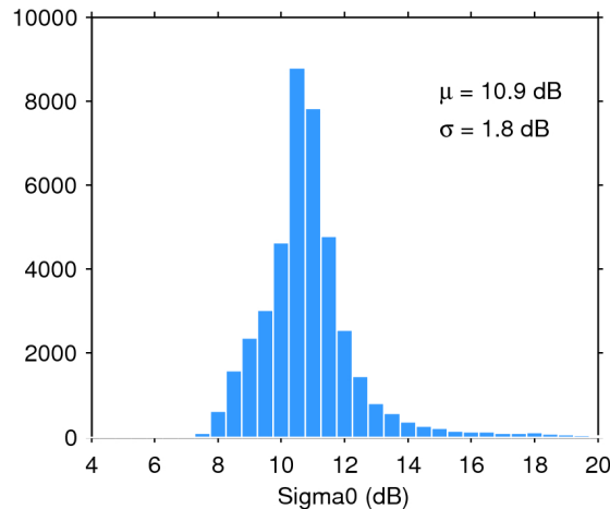
Figure 25. Histogram of flag-valid sigma0 over oceans and lakes for 04/06/2018. The mean ( \mu ) and standard deviation ( \sigma ) are also shown. Note that values outside [4 20] dB are excluded from the histogram for the sake of readability but not from the computation of \mu and \sigma .
