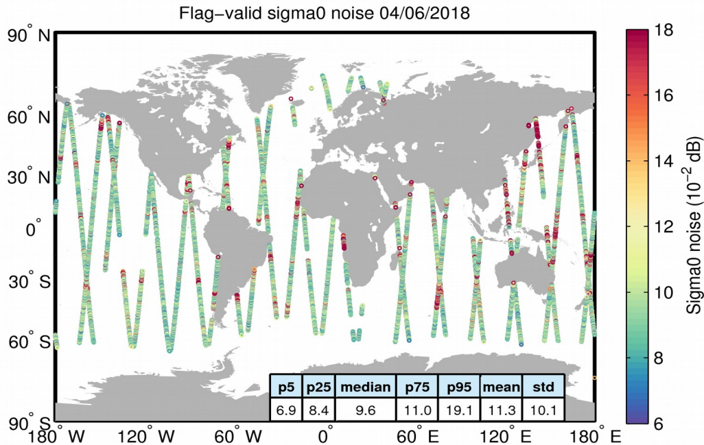
Figure 26. Geographical distribution of flag-valid 20-Hz sigma0 measurement noise over oceans and lakes for 04/06/2018. The statistical values shown in the table refer to the sigma0 noise and are calculated over all measurements shown in the figure.
