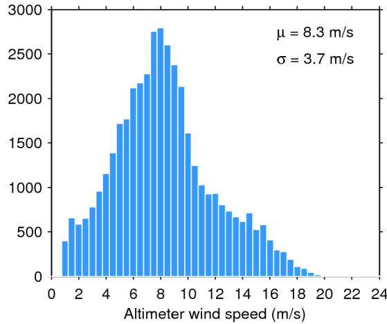
Figure 33. Histogram of flag-valid wind over oceans and lakes for 04/06/2018. The mean ( \mu ) and standard deviation ( \sigma ) are also shown. Note that values larger than 24 m/s are excluded from the histogram for the sake of readability but not from the computation of \mu and \sigma .
