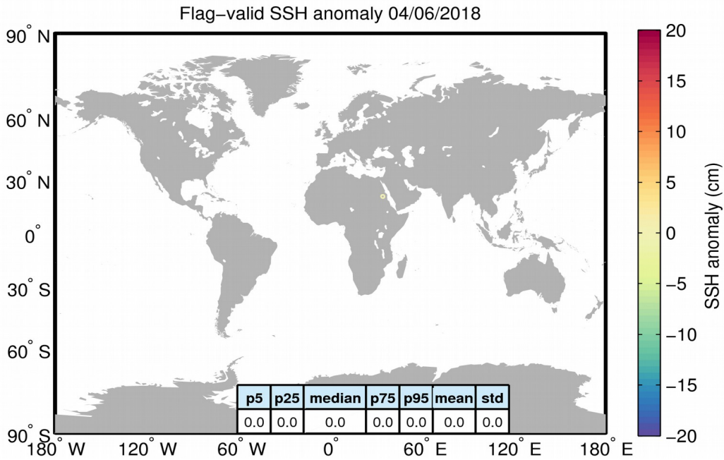
Figure 5. Geographical distribution of flag-valid 1-Hz SSH anomaly data over oceans and lakes for 04/06/2018. The statistical values shown in the table refer to the SSH anomaly in cm and are calculated over all measurements shown in the figure.
