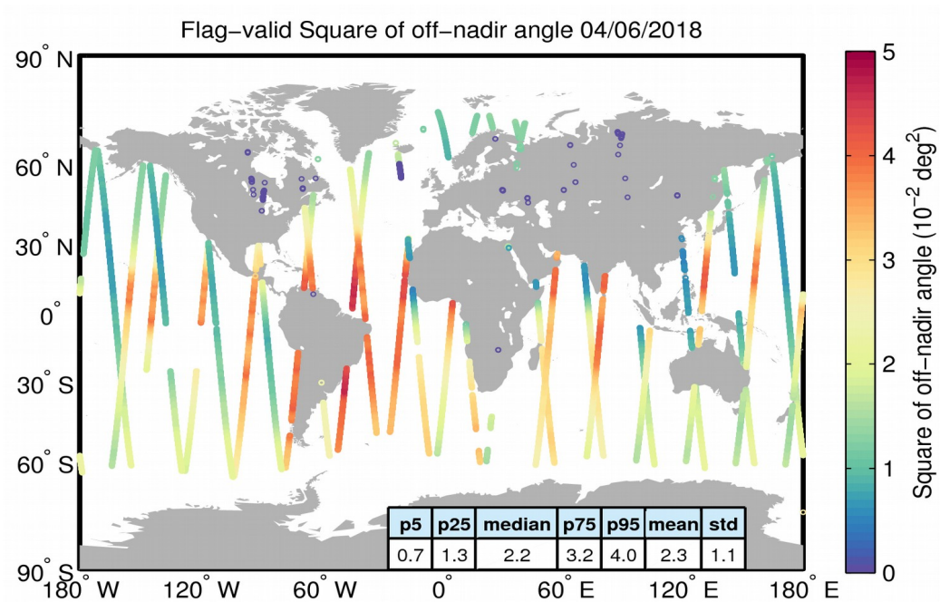
Figure 37. Geographical distribution of flag-valid mispointing data over oceans and lakes for 04/06/2018. The statistical values shown in the table refer to the mispointing in 10^{-2} \text{ deg}^2 and are calculated over all measurements shown in the figure.
