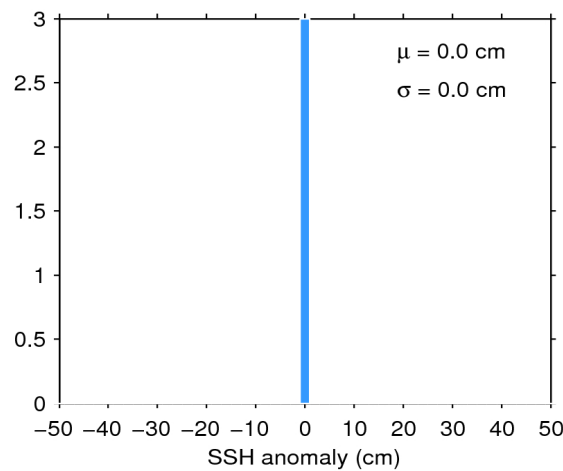
Figure 7. Histogram of flag-valid SSH anomaly over oceans and lakes for 04/06/2018. The mean ( \mu ) and standard deviation ( \sigma ) are also shown. Note that values outside [-50\ 50] cm are excluded from the histogram for the sake of readability but not from the computation of \mu and \sigma .
