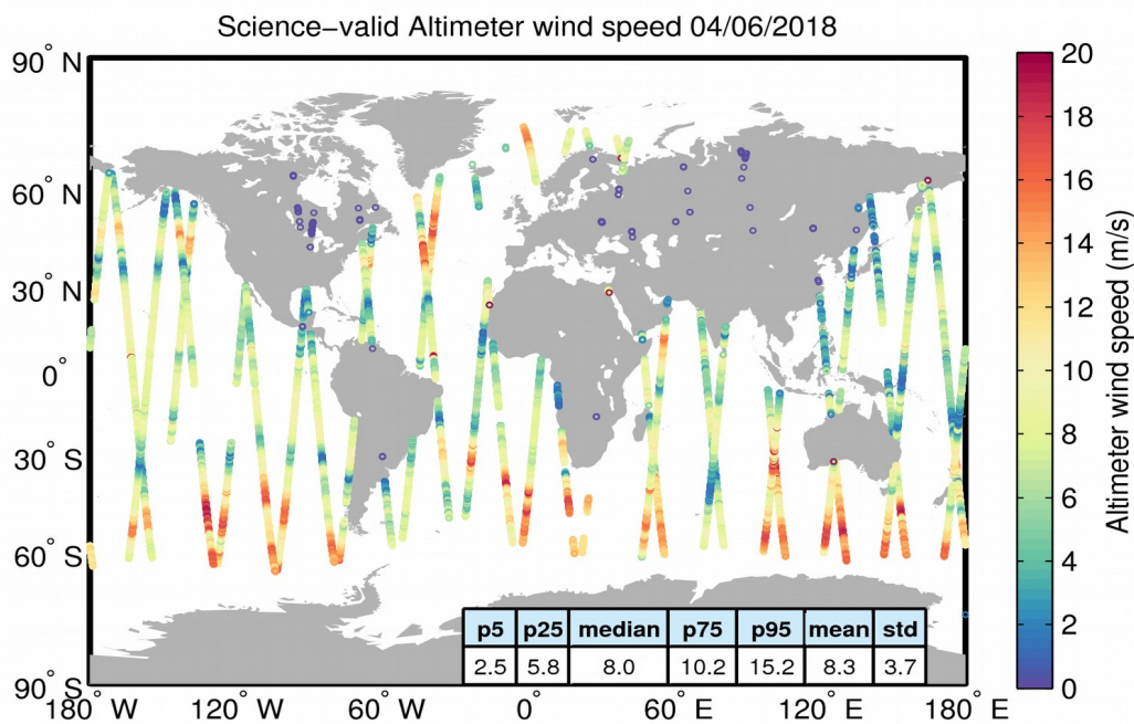
Figure 34. Geographical distribution of science-valid wind data over oceans and lakes for 04/06/2018. The statistical values shown in the table refer to the wind in m/s and are calculated over all measurements shown in the figure. Gray circles denote records that have been rejected based on the editing criteria described in Table 5.
