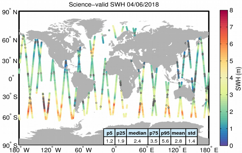
Figure 19. Geographical distribution of science-valid SWH data over oceans and lakes for 04/06/2018. The statistical values shown in the table refer to the SWH in m and are calculated over all measurements shown in the figure. Gray circles denote records that have been rejected based on the editing criteria described in Table 3.
