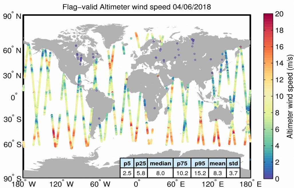
Figure 31. Geographical distribution of flag-valid wind data over oceans and lakes for 04/06/2018. The statistical values shown in the table refer to the wind in m/s and are calculated over all measurements shown in the figure.
