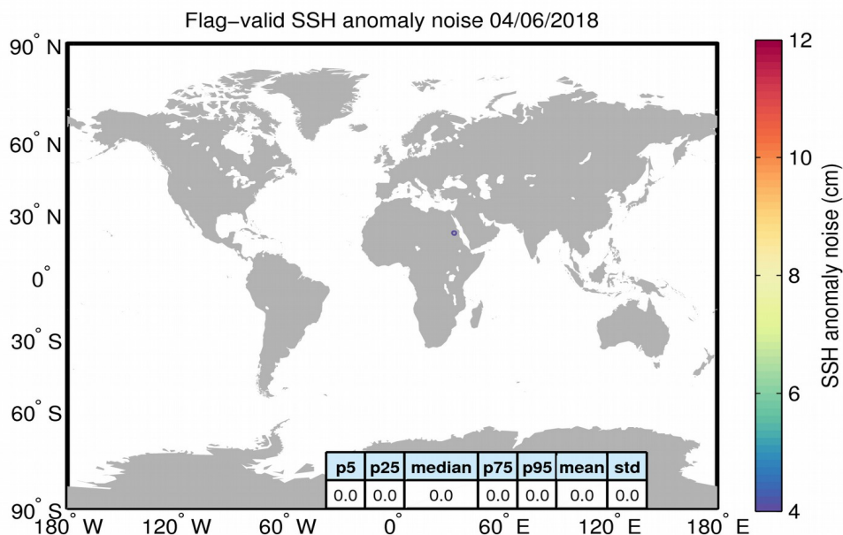
Figure 8. Geographical distribution of flag-valid 20-Hz SSH anomaly measurement noise over oceans and lakes for 04/06/2018. The statistical values shown in the table refer to the SSH anomaly noise and are calculated over all measurements shown in the figure.
