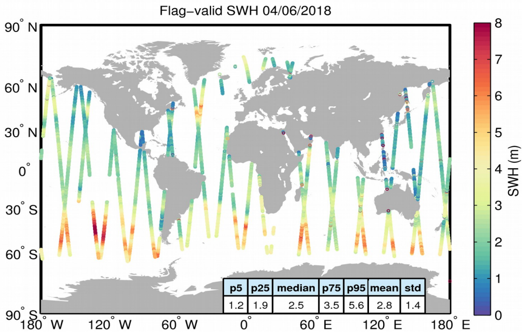
Figure 15. Geographical distribution of flag-valid SWH data over oceans and lakes for 04/06/2018. The statistical values shown in the table refer to the SWH in m and are calculated over all measurements shown in the figure.
