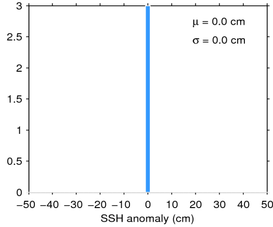
Figure 11. Histogram of science-valid SSH anomaly over oceans and lakes for 04/06/2018. The mean ( \mu ) and standard deviation ( \sigma ) are also shown. Note that values outside [-50 50] cm are excluded from the histogram for the sake of readability but not from the computation of \mu and \sigma .
