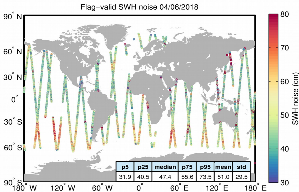
Figure 18. Geographical distribution of flag-valid 20-Hz SWH measurement noise over oceans and lakes for 04/06/2018. The statistical values shown in the table refer to the SWH noise and are calculated over all measurements shown in the figure.
