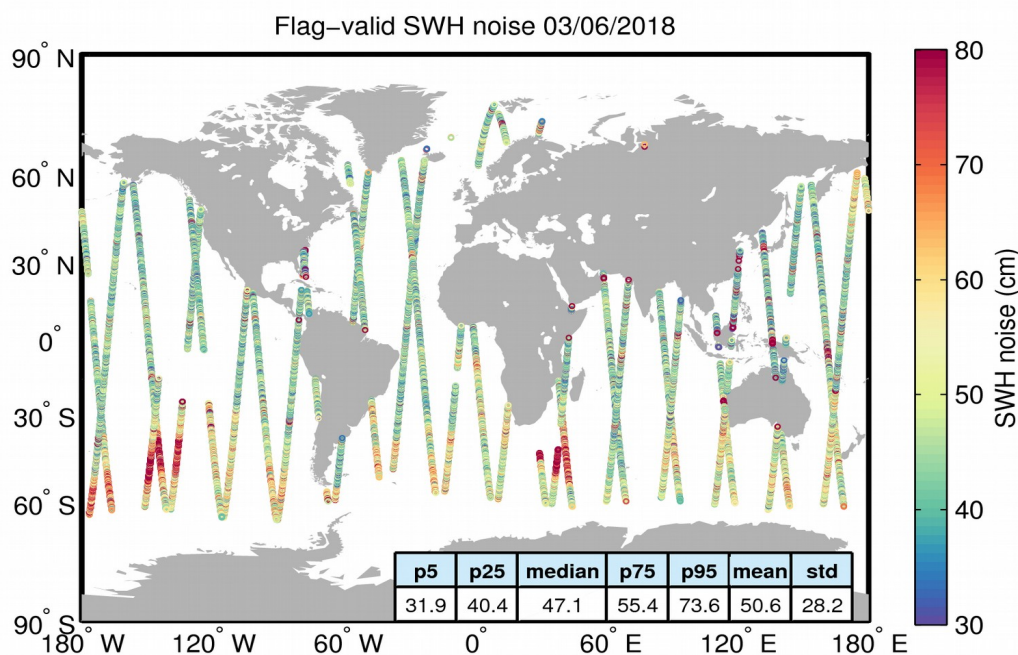
Figure 18. Geographical distribution of flag-valid 20-Hz SWH measurement noise over oceans and lakes for 03/06/2018. The statistical values shown in the table refer to the SWH noise and are calculated over all measurements shown in the figure.
