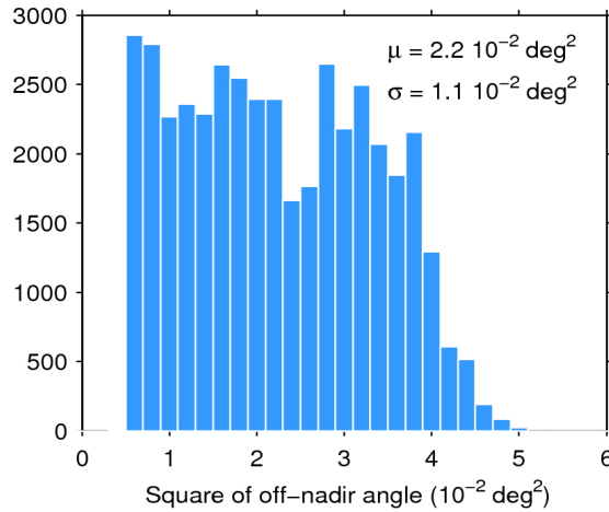
Figure 39. Histogram of flag-valid mispointing over oceans and lakes for 03/06/2018. The mean ( \mu ) and standard deviation ( \sigma ) are also shown. Note that values larger than 6 \cdot 10^{-2} \text{ deg}^2 are excluded from the histogram for the sake of readability but not from the computation of \mu and \sigma .
