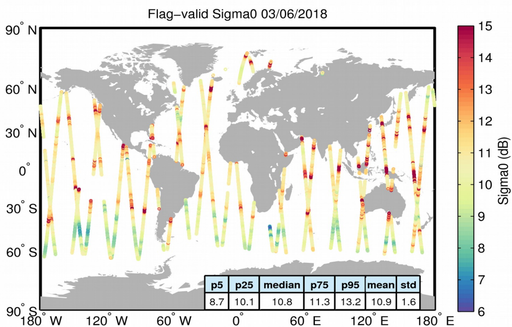
Figure 23. Geographical distribution of flag-valid sigma0 data over oceans and lakes for 03/06/2018. The statistical values shown in the table refer to the sigma0 in dB and are calculated over all measurements shown in the figure.
