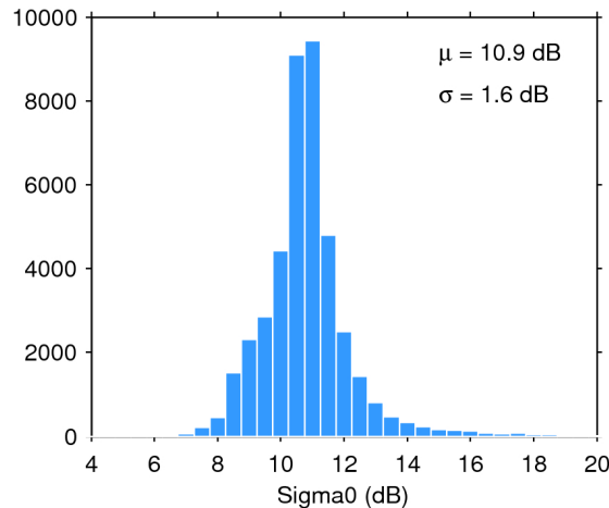
Figure 25. Histogram of flag-valid sigma0 over oceans and lakes for 03/06/2018. The mean ( \mu ) and standard deviation ( \sigma ) are also shown. Note that values outside [4 20] dB are excluded from the histogram for the sake of readability but not from the computation of \mu and \sigma .
