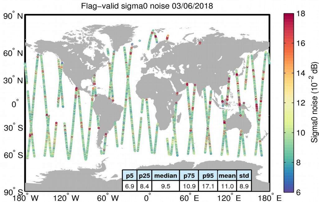
Figure 26. Geographical distribution of flag-valid 20-Hz sigma0 measurement noise over oceans and lakes for 03/06/2018. The statistical values shown in the table refer to the sigma0 noise and are calculated over all measurements shown in the figure.
