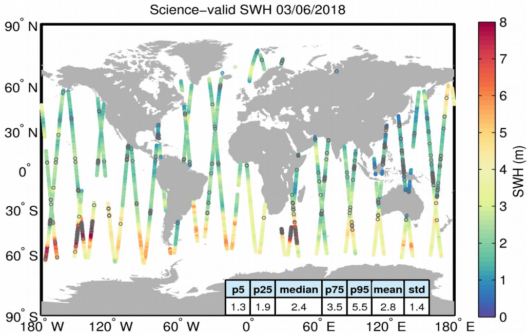
Figure 19. Geographical distribution of science-valid SWH data over oceans and lakes for 03/06/2018. The statistical values shown in the table refer to the SWH in m and are calculated over all measurements shown in the figure. Gray circles denote records that have been rejected based on the editing criteria described in Table 3.
