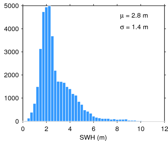
Figure 20. Histogram of science-valid SWH over oceans and lakes for 03/06/2018. The mean ( \mu ) and standard deviation ( \sigma ) are also shown. Note that values larger than 12 m are excluded from the histogram for the sake of readability but not from the computation of \mu and \sigma .
