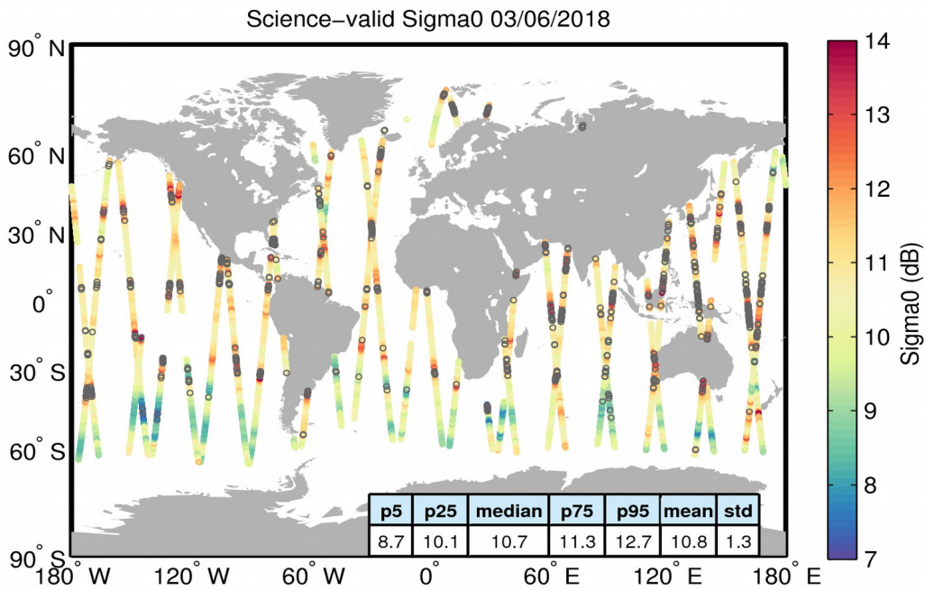
Figure 27. Geographical distribution of science-valid sigma0 data over oceans and lakes for 03/06/2018. The statistical values shown in the table refer to the sigma0 in dB and are calculated over all measurements shown in the figure. Gray circles denote records that have been rejected based on the editing criteria described in Table 4.
