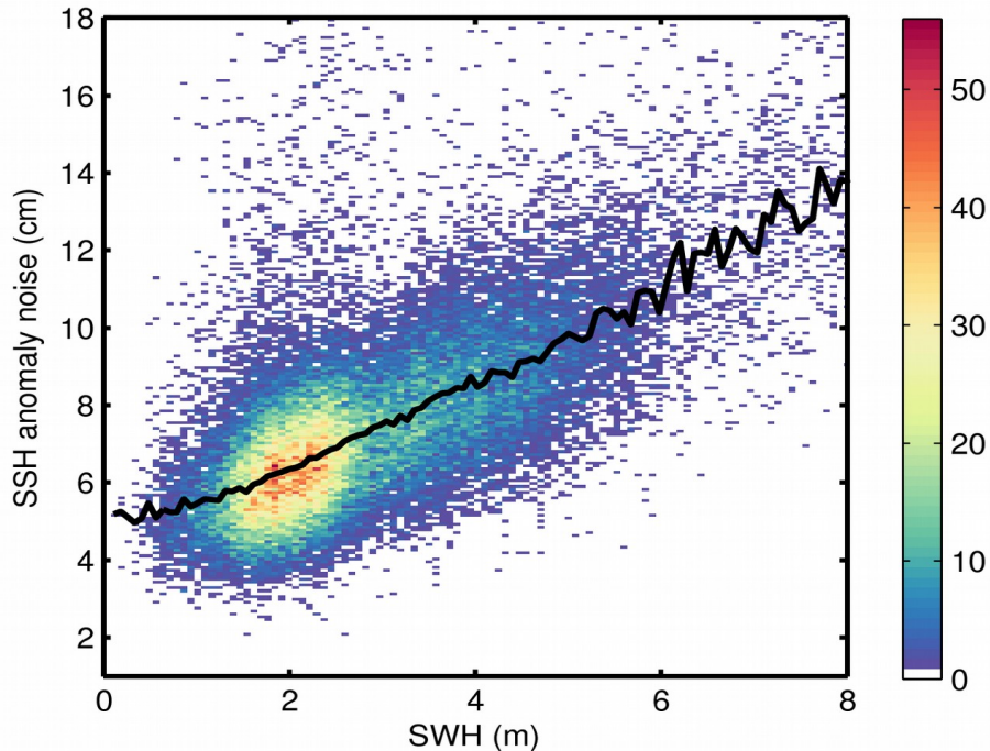
Figure 9. 2D histogram showing flag-valid SSH anomaly noise as a function of SWH for 03/06/2018. The black line denotes the median SSH anomaly noise as a function of SWH.
