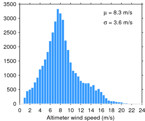
Figure 33. Histogram of flag-valid wind over oceans and lakes for 03/06/2018. The mean ( \mu ) and standard deviation ( \sigma ) are also shown. Note that values larger than 24 m/s are excluded from the histogram for the sake of readability but not from the computation of \mu and \sigma .
