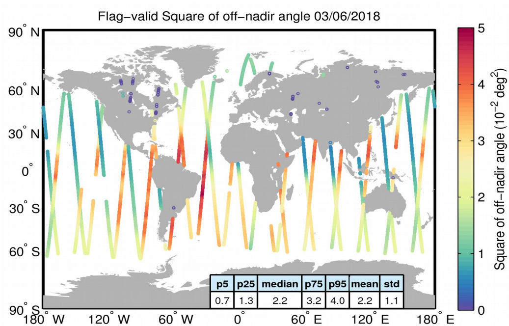
Figure 37. Geographical distribution of flag-valid mispointing data over oceans and lakes for 03/06/2018. The statistical values shown in the table refer to the mispointing in 10^{-2} \text{ deg}^2 and are calculated over all measurements shown in the figure.
