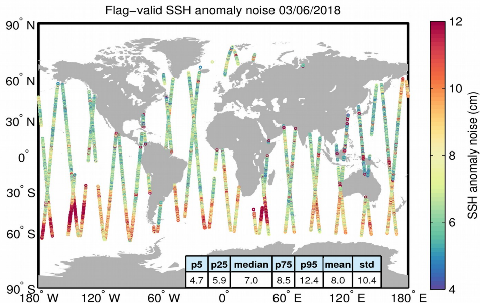
Figure 8. Geographical distribution of flag-valid 20-Hz SSH anomaly measurement noise over oceans and lakes for 03/06/2018. The statistical values shown in the table refer to the SSH anomaly noise and are calculated over all measurements shown in the figure.
