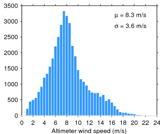
Figure 35. Histogram of science-valid wind over oceans and lakes for 03/06/2018. The mean ( \mu ) and standard deviation ( \sigma ) are also shown. Note that values larger than 24 m/s are excluded from the histogram for the sake of readability but not from the computation of \mu and \sigma .
