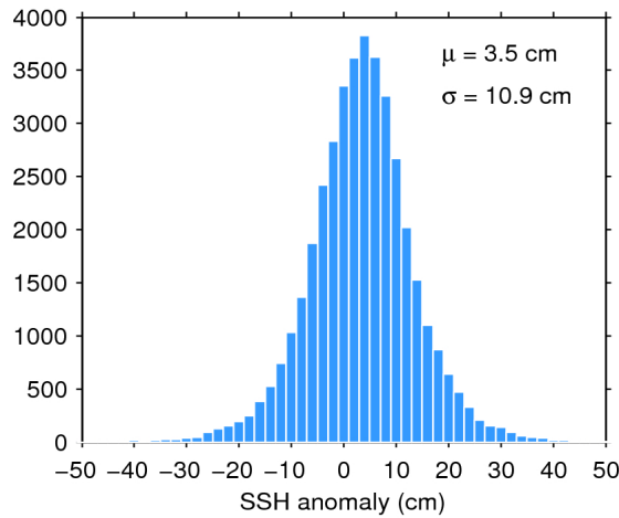
Figure 11. Histogram of science-valid SSH anomaly over oceans and lakes for 03/06/2018. The mean ( \mu ) and standard deviation ( \sigma ) are also shown. Note that values outside [-50 50] cm are excluded from the histogram for the sake of readability but not from the computation of \mu and \sigma .
