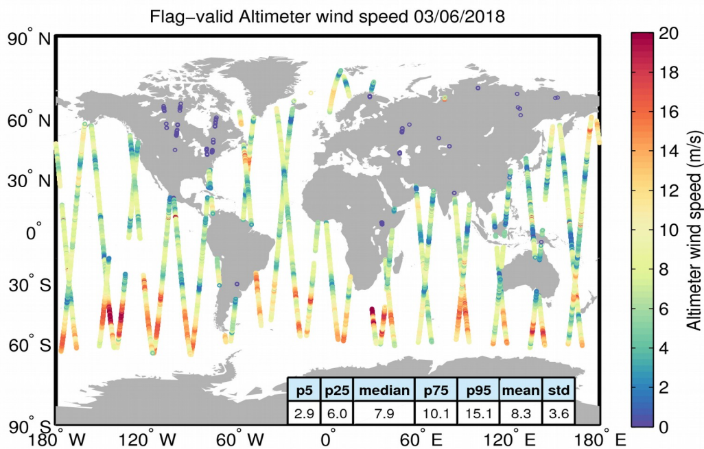
Figure 31. Geographical distribution of flag-valid wind data over oceans and lakes for 03/06/2018. The statistical values shown in the table refer to the wind in m/s and are calculated over all measurements shown in the figure.
