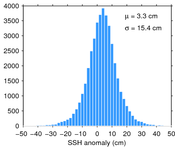
Figure 7. Histogram of flag-valid SSH anomaly over oceans and lakes for 03/06/2018. The mean ( \mu ) and standard deviation ( \sigma ) are also shown. Note that values outside [-50\ 50] cm are excluded from the histogram for the sake of readability but not from the computation of \mu and \sigma .
