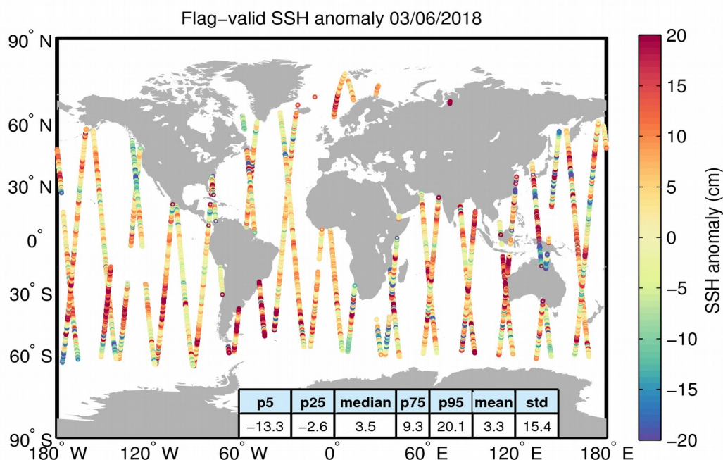
Figure 5. Geographical distribution of flag-valid 1-Hz SSH anomaly data over oceans and lakes for 03/06/2018. The statistical values shown in the table refer to the SSH anomaly in cm and are calculated over all measurements shown in the figure.
