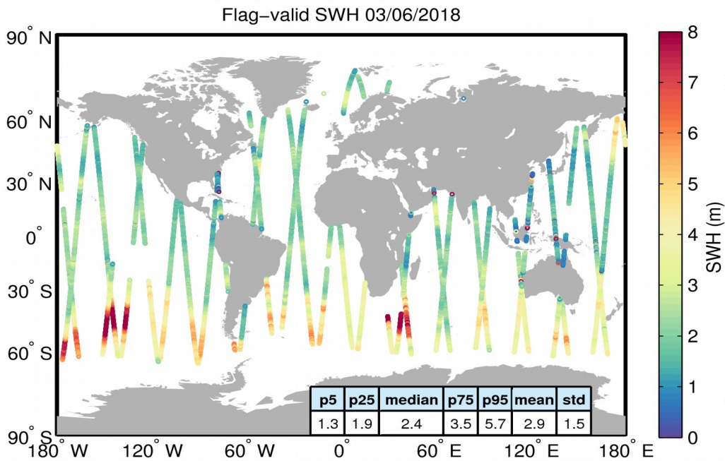
Figure 15. Geographical distribution of flag-valid SWH data over oceans and lakes for 03/06/2018. The statistical values shown in the table refer to the SWH in m and are calculated over all measurements shown in the figure.
