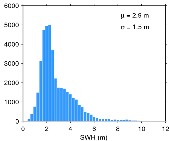
Figure 17. Histogram of flag-valid SWH over oceans and lakes for 03/06/2018. The mean ( \mu ) and standard deviation ( \sigma ) are also shown. Note that values larger than 12 m are excluded from the histogram for the sake of readability but not from the computation of \mu and \sigma .
