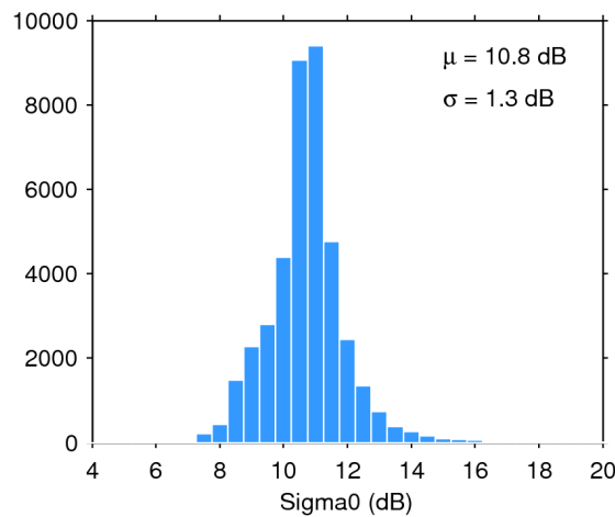
Figure 28. Histogram of science-valid sigma0 over oceans and lakes for 03/06/2018. The mean ( \mu ) and standard deviation ( \sigma ) are also shown. Note that values outside [4 20] dB are excluded from the histogram for the sake of readability but not from the computation of \mu and \sigma .
