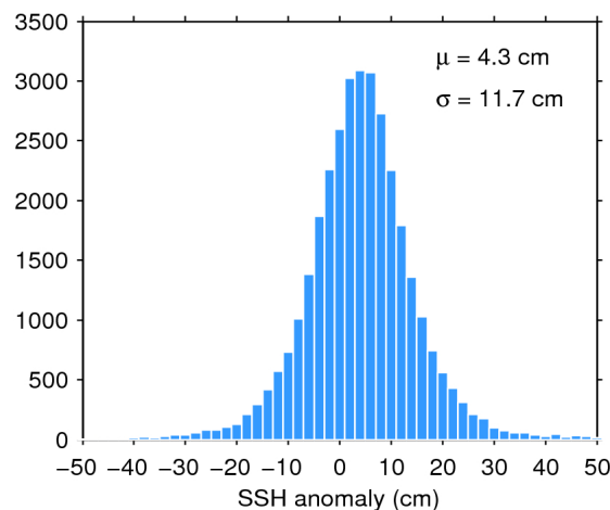
Figure 11. Histogram of science-valid SSH anomaly over oceans and lakes for 31/05/2018. The mean ( \mu ) and standard deviation ( \sigma ) are also shown. Note that values outside [-50 50] cm are excluded from the histogram for the sake of readability but not from the computation of \mu and \sigma .
