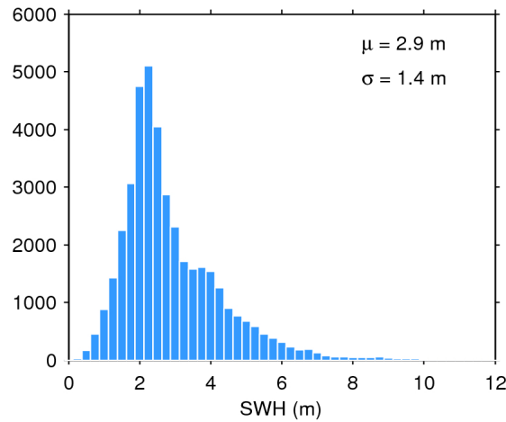
Figure 17. Histogram of flag-valid SWH over oceans and lakes for 31/05/2018. The mean ( \mu ) and standard deviation ( \sigma ) are also shown. Note that values larger than 12 m are excluded from the histogram for the sake of readability but not from the computation of \mu and \sigma .
