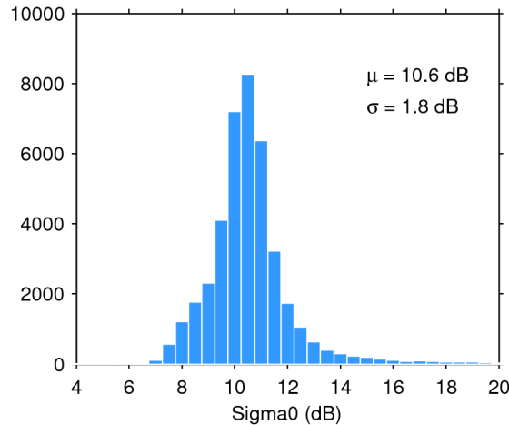
Figure 25. Histogram of flag-valid sigma0 over oceans and lakes for 31/05/2018. The mean ( \mu ) and standard deviation ( \sigma ) are also shown. Note that values outside [4 20] dB are excluded from the histogram for the sake of readability but not from the computation of \mu and \sigma .
