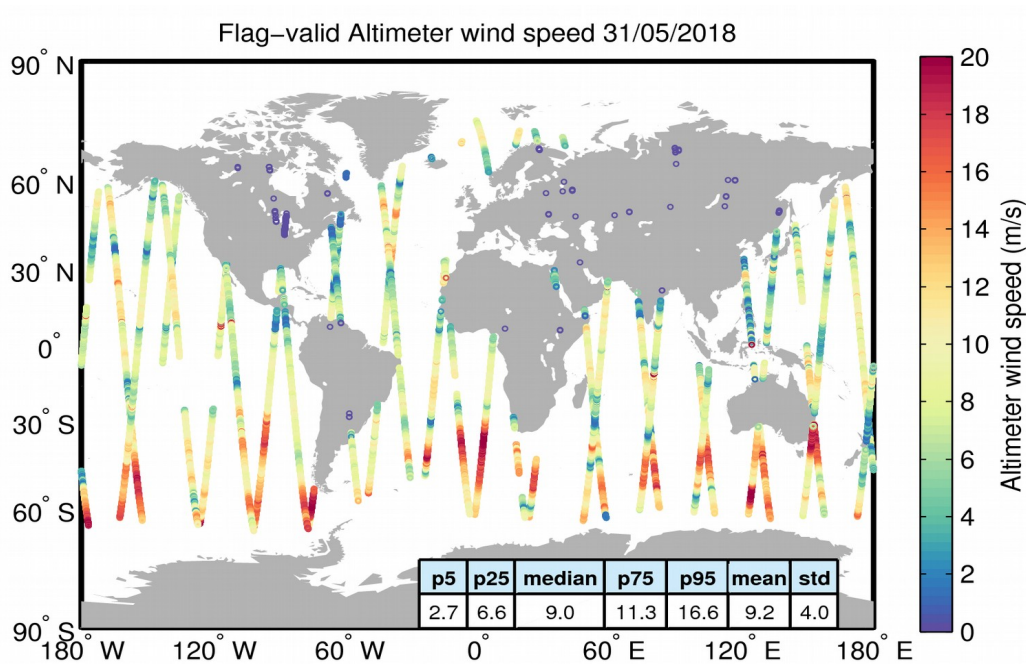
Figure 31. Geographical distribution of flag-valid wind data over oceans and lakes for 31/05/2018. The statistical values shown in the table refer to the wind in m/s and are calculated over all measurements shown in the figure.
