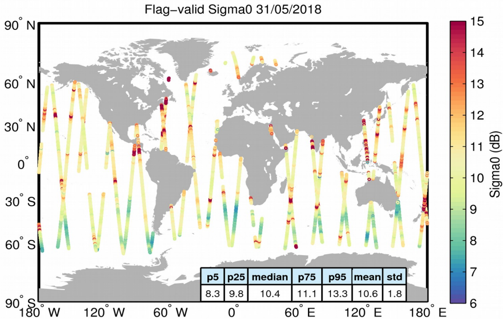
Figure 23. Geographical distribution of flag-valid sigma0 data over oceans and lakes for 31/05/2018. The statistical values shown in the table refer to the sigma0 in dB and are calculated over all measurements shown in the figure.
