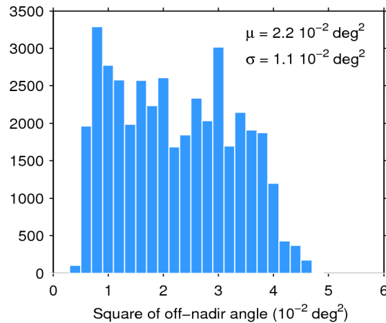
Figure 39. Histogram of flag-valid mispointing over oceans and lakes for 31/05/2018. The mean ( \mu ) and standard deviation ( \sigma ) are also shown. Note that values larger than 6 \cdot 10^{-2} \text{ deg}^2 are excluded from the histogram for the sake of readability but not from the computation of \mu and \sigma .
