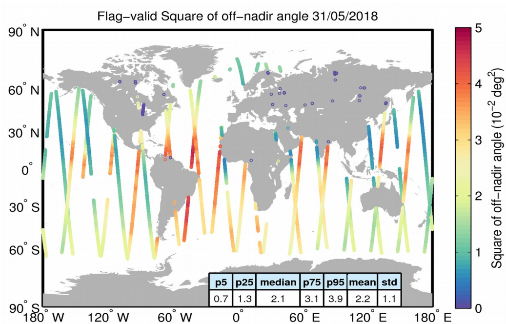
Figure 37. Geographical distribution of flag-valid mispointing data over oceans and lakes for 31/05/2018. The statistical values shown in the table refer to the mispointing in 10^{-2} \text{ deg}^2 and are calculated over all measurements shown in the figure.
