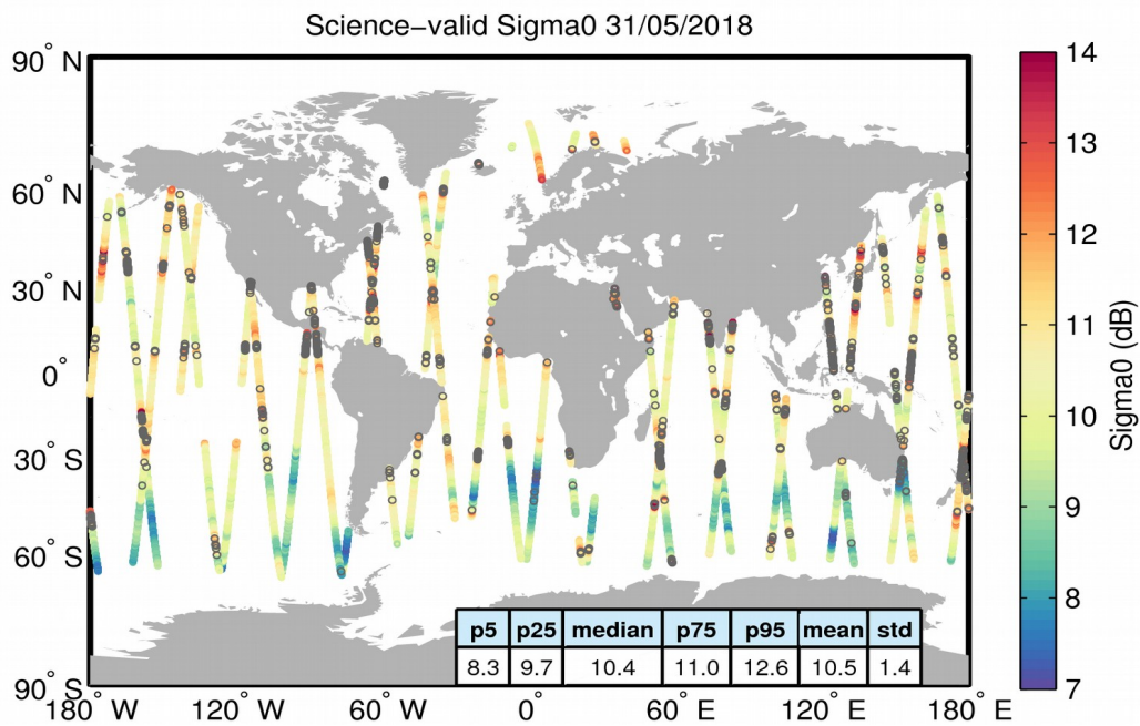
Figure 27. Geographical distribution of science-valid sigma0 data over oceans and lakes for 31/05/2018. The statistical values shown in the table refer to the sigma0 in dB and are calculated over all measurements shown in the figure. Gray circles denote records that have been rejected based on the editing criteria described in Table 4.
