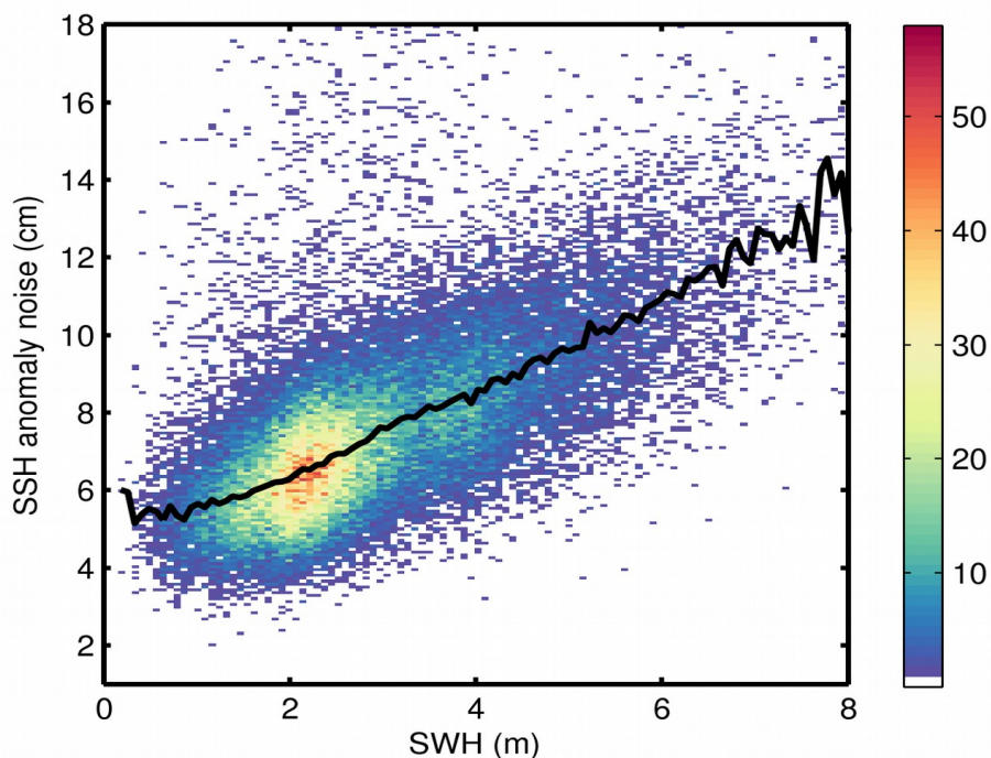
Figure 9. 2D histogram showing flag-valid SSH anomaly noise as a function of SWH for 31/05/2018. The black line denotes the median SSH anomaly noise as a function of SWH.
