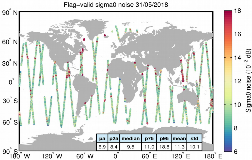
Figure 26. Geographical distribution of flag-valid 20-Hz sigma0 measurement noise over oceans and lakes for 31/05/2018. The statistical values shown in the table refer to the sigma0 noise and are calculated over all measurements shown in the figure.
