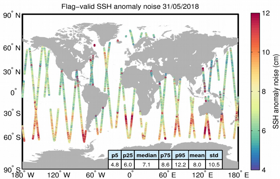
Figure 8. Geographical distribution of flag-valid 20-Hz SSH anomaly measurement noise over oceans and lakes for 31/05/2018. The statistical values shown in the table refer to the SSH anomaly noise and are calculated over all measurements shown in the figure.
