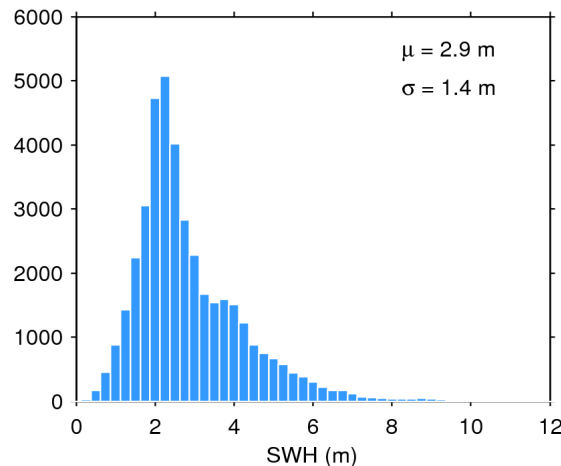
Figure 20. Histogram of science-valid SWH over oceans and lakes for 31/05/2018. The mean ( \mu ) and standard deviation ( \sigma ) are also shown. Note that values larger than 12 m are excluded from the histogram for the sake of readability but not from the computation of \mu and \sigma .
