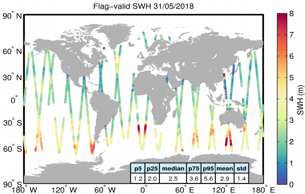
Figure 15. Geographical distribution of flag-valid SWH data over oceans and lakes for 31/05/2018. The statistical values shown in the table refer to the SWH in m and are calculated over all measurements shown in the figure.
