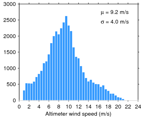
Figure 33. Histogram of flag-valid wind over oceans and lakes for 31/05/2018. The mean ( \mu ) and standard deviation ( \sigma ) are also shown. Note that values larger than 24 m/s are excluded from the histogram for the sake of readability but not from the computation of \mu and \sigma .
