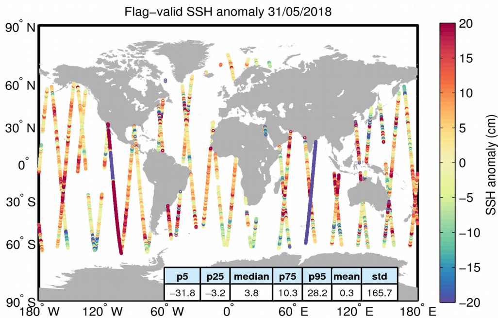
Figure 5. Geographical distribution of flag-valid 1-Hz SSH anomaly data over oceans and lakes for 31/05/2018. The statistical values shown in the table refer to the SSH anomaly in cm and are calculated over all measurements shown in the figure.
