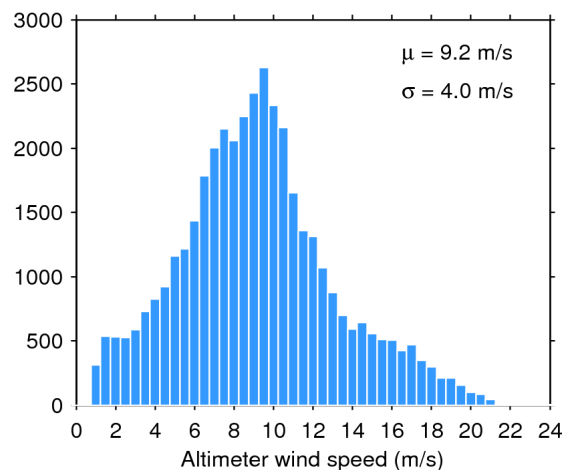
Figure 35. Histogram of science-valid wind over oceans and lakes for 31/05/2018. The mean ( \mu ) and standard deviation ( \sigma ) are also shown. Note that values larger than 24 m/s are excluded from the histogram for the sake of readability but not from the computation of \mu and \sigma .
