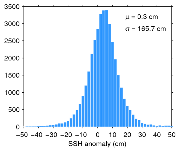
Figure 7. Histogram of flag-valid SSH anomaly over oceans and lakes for 31/05/2018. The mean ( \mu ) and standard deviation ( \sigma ) are also shown. Note that values outside [-50 50] cm are excluded from the histogram for the sake of readability but not from the computation of \mu and \sigma .
