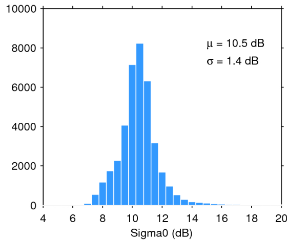
Figure 28. Histogram of science-valid sigma0 over oceans and lakes for 31/05/2018. The mean ( \mu ) and standard deviation ( \sigma ) are also shown. Note that values outside [4 20] dB are excluded from the histogram for the sake of readability but not from the computation of \mu and \sigma .
