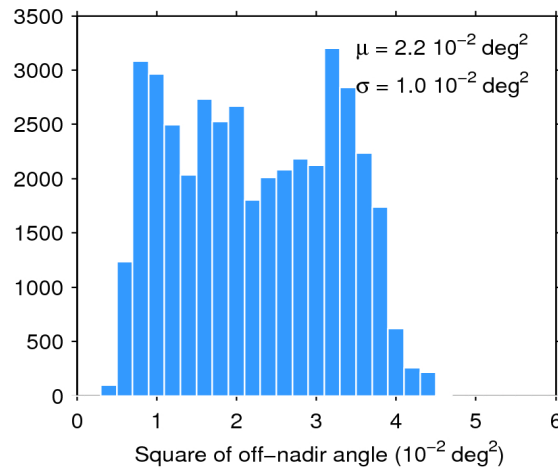
Figure 39. Histogram of flag-valid mispointing over oceans and lakes for 29/05/2018. The mean ( \mu ) and standard deviation ( \sigma ) are also shown. Note that values larger than 6 \cdot 10^{-2} \text{ deg}^2 are excluded from the histogram for the sake of readability but not from the computation of \mu and \sigma .
