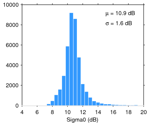
Figure 25. Histogram of flag-valid sigma0 over oceans and lakes for 29/05/2018. The mean ( \mu ) and standard deviation ( \sigma ) are also shown. Note that values outside [4 20] dB are excluded from the histogram for the sake of readability but not from the computation of \mu and \sigma .
