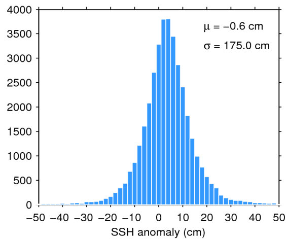
Figure 7. Histogram of flag-valid SSH anomaly over oceans and lakes for 29/05/2018. The mean ( \mu ) and standard deviation ( \sigma ) are also shown. Note that values outside [-50 50] cm are excluded from the histogram for the sake of readability but not from the computation of \mu and \sigma .
