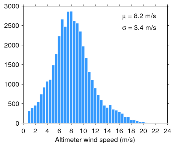
Figure 35. Histogram of science-valid wind over oceans and lakes for 29/05/2018. The mean ( \mu ) and standard deviation ( \sigma ) are also shown. Note that values larger than 24 m/s are excluded from the histogram for the sake of readability but not from the computation of \mu and \sigma .
