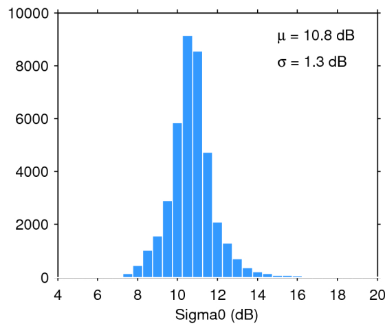
Figure 28. Histogram of science-valid sigma0 over oceans and lakes for 29/05/2018. The mean ( \mu ) and standard deviation ( \sigma ) are also shown. Note that values outside [4 20] dB are excluded from the histogram for the sake of readability but not from the computation of \mu and \sigma .
