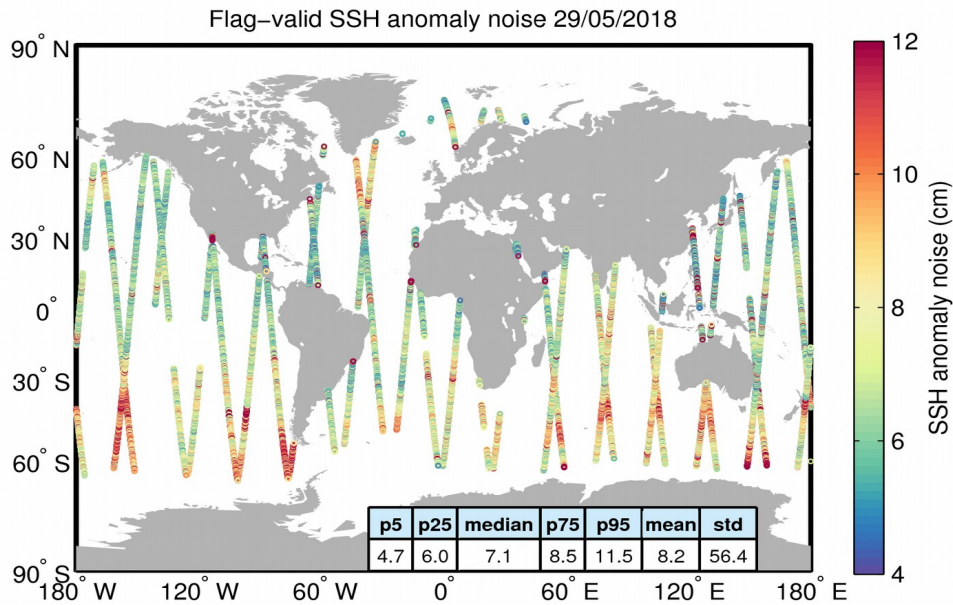
Figure 8. Geographical distribution of flag-valid 20-Hz SSH anomaly measurement noise over oceans and lakes for 29/05/2018. The statistical values shown in the table refer to the SSH anomaly noise and are calculated over all measurements shown in the figure.
