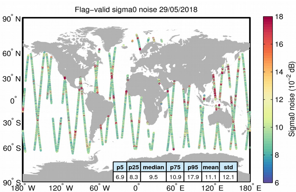
Figure 26. Geographical distribution of flag-valid 20-Hz sigma0 measurement noise over oceans and lakes for 29/05/2018. The statistical values shown in the table refer to the sigma0 noise and are calculated over all measurements shown in the figure.
