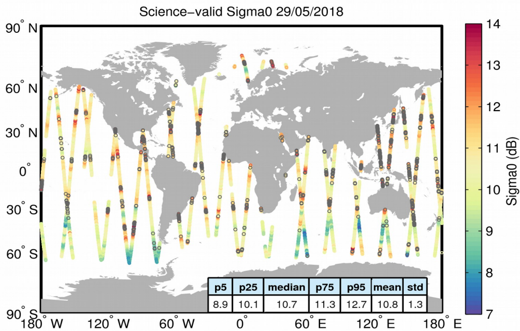
Figure 27. Geographical distribution of science-valid sigma0 data over oceans and lakes for 29/05/2018. The statistical values shown in the table refer to the sigma0 in dB and are calculated over all measurements shown in the figure. Gray circles denote records that have been rejected based on the editing criteria described in Table 4.
