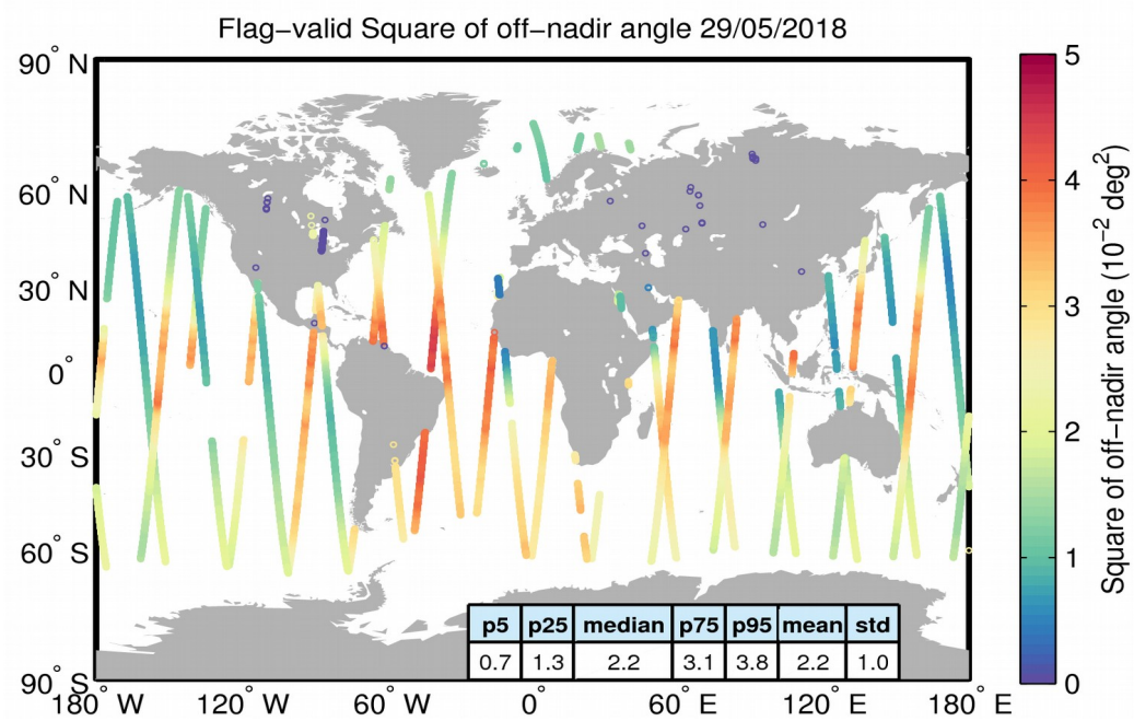
Figure 37. Geographical distribution of flag-valid mispointing data over oceans and lakes for 29/05/2018. The statistical values shown in the table refer to the mispointing in 10^{-2} \text{ deg}^2 and are calculated over all measurements shown in the figure.
