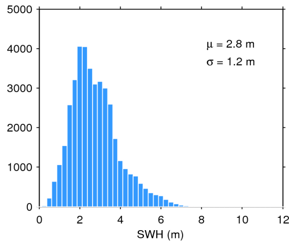
Figure 17. Histogram of flag-valid SWH over oceans and lakes for 29/05/2018. The mean ( \mu ) and standard deviation ( \sigma ) are also shown. Note that values larger than 12 m are excluded from the histogram for the sake of readability but not from the computation of \mu and \sigma .
