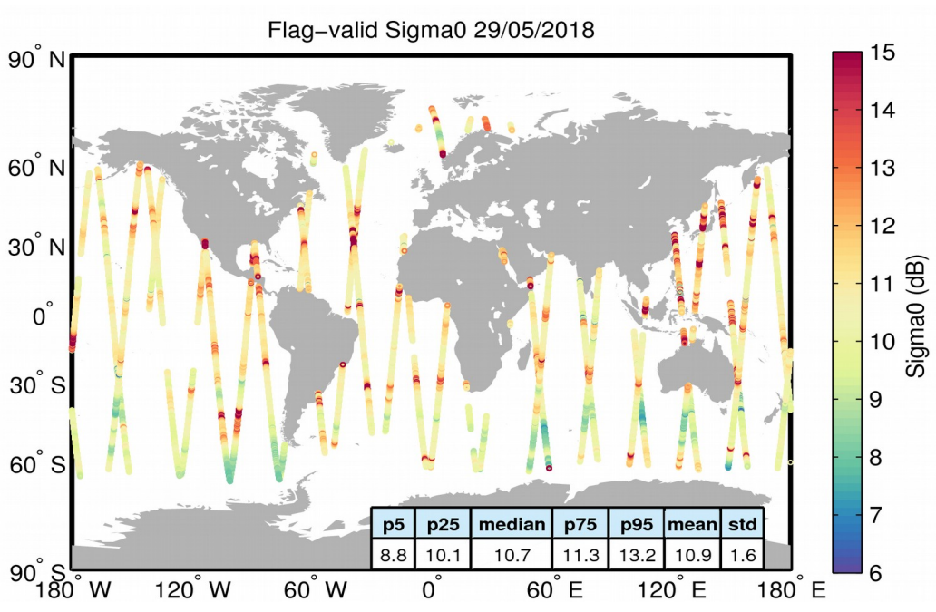
Figure 23. Geographical distribution of flag-valid sigma0 data over oceans and lakes for 29/05/2018. The statistical values shown in the table refer to the sigma0 in dB and are calculated over all measurements shown in the figure.
