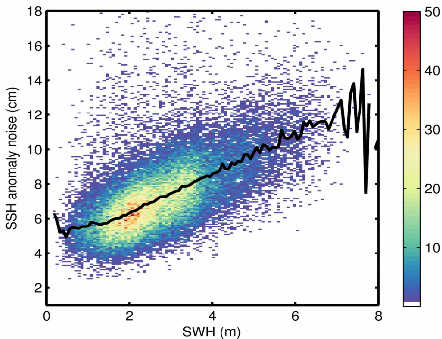
Figure 9. 2D histogram showing flag-valid SSH anomaly noise as a function of SWH for 29/05/2018. The black line denotes the median SSH anomaly noise as a function of SWH.
