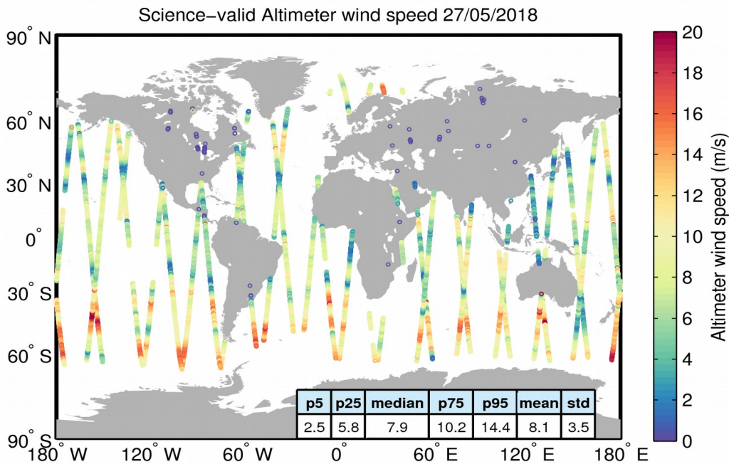
Figure 34. Geographical distribution of science-valid wind data over oceans and lakes for 27/05/2018. The statistical values shown in the table refer to the wind in m/s and are calculated over all measurements shown in the figure. Gray circles denote records that have been rejected based on the editing criteria described in Table 5.
