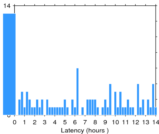
Figure 2. Histogram of the data latency for 27/05/2018. The y-axis denotes the number of files that are made available with a delay of x-hours with respect to the mean time of the records stored in the file.
