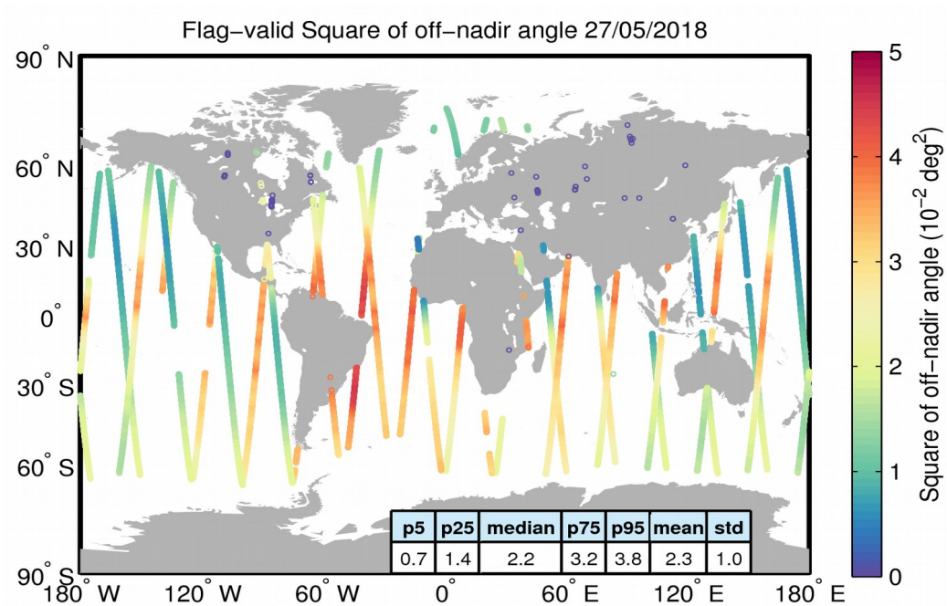
Figure 37. Geographical distribution of flag-valid mispointing data over oceans and lakes for 27/05/2018. The statistical values shown in the table refer to the mispointing in 10^{-2} \text{ deg}^2 and are calculated over all measurements shown in the figure.
