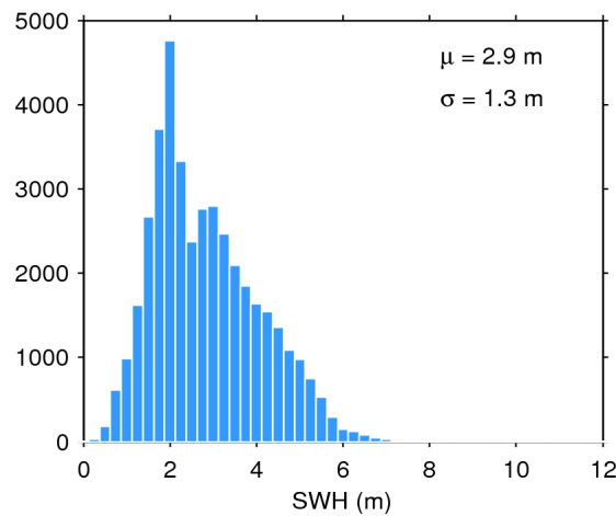
Figure 17. Histogram of flag-valid SWH over oceans and lakes for 27/05/2018. The mean ( \mu ) and standard deviation ( \sigma ) are also shown. Note that values larger than 12 m are excluded from the histogram for the sake of readability but not from the computation of \mu and \sigma .
