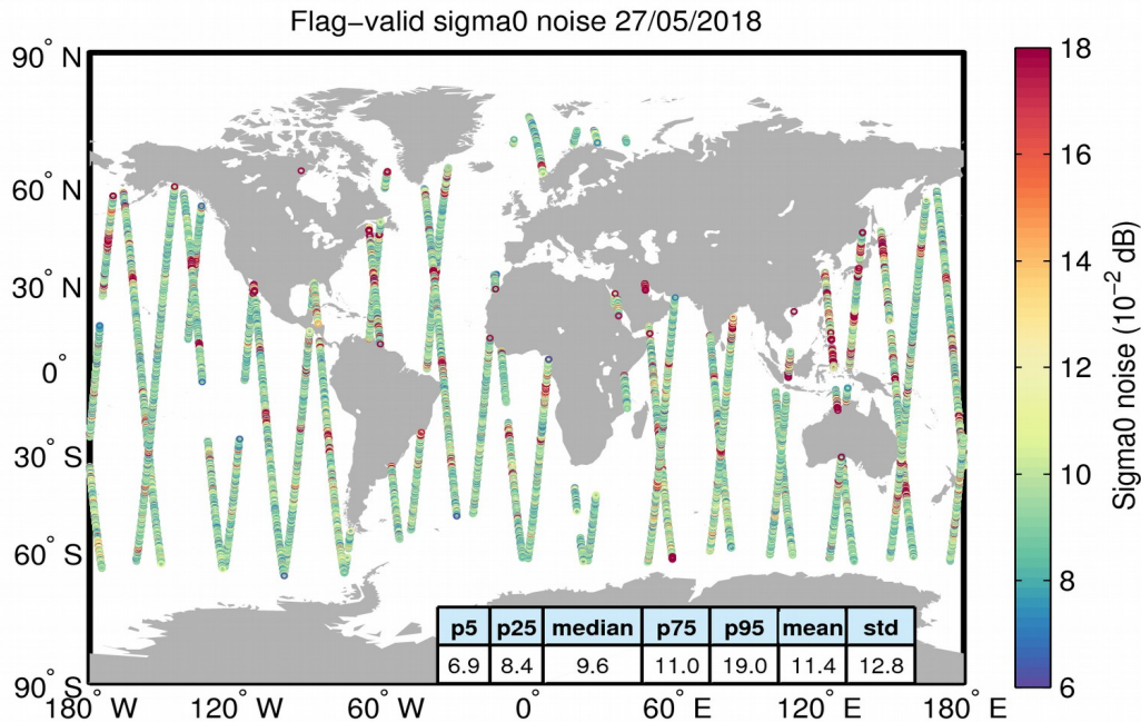
Figure 26. Geographical distribution of flag-valid 20-Hz sigma0 measurement noise over oceans and lakes for 27/05/2018. The statistical values shown in the table refer to the sigma0 noise and are calculated over all measurements shown in the figure.
