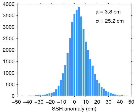
Figure 7. Histogram of flag-valid SSH anomaly over oceans and lakes for 27/05/2018. The mean ( \mu ) and standard deviation ( \sigma ) are also shown. Note that values outside [-50 50] cm are excluded from the histogram for the sake of readability but not from the computation of \mu and \sigma .
