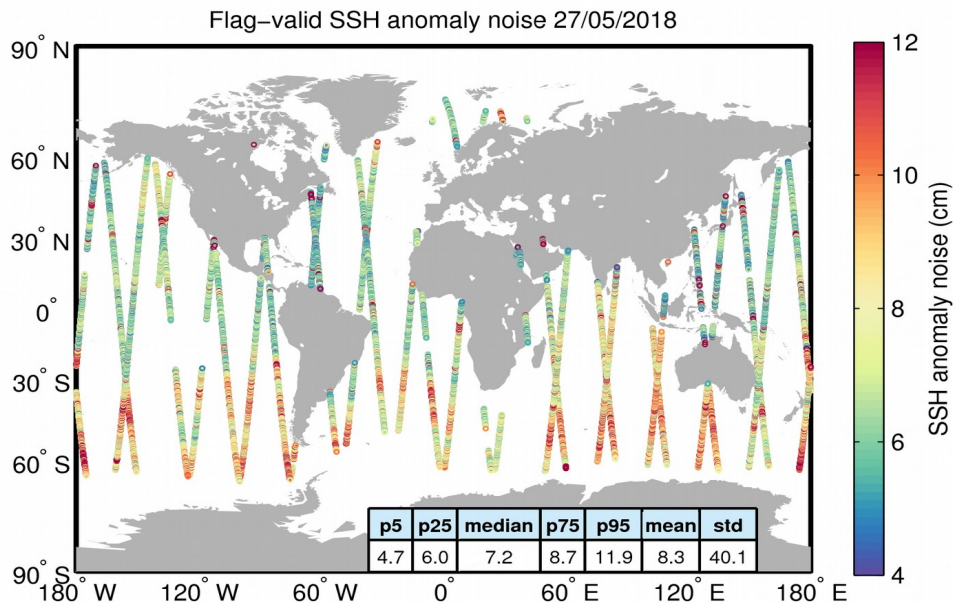
Figure 8. Geographical distribution of flag-valid 20-Hz SSH anomaly measurement noise over oceans and lakes for 27/05/2018. The statistical values shown in the table refer to the SSH anomaly noise and are calculated over all measurements shown in the figure.
