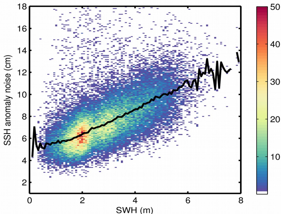
Figure 9. 2D histogram showing flag-valid SSH anomaly noise as a function of SWH for 27/05/2018. The black line denotes the median SSH anomaly noise as a function of SWH.
