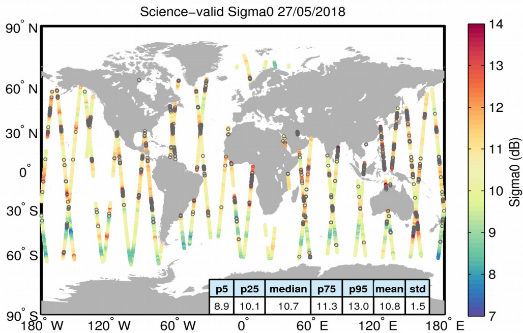
Figure 27. Geographical distribution of science-valid sigma0 data over oceans and lakes for 27/05/2018. The statistical values shown in the table refer to the sigma0 in dB and are calculated over all measurements shown in the figure. Gray circles denote records that have been rejected based on the editing criteria described in Table 4.
