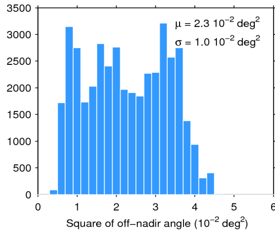
Figure 39. Histogram of flag-valid mispointing over oceans and lakes for 27/05/2018. The mean ( \mu ) and standard deviation ( \sigma ) are also shown. Note that values larger than 6 \cdot 10^{-2} \text{ deg}^2 are excluded from the histogram for the sake of readability but not from the computation of \mu and \sigma .
