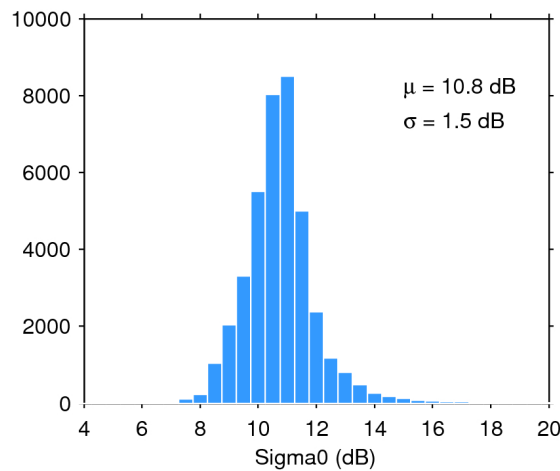
Figure 28. Histogram of science-valid sigma0 over oceans and lakes for 27/05/2018. The mean ( \mu ) and standard deviation ( \sigma ) are also shown. Note that values outside [4 20] dB are excluded from the histogram for the sake of readability but not from the computation of \mu and \sigma .
