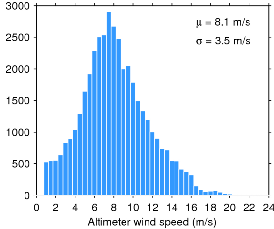
Figure 33. Histogram of flag-valid wind over oceans and lakes for 27/05/2018. The mean ( \mu ) and standard deviation ( \sigma ) are also shown. Note that values larger than 24 m/s are excluded from the histogram for the sake of readability but not from the computation of \mu and \sigma .
