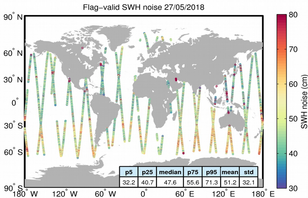
Figure 18. Geographical distribution of flag-valid 20-Hz SWH measurement noise over oceans and lakes for 27/05/2018. The statistical values shown in the figure refer to the SWH noise and are calculated over all measurements shown in the figure.
