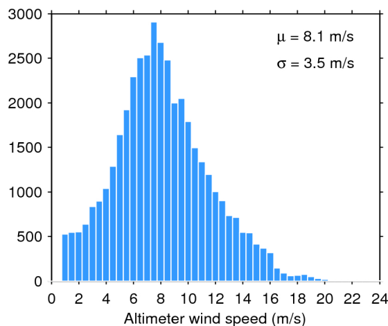
Figure 35. Histogram of science-valid wind over oceans and lakes for 27/05/2018. The mean ( \mu ) and standard deviation ( \sigma ) are also shown. Note that values larger than 24 m/s are excluded from the histogram for the sake of readability but not from the computation of \mu and \sigma .
