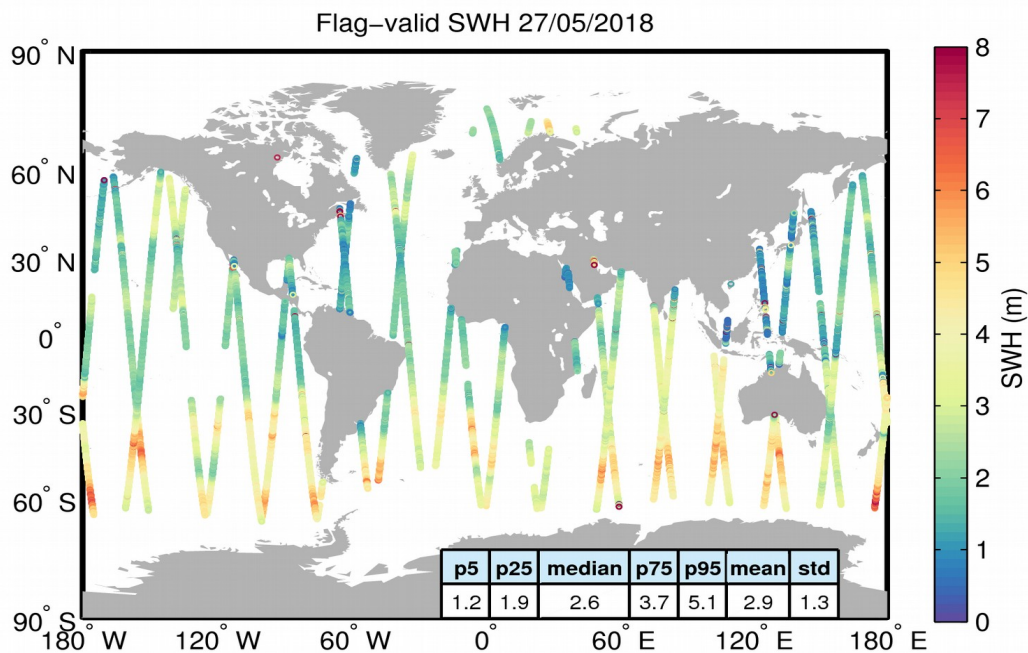
Figure 15. Geographical distribution of flag-valid SWH data over oceans and lakes for 27/05/2018. The statistical values shown in the table refer to the SWH in m and are calculated over all measurements shown in the figure.
