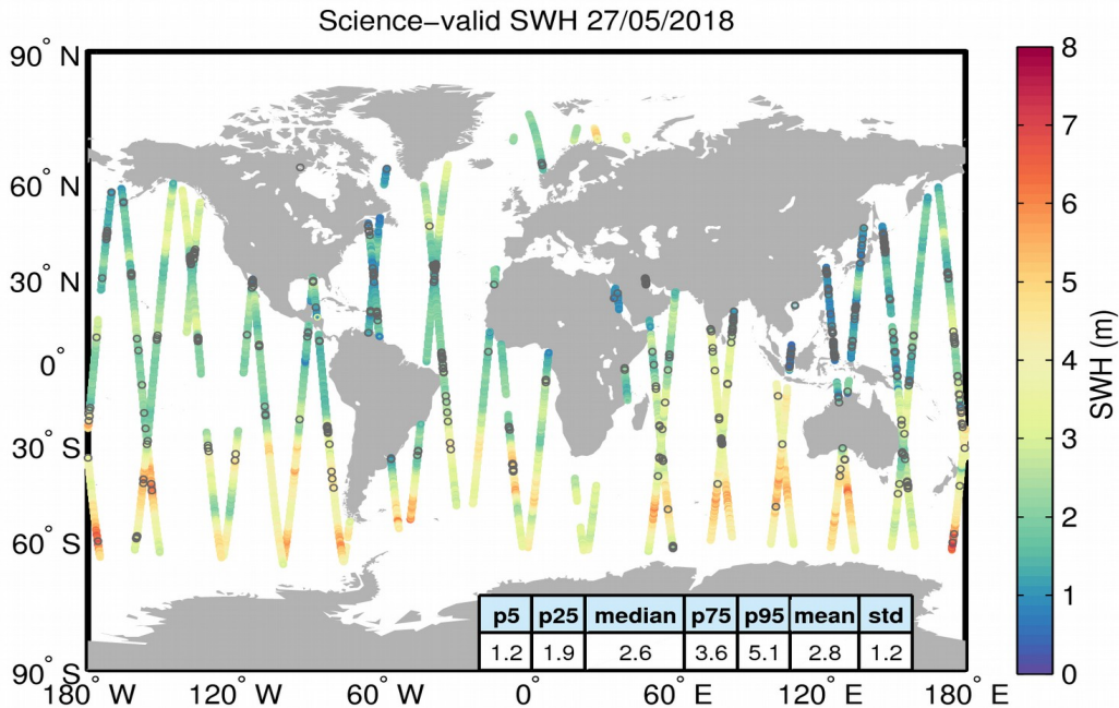
Figure 19. Geographical distribution of science-valid SWH data over oceans and lakes for 27/05/2018. The statistical values shown in the table refer to the SWH in m and are calculated over all measurements shown in the figure. Gray circles denote records that have been rejected based on the editing criteria described in Table 3.
