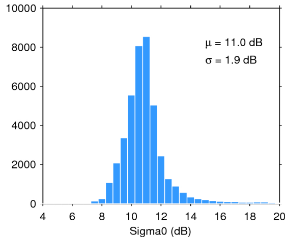
Figure 25. Histogram of flag-valid sigma0 over oceans and lakes for 27/05/2018. The mean ( \mu ) and standard deviation ( \sigma ) are also shown. Note that values outside [4 20] dB are excluded from the histogram for the sake of readability but not from the computation of \mu and \sigma .
