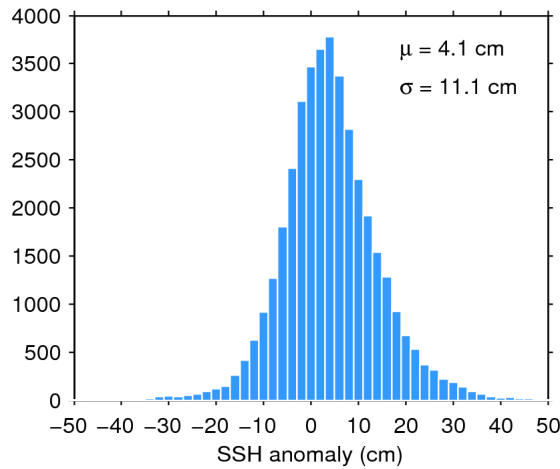
Figure 11. Histogram of science-valid SSH anomaly over oceans and lakes for 27/05/2018. The mean ( \mu ) and standard deviation ( \sigma ) are also shown. Note that values outside [-50 50] cm are excluded from the histogram for the sake of readability but not from the computation of \mu and \sigma .
