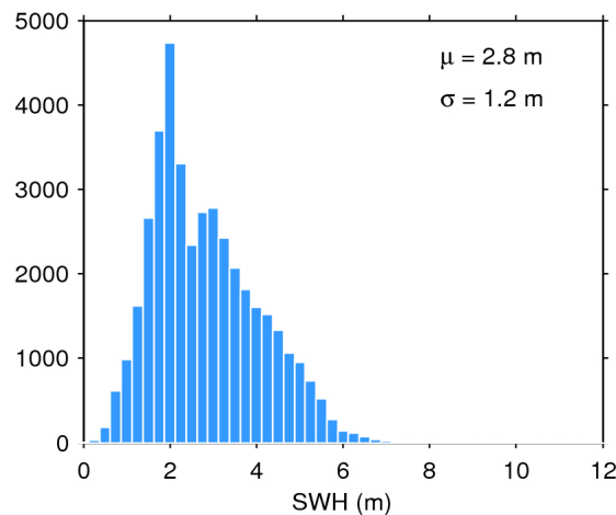
Figure 20. Histogram of science-valid SWH over oceans and lakes for 27/05/2018. The mean ( \mu ) and standard deviation ( \sigma ) are also shown. Note that values larger than 12 m are excluded from the histogram for the sake of readability but not from the computation of \mu and \sigma .
