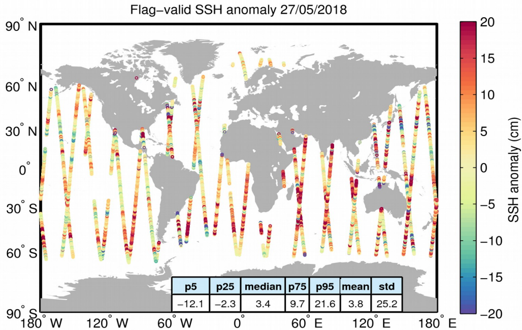
Figure 5. Geographical distribution of flag-valid 1-Hz SSH anomaly data over oceans and lakes for 27/05/2018. The statistical values shown in the table refer to the SSH anomaly in cm and are calculated over all measurements shown in the figure.
