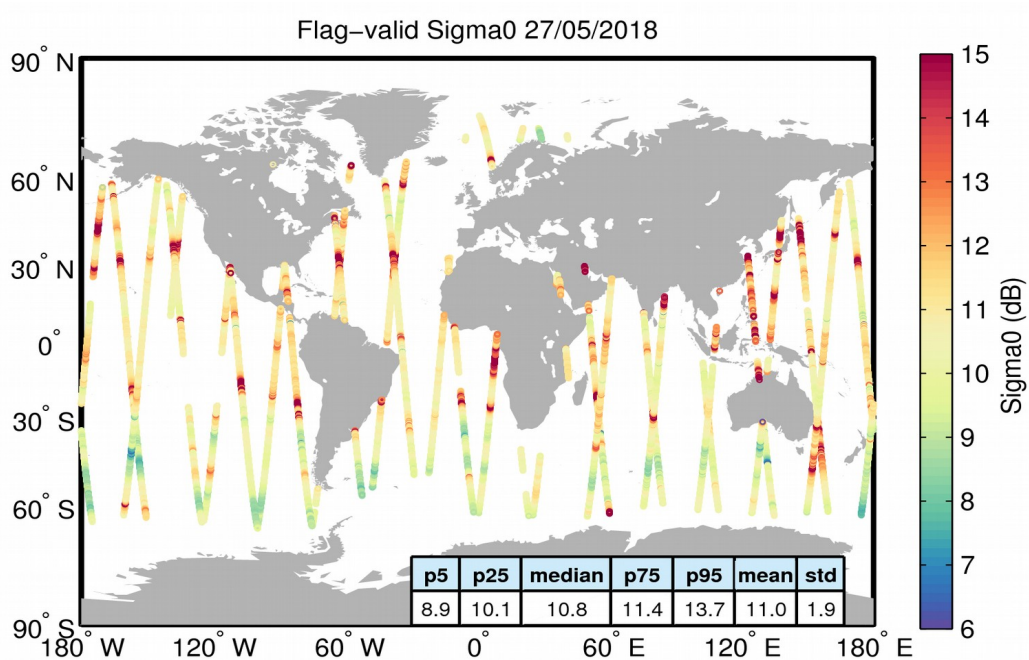
Figure 23. Geographical distribution of flag-valid sigma0 data over oceans and lakes for 27/05/2018. The statistical values shown in the table refer to the sigma0 in dB and are calculated over all measurements shown in the figure.
