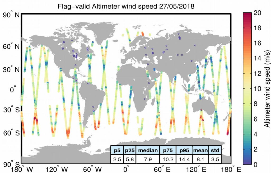
Figure 31. Geographical distribution of flag-valid wind data over oceans and lakes for 27/05/2018. The statistical values shown in the table refer to the wind in m/s and are calculated over all measurements shown in the figure.
