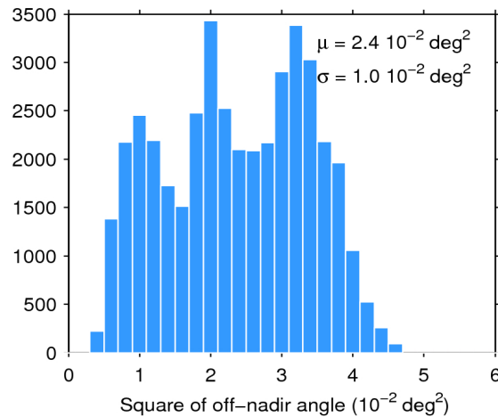
Figure 39. Histogram of flag-valid mispointing over oceans and lakes for 26/05/2018. The mean ( \mu ) and standard deviation ( \sigma ) are also shown. Note that values larger than 6 \cdot 10^{-2} \text{ deg}^2 are excluded from the histogram for the sake of readability but not from the computation of \mu and \sigma .
