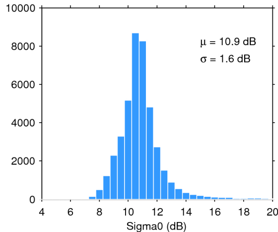
Figure 25. Histogram of flag-valid sigma0 over oceans and lakes for 26/05/2018. The mean ( \mu ) and standard deviation ( \sigma ) are also shown. Note that values outside [4 20] dB are excluded from the histogram for the sake of readability but not from the computation of \mu and \sigma .
