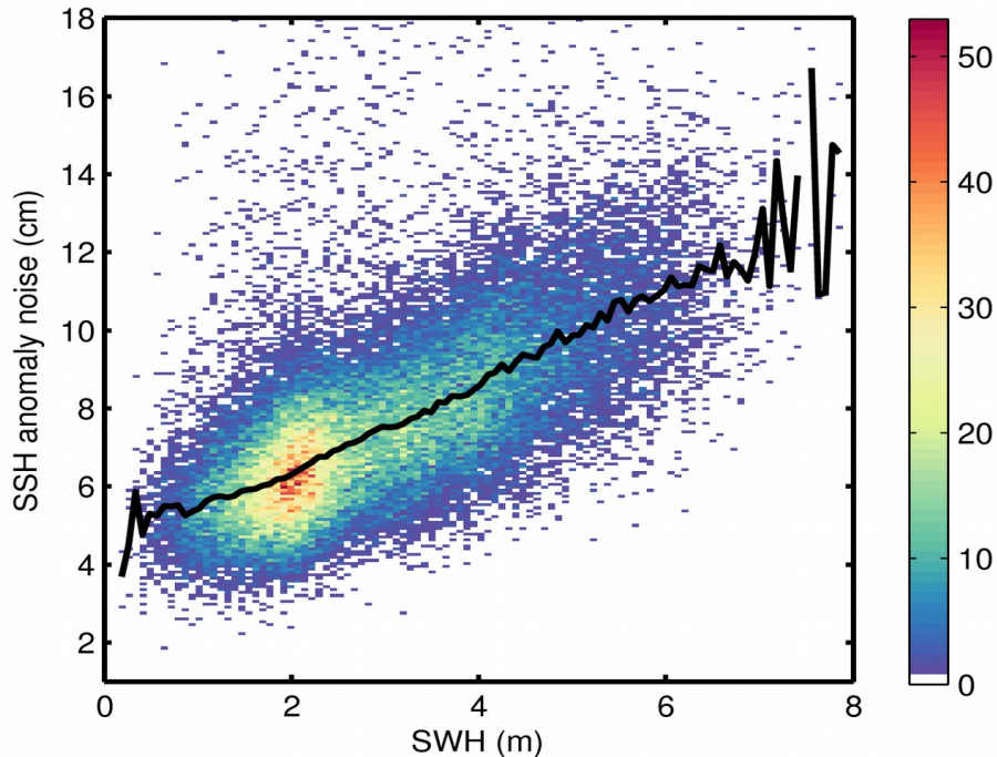
Figure 9. 2D histogram showing flag-valid SSH anomaly noise as a function of SWH for 26/05/2018. The black line denotes the median SSH anomaly noise as a function of SWH.
