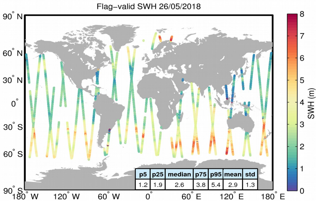
Figure 15. Geographical distribution of flag-valid SWH data over oceans and lakes for 26/05/2018. The statistical values shown in the table refer to the SWH in m and are calculated over all measurements shown in the figure.
