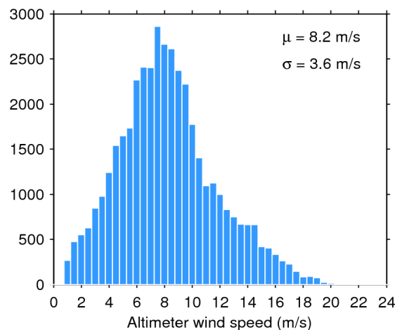
Figure 35. Histogram of science-valid wind over oceans and lakes for 26/05/2018. The mean ( \mu ) and standard deviation ( \sigma ) are also shown. Note that values larger than 24 m/s are excluded from the histogram for the sake of readability but not from the computation of \mu and \sigma .
