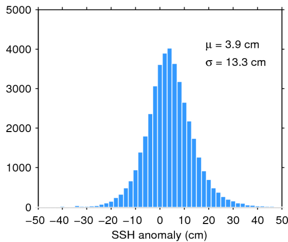
Figure 7. Histogram of flag-valid SSH anomaly over oceans and lakes for 26/05/2018. The mean ( \mu ) and standard deviation ( \sigma ) are also shown. Note that values outside [-50 50] cm are excluded from the histogram for the sake of readability but not from the computation of \mu and \sigma .
