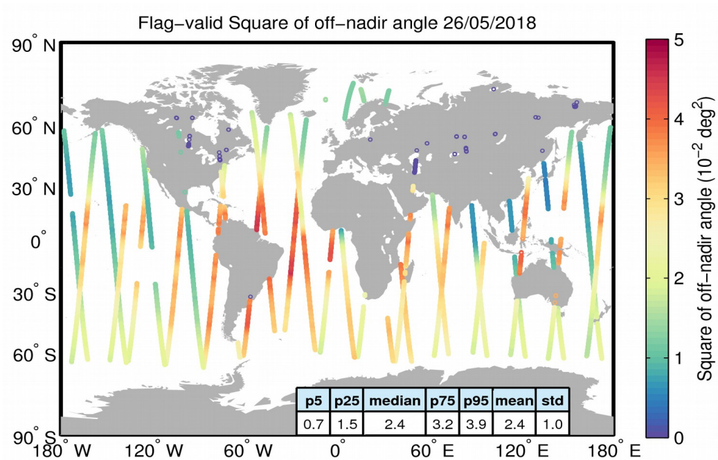
Figure 37. Geographical distribution of flag-valid mispointing data over oceans and lakes for 26/05/2018. The statistical values shown in the table refer to the mispointing in 10^{-2} \text{ deg}^2 and are calculated over all measurements shown in the figure.
