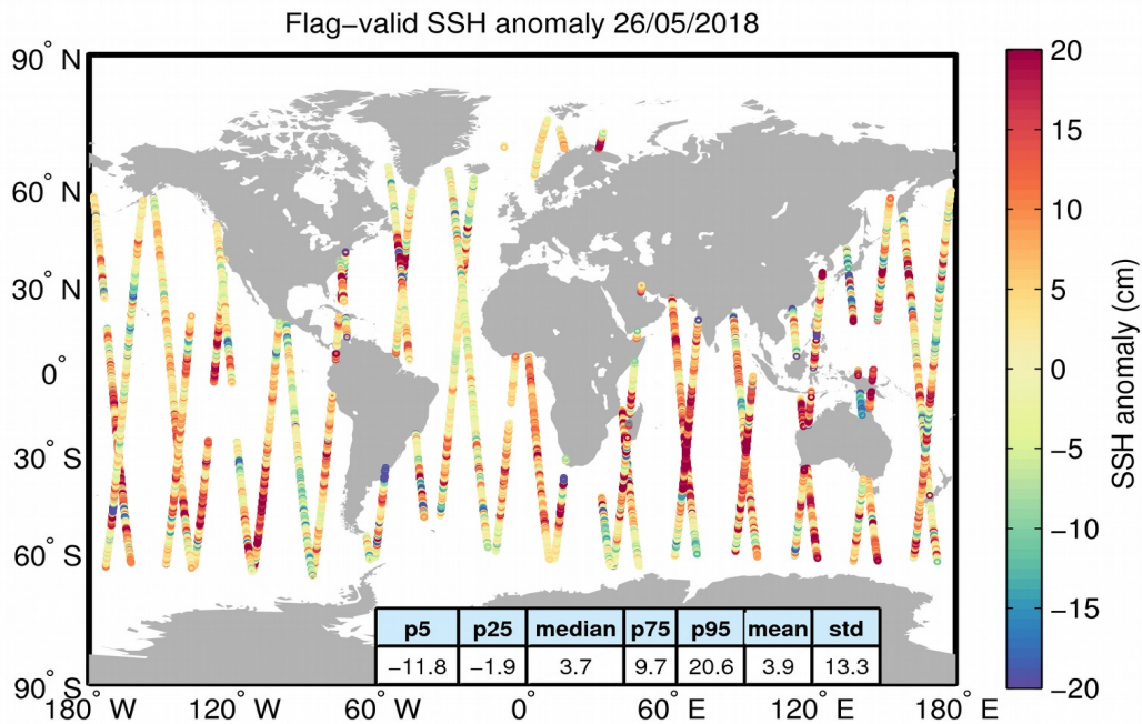
Figure 5. Geographical distribution of flag-valid 1-Hz SSH anomaly data over oceans and lakes for 26/05/2018. The statistical values shown in the table refer to the SSH anomaly in cm and are calculated over all measurements shown in the figure.
