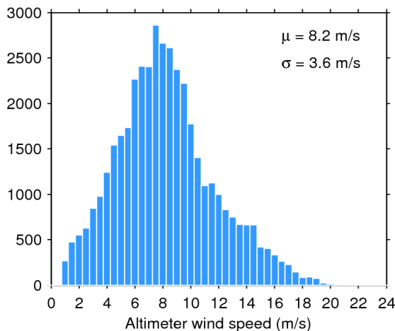
Figure 33. Histogram of flag-valid wind over oceans and lakes for 26/05/2018. The mean ( \mu ) and standard deviation ( \sigma ) are also shown. Note that values larger than 24 m/s are excluded from the histogram for the sake of readability but not from the computation of \mu and \sigma .
