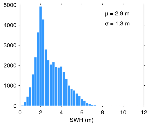
Figure 20. Histogram of science-valid SWH over oceans and lakes for 26/05/2018. The mean ( \mu ) and standard deviation ( \sigma ) are also shown. Note that values larger than 12 m are excluded from the histogram for the sake of readability but not from the computation of \mu and \sigma .
