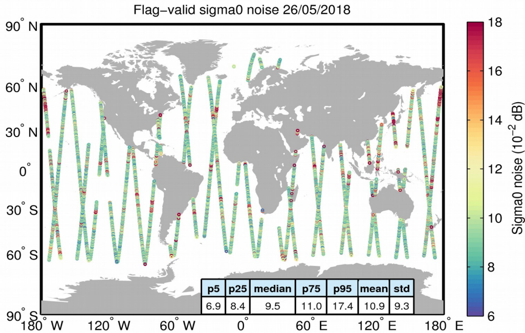
Figure 26. Geographical distribution of flag-valid 20-Hz sigma0 measurement noise over oceans and lakes for 26/05/2018. The statistical values shown in the table refer to the sigma0 noise and are calculated over all measurements shown in the figure.
