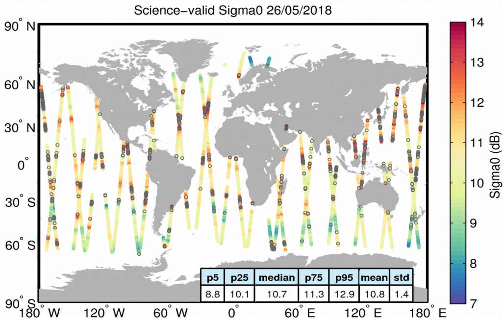
Figure 27. Geographical distribution of science-valid sigma0 data over oceans and lakes for 26/05/2018. The statistical values shown in the table refer to the sigma0 in dB and are calculated over all measurements shown in the figure. Gray circles denote records that have been rejected based on the editing criteria described in Table 4.
