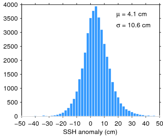
Figure 11. Histogram of science-valid SSH anomaly over oceans and lakes for 26/05/2018. The mean ( \mu ) and standard deviation ( \sigma ) are also shown. Note that values outside [-50 50] cm are excluded from the histogram for the sake of readability but not from the computation of \mu and \sigma .
