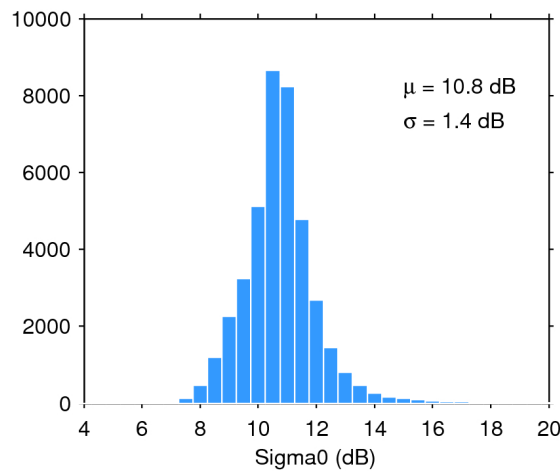
Figure 28. Histogram of science-valid sigma0 over oceans and lakes for 26/05/2018. The mean ( \mu ) and standard deviation ( \sigma ) are also shown. Note that values outside [4 20] dB are excluded from the histogram for the sake of readability but not from the computation of \mu and \sigma .
