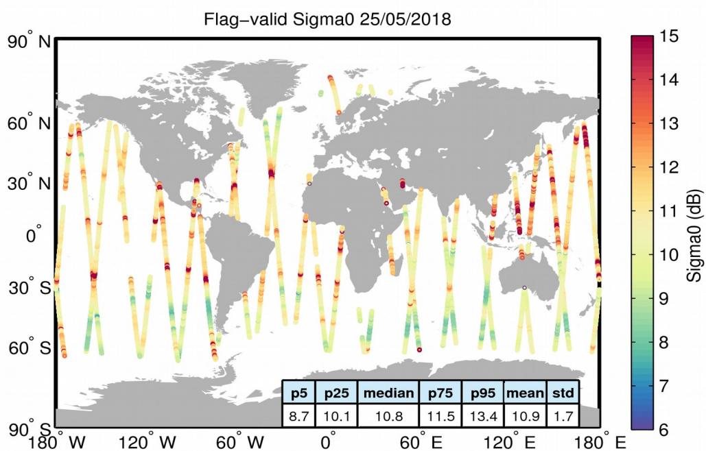
Figure 23. Geographical distribution of flag-valid sigma0 data over oceans and lakes for 25/05/2018. The statistical values shown in the table refer to the sigma0 in dB and are calculated over all measurements shown in the figure.
