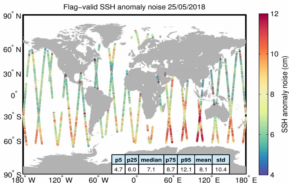
Figure 8. Geographical distribution of flag-valid 20-Hz SSH anomaly measurement noise over oceans and lakes for 25/05/2018. The statistical values shown in the table refer to the SSH anomaly noise and are calculated over all measurements shown in the figure.
