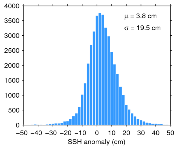
Figure 7. Histogram of flag-valid SSH anomaly over oceans and lakes for 25/05/2018. The mean ( \mu ) and standard deviation ( \sigma ) are also shown. Note that values outside [-50\ 50] cm are excluded from the histogram for the sake of readability but not from the computation of \mu and \sigma .
