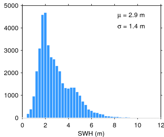
Figure 17. Histogram of flag-valid SWH over oceans and lakes for 25/05/2018. The mean ( \mu ) and standard deviation ( \sigma ) are also shown. Note that values larger than 12 m are excluded from the histogram for the sake of readability but not from the computation of \mu and \sigma .
