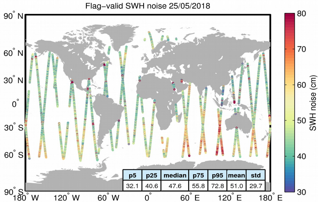
Figure 18. Geographical distribution of flag-valid 20-Hz SWH measurement noise over oceans and lakes for 25/05/2018. The statistical values shown in the figure refer to the SWH noise and are calculated over all measurements shown in the figure.
