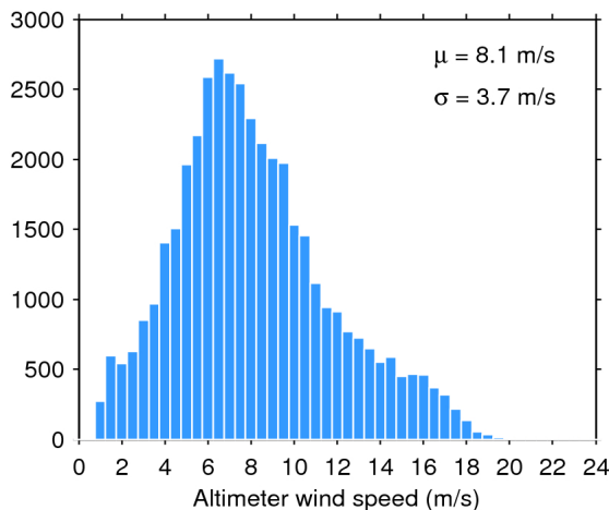
Figure 33. Histogram of flag-valid wind over oceans and lakes for 25/05/2018. The mean ( \mu ) and standard deviation ( \sigma ) are also shown. Note that values larger than 24 m/s are excluded from the histogram for the sake of readability but not from the computation of \mu and \sigma .
