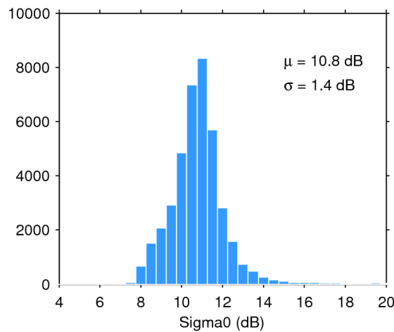
Figure 28. Histogram of science-valid sigma0 over oceans and lakes for 25/05/2018. The mean ( \mu ) and standard deviation ( \sigma ) are also shown. Note that values outside [4 20] dB are excluded from the histogram for the sake of readability but not from the computation of \mu and \sigma .
