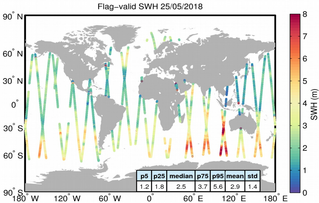
Figure 15. Geographical distribution of flag-valid SWH data over oceans and lakes for 25/05/2018. The statistical values shown in the table refer to the SWH in m and are calculated over all measurements shown in the figure.
