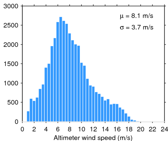
Figure 35. Histogram of science-valid wind over oceans and lakes for 25/05/2018. The mean ( \mu ) and standard deviation ( \sigma ) are also shown. Note that values larger than 24 m/s are excluded from the histogram for the sake of readability but not from the computation of \mu and \sigma .
