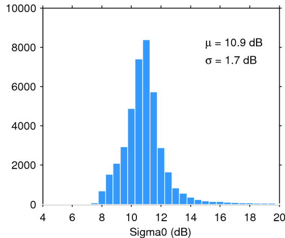
Figure 25. Histogram of flag-valid sigma0 over oceans and lakes for 25/05/2018. The mean ( \mu ) and standard deviation ( \sigma ) are also shown. Note that values outside [4 20] dB are excluded from the histogram for the sake of readability but not from the computation of \mu and \sigma .
