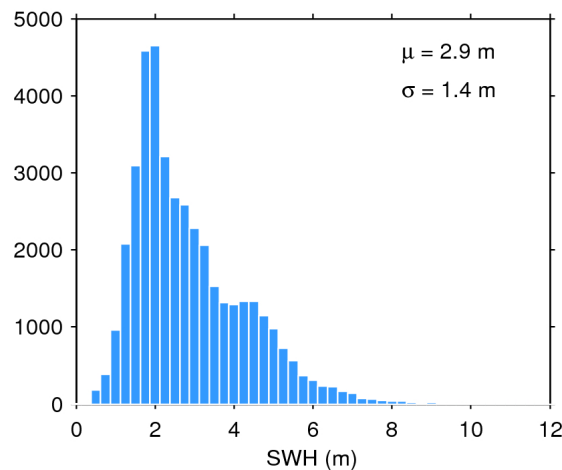
Figure 20. Histogram of science-valid SWH over oceans and lakes for 25/05/2018. The mean ( \mu ) and standard deviation ( \sigma ) are also shown. Note that values larger than 12 m are excluded from the histogram for the sake of readability but not from the computation of \mu and \sigma .
