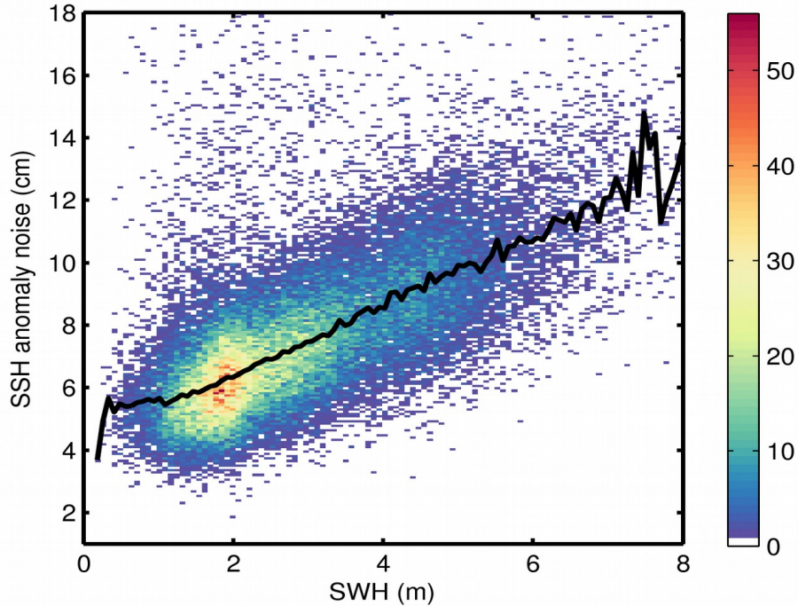
Figure 9. 2D histogram showing flag-valid SSH anomaly noise as a function of SWH for 25/05/2018. The black line denotes the median SSH anomaly noise as a function of SWH.
