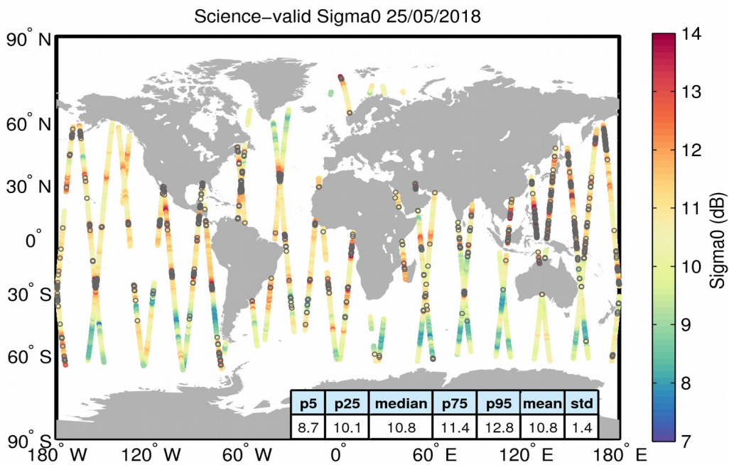
Figure 27. Geographical distribution of science-valid sigma0 data over oceans and lakes for 25/05/2018. The statistical values shown in the table refer to the sigma0 in dB and are calculated over all measurements shown in the figure. Gray circles denote records that have been rejected based on the editing criteria described in Table 4.
