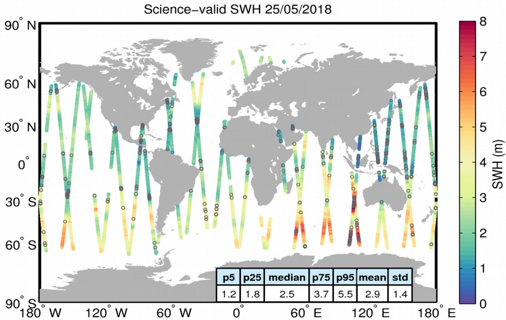
Figure 19. Geographical distribution of science-valid SWH data over oceans and lakes for 25/05/2018. The statistical values shown in the table refer to the SWH in m and are calculated over all measurements shown in the figure. Gray circles denote records that have been rejected based on the editing criteria described in Table 3.
