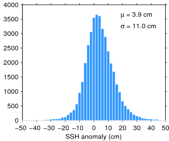
Figure 11. Histogram of science-valid SSH anomaly over oceans and lakes for 25/05/2018. The mean ( \mu ) and standard deviation ( \sigma ) are also shown. Note that values outside [-50 50] cm are excluded from the histogram for the sake of readability but not from the computation of \mu and \sigma .
