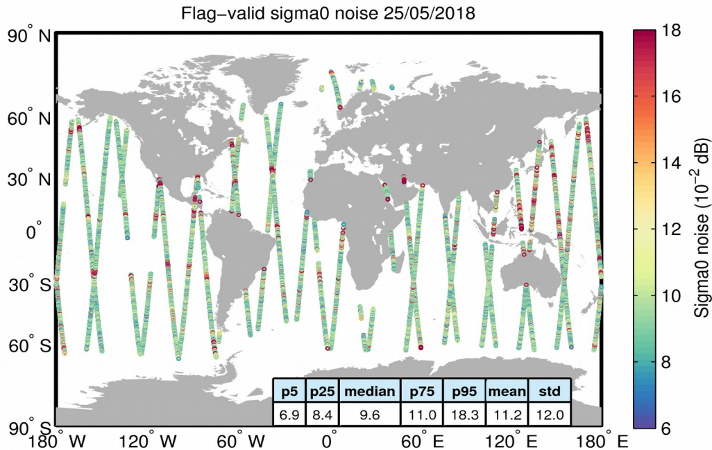
Figure 26. Geographical distribution of flag-valid 20-Hz sigma0 measurement noise over oceans and lakes for 25/05/2018. The statistical values shown in the table refer to the sigma0 noise and are calculated over all measurements shown in the figure.
