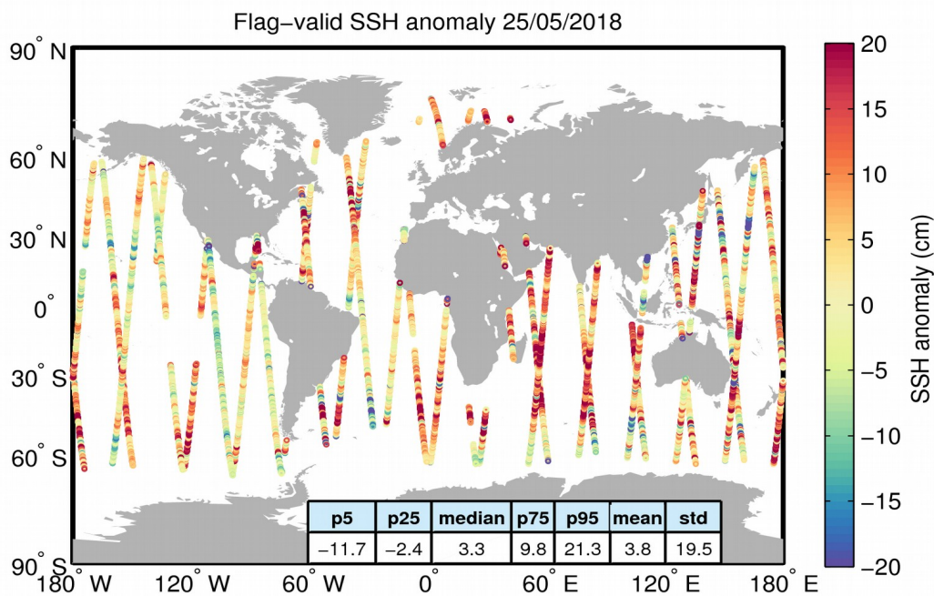
Figure 5. Geographical distribution of flag-valid 1-Hz SSH anomaly data over oceans and lakes for 25/05/2018. The statistical values shown in the table refer to the SSH anomaly in cm and are calculated over all measurements shown in the figure.
