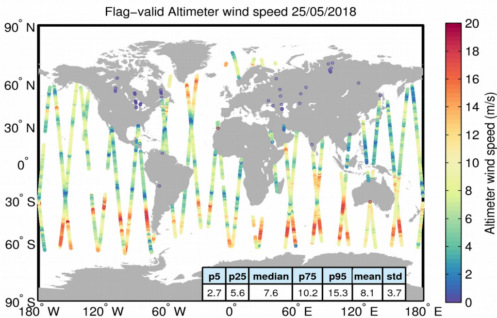
Figure 31. Geographical distribution of flag-valid wind data over oceans and lakes for 25/05/2018. The statistical values shown in the table refer to the wind in m/s and are calculated over all measurements shown in the figure.
