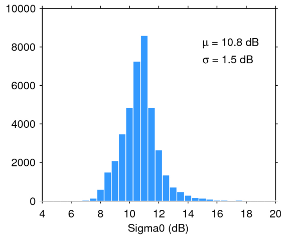
Figure 28. Histogram of science-valid sigma0 over oceans and lakes for 24/05/2018. The mean ( \mu ) and standard deviation ( \sigma ) are also shown. Note that values outside [4 20] dB are excluded from the histogram for the sake of readability but not from the computation of \mu and \sigma .
