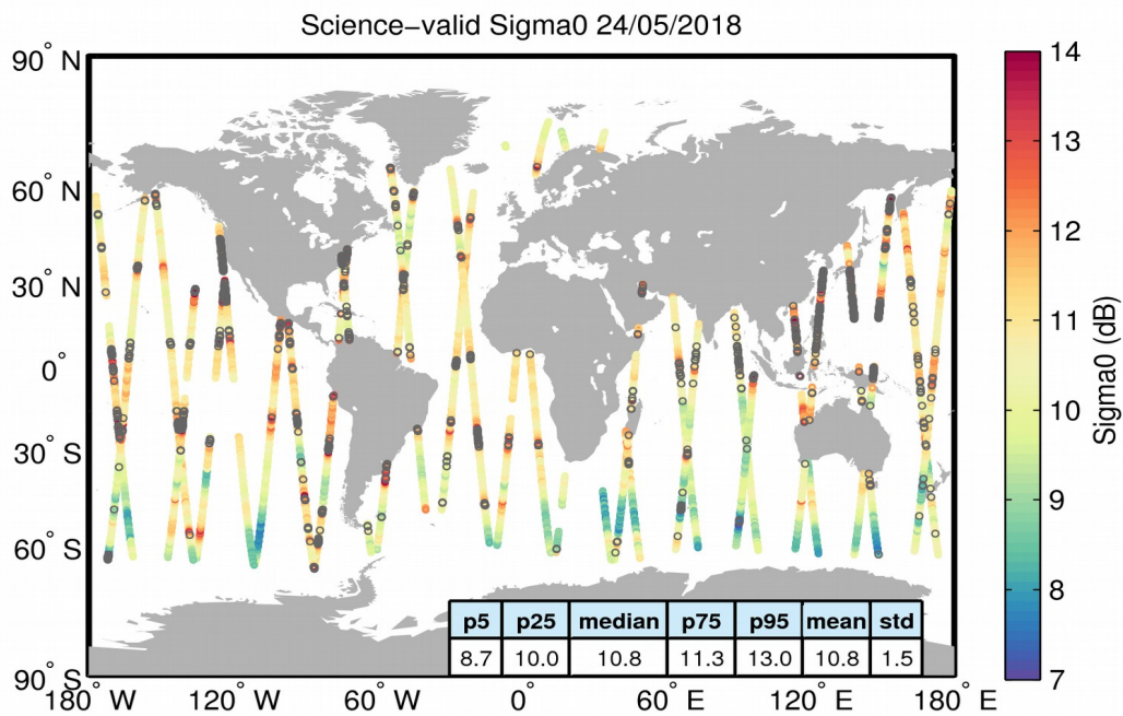
Figure 27. Geographical distribution of science-valid sigma0 data over oceans and lakes for 24/05/2018. The statistical values shown in the table refer to the sigma0 in dB and are calculated over all measurements shown in the figure. Gray circles denote records that have been rejected based on the editing criteria described in Table 4.
