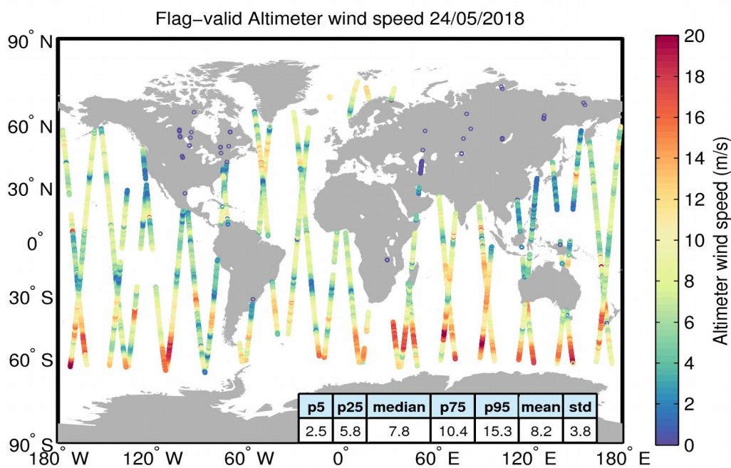
Figure 31. Geographical distribution of flag-valid wind data over oceans and lakes for 24/05/2018. The statistical values shown in the table refer to the wind in m/s and are calculated over all measurements shown in the figure.
