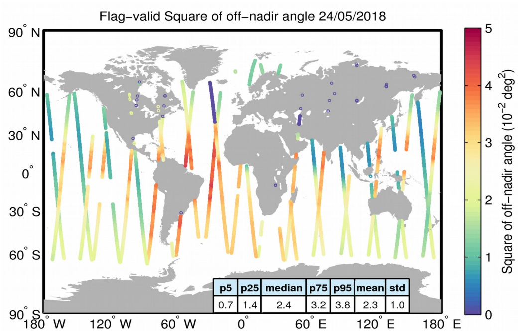
Figure 37. Geographical distribution of flag-valid mispointing data over oceans and lakes for 24/05/2018. The statistical values shown in the table refer to the mispointing in 10^{-2} \text{ deg}^2 and are calculated over all measurements shown in the figure.
