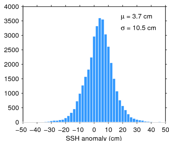
Figure 11. Histogram of science-valid SSH anomaly over oceans and lakes for 24/05/2018. The mean ( \mu ) and standard deviation ( \sigma ) are also shown. Note that values outside [-50 50] cm are excluded from the histogram for the sake of readability but not from the computation of \mu and \sigma .
