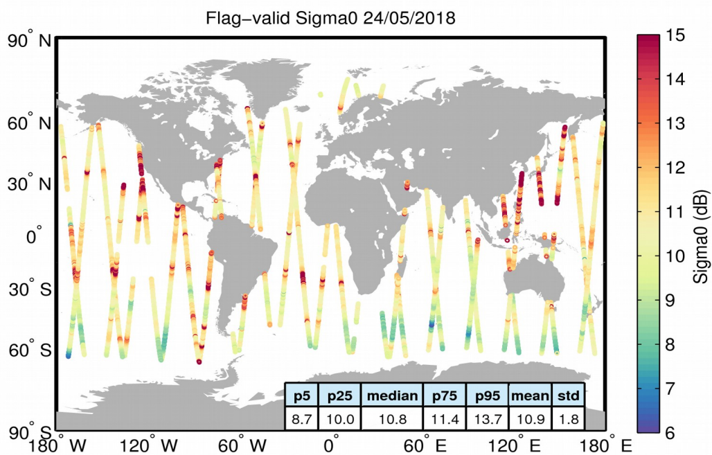
Figure 23. Geographical distribution of flag-valid sigma0 data over oceans and lakes for 24/05/2018. The statistical values shown in the table refer to the sigma0 in dB and are calculated over all measurements shown in the figure.
