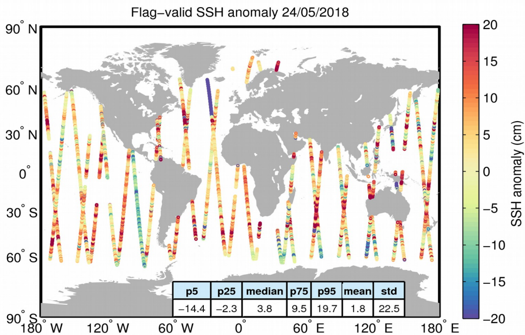
Figure 5. Geographical distribution of flag-valid 1-Hz SSH anomaly data over oceans and lakes for 24/05/2018. The statistical values shown in the table refer to the SSH anomaly in cm and are calculated over all measurements shown in the figure.
