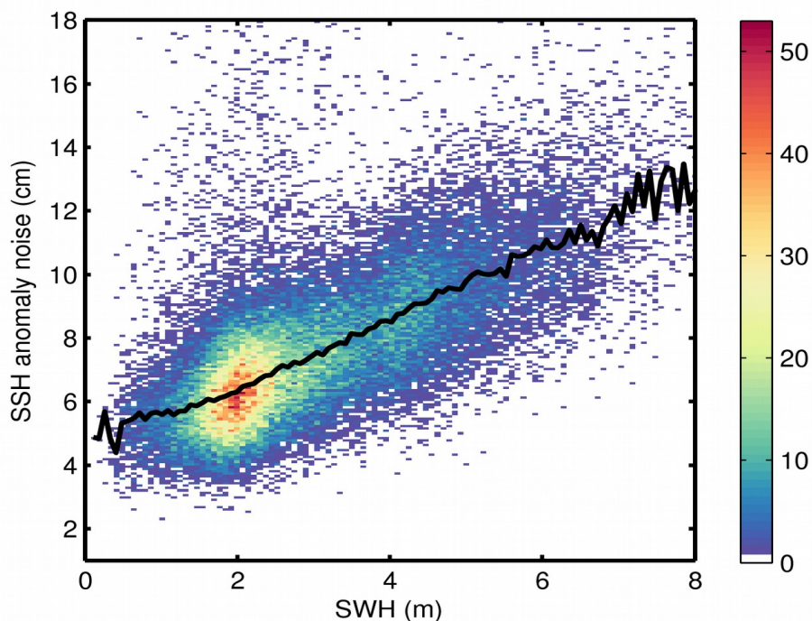
Figure 9. 2D histogram showing flag-valid SSH anomaly noise as a function of SWH for 24/05/2018. The black line denotes the median SSH anomaly noise as a function of SWH.
