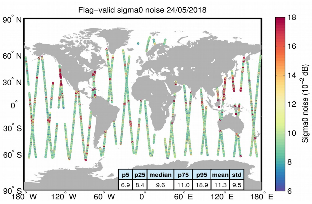
Figure 26. Geographical distribution of flag-valid 20-Hz sigma0 measurement noise over oceans and lakes for 24/05/2018. The statistical values shown in the table refer to the sigma0 noise and are calculated over all measurements shown in the figure.
