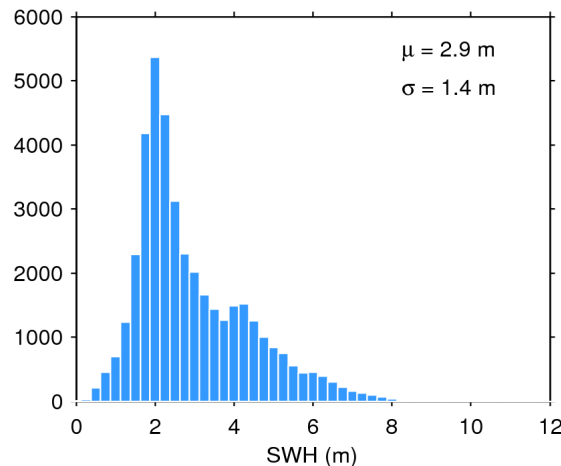
Figure 20. Histogram of science-valid SWH over oceans and lakes for 24/05/2018. The mean ( \mu ) and standard deviation ( \sigma ) are also shown. Note that values larger than 12 m are excluded from the histogram for the sake of readability but not from the computation of \mu and \sigma .
