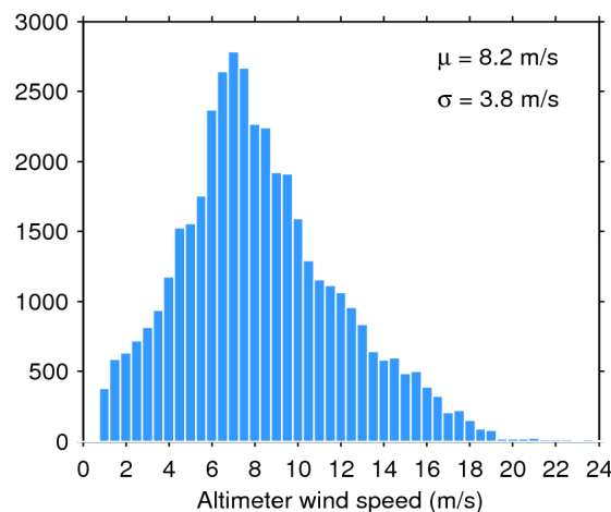
Figure 35. Histogram of science-valid wind over oceans and lakes for 24/05/2018. The mean ( \mu ) and standard deviation ( \sigma ) are also shown. Note that values larger than 24 m/s are excluded from the histogram for the sake of readability but not from the computation of \mu and \sigma .
