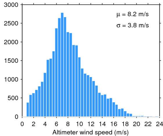
Figure 33. Histogram of flag-valid wind over oceans and lakes for 24/05/2018. The mean ( \mu ) and standard deviation ( \sigma ) are also shown. Note that values larger than 24 m/s are excluded from the histogram for the sake of readability but not from the computation of \mu and \sigma .
