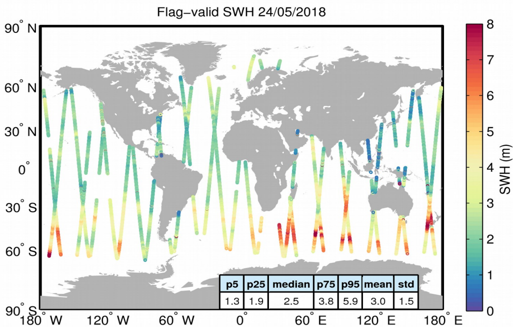
Figure 15. Geographical distribution of flag-valid SWH data over oceans and lakes for 24/05/2018. The statistical values shown in the table refer to the SWH in m and are calculated over all measurements shown in the figure.
