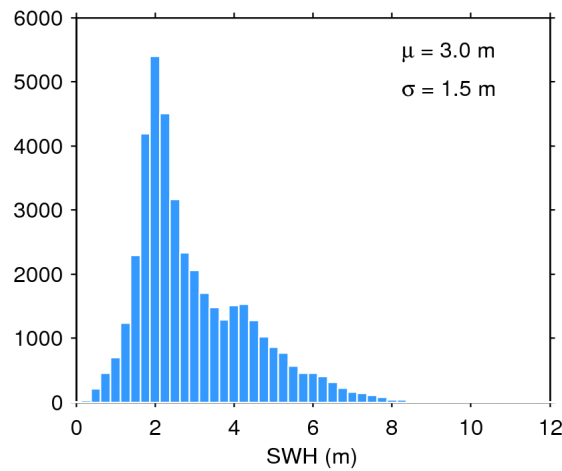
Figure 17. Histogram of flag-valid SWH over oceans and lakes for 24/05/2018. The mean ( \mu ) and standard deviation ( \sigma ) are also shown. Note that values larger than 12 m are excluded from the histogram for the sake of readability but not from the computation of \mu and \sigma .
