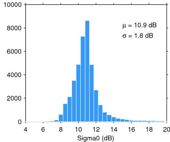
Figure 25. Histogram of flag-valid sigma0 over oceans and lakes for 24/05/2018. The mean ( \mu ) and standard deviation ( \sigma ) are also shown. Note that values outside [4 20] dB are excluded from the histogram for the sake of readability but not from the computation of \mu and \sigma .
