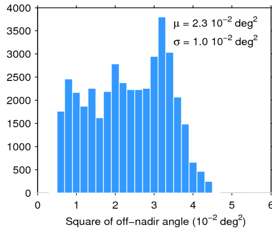
Figure 39. Histogram of flag-valid mispointing over oceans and lakes for 24/05/2018. The mean ( \mu ) and standard deviation ( \sigma ) are also shown. Note that values larger than 6 \cdot 10^{-2} \text{ deg}^2 are excluded from the histogram for the sake of readability but not from the computation of \mu and \sigma .
