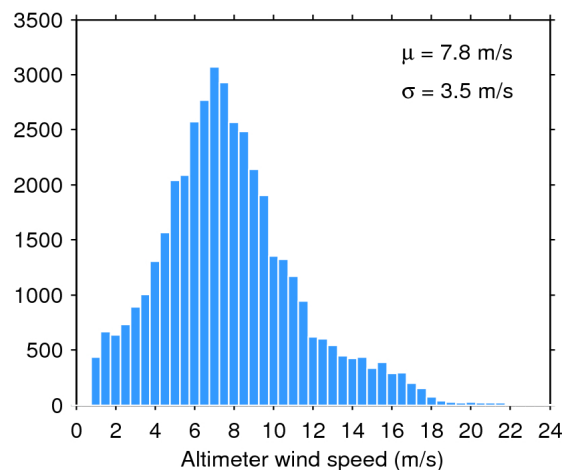
Figure 35. Histogram of science-valid wind over oceans and lakes for 23/05/2018. The mean ( \mu ) and standard deviation ( \sigma ) are also shown. Note that values larger than 24 m/s are excluded from the histogram for the sake of readability but not from the computation of \mu and \sigma .
