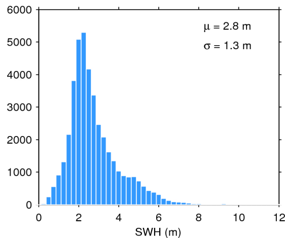
Figure 17. Histogram of flag-valid SWH over oceans and lakes for 23/05/2018. The mean ( \mu ) and standard deviation ( \sigma ) are also shown. Note that values larger than 12 m are excluded from the histogram for the sake of readability but not from the computation of \mu and \sigma .
