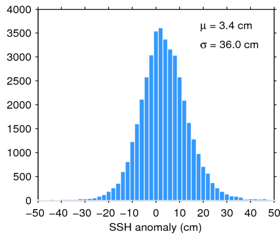
Figure 7. Histogram of flag-valid SSH anomaly over oceans and lakes for 23/05/2018. The mean ( \mu ) and standard deviation ( \sigma ) are also shown. Note that values outside [-50 50] cm are excluded from the histogram for the sake of readability but not from the computation of \mu and \sigma .
