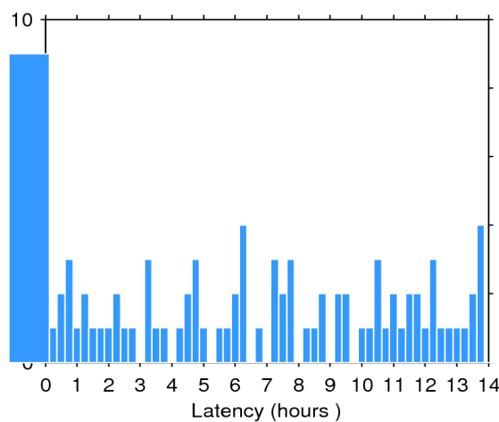
Figure 2. Histogram of the data latency for 23/05/2018. The y-axis denotes the number of files that are made available with a delay of x-hours with respect to the mean time of the records stored in the file.
