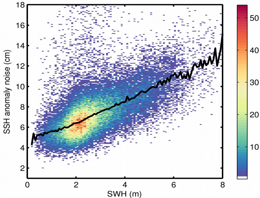
Figure 9. 2D histogram showing flag-valid SSH anomaly noise as a function of SWH for 23/05/2018. The black line denotes the median SSH anomaly noise as a function of SWH.
