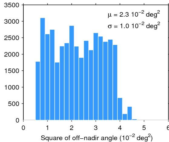
Figure 39. Histogram of flag-valid mispointing over oceans and lakes for 23/05/2018. The mean ( \mu ) and standard deviation ( \sigma ) are also shown. Note that values larger than 6 \cdot 10^{-2} \text{ deg}^2 are excluded from the histogram for the sake of readability but not from the computation of \mu and \sigma .
