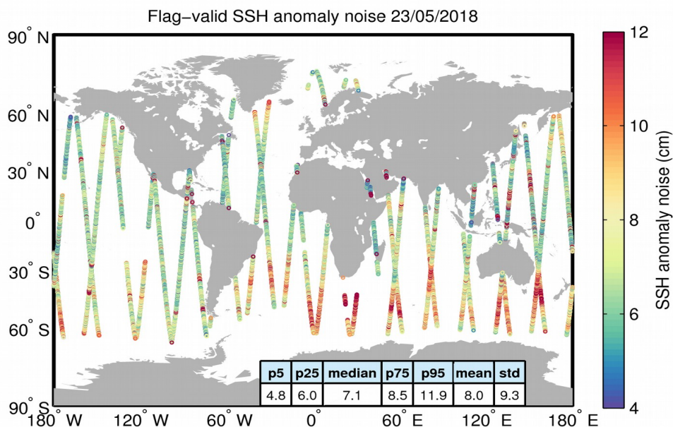
Figure 8. Geographical distribution of flag-valid 20-Hz SSH anomaly measurement noise over oceans and lakes for 23/05/2018. The statistical values shown in the table refer to the SSH anomaly noise and are calculated over all measurements shown in the figure.
