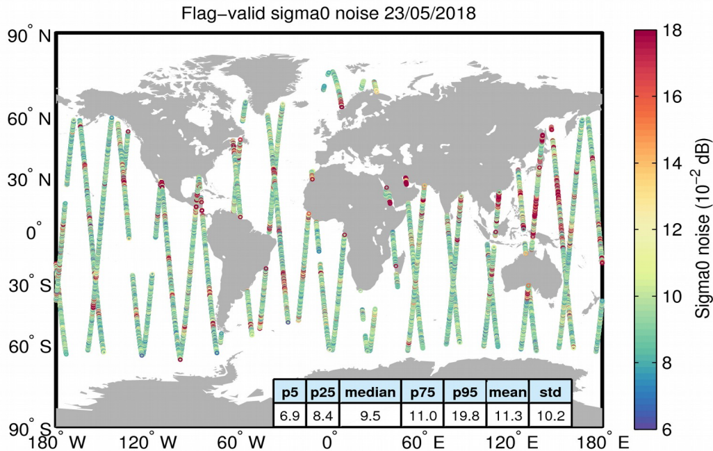
Figure 26. Geographical distribution of flag-valid 20-Hz sigma0 measurement noise over oceans and lakes for 23/05/2018. The statistical values shown in the table refer to the sigma0 noise and are calculated over all measurements shown in the figure.
