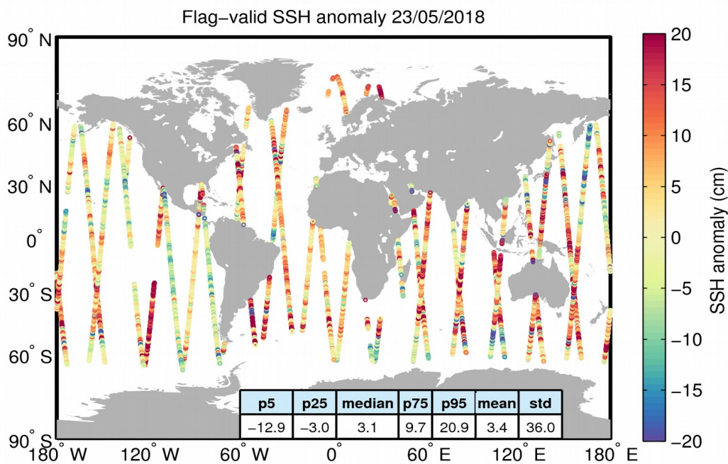
Figure 5. Geographical distribution of flag-valid 1-Hz SSH anomaly data over oceans and lakes for 23/05/2018. The statistical values shown in the table refer to the SSH anomaly in cm and are calculated over all measurements shown in the figure.
