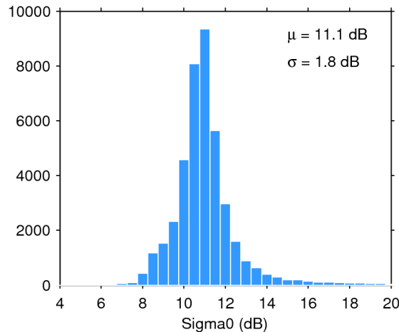
Figure 25. Histogram of flag-valid sigma0 over oceans and lakes for 23/05/2018. The mean ( \mu ) and standard deviation ( \sigma ) are also shown. Note that values outside [4 20] dB are excluded from the histogram for the sake of readability but not from the computation of \mu and \sigma .
