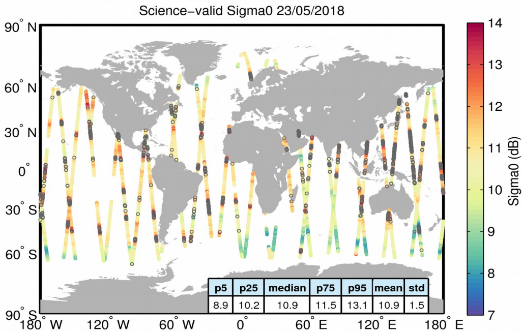
Figure 27. Geographical distribution of science-valid sigma0 data over oceans and lakes for 23/05/2018. The statistical values shown in the table refer to the sigma0 in dB and are calculated over all measurements shown in the figure. Gray circles denote records that have been rejected based on the editing criteria described in Table 4.
