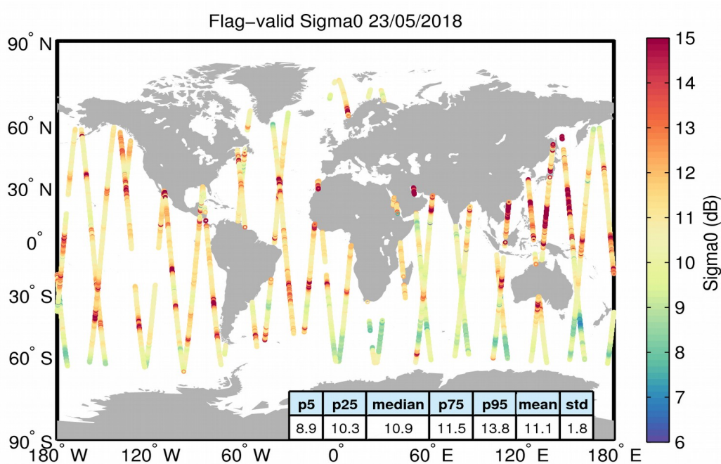
Figure 23. Geographical distribution of flag-valid sigma0 data over oceans and lakes for 23/05/2018. The statistical values shown in the table refer to the sigma0 in dB and are calculated over all measurements shown in the figure.
