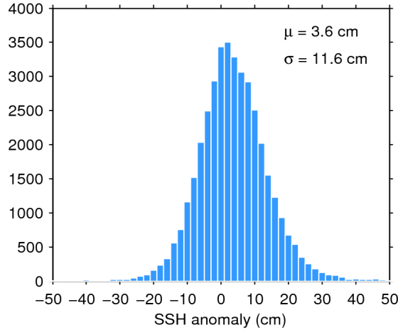
Figure 11. Histogram of science-valid SSH anomaly over oceans and lakes for 23/05/2018. The mean ( \mu ) and standard deviation ( \sigma ) are also shown. Note that values outside [-50 50] cm are excluded from the histogram for the sake of readability but not from the computation of \mu and \sigma .
