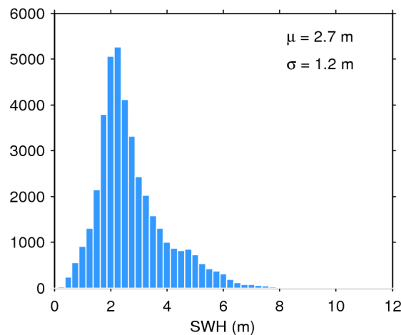
Figure 20. Histogram of science-valid SWH over oceans and lakes for 23/05/2018. The mean ( \mu ) and standard deviation ( \sigma ) are also shown. Note that values larger than 12 m are excluded from the histogram for the sake of readability but not from the computation of \mu and \sigma .
