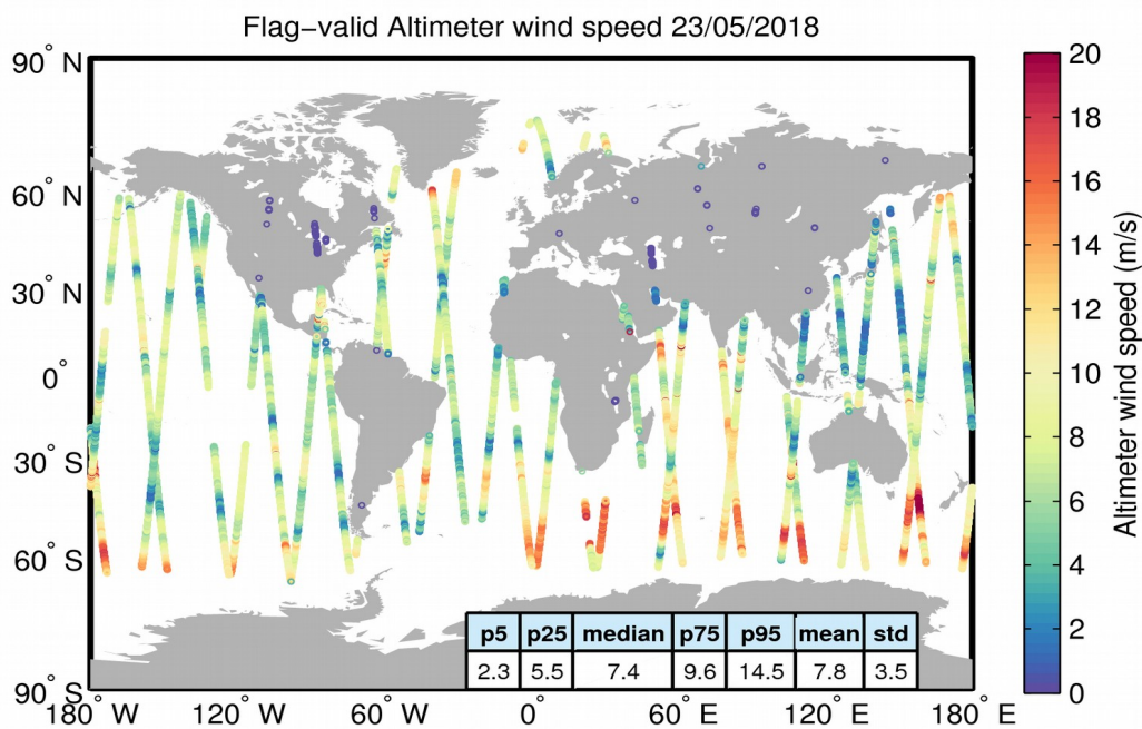
Figure 31. Geographical distribution of flag-valid wind data over oceans and lakes for 23/05/2018. The statistical values shown in the table refer to the wind in m/s and are calculated over all measurements shown in the figure.
