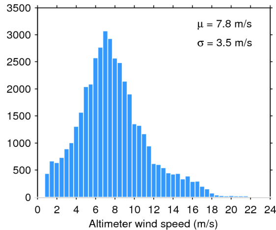
Figure 33. Histogram of flag-valid wind over oceans and lakes for 23/05/2018. The mean ( \mu ) and standard deviation ( \sigma ) are also shown. Note that values larger than 24 m/s are excluded from the histogram for the sake of readability but not from the computation of \mu and \sigma .
