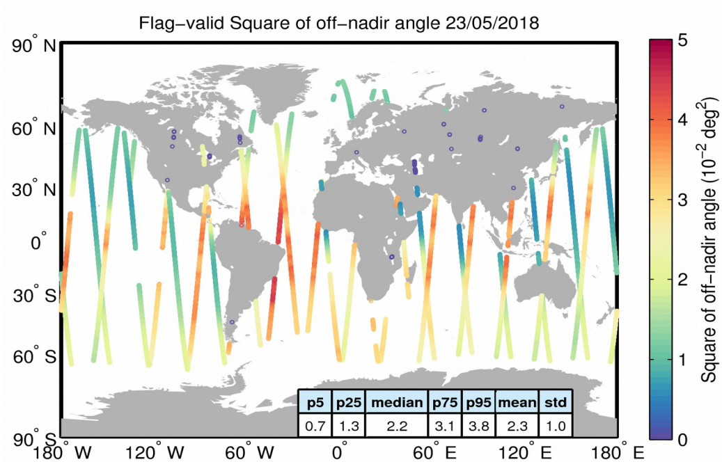
Figure 37. Geographical distribution of flag-valid mispointing data over oceans and lakes for 23/05/2018. The statistical values shown in the table refer to the mispointing in 10^{-2} \text{ deg}^2 and are calculated over all measurements shown in the figure.
