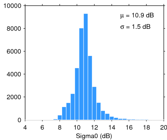
Figure 28. Histogram of science-valid sigma0 over oceans and lakes for 23/05/2018. The mean ( \mu ) and standard deviation ( \sigma ) are also shown. Note that values outside [4 20] dB are excluded from the histogram for the sake of readability but not from the computation of \mu and \sigma .
