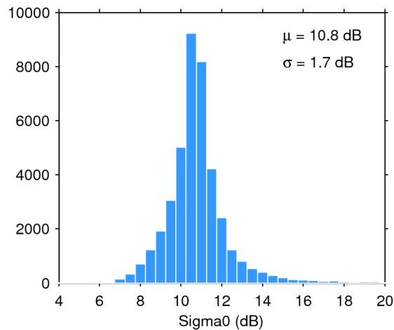
Figure 25. Histogram of flag-valid sigma0 over oceans and lakes for 21/05/2018. The mean ( \mu ) and standard deviation ( \sigma ) are also shown. Note that values outside [4 20] dB are excluded from the histogram for the sake of readability but not from the computation of \mu and \sigma .
