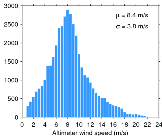
Figure 35. Histogram of science-valid wind over oceans and lakes for 21/05/2018. The mean ( \mu ) and standard deviation ( \sigma ) are also shown. Note that values larger than 24 m/s are excluded from the histogram for the sake of readability but not from the computation of \mu and \sigma .
