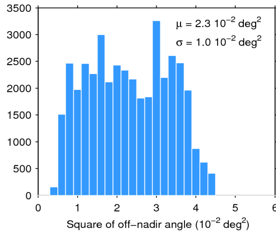
Figure 39. Histogram of flag-valid mispointing over oceans and lakes for 21/05/2018. The mean ( \mu ) and standard deviation ( \sigma ) are also shown. Note that values larger than 6 \cdot 10^{-2} \text{ deg}^2 are excluded from the histogram for the sake of readability but not from the computation of \mu and \sigma .
