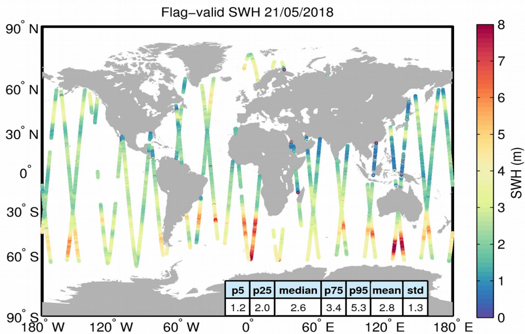
Figure 15. Geographical distribution of flag-valid SWH data over oceans and lakes for 21/05/2018. The statistical values shown in the table refer to the SWH in m and are calculated over all measurements shown in the figure.
