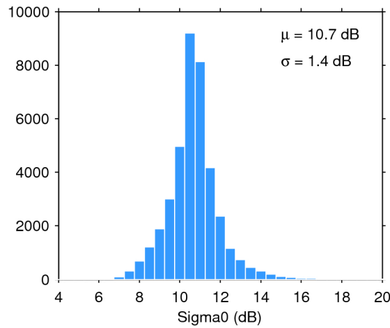
Figure 28. Histogram of science-valid sigma0 over oceans and lakes for 21/05/2018. The mean ( \mu ) and standard deviation ( \sigma ) are also shown. Note that values outside [4 20] dB are excluded from the histogram for the sake of readability but not from the computation of \mu and \sigma .
