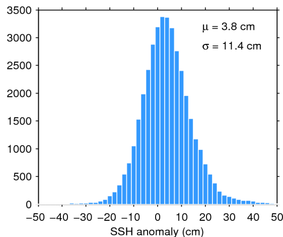
Figure 11. Histogram of science-valid SSH anomaly over oceans and lakes for 21/05/2018. The mean ( \mu ) and standard deviation ( \sigma ) are also shown. Note that values outside [-50 50] cm are excluded from the histogram for the sake of readability but not from the computation of \mu and \sigma .
