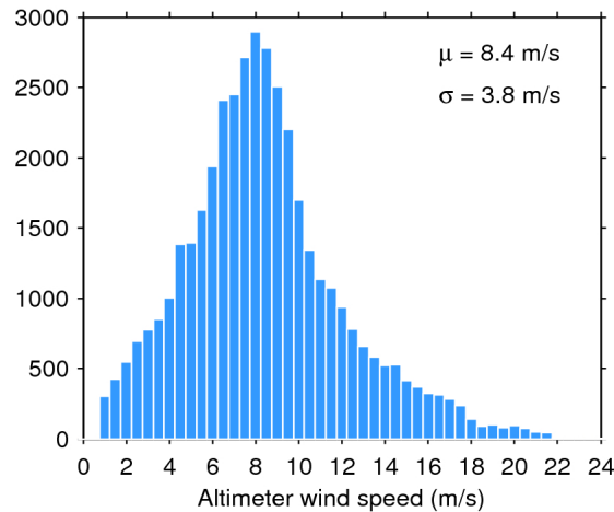
Figure 33. Histogram of flag-valid wind over oceans and lakes for 21/05/2018. The mean ( \mu ) and standard deviation ( \sigma ) are also shown. Note that values larger than 24 m/s are excluded from the histogram for the sake of readability but not from the computation of \mu and \sigma .
