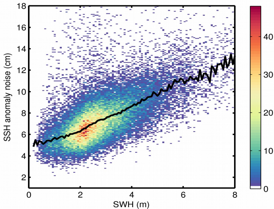
Figure 9. 2D histogram showing flag-valid SSH anomaly noise as a function of SWH for 21/05/2018. The black line denotes the median SSH anomaly noise as a function of SWH.
