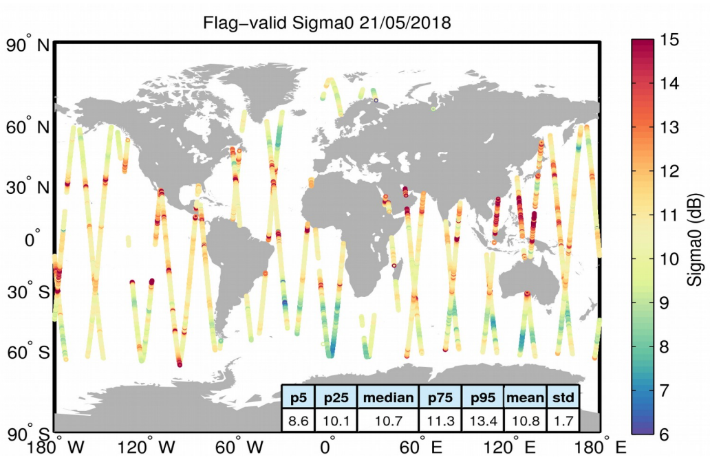
Figure 23. Geographical distribution of flag-valid sigma0 data over oceans and lakes for 21/05/2018. The statistical values shown in the table refer to the sigma0 in dB and are calculated over all measurements shown in the figure.
