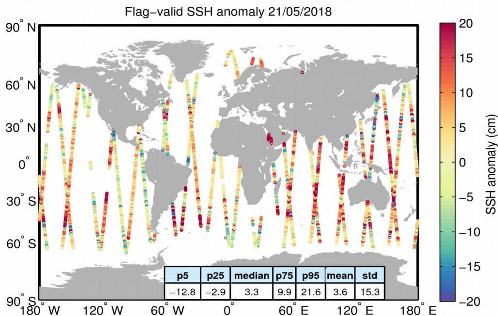
Figure 5. Geographical distribution of flag-valid 1-Hz SSH anomaly data over oceans and lakes for 21/05/2018. The statistical values shown in the table refer to the SSH anomaly in cm and are calculated over all measurements shown in the figure.
