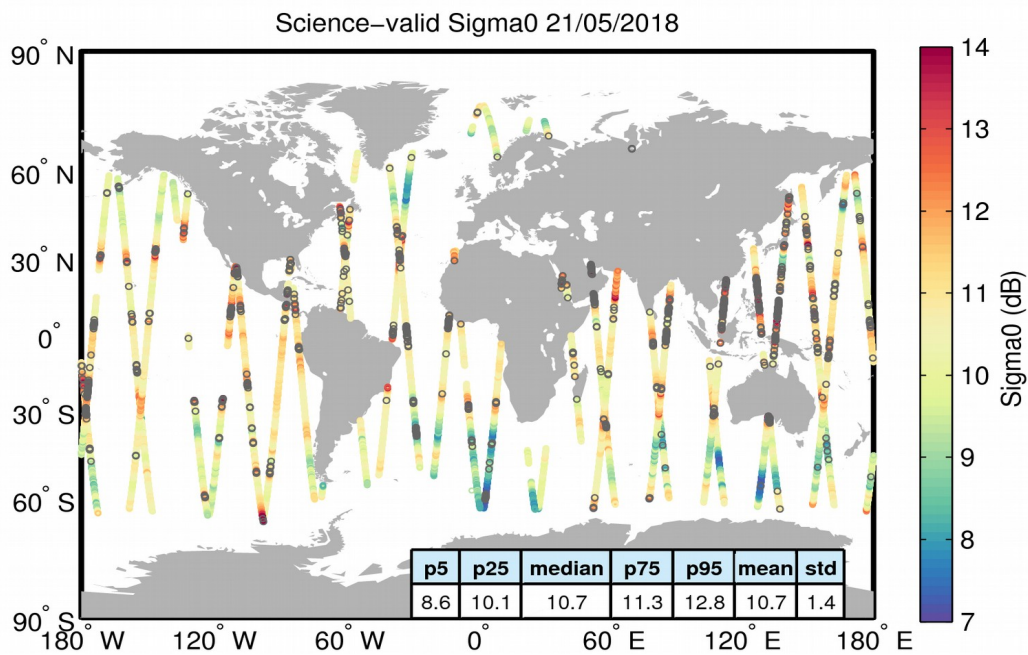
Figure 27. Geographical distribution of science-valid sigma0 data over oceans and lakes for 21/05/2018. The statistical values shown in the table refer to the sigma0 in dB and are calculated over all measurements shown in the figure. Gray circles denote records that have been rejected based on the editing criteria described in Table 4.
