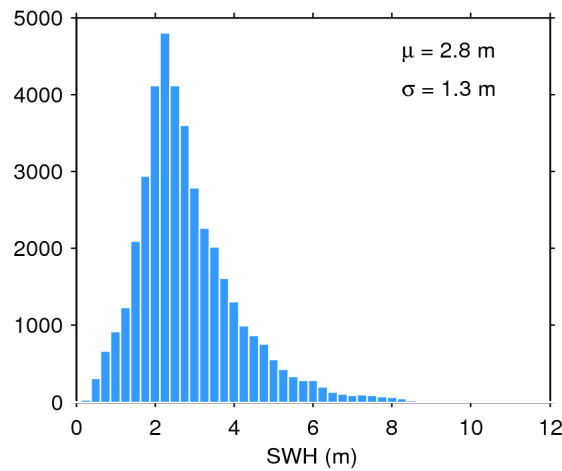
Figure 17. Histogram of flag-valid SWH over oceans and lakes for 21/05/2018. The mean ( \mu ) and standard deviation ( \sigma ) are also shown. Note that values larger than 12 m are excluded from the histogram for the sake of readability but not from the computation of \mu and \sigma .
