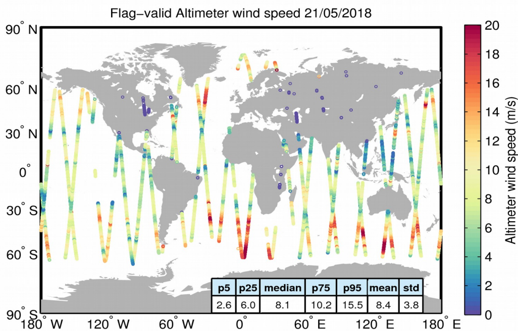
Figure 31. Geographical distribution of flag-valid wind data over oceans and lakes for 21/05/2018. The statistical values shown in the table refer to the wind in m/s and are calculated over all measurements shown in the figure.
