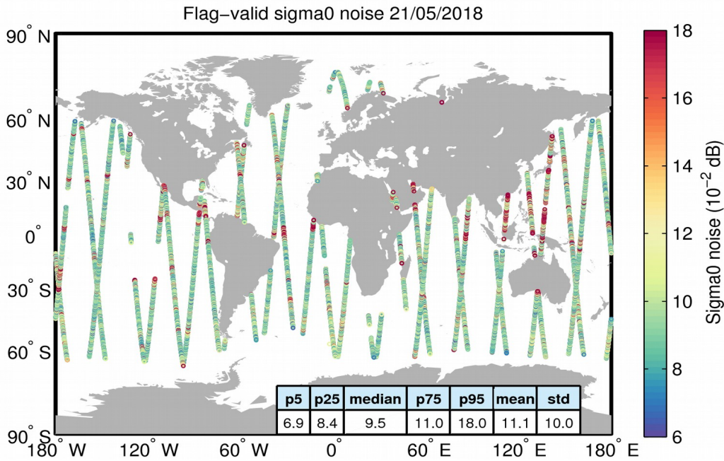
Figure 26. Geographical distribution of flag-valid 20-Hz sigma0 measurement noise over oceans and lakes for 21/05/2018. The statistical values shown in the table refer to the sigma0 noise and are calculated over all measurements shown in the figure.
