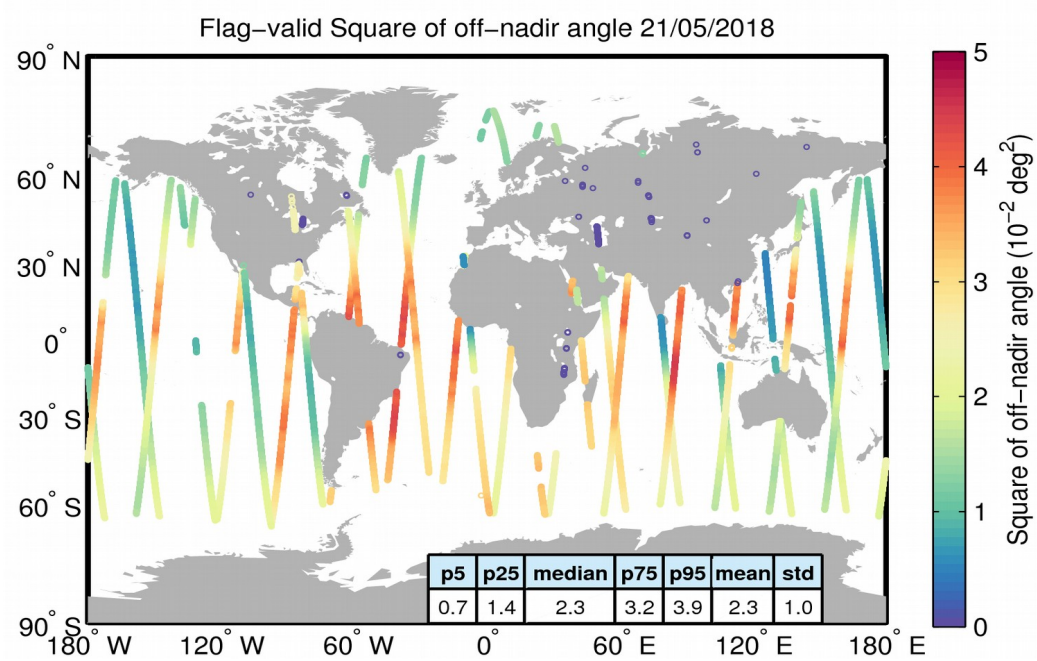
Figure 37. Geographical distribution of flag-valid mispointing data over oceans and lakes for 21/05/2018. The statistical values shown in the table refer to the mispointing in 10^{-2} \text{ deg}^2 and are calculated over all measurements shown in the figure.
