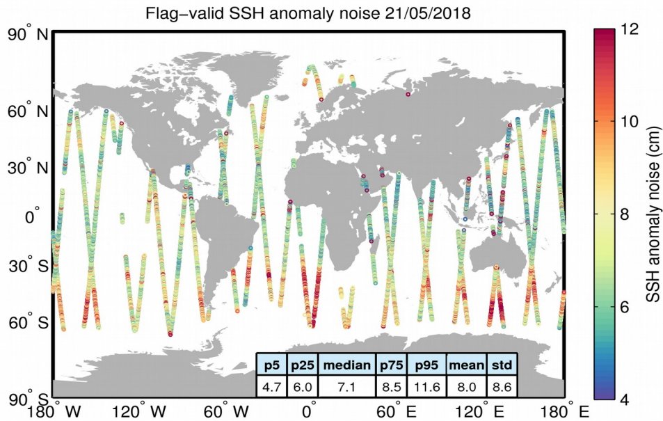
Figure 8. Geographical distribution of flag-valid 20-Hz SSH anomaly measurement noise over oceans and lakes for 21/05/2018. The statistical values shown in the table refer to the SSH anomaly noise and are calculated over all measurements shown in the figure.
