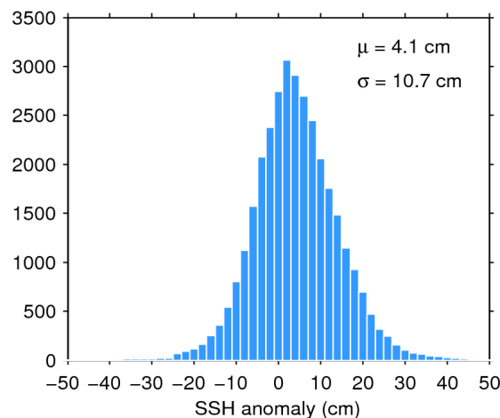
Figure 11. Histogram of science-valid SSH anomaly over oceans and lakes for 20/05/2018. The mean ( \mu ) and standard deviation ( \sigma ) are also shown. Note that values outside [-50 50] cm are excluded from the histogram for the sake of readability but not from the computation of \mu and \sigma .
