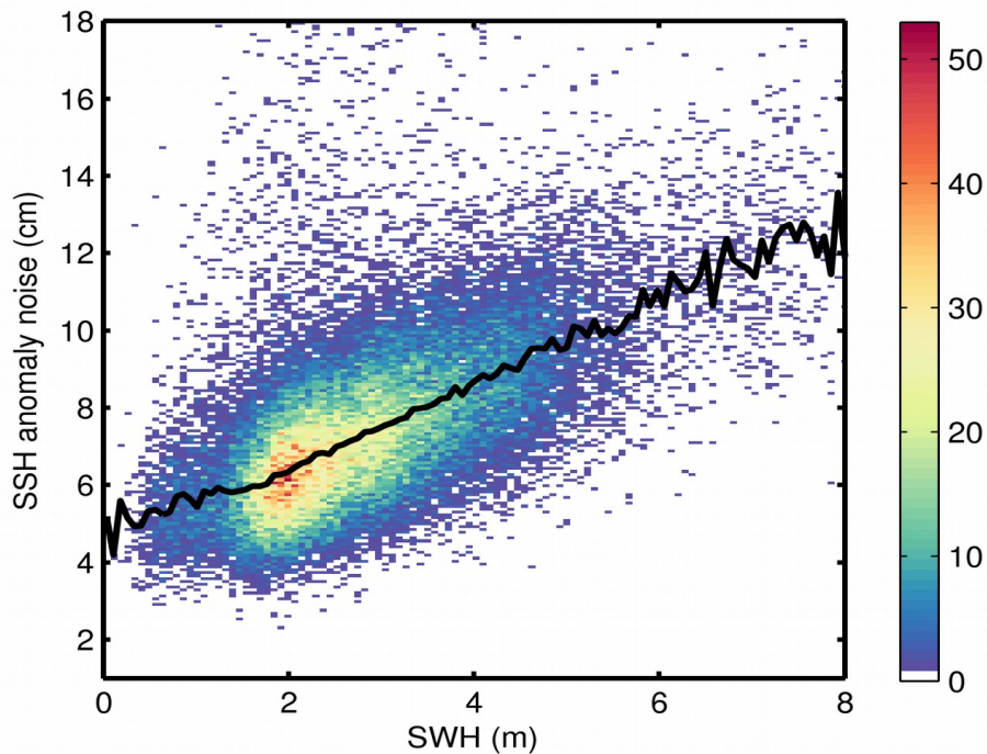
Figure 9. 2D histogram showing flag-valid SSH anomaly noise as a function of SWH for 20/05/2018. The black line denotes the median SSH anomaly noise as a function of SWH.
