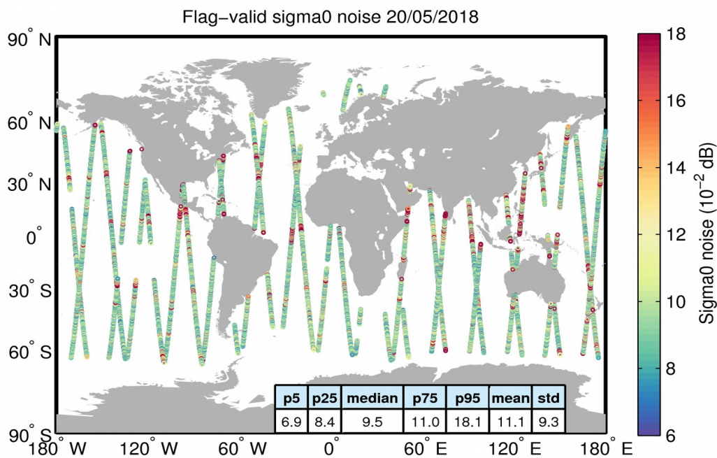
Figure 26. Geographical distribution of flag-valid 20-Hz sigma0 measurement noise over oceans and lakes for 20/05/2018. The statistical values shown in the table refer to the sigma0 noise and are calculated over all measurements shown in the figure.
