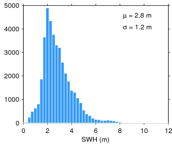
Figure 17. Histogram of flag-valid SWH over oceans and lakes for 20/05/2018. The mean ( \mu ) and standard deviation ( \sigma ) are also shown. Note that values larger than 12 m are excluded from the histogram for the sake of readability but not from the computation of \mu and \sigma .
