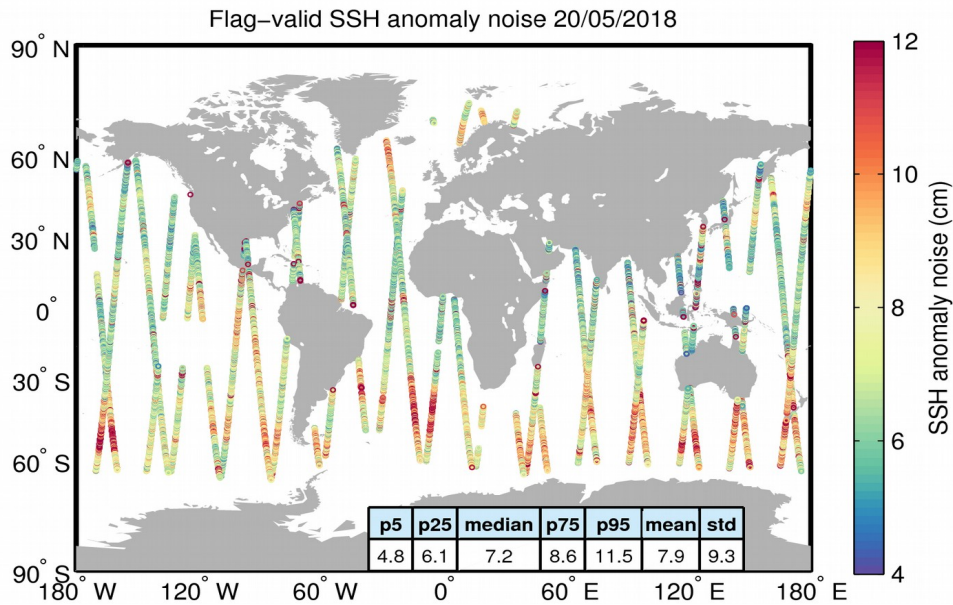
Figure 8. Geographical distribution of flag-valid 20-Hz SSH anomaly measurement noise over oceans and lakes for 20/05/2018. The statistical values shown in the table refer to the SSH anomaly noise and are calculated over all measurements shown in the figure.
