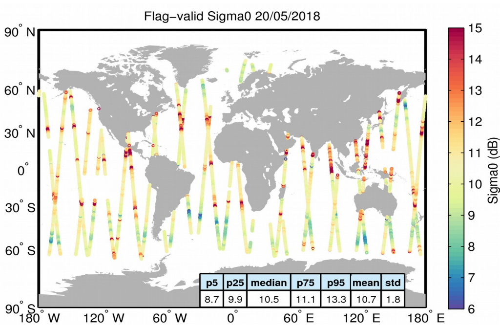
Figure 23. Geographical distribution of flag-valid sigma0 data over oceans and lakes for 20/05/2018. The statistical values shown in the table refer to the sigma0 in dB and are calculated over all measurements shown in the figure.
