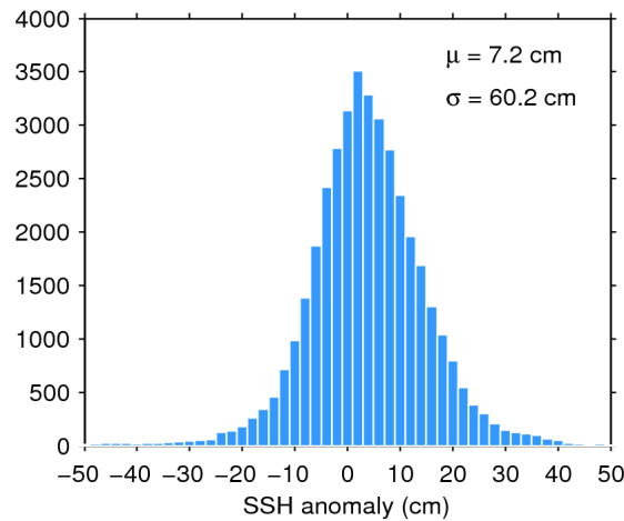
Figure 7. Histogram of flag-valid SSH anomaly over oceans and lakes for 20/05/2018. The mean ( \mu ) and standard deviation ( \sigma ) are also shown. Note that values outside [-50\ 50] cm are excluded from the histogram for the sake of readability but not from the computation of \mu and \sigma .
