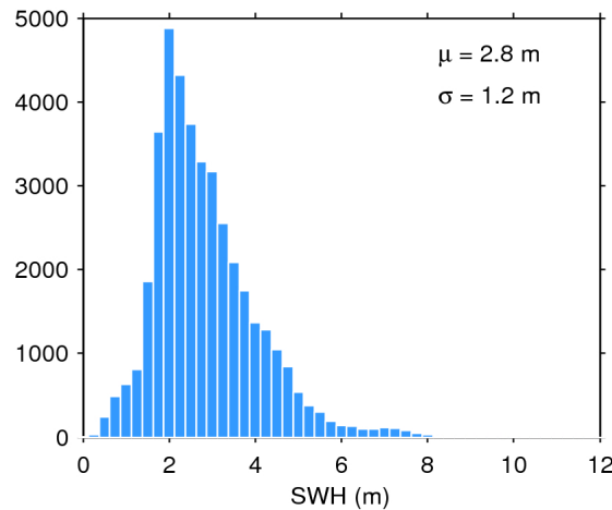
Figure 20. Histogram of science-valid SWH over oceans and lakes for 20/05/2018. The mean ( \mu ) and standard deviation ( \sigma ) are also shown. Note that values larger than 12 m are excluded from the histogram for the sake of readability but not from the computation of \mu and \sigma .
