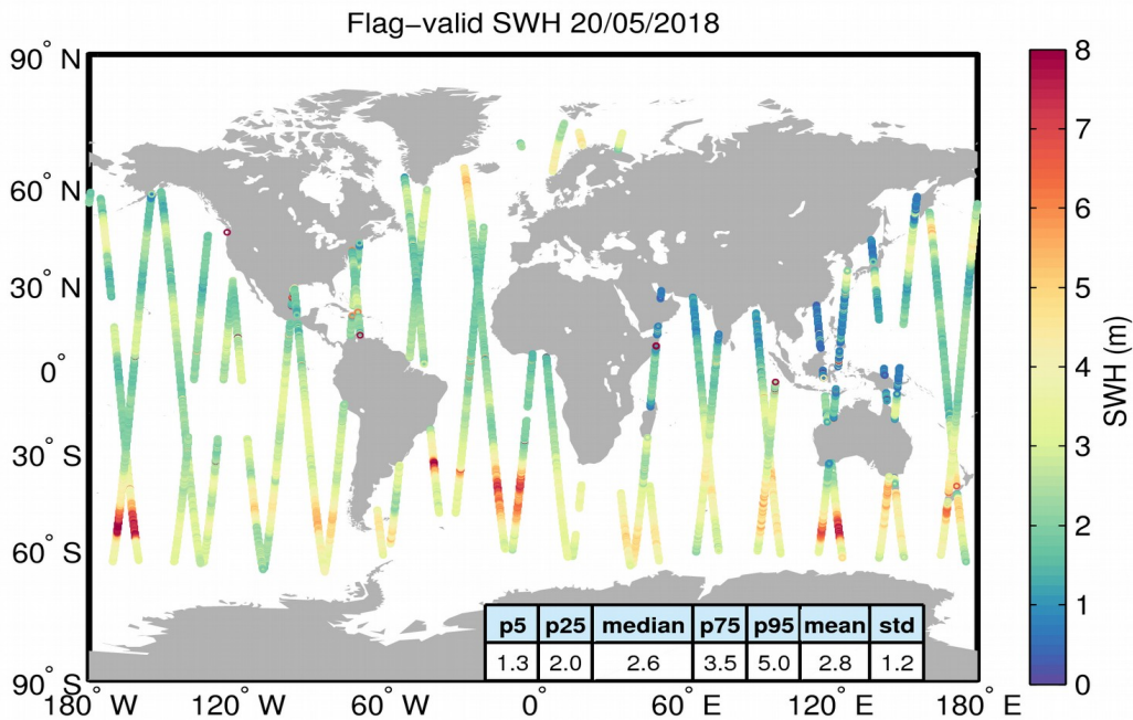
Figure 15. Geographical distribution of flag-valid SWH data over oceans and lakes for 20/05/2018. The statistical values shown in the table refer to the SWH in m and are calculated over all measurements shown in the figure.
