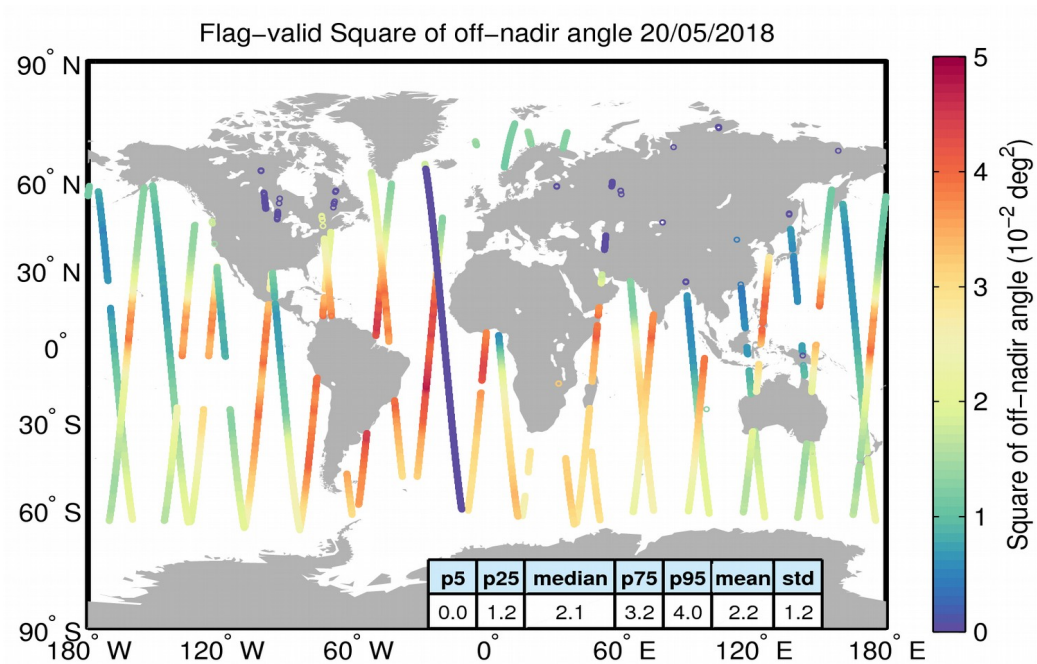
Figure 37. Geographical distribution of flag-valid mispointing data over oceans and lakes for 20/05/2018. The statistical values shown in the table refer to the mispointing in 10^{-2} \text{ deg}^2 and are calculated over all measurements shown in the figure.
