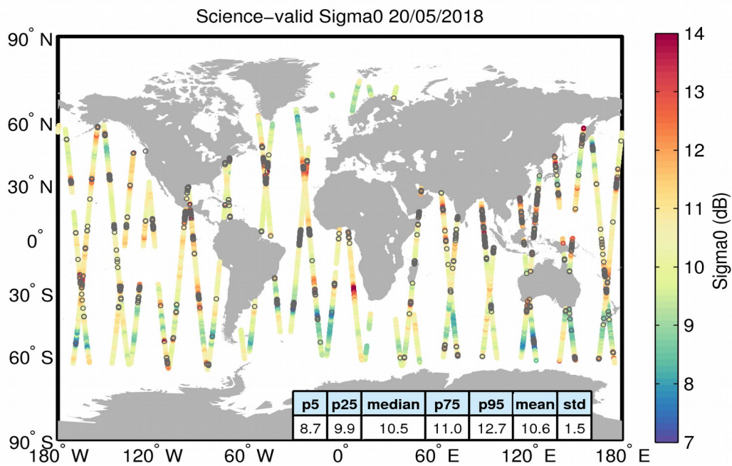
Figure 27. Geographical distribution of science-valid sigma0 data over oceans and lakes for 20/05/2018. The statistical values shown in the table refer to the sigma0 in dB and are calculated over all measurements shown in the figure. Gray circles denote records that have been rejected based on the editing criteria described in Table 4.
