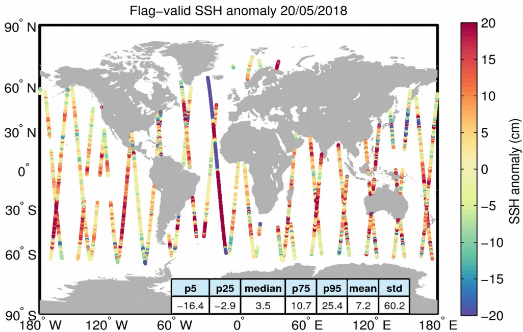
Figure 5. Geographical distribution of flag-valid 1-Hz SSH anomaly data over oceans and lakes for 20/05/2018. The statistical values shown in the table refer to the SSH anomaly in cm and are calculated over all measurements shown in the figure.
