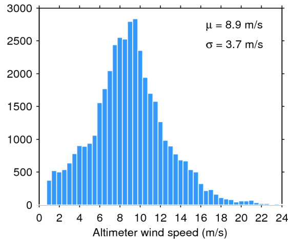
Figure 33. Histogram of flag-valid wind over oceans and lakes for 20/05/2018. The mean ( \mu ) and standard deviation ( \sigma ) are also shown. Note that values larger than 24 m/s are excluded from the histogram for the sake of readability but not from the computation of \mu and \sigma .
