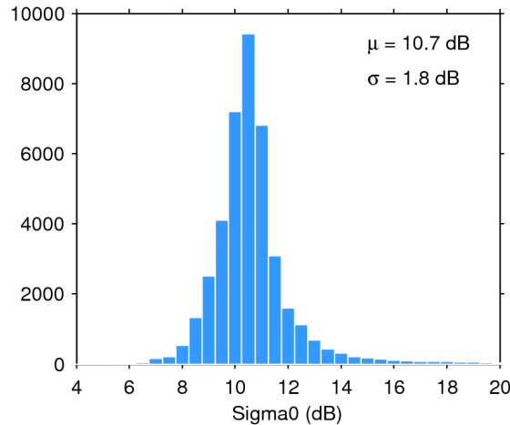
Figure 25. Histogram of flag-valid sigma0 over oceans and lakes for 20/05/2018. The mean ( \mu ) and standard deviation ( \sigma ) are also shown. Note that values outside [4 20] dB are excluded from the histogram for the sake of readability but not from the computation of \mu and \sigma .
