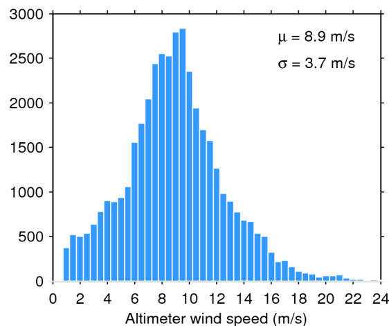
Figure 35. Histogram of science-valid wind over oceans and lakes for 20/05/2018. The mean ( \mu ) and standard deviation ( \sigma ) are also shown. Note that values larger than 24 m/s are excluded from the histogram for the sake of readability but not from the computation of \mu and \sigma .
