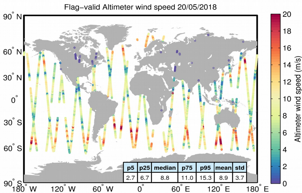
Figure 31. Geographical distribution of flag-valid wind data over oceans and lakes for 20/05/2018. The statistical values shown in the table refer to the wind in m/s and are calculated over all measurements shown in the figure.
