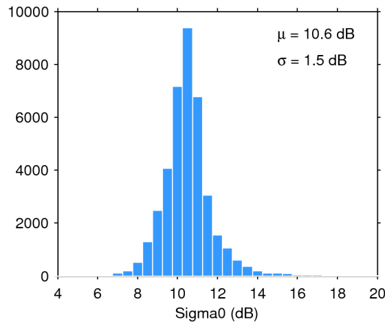
Figure 28. Histogram of science-valid sigma0 over oceans and lakes for 20/05/2018. The mean ( \mu ) and standard deviation ( \sigma ) are also shown. Note that values outside [4 20] dB are excluded from the histogram for the sake of readability but not from the computation of \mu and \sigma .
