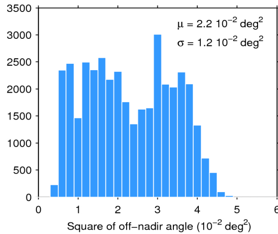
Figure 39. Histogram of flag-valid mispointing over oceans and lakes for 20/05/2018. The mean ( \mu ) and standard deviation ( \sigma ) are also shown. Note that values larger than 6 \cdot 10^{-2} \text{ deg}^2 are excluded from the histogram for the sake of readability but not from the computation of \mu and \sigma .
