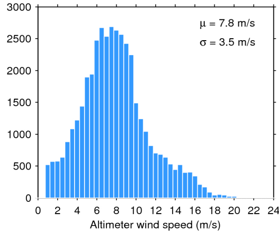
Figure 33. Histogram of flag-valid wind over oceans and lakes for 19/05/2018. The mean ( \mu ) and standard deviation ( \sigma ) are also shown. Note that values larger than 24 m/s are excluded from the histogram for the sake of readability but not from the computation of \mu and \sigma .
