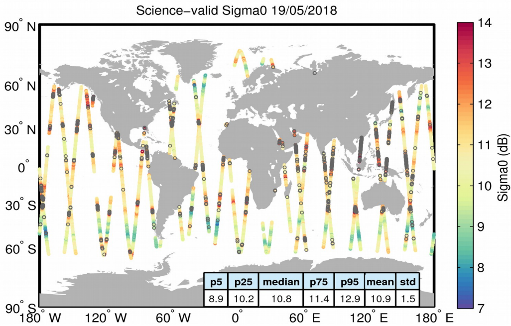
Figure 27. Geographical distribution of science-valid sigma0 data over oceans and lakes for 19/05/2018. The statistical values shown in the table refer to the sigma0 in dB and are calculated over all measurements shown in the figure. Gray circles denote records that have been rejected based on the editing criteria described in Table 4.
