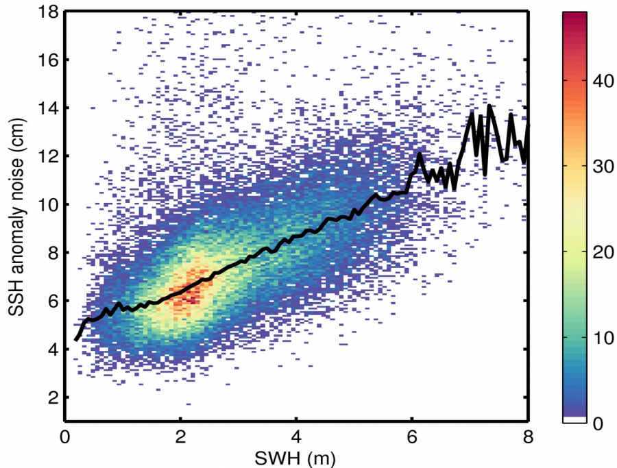
Figure 9. 2D histogram showing flag-valid SSH anomaly noise as a function of SWH for 19/05/2018. The black line denotes the median SSH anomaly noise as a function of SWH.
