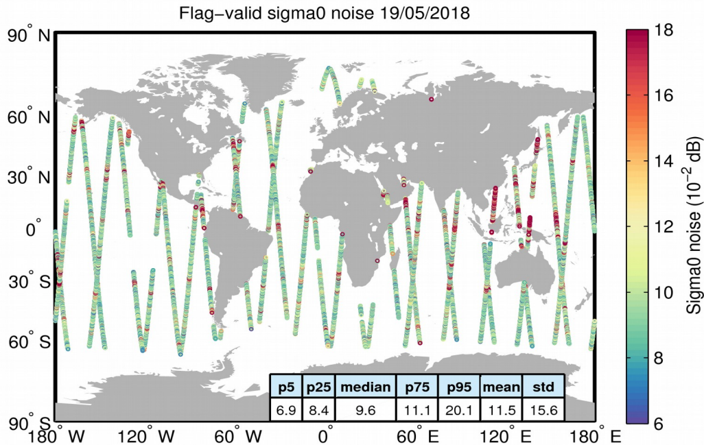
Figure 26. Geographical distribution of flag-valid 20-Hz sigma0 measurement noise over oceans and lakes for 19/05/2018. The statistical values shown in the table refer to the sigma0 noise and are calculated over all measurements shown in the figure.
