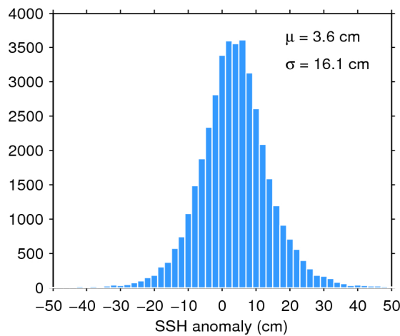
Figure 7. Histogram of flag-valid SSH anomaly over oceans and lakes for 19/05/2018. The mean ( \mu ) and standard deviation ( \sigma ) are also shown. Note that values outside [-50 50] cm are excluded from the histogram for the sake of readability but not from the computation of \mu and \sigma .
