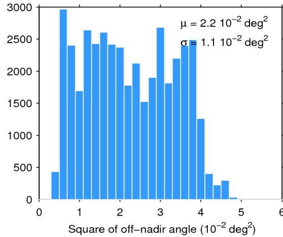
Figure 39. Histogram of flag-valid mispointing over oceans and lakes for 19/05/2018. The mean ( \mu ) and standard deviation ( \sigma ) are also shown. Note that values larger than 6 \cdot 10^{-2} \text{ deg}^2 are excluded from the histogram for the sake of readability but not from the computation of \mu and \sigma .
