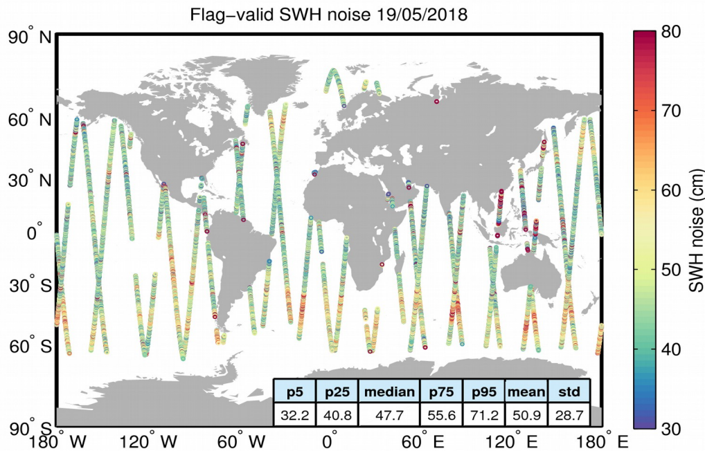
Figure 18. Geographical distribution of flag-valid 20-Hz SWH measurement noise over oceans and lakes for 19/05/2018. The statistical values shown in the figure refer to the SWH noise and are calculated over all measurements shown in the figure.
