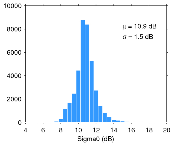
Figure 28. Histogram of science-valid sigma0 over oceans and lakes for 19/05/2018. The mean ( \mu ) and standard deviation ( \sigma ) are also shown. Note that values outside [4 20] dB are excluded from the histogram for the sake of readability but not from the computation of \mu and \sigma .
