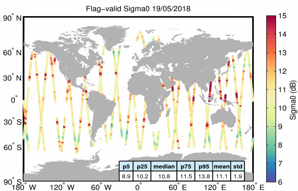
Figure 23. Geographical distribution of flag-valid sigma0 data over oceans and lakes for 19/05/2018. The statistical values shown in the table refer to the sigma0 in dB and are calculated over all measurements shown in the figure.
