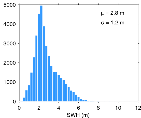
Figure 20. Histogram of science-valid SWH over oceans and lakes for 19/05/2018. The mean ( \mu ) and standard deviation ( \sigma ) are also shown. Note that values larger than 12 m are excluded from the histogram for the sake of readability but not from the computation of \mu and \sigma .
