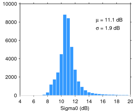
Figure 25. Histogram of flag-valid sigma0 over oceans and lakes for 19/05/2018. The mean ( \mu ) and standard deviation ( \sigma ) are also shown. Note that values outside [4 20] dB are excluded from the histogram for the sake of readability but not from the computation of \mu and \sigma .
