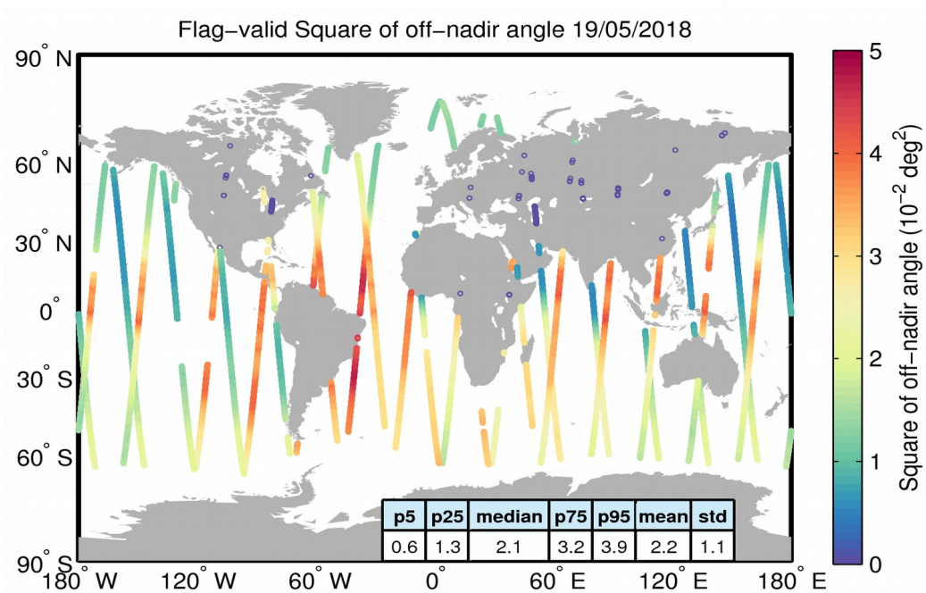
Figure 37. Geographical distribution of flag-valid mispointing data over oceans and lakes for 19/05/2018. The statistical values shown in the table refer to the mispointing in 10^{-2} \text{ deg}^2 and are calculated over all measurements shown in the figure.
