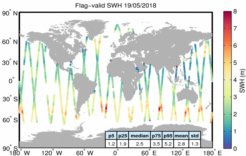
Figure 15. Geographical distribution of flag-valid SWH data over oceans and lakes for 19/05/2018. The statistical values shown in the table refer to the SWH in m and are calculated over all measurements shown in the figure.
