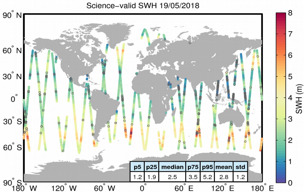
Figure 19. Geographical distribution of science-valid SWH data over oceans and lakes for 19/05/2018. The statistical values shown in the table refer to the SWH in m and are calculated over all measurements shown in the figure. Gray circles denote records that have been rejected based on the editing criteria described in Table 3.
