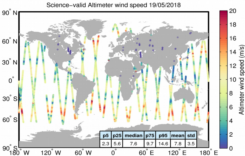
Figure 34. Geographical distribution of science-valid wind data over oceans and lakes for 19/05/2018. The statistical values shown in the table refer to the wind in m/s and are calculated over all measurements shown in the figure. Gray circles denote records that have been rejected based on the editing criteria described in Table 5.
