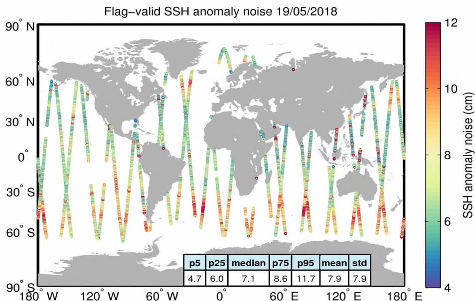
Figure 8. Geographical distribution of flag-valid 20-Hz SSH anomaly measurement noise over oceans and lakes for 19/05/2018. The statistical values shown in the table refer to the SSH anomaly noise and are calculated over all measurements shown in the figure.
