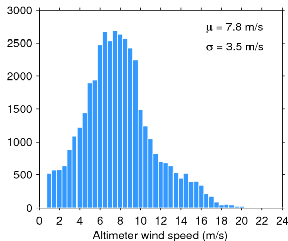
Figure 35. Histogram of science-valid wind over oceans and lakes for 19/05/2018. The mean ( \mu ) and standard deviation ( \sigma ) are also shown. Note that values larger than 24 m/s are excluded from the histogram for the sake of readability but not from the computation of \mu and \sigma .
