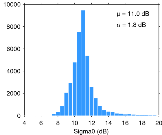
Figure 25. Histogram of flag-valid sigma0 over oceans and lakes for 18/05/2018. The mean ( \mu ) and standard deviation ( \sigma ) are also shown. Note that values outside [4 20] dB are excluded from the histogram for the sake of readability but not from the computation of \mu and \sigma .
