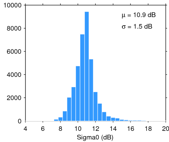
Figure 28. Histogram of science-valid sigma0 over oceans and lakes for 18/05/2018. The mean ( \mu ) and standard deviation ( \sigma ) are also shown. Note that values outside [4 20] dB are excluded from the histogram for the sake of readability but not from the computation of \mu and \sigma .
