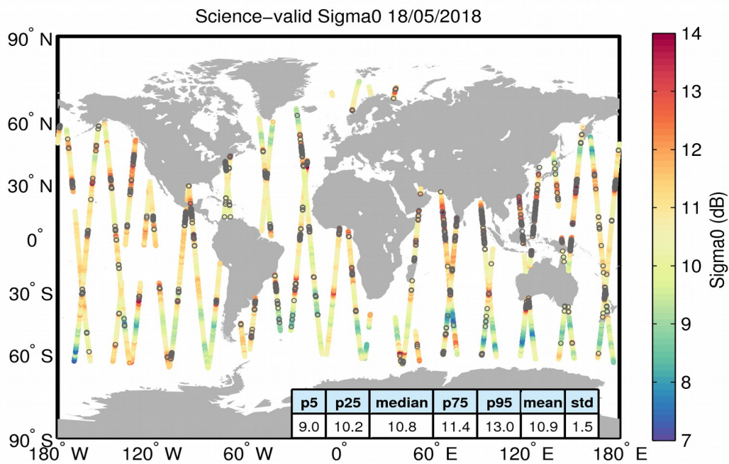
Figure 27. Geographical distribution of science-valid sigma0 data over oceans and lakes for 18/05/2018. The statistical values shown in the table refer to the sigma0 in dB and are calculated over all measurements shown in the figure. Gray circles denote records that have been rejected based on the editing criteria described in Table 4.
