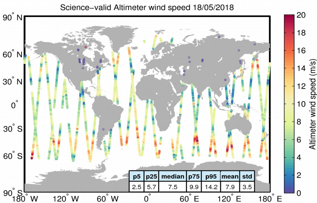
Figure 34. Geographical distribution of science-valid wind data over oceans and lakes for 18/05/2018. The statistical values shown in the table refer to the wind in m/s and are calculated over all measurements shown in the figure. Gray circles denote records that have been rejected based on the editing criteria described in Table 5.
