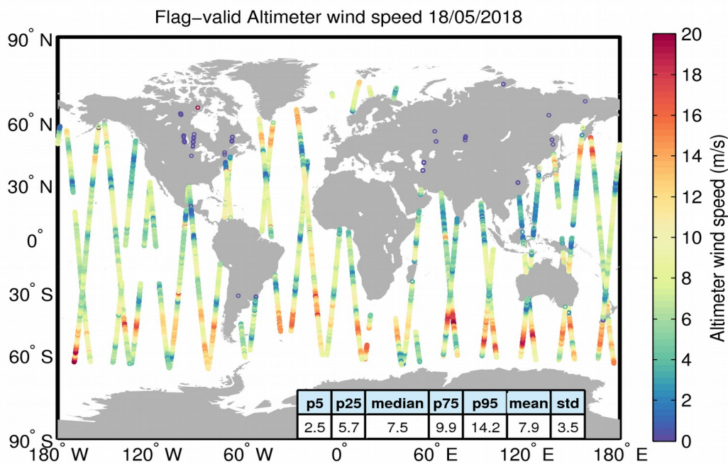
Figure 31. Geographical distribution of flag-valid wind data over oceans and lakes for 18/05/2018. The statistical values shown in the table refer to the wind in m/s and are calculated over all measurements shown in the figure.
