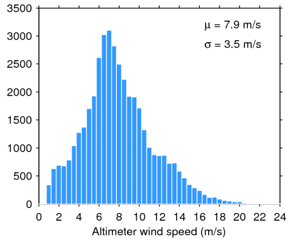
Figure 33. Histogram of flag-valid wind over oceans and lakes for 18/05/2018. The mean ( \mu ) and standard deviation ( \sigma ) are also shown. Note that values larger than 24 m/s are excluded from the histogram for the sake of readability but not from the computation of \mu and \sigma .
