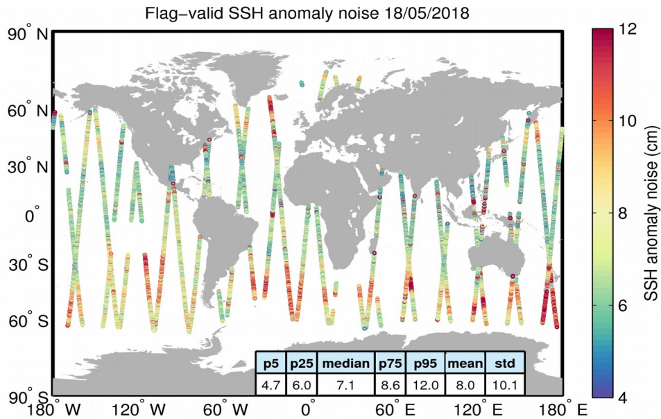
Figure 8. Geographical distribution of flag-valid 20-Hz SSH anomaly measurement noise over oceans and lakes for 18/05/2018. The statistical values shown in the table refer to the SSH anomaly noise and are calculated over all measurements shown in the figure.
