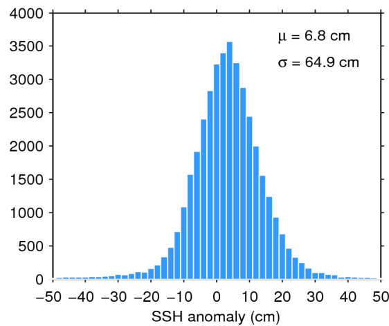
Figure 7. Histogram of flag-valid SSH anomaly over oceans and lakes for 18/05/2018. The mean ( \mu ) and standard deviation ( \sigma ) are also shown. Note that values outside [-50 50] cm are excluded from the histogram for the sake of readability but not from the computation of \mu and \sigma .
