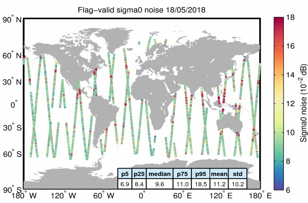
Figure 26. Geographical distribution of flag-valid 20-Hz sigma0 measurement noise over oceans and lakes for 18/05/2018. The statistical values shown in the table refer to the sigma0 noise and are calculated over all measurements shown in the figure.
