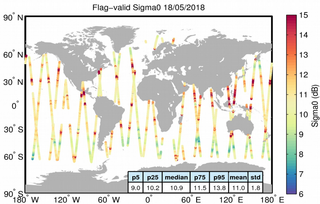
Figure 23. Geographical distribution of flag-valid sigma0 data over oceans and lakes for 18/05/2018. The statistical values shown in the table refer to the sigma0 in dB and are calculated over all measurements shown in the figure.
