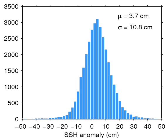
Figure 11. Histogram of science-valid SSH anomaly over oceans and lakes for 18/05/2018. The mean ( \mu ) and standard deviation ( \sigma ) are also shown. Note that values outside [-50 \text{ } 50] cm are excluded from the histogram for the sake of readability but not from the computation of \mu and \sigma .
