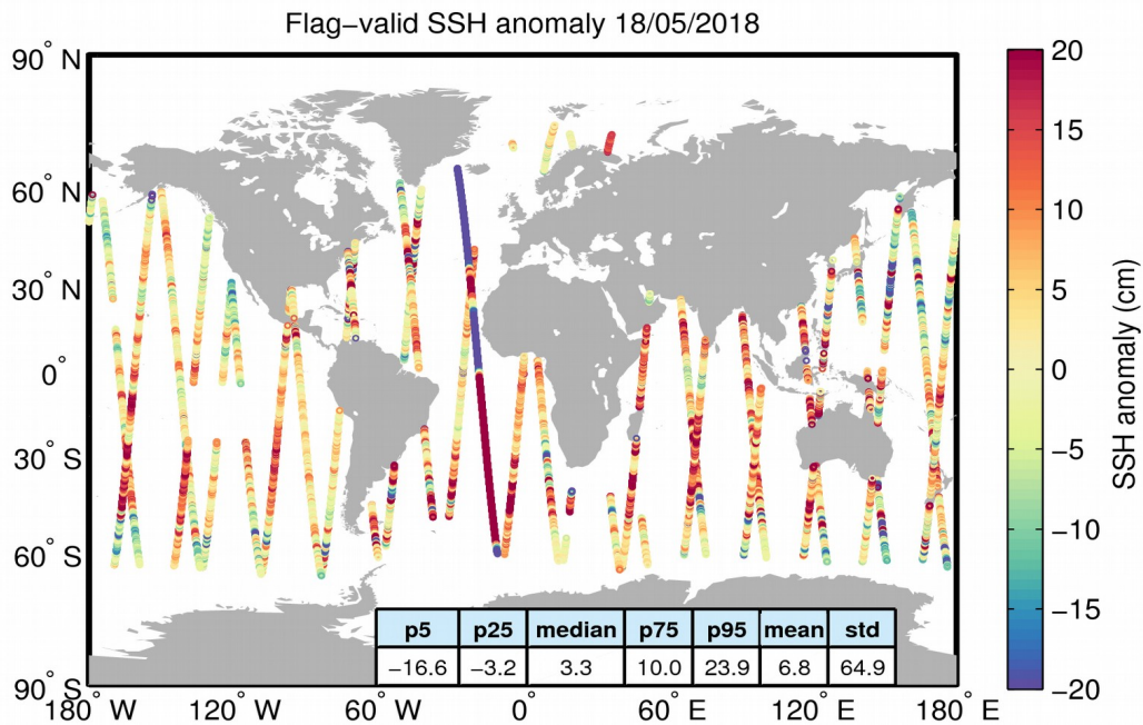
Figure 5. Geographical distribution of flag-valid 1-Hz SSH anomaly data over oceans and lakes for 18/05/2018. The statistical values shown in the table refer to the SSH anomaly in cm and are calculated over all measurements shown in the figure.
