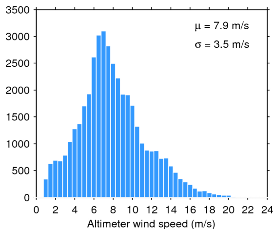
Figure 35. Histogram of science-valid wind over oceans and lakes for 18/05/2018. The mean ( \mu ) and standard deviation ( \sigma ) are also shown. Note that values larger than 24 m/s are excluded from the histogram for the sake of readability but not from the computation of \mu and \sigma .
