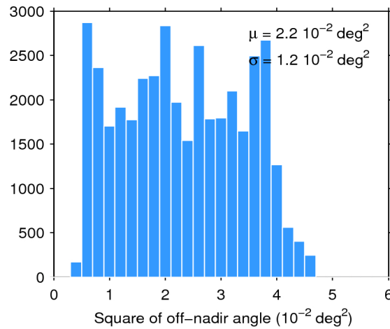
Figure 39. Histogram of flag-valid mispointing over oceans and lakes for 18/05/2018. The mean ( \mu ) and standard deviation ( \sigma ) are also shown. Note that values larger than 6 \cdot 10^{-2} \text{ deg}^2 are excluded from the histogram for the sake of readability but not from the computation of \mu and \sigma .
