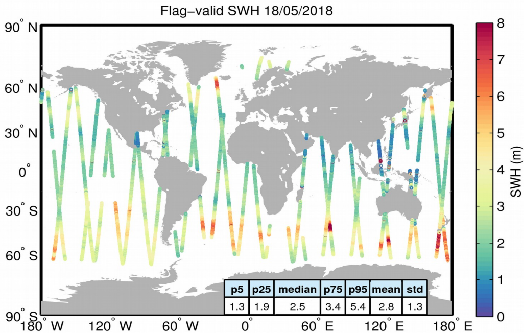
Figure 15. Geographical distribution of flag-valid SWH data over oceans and lakes for 18/05/2018. The statistical values shown in the table refer to the SWH in m and are calculated over all measurements shown in the figure.
