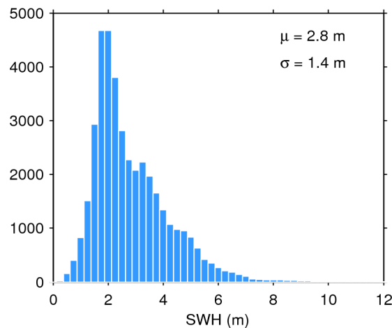
Figure 20. Histogram of science-valid SWH over oceans and lakes for 17/05/2018. The mean ( \mu ) and standard deviation ( \sigma ) are also shown. Note that values larger than 12 m are excluded from the histogram for the sake of readability but not from the computation of \mu and \sigma .
