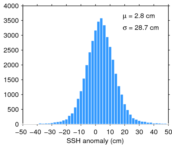
Figure 7. Histogram of flag-valid SSH anomaly over oceans and lakes for 17/05/2018. The mean ( \mu ) and standard deviation ( \sigma ) are also shown. Note that values outside [-50\ 50] cm are excluded from the histogram for the sake of readability but not from the computation of \mu and \sigma .
