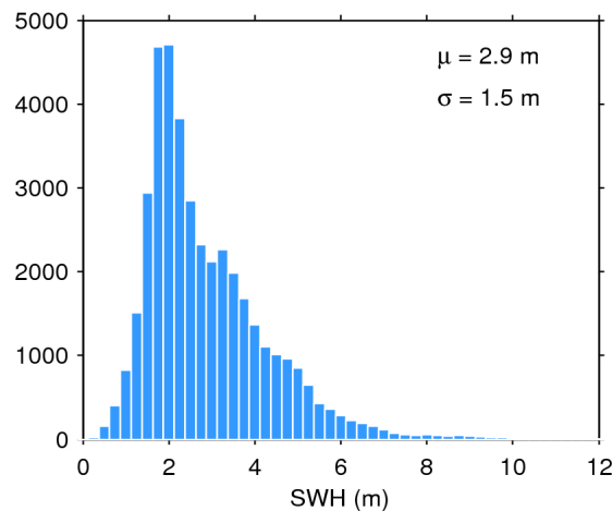
Figure 17. Histogram of flag-valid SWH over oceans and lakes for 17/05/2018. The mean ( \mu ) and standard deviation ( \sigma ) are also shown. Note that values larger than 12 m are excluded from the histogram for the sake of readability but not from the computation of \mu and \sigma .
