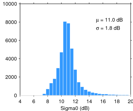
Figure 25. Histogram of flag-valid sigma0 over oceans and lakes for 17/05/2018. The mean ( \mu ) and standard deviation ( \sigma ) are also shown. Note that values outside [4 20] dB are excluded from the histogram for the sake of readability but not from the computation of \mu and \sigma .
