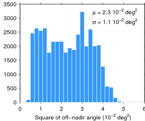
Figure 39. Histogram of flag-valid mispointing over oceans and lakes for 17/05/2018. The mean ( \mu ) and standard deviation ( \sigma ) are also shown. Note that values larger than 6 \cdot 10^{-2} \text{ deg}^2 are excluded from the histogram for the sake of readability but not from the computation of \mu and \sigma .
