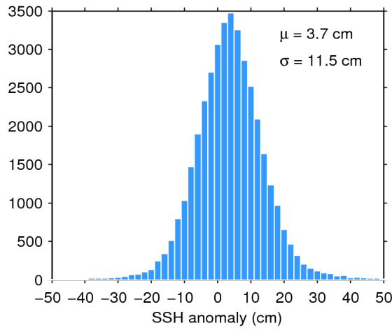
Figure 11. Histogram of science-valid SSH anomaly over oceans and lakes for 17/05/2018. The mean ( \mu ) and standard deviation ( \sigma ) are also shown. Note that values outside [-50 50] cm are excluded from the histogram for the sake of readability but not from the computation of \mu and \sigma .
