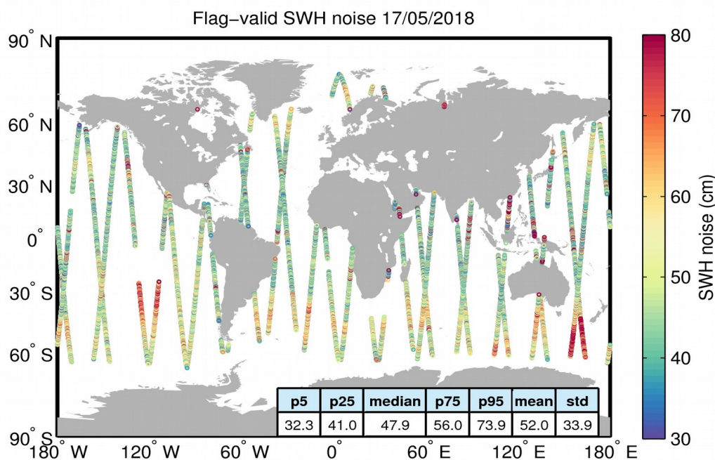
Figure 18. Geographical distribution of flag-valid 20-Hz SWH measurement noise over oceans and lakes for 17/05/2018. The statistical values shown in the figure refer to the SWH noise and are calculated over all measurements shown in the figure.
