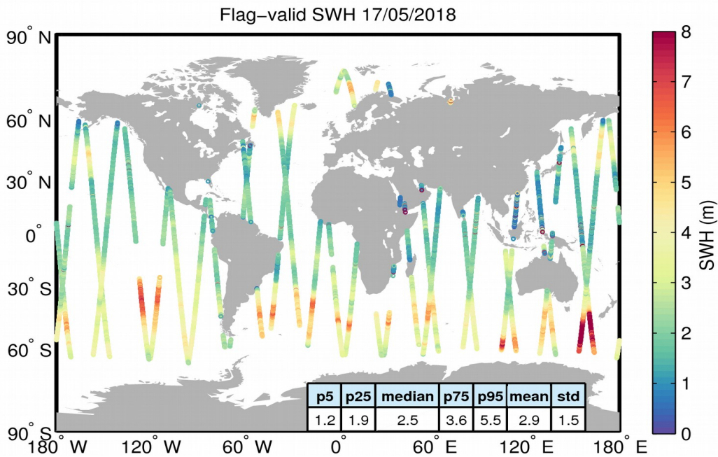
Figure 15. Geographical distribution of flag-valid SWH data over oceans and lakes for 17/05/2018. The statistical values shown in the table refer to the SWH in m and are calculated over all measurements shown in the figure.
