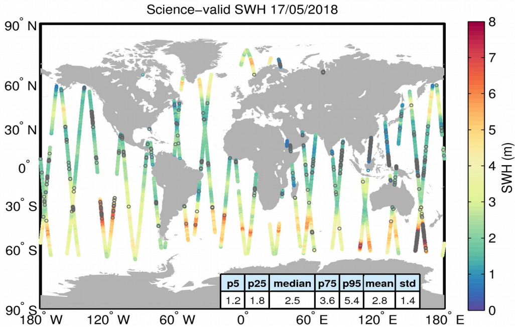
Figure 19. Geographical distribution of science-valid SWH data over oceans and lakes for 17/05/2018. The statistical values shown in the table refer to the SWH in m and are calculated over all measurements shown in the figure. Gray circles denote records that have been rejected based on the editing criteria described in Table 3.
