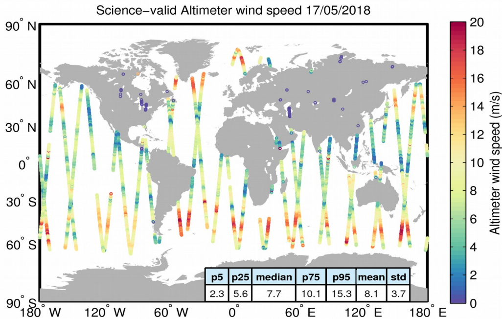
Figure 34. Geographical distribution of science-valid wind data over oceans and lakes for 17/05/2018. The statistical values shown in the table refer to the wind in m/s and are calculated over all measurements shown in the figure. Gray circles denote records that have been rejected based on the editing criteria described in Table 5.
