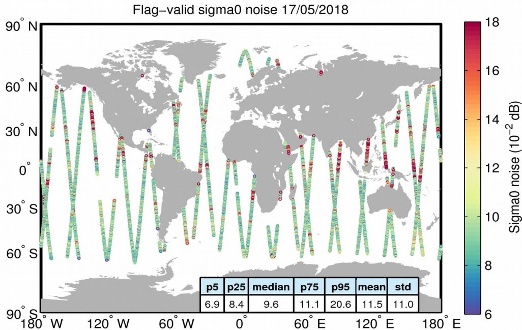
Figure 26. Geographical distribution of flag-valid 20-Hz sigma0 measurement noise over oceans and lakes for 17/05/2018. The statistical values shown in the table refer to the sigma0 noise and are calculated over all measurements shown in the figure.
