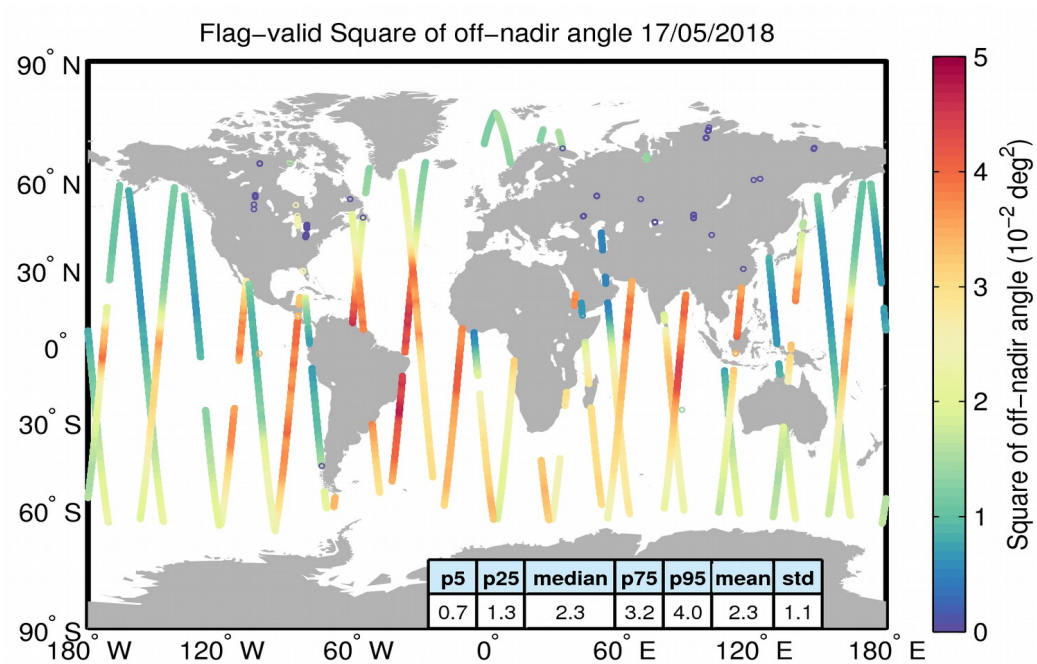
Figure 37. Geographical distribution of flag-valid mispointing data over oceans and lakes for 17/05/2018. The statistical values shown in the table refer to the mispointing in 10^{-2} \text{ deg}^2 and are calculated over all measurements shown in the figure.
