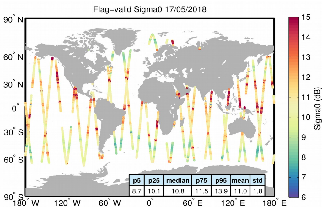
Figure 23. Geographical distribution of flag-valid sigma0 data over oceans and lakes for 17/05/2018. The statistical values shown in the table refer to the sigma0 in dB and are calculated over all measurements shown in the figure.
