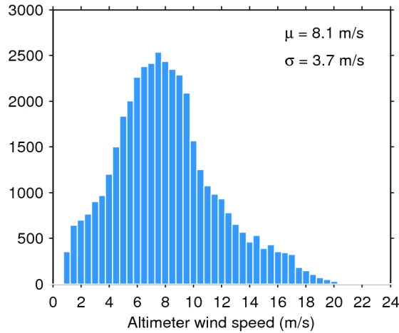
Figure 33. Histogram of flag-valid wind over oceans and lakes for 17/05/2018. The mean ( \mu ) and standard deviation ( \sigma ) are also shown. Note that values larger than 24 m/s are excluded from the histogram for the sake of readability but not from the computation of \mu and \sigma .
