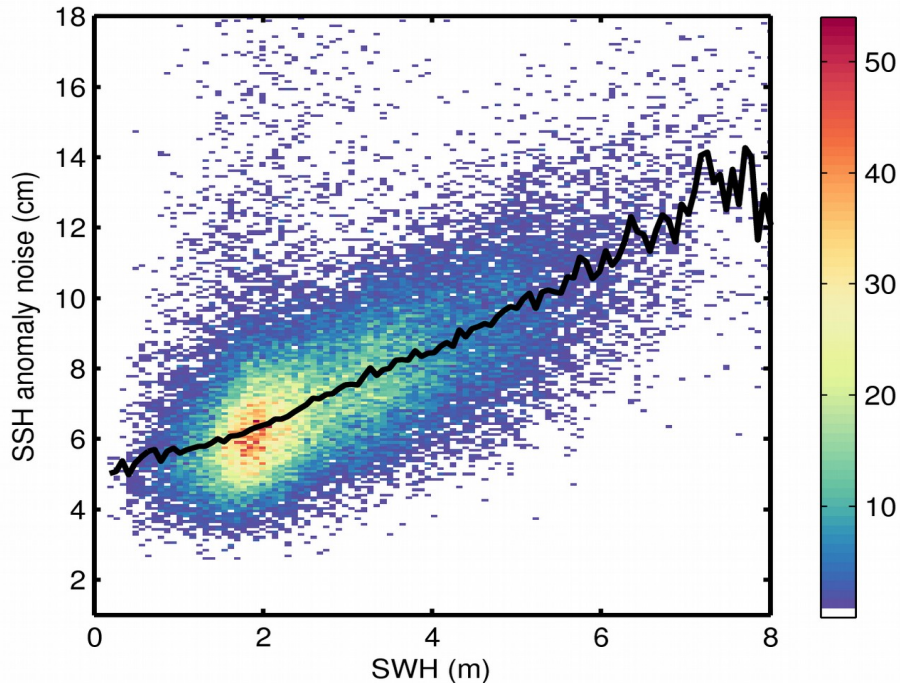
Figure 9. 2D histogram showing flag-valid SSH anomaly noise as a function of SWH for 17/05/2018. The black line denotes the median SSH anomaly noise as a function of SWH.
