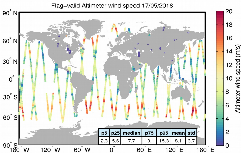
Figure 31. Geographical distribution of flag-valid wind data over oceans and lakes for 17/05/2018. The statistical values shown in the table refer to the wind in m/s and are calculated over all measurements shown in the figure.
