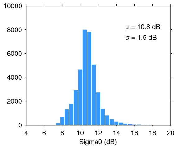
Figure 28. Histogram of science-valid sigma0 over oceans and lakes for 17/05/2018. The mean ( \mu ) and standard deviation ( \sigma ) are also shown. Note that values outside [4 20] dB are excluded from the histogram for the sake of readability but not from the computation of \mu and \sigma .
