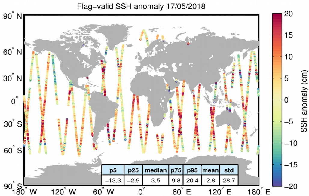
Figure 5. Geographical distribution of flag-valid 1-Hz SSH anomaly data over oceans and lakes for 17/05/2018. The statistical values shown in the table refer to the SSH anomaly in cm and are calculated over all measurements shown in the figure.
