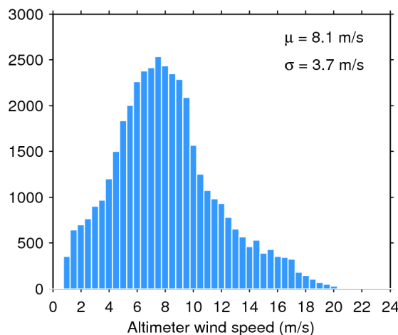
Figure 35. Histogram of science-valid wind over oceans and lakes for 17/05/2018. The mean ( \mu ) and standard deviation ( \sigma ) are also shown. Note that values larger than 24 m/s are excluded from the histogram for the sake of readability but not from the computation of \mu and \sigma .
