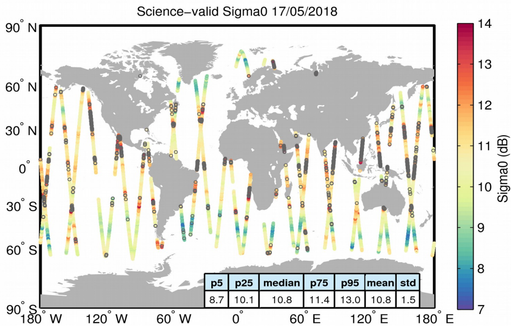
Figure 27. Geographical distribution of science-valid sigma0 data over oceans and lakes for 17/05/2018. The statistical values shown in the table refer to the sigma0 in dB and are calculated over all measurements shown in the figure. Gray circles denote records that have been rejected based on the editing criteria described in Table 4.
