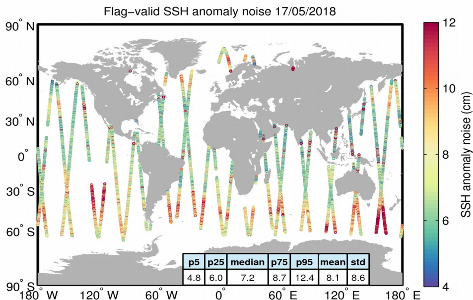
Figure 8. Geographical distribution of flag-valid 20-Hz SSH anomaly measurement noise over oceans and lakes for 17/05/2018. The statistical values shown in the table refer to the SSH anomaly noise and are calculated over all measurements shown in the figure.
