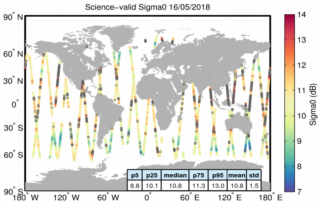
Figure 27. Geographical distribution of science-valid sigma0 data over oceans and lakes for 16/05/2018. The statistical values shown in the table refer to the sigma0 in dB and are calculated over all measurements shown in the figure. Gray circles denote records that have been rejected based on the editing criteria described in Table 4.
