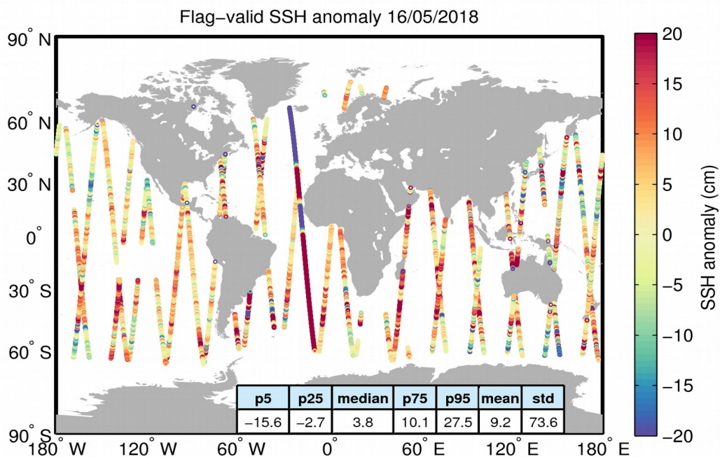
Figure 5. Geographical distribution of flag-valid 1-Hz SSH anomaly data over oceans and lakes for 16/05/2018. The statistical values shown in the table refer to the SSH anomaly in cm and are calculated over all measurements shown in the figure.
