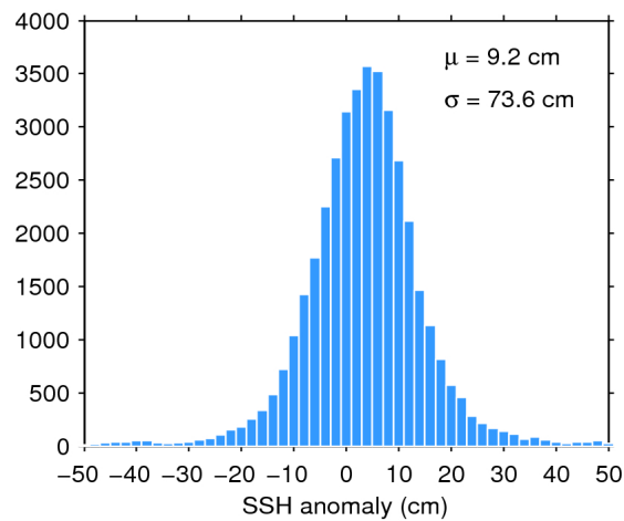
Figure 7. Histogram of flag-valid SSH anomaly over oceans and lakes for 16/05/2018. The mean ( \mu ) and standard deviation ( \sigma ) are also shown. Note that values outside [-50 50] cm are excluded from the histogram for the sake of readability but not from the computation of \mu and \sigma .
