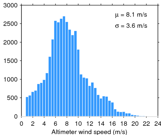
Figure 35. Histogram of science-valid wind over oceans and lakes for 16/05/2018. The mean ( \mu ) and standard deviation ( \sigma ) are also shown. Note that values larger than 24 m/s are excluded from the histogram for the sake of readability but not from the computation of \mu and \sigma .
