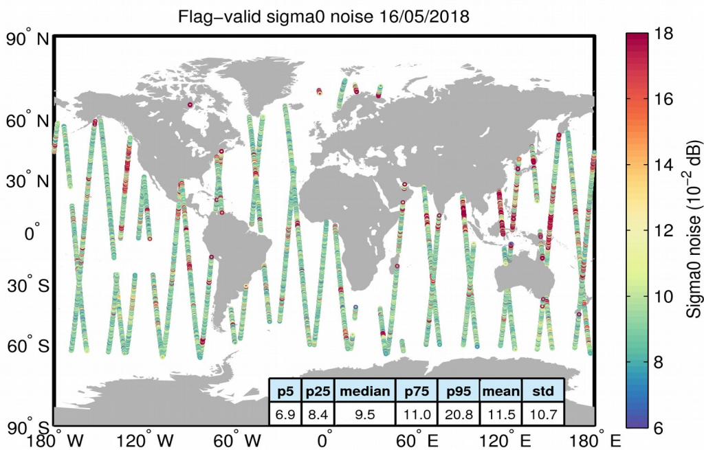
Figure 26. Geographical distribution of flag-valid 20-Hz sigma0 measurement noise over oceans and lakes for 16/05/2018. The statistical values shown in the table refer to the sigma0 noise and are calculated over all measurements shown in the figure.
