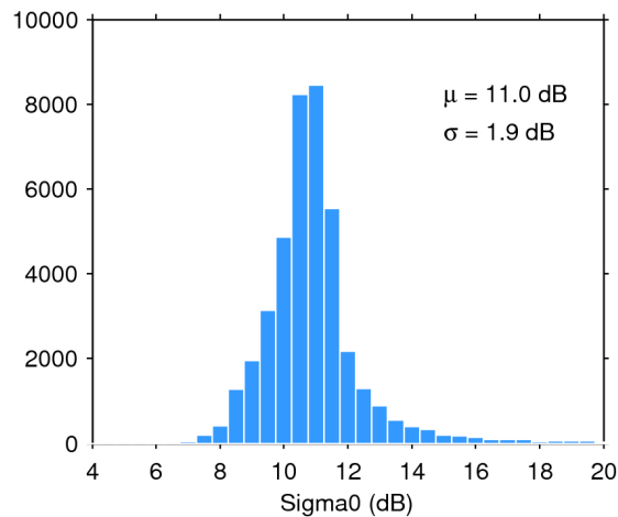
Figure 25. Histogram of flag-valid sigma0 over oceans and lakes for 16/05/2018. The mean ( \mu ) and standard deviation ( \sigma ) are also shown. Note that values outside [4 20] dB are excluded from the histogram for the sake of readability but not from the computation of \mu and \sigma .
