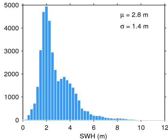
Figure 20. Histogram of science-valid SWH over oceans and lakes for 16/05/2018. The mean ( \mu ) and standard deviation ( \sigma ) are also shown. Note that values larger than 12 m are excluded from the histogram for the sake of readability but not from the computation of \mu and \sigma .
