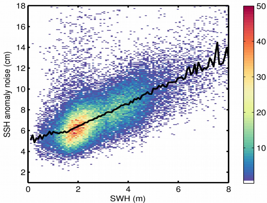
Figure 9. 2D histogram showing flag-valid SSH anomaly noise as a function of SWH for 16/05/2018. The black line denotes the median SSH anomaly noise as a function of SWH.
