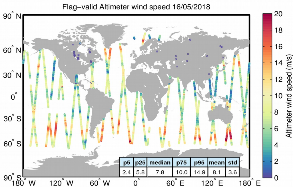
Figure 31. Geographical distribution of flag-valid wind data over oceans and lakes for 16/05/2018. The statistical values shown in the table refer to the wind in m/s and are calculated over all measurements shown in the figure.
