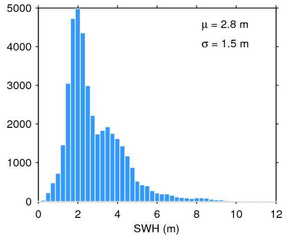
Figure 17. Histogram of flag-valid SWH over oceans and lakes for 16/05/2018. The mean ( \mu ) and standard deviation ( \sigma ) are also shown. Note that values larger than 12 m are excluded from the histogram for the sake of readability but not from the computation of \mu and \sigma .
