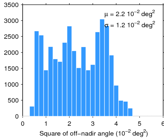
Figure 39. Histogram of flag-valid mispointing over oceans and lakes for 16/05/2018. The mean ( \mu ) and standard deviation ( \sigma ) are also shown. Note that values larger than 6 \cdot 10^{-2} \text{ deg}^2 are excluded from the histogram for the sake of readability but not from the computation of \mu and \sigma .
