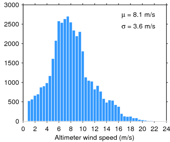
Figure 33. Histogram of flag-valid wind over oceans and lakes for 16/05/2018. The mean ( \mu ) and standard deviation ( \sigma ) are also shown. Note that values larger than 24 m/s are excluded from the histogram for the sake of readability but not from the computation of \mu and \sigma .
