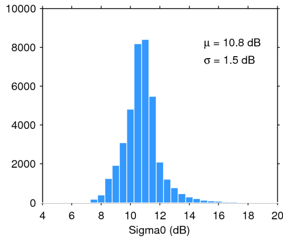
Figure 28. Histogram of science-valid sigma0 over oceans and lakes for 16/05/2018. The mean ( \mu ) and standard deviation ( \sigma ) are also shown. Note that values outside [4 20] dB are excluded from the histogram for the sake of readability but not from the computation of \mu and \sigma .
