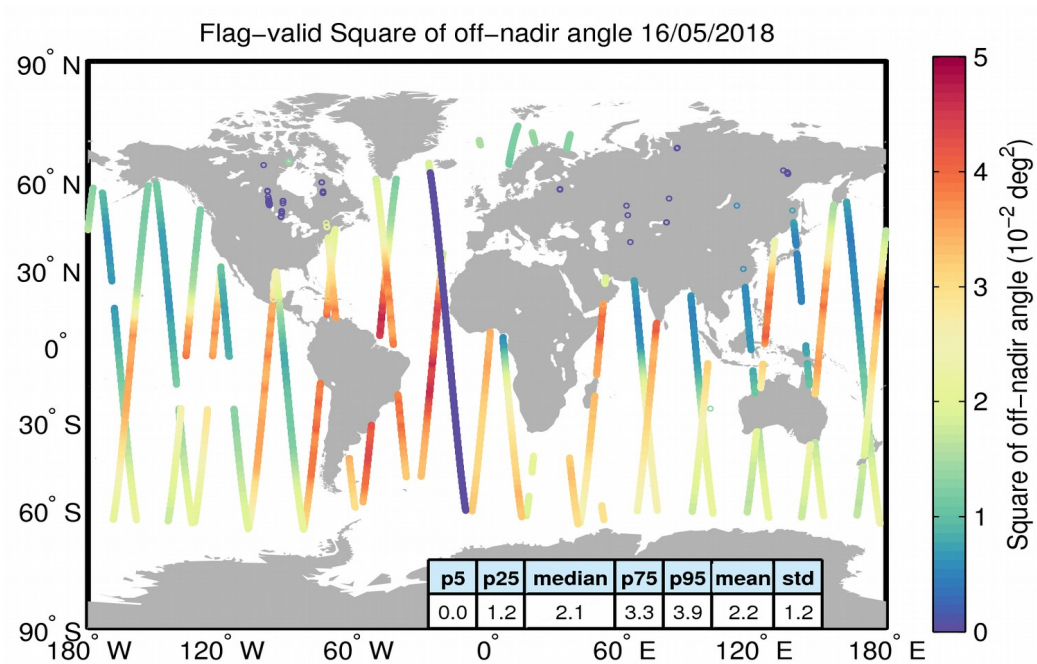
Figure 37. Geographical distribution of flag-valid mispointing data over oceans and lakes for 16/05/2018. The statistical values shown in the table refer to the mispointing in 10^{-2} \text{ deg}^2 and are calculated over all measurements shown in the figure.
