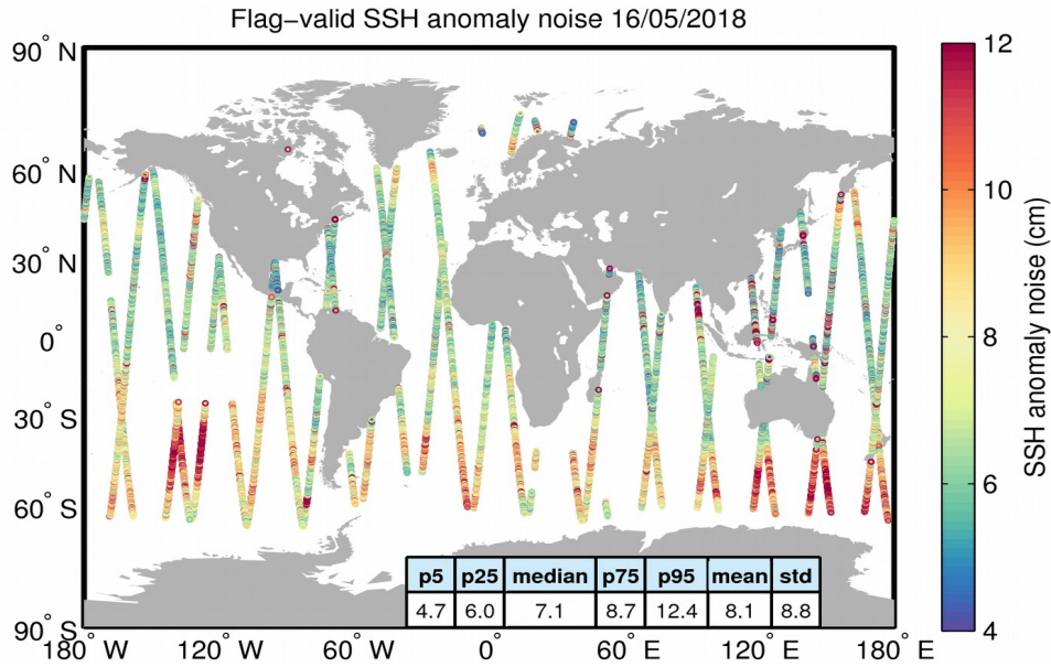
Figure 8. Geographical distribution of flag-valid 20-Hz SSH anomaly measurement noise over oceans and lakes for 16/05/2018. The statistical values shown in the table refer to the SSH anomaly noise and are calculated over all measurements shown in the figure.
