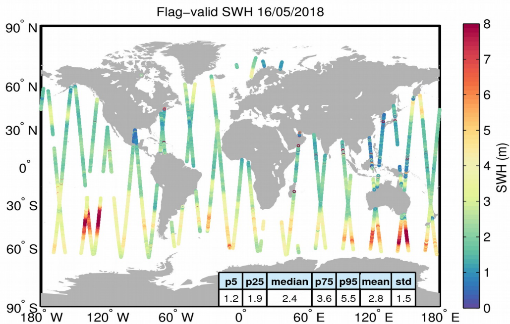
Figure 15. Geographical distribution of flag-valid SWH data over oceans and lakes for 16/05/2018. The statistical values shown in the table refer to the SWH in m and are calculated over all measurements shown in the figure.
