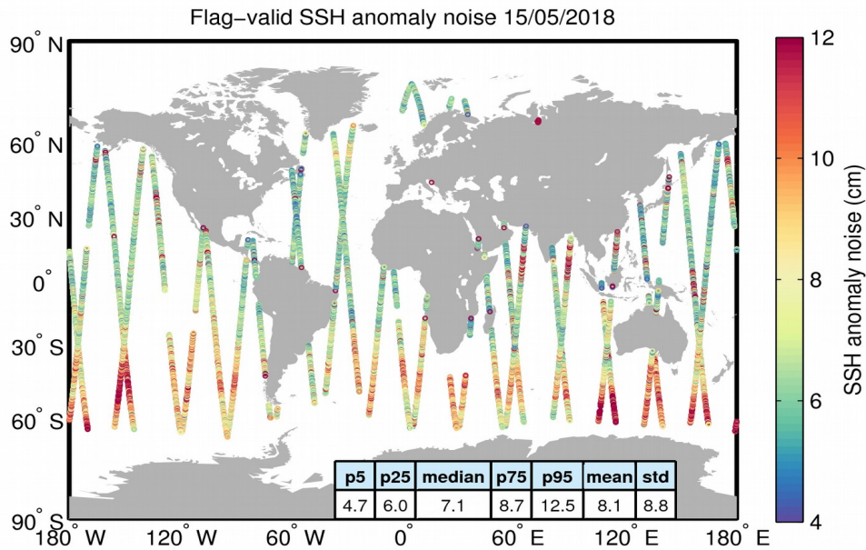
Figure 8. Geographical distribution of flag-valid 20-Hz SSH anomaly measurement noise over oceans and lakes for 15/05/2018. The statistical values shown in the table refer to the SSH anomaly noise and are calculated over all measurements shown in the figure.
