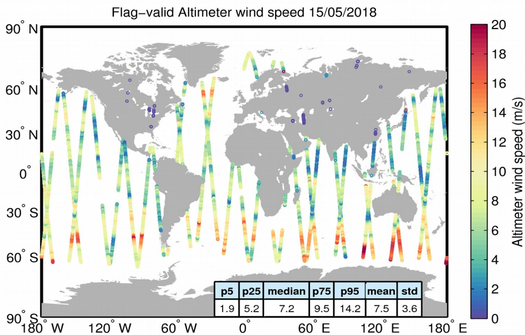
Figure 31. Geographical distribution of flag-valid wind data over oceans and lakes for 15/05/2018. The statistical values shown in the table refer to the wind in m/s and are calculated over all measurements shown in the figure.
