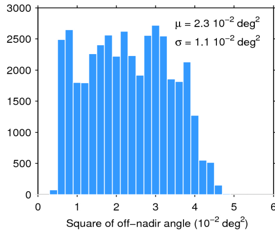
Figure 39. Histogram of flag-valid mispointing over oceans and lakes for 15/05/2018. The mean ( \mu ) and standard deviation ( \sigma ) are also shown. Note that values larger than 6 \cdot 10^{-2} \text{ deg}^2 are excluded from the histogram for the sake of readability but not from the computation of \mu and \sigma .
