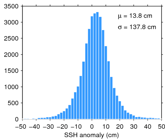
Figure 7. Histogram of flag-valid SSH anomaly over oceans and lakes for 15/05/2018. The mean ( \mu ) and standard deviation ( \sigma ) are also shown. Note that values outside [-50\ 50] cm are excluded from the histogram for the sake of readability but not from the computation of \mu and \sigma .
