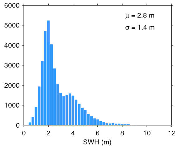
Figure 20. Histogram of science-valid SWH over oceans and lakes for 15/05/2018. The mean ( \mu ) and standard deviation ( \sigma ) are also shown. Note that values larger than 12 m are excluded from the histogram for the sake of readability but not from the computation of \mu and \sigma .
