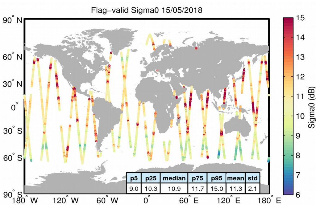
Figure 23. Geographical distribution of flag-valid sigma0 data over oceans and lakes for 15/05/2018. The statistical values shown in the table refer to the sigma0 in dB and are calculated over all measurements shown in the figure.
