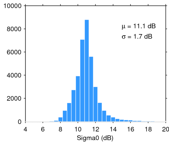
Figure 28. Histogram of science-valid sigma0 over oceans and lakes for 15/05/2018. The mean ( \mu ) and standard deviation ( \sigma ) are also shown. Note that values outside [4 20] dB are excluded from the histogram for the sake of readability but not from the computation of \mu and \sigma .
