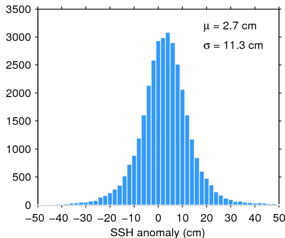
Figure 11. Histogram of science-valid SSH anomaly over oceans and lakes for 15/05/2018. The mean ( \mu ) and standard deviation ( \sigma ) are also shown. Note that values outside [-50 50] cm are excluded from the histogram for the sake of readability but not from the computation of \mu and \sigma .
