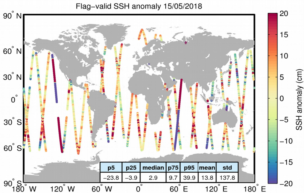
Figure 5. Geographical distribution of flag-valid 1-Hz SSH anomaly data over oceans and lakes for 15/05/2018. The statistical values shown in the table refer to the SSH anomaly in cm and are calculated over all measurements shown in the figure.
