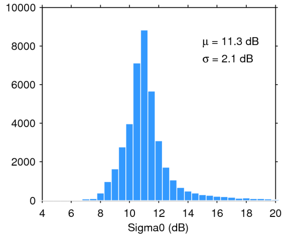
Figure 25. Histogram of flag-valid sigma0 over oceans and lakes for 15/05/2018. The mean ( \mu ) and standard deviation ( \sigma ) are also shown. Note that values outside [4 20] dB are excluded from the histogram for the sake of readability but not from the computation of \mu and \sigma .
