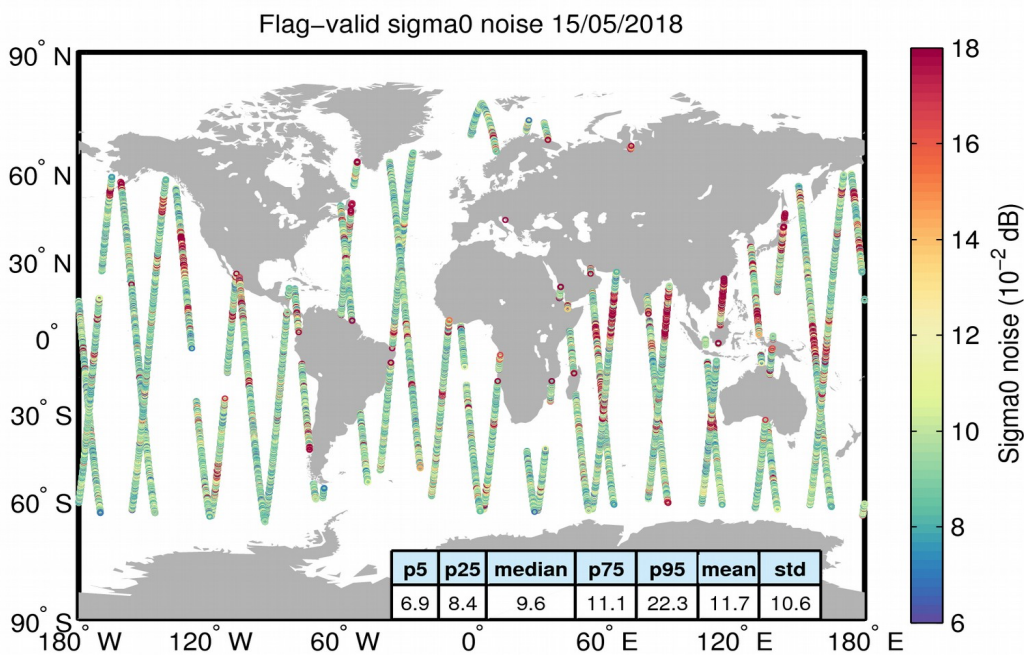
Figure 26. Geographical distribution of flag-valid 20-Hz sigma0 measurement noise over oceans and lakes for 15/05/2018. The statistical values shown in the table refer to the sigma0 noise and are calculated over all measurements shown in the figure.
