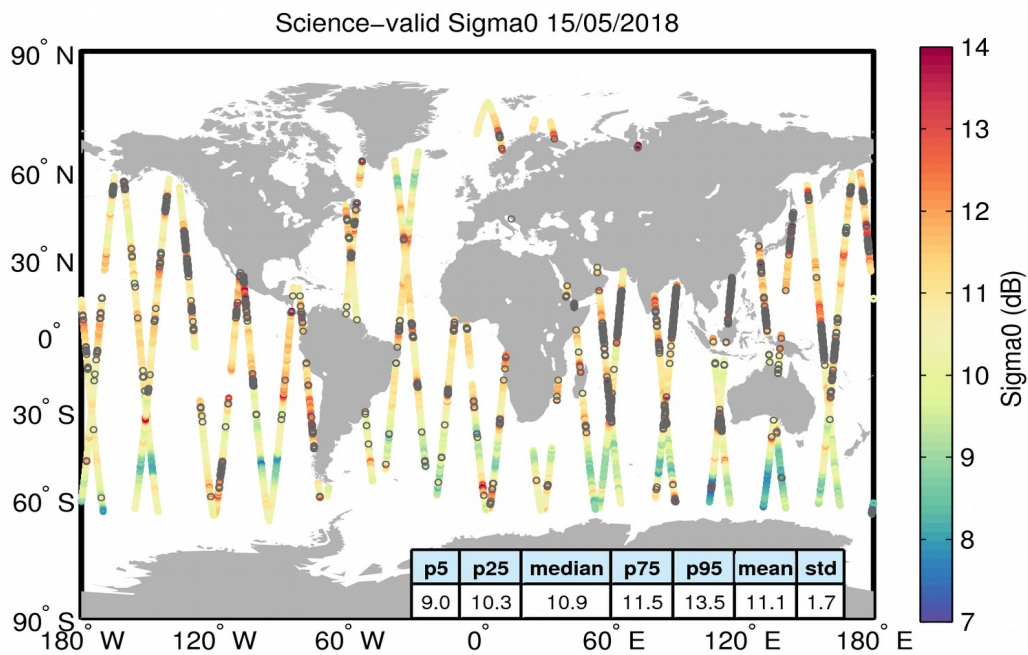
Figure 27. Geographical distribution of science-valid sigma0 data over oceans and lakes for 15/05/2018. The statistical values shown in the table refer to the sigma0 in dB and are calculated over all measurements shown in the figure. Gray circles denote records that have been rejected based on the editing criteria described in Table 4.
