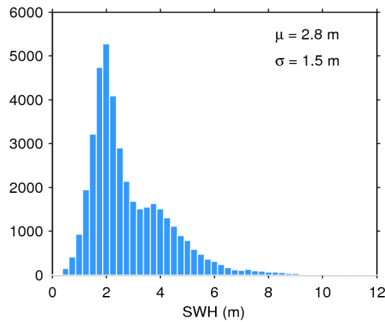
Figure 17. Histogram of flag-valid SWH over oceans and lakes for 15/05/2018. The mean ( \mu ) and standard deviation ( \sigma ) are also shown. Note that values larger than 12 m are excluded from the histogram for the sake of readability but not from the computation of \mu and \sigma .
