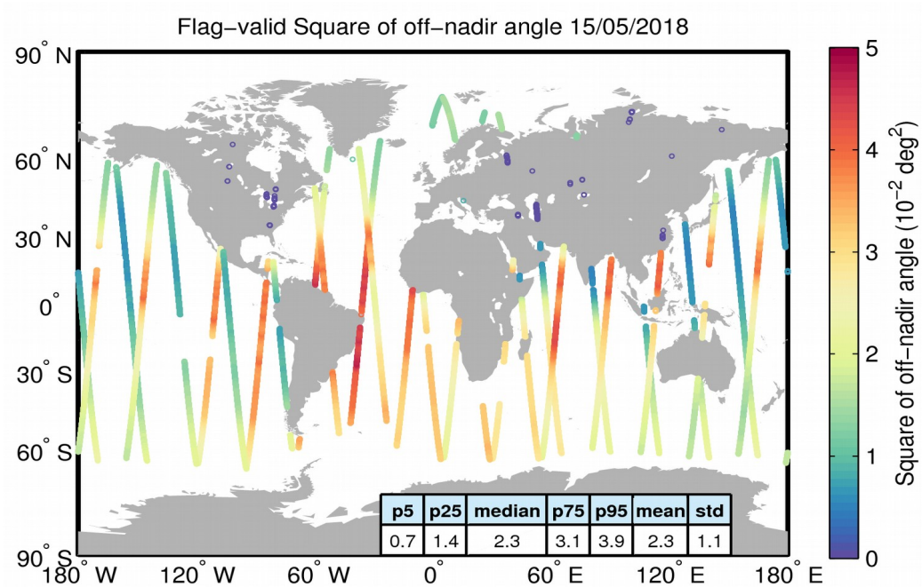
Figure 37. Geographical distribution of flag-valid mispointing data over oceans and lakes for 15/05/2018. The statistical values shown in the table refer to the mispointing in 10^{-2} \text{ deg}^2 and are calculated over all measurements shown in the figure.
