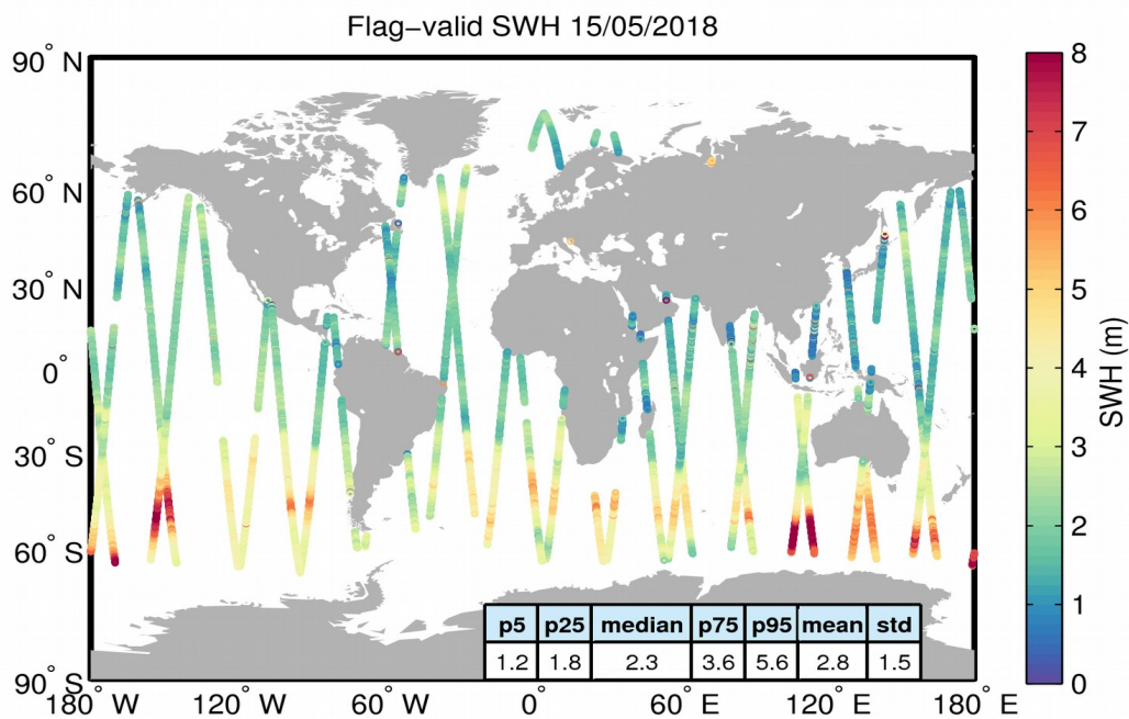
Figure 15. Geographical distribution of flag-valid SWH data over oceans and lakes for 15/05/2018. The statistical values shown in the table refer to the SWH in m and are calculated over all measurements shown in the figure.
