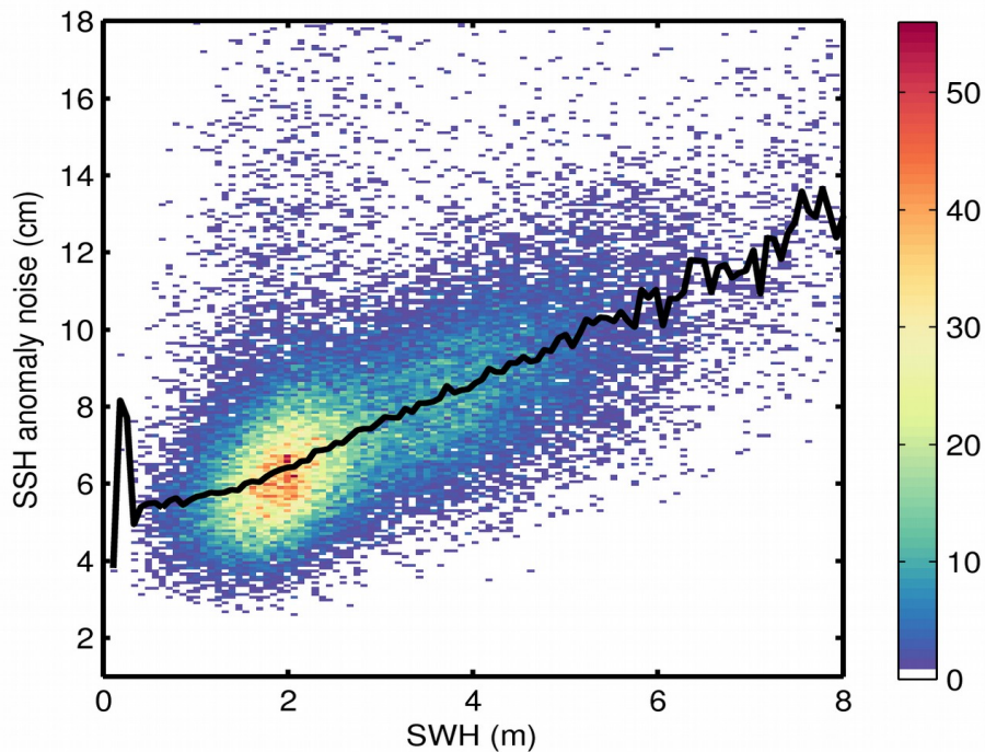
Figure 9. 2D histogram showing flag-valid SSH anomaly noise as a function of SWH for 15/05/2018. The black line denotes the median SSH anomaly noise as a function of SWH.
