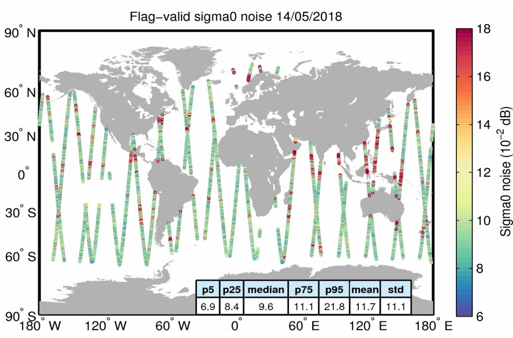
Figure 26. Geographical distribution of flag-valid 20-Hz sigma0 measurement noise over oceans and lakes for 14/05/2018. The statistical values shown in the table refer to the sigma0 noise and are calculated over all measurements shown in the figure.
