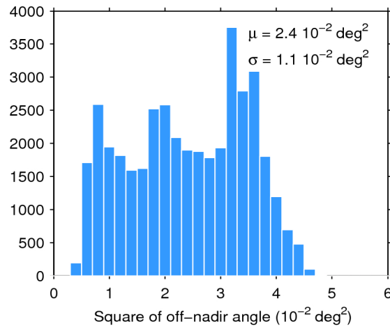
Figure 39. Histogram of flag-valid mispointing over oceans and lakes for 14/05/2018. The mean ( \mu ) and standard deviation ( \sigma ) are also shown. Note that values larger than 6 \cdot 10^{-2} \text{ deg}^2 are excluded from the histogram for the sake of readability but not from the computation of \mu and \sigma .
