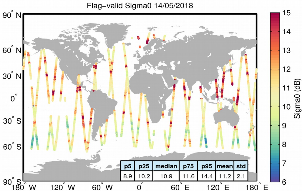
Figure 23. Geographical distribution of flag-valid sigma0 data over oceans and lakes for 14/05/2018. The statistical values shown in the table refer to the sigma0 in dB and are calculated over all measurements shown in the figure.
