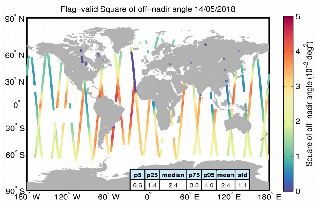
Figure 37. Geographical distribution of flag-valid mispointing data over oceans and lakes for 14/05/2018. The statistical values shown in the table refer to the mispointing in 10^{-2} deg 2 and are calculated over all measurements shown in the figure.
