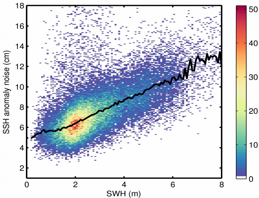
Figure 9. 2D histogram showing flag-valid SSH anomaly noise as a function of SWH for 14/05/2018. The black line denotes the median SSH anomaly noise as a function of SWH.
