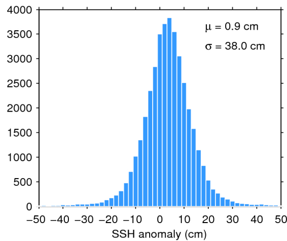
Figure 7. Histogram of flag-valid SSH anomaly over oceans and lakes for 14/05/2018. The mean ( \mu ) and standard deviation ( \sigma ) are also shown. Note that values outside [-50 50] cm are excluded from the histogram for the sake of readability but not from the computation of \mu and \sigma .
