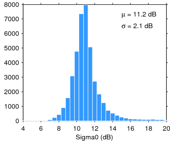
Figure 25. Histogram of flag-valid sigma0 over oceans and lakes for 14/05/2018. The mean ( \mu ) and standard deviation ( \sigma ) are also shown. Note that values outside [4 20] dB are excluded from the histogram for the sake of readability but not from the computation of \mu and \sigma .
