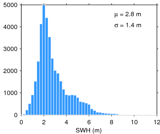
Figure 20. Histogram of science-valid SWH over oceans and lakes for 14/05/2018. The mean ( \mu ) and standard deviation ( \sigma ) are also shown. Note that values larger than 12 m are excluded from the histogram for the sake of readability but not from the computation of \mu and \sigma .
