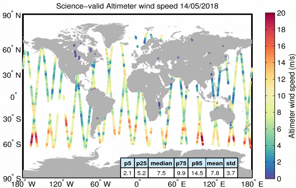
Figure 34. Geographical distribution of science-valid wind data over oceans and lakes for 14/05/2018. The statistical values shown in the table refer to the wind in m/s and are calculated over all measurements shown in the figure. Gray circles denote records that have been rejected based on the editing criteria described in Table 5.
