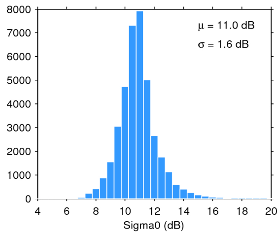
Figure 28. Histogram of science-valid sigma0 over oceans and lakes for 14/05/2018. The mean ( \mu ) and standard deviation ( \sigma ) are also shown. Note that values outside [4 20] dB are excluded from the histogram for the sake of readability but not from the computation of \mu and \sigma .
