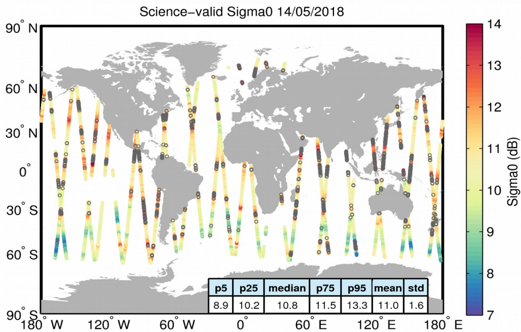
Figure 27. Geographical distribution of science-valid sigma0 data over oceans and lakes for 14/05/2018. The statistical values shown in the table refer to the sigma0 in dB and are calculated over all measurements shown in the figure. Gray circles denote records that have been rejected based on the editing criteria described in Table 4.
