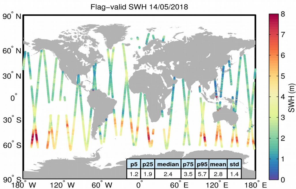
Figure 15. Geographical distribution of flag-valid SWH data over oceans and lakes for 14/05/2018. The statistical values shown in the table refer to the SWH in m and are calculated over all measurements shown in the figure.
