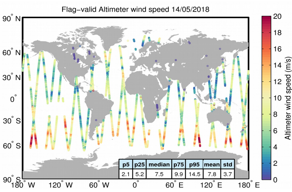
Figure 31. Geographical distribution of flag-valid wind data over oceans and lakes for 14/05/2018. The statistical values shown in the table refer to the wind in m/s and are calculated over all measurements shown in the figure.
