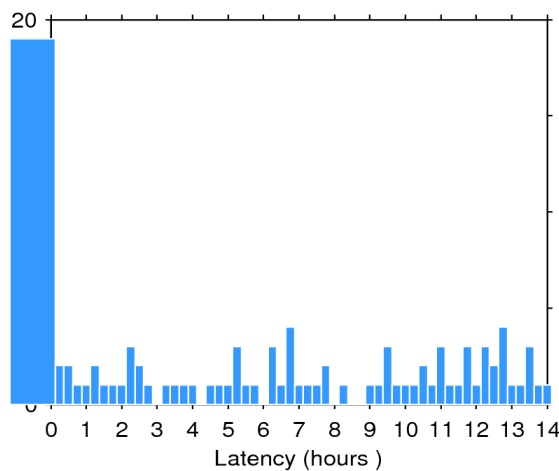
Figure 2. Histogram of the data latency for 14/05/2018. The y-axis denotes the number of files that are made available with a delay of x-hours with respect to the mean time of the records stored in the file.
