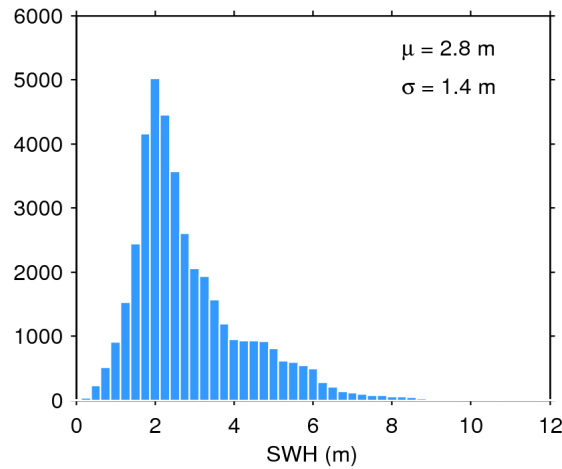
Figure 17. Histogram of flag-valid SWH over oceans and lakes for 14/05/2018. The mean ( \mu ) and standard deviation ( \sigma ) are also shown. Note that values larger than 12 m are excluded from the histogram for the sake of readability but not from the computation of \mu and \sigma .
