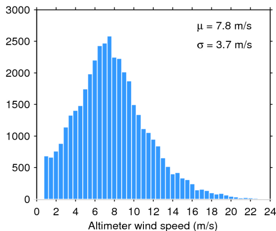
Figure 35. Histogram of science-valid wind over oceans and lakes for 14/05/2018. The mean ( \mu ) and standard deviation ( \sigma ) are also shown. Note that values larger than 24 m/s are excluded from the histogram for the sake of readability but not from the computation of \mu and \sigma .
