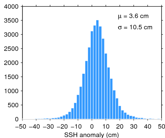
Figure 11. Histogram of science-valid SSH anomaly over oceans and lakes for 14/05/2018. The mean ( \mu ) and standard deviation ( \sigma ) are also shown. Note that values outside [-50 50] cm are excluded from the histogram for the sake of readability but not from the computation of \mu and \sigma .
