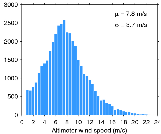
Figure 33. Histogram of flag-valid wind over oceans and lakes for 14/05/2018. The mean ( \mu ) and standard deviation ( \sigma ) are also shown. Note that values larger than 24 m/s are excluded from the histogram for the sake of readability but not from the computation of \mu and \sigma .
