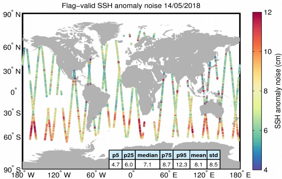
Figure 8. Geographical distribution of flag-valid 20-Hz SSH anomaly measurement noise over oceans and lakes for 14/05/2018. The statistical values shown in the table refer to the SSH anomaly noise and are calculated over all measurements shown in the figure.
