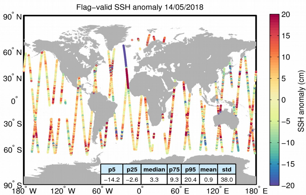
Figure 5. Geographical distribution of flag-valid 1-Hz SSH anomaly data over oceans and lakes for 14/05/2018. The statistical values shown in the table refer to the SSH anomaly in cm and are calculated over all measurements shown in the figure.
