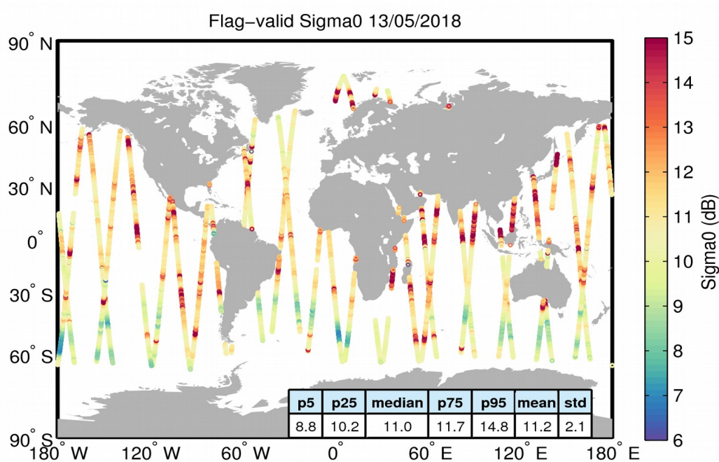
Figure 23. Geographical distribution of flag-valid sigma0 data over oceans and lakes for 13/05/2018. The statistical values shown in the table refer to the sigma0 in dB and are calculated over all measurements shown in the figure.
