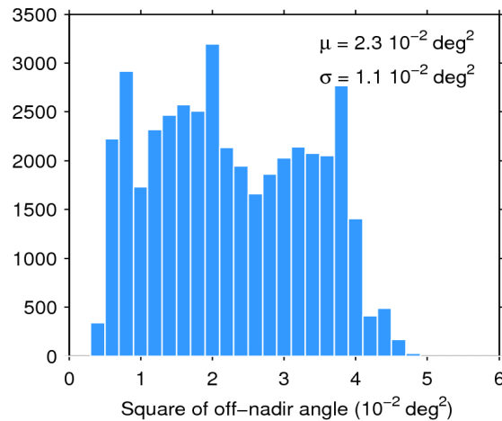
Figure 39. Histogram of flag-valid mispointing over oceans and lakes for 13/05/2018. The mean ( \mu ) and standard deviation ( \sigma ) are also shown. Note that values larger than 6 \cdot 10^{-2} \text{ deg}^2 are excluded from the histogram for the sake of readability but not from the computation of \mu and \sigma .
