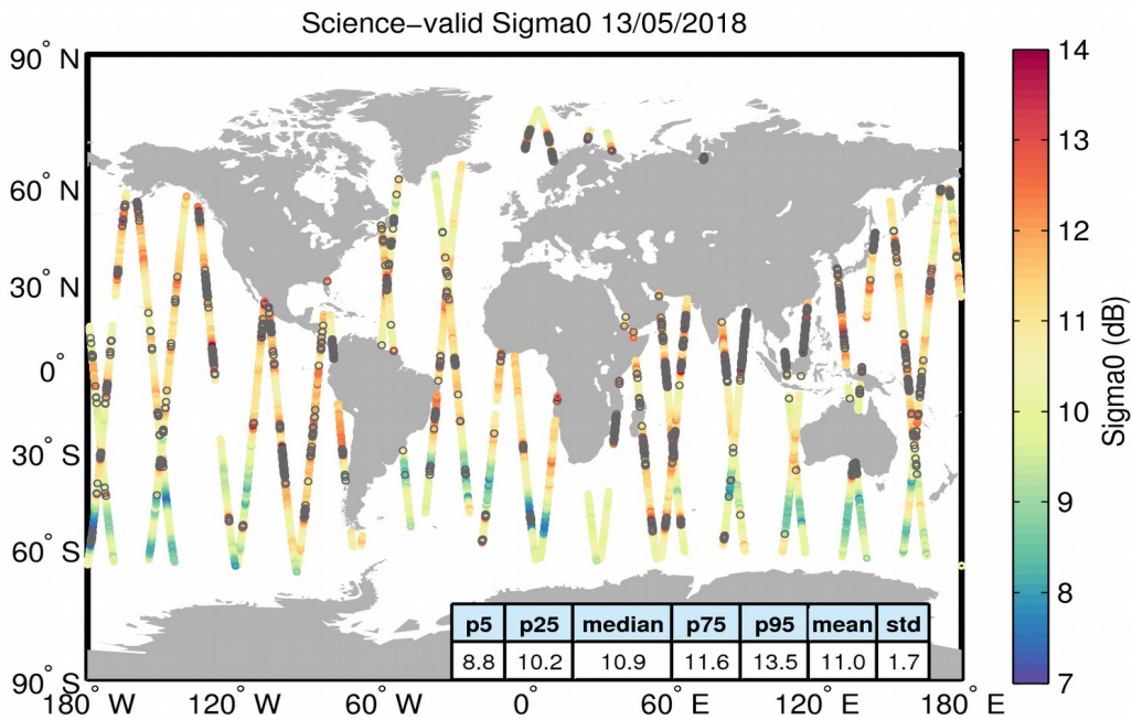
Figure 27. Geographical distribution of science-valid sigma0 data over oceans and lakes for 13/05/2018. The statistical values shown in the table refer to the sigma0 in dB and are calculated over all measurements shown in the figure. Gray circles denote records that have been rejected based on the editing criteria described in Table 4.
