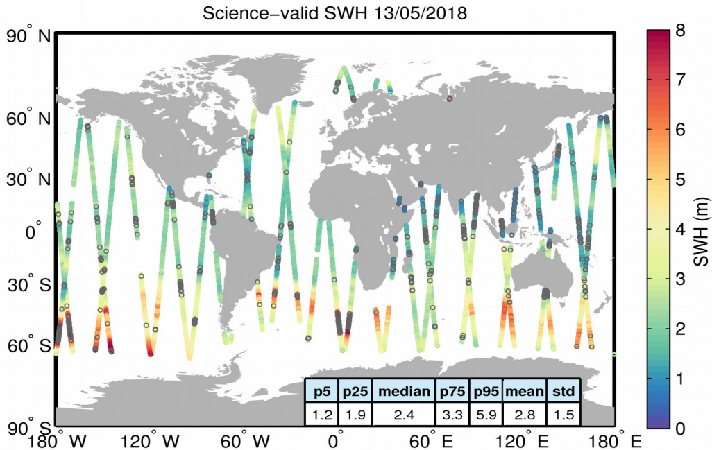
Figure 19. Geographical distribution of science-valid SWH data over oceans and lakes for 13/05/2018. The statistical values shown in the table refer to the SWH in m and are calculated over all measurements shown in the figure. Gray circles denote records that have been rejected based on the editing criteria described in Table 3.
