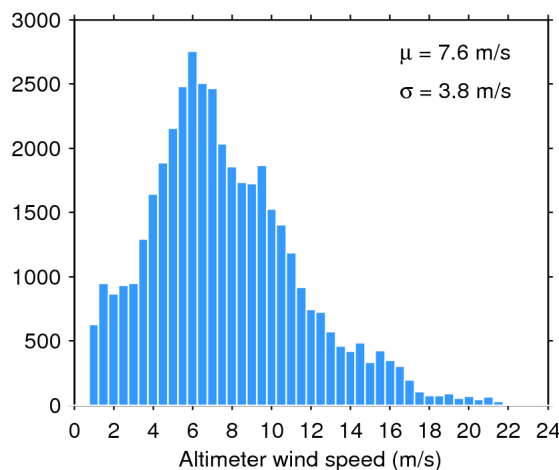
Figure 35. Histogram of science-valid wind over oceans and lakes for 13/05/2018. The mean ( \mu ) and standard deviation ( \sigma ) are also shown. Note that values larger than 24 m/s are excluded from the histogram for the sake of readability but not from the computation of \mu and \sigma .
