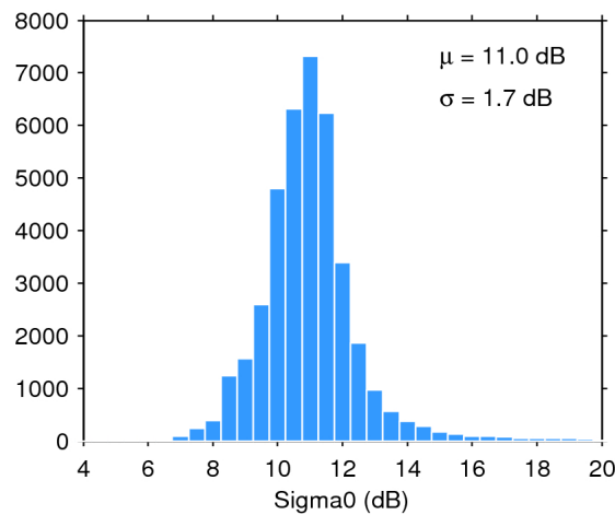
Figure 28. Histogram of science-valid sigma0 over oceans and lakes for 13/05/2018. The mean ( \mu ) and standard deviation ( \sigma ) are also shown. Note that values outside [4 20] dB are excluded from the histogram for the sake of readability but not from the computation of \mu and \sigma .
