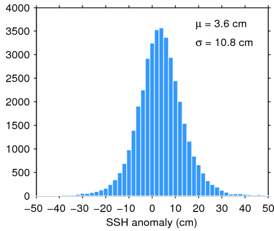
Figure 11. Histogram of science-valid SSH anomaly over oceans and lakes for 13/05/2018. The mean ( \mu ) and standard deviation ( \sigma ) are also shown. Note that values outside [-50 50] cm are excluded from the histogram for the sake of readability but not from the computation of \mu and \sigma .
