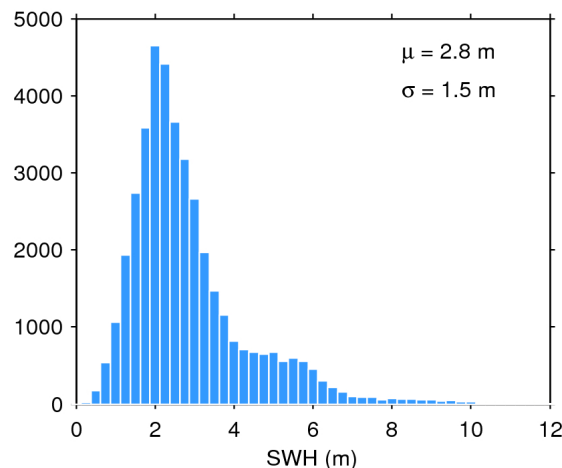
Figure 20. Histogram of science-valid SWH over oceans and lakes for 13/05/2018. The mean ( \mu ) and standard deviation ( \sigma ) are also shown. Note that values larger than 12 m are excluded from the histogram for the sake of readability but not from the computation of \mu and \sigma .
