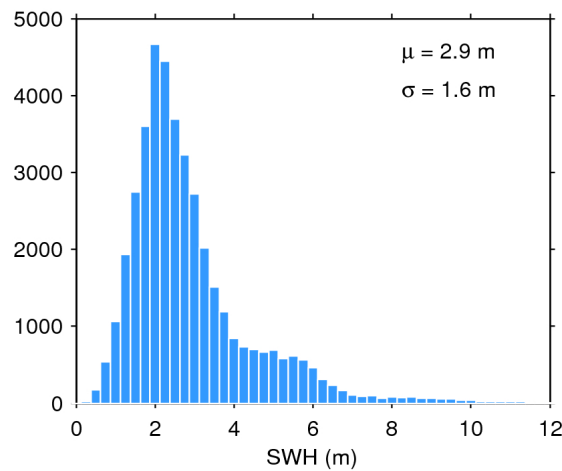
Figure 17. Histogram of flag-valid SWH over oceans and lakes for 13/05/2018. The mean ( \mu ) and standard deviation ( \sigma ) are also shown. Note that values larger than 12 m are excluded from the histogram for the sake of readability but not from the computation of \mu and \sigma .
