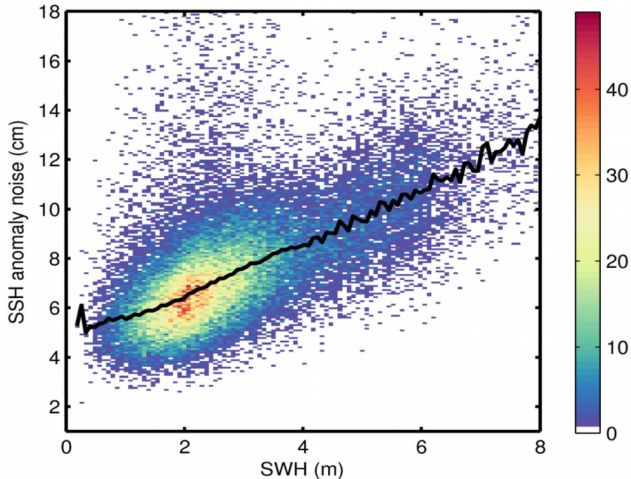
Figure 9. 2D histogram showing flag-valid SSH anomaly noise as a function of SWH for 13/05/2018. The black line denotes the median SSH anomaly noise as a function of SWH.
