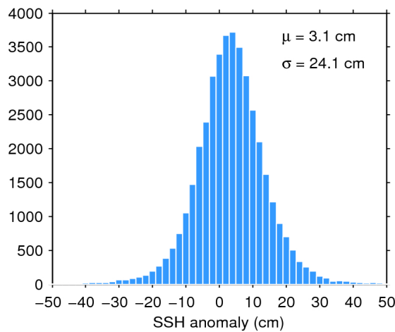
Figure 7. Histogram of flag-valid SSH anomaly over oceans and lakes for 13/05/2018. The mean ( \mu ) and standard deviation ( \sigma ) are also shown. Note that values outside [-50 50] cm are excluded from the histogram for the sake of readability but not from the computation of \mu and \sigma .
