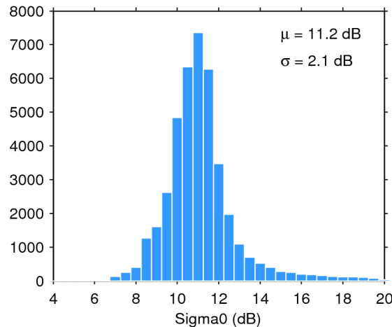
Figure 25. Histogram of flag-valid sigma0 over oceans and lakes for 13/05/2018. The mean ( \mu ) and standard deviation ( \sigma ) are also shown. Note that values outside [4 20] dB are excluded from the histogram for the sake of readability but not from the computation of \mu and \sigma .
