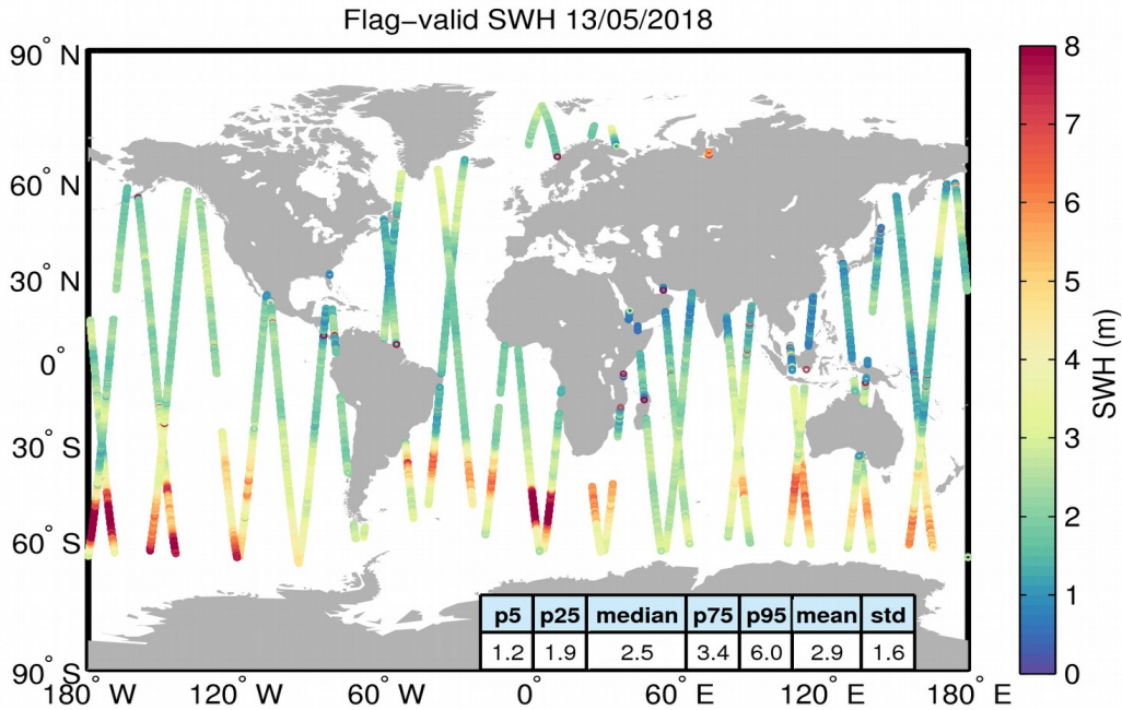
Figure 15. Geographical distribution of flag-valid SWH data over oceans and lakes for 13/05/2018. The statistical values shown in the table refer to the SWH in m and are calculated over all measurements shown in the figure.
