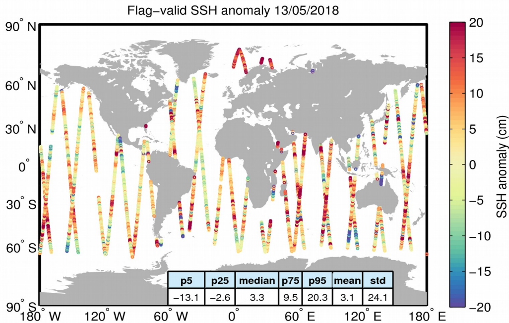
Figure 5. Geographical distribution of flag-valid 1-Hz SSH anomaly data over oceans and lakes for 13/05/2018. The statistical values shown in the table refer to the SSH anomaly in cm and are calculated over all measurements shown in the figure.
