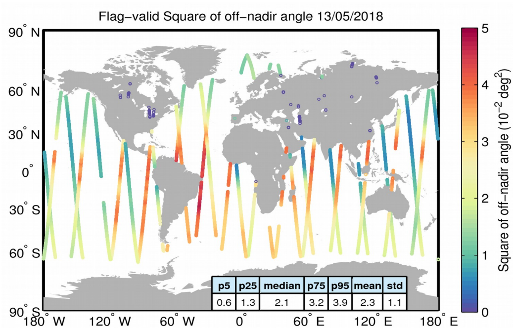
Figure 37. Geographical distribution of flag-valid mispointing data over oceans and lakes for 13/05/2018. The statistical values shown in the table refer to the mispointing in 10^{-2} deg 2 and are calculated over all measurements shown in the figure.
