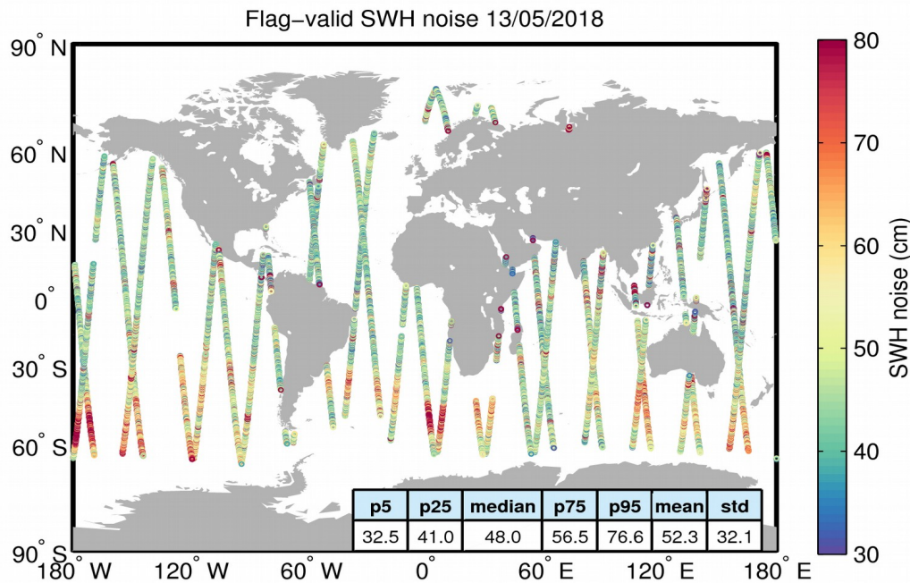
Figure 18. Geographical distribution of flag-valid 20-Hz SWH measurement noise over oceans and lakes for 13/05/2018. The statistical values shown in the table refer to the SWH noise and are calculated over all measurements shown in the figure.
