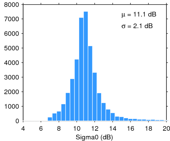
Figure 25. Histogram of flag-valid sigma0 over oceans and lakes for 12/05/2018. The mean ( \mu ) and standard deviation ( \sigma ) are also shown. Note that values outside [4 20] dB are excluded from the histogram for the sake of readability but not from the computation of \mu and \sigma .
