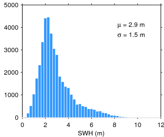
Figure 20. Histogram of science-valid SWH over oceans and lakes for 12/05/2018. The mean ( \mu ) and standard deviation ( \sigma ) are also shown. Note that values larger than 12 m are excluded from the histogram for the sake of readability but not from the computation of \mu and \sigma .
