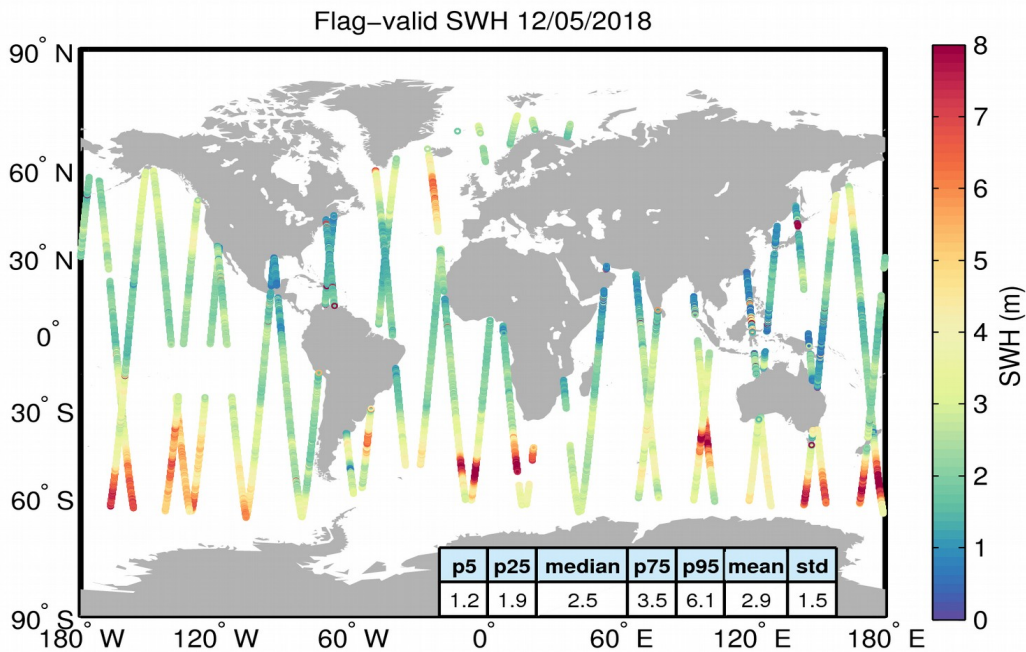
Figure 15. Geographical distribution of flag-valid SWH data over oceans and lakes for 12/05/2018. The statistical values shown in the table refer to the SWH in m and are calculated over all measurements shown in the figure.
