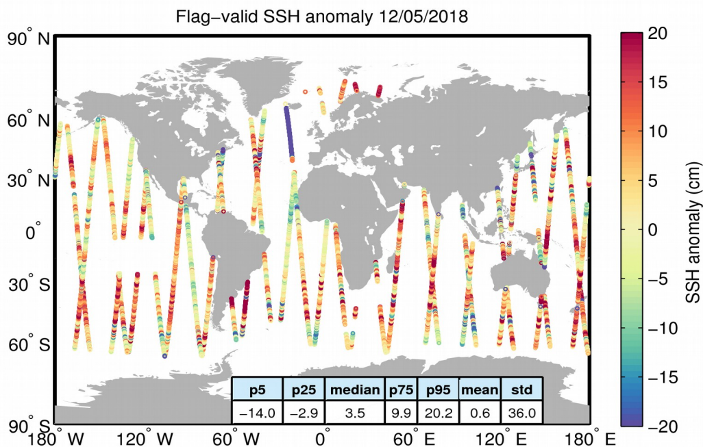
Figure 5. Geographical distribution of flag-valid 1-Hz SSH anomaly data over oceans and lakes for 12/05/2018. The statistical values shown in the table refer to the SSH anomaly in cm and are calculated over all measurements shown in the figure.
