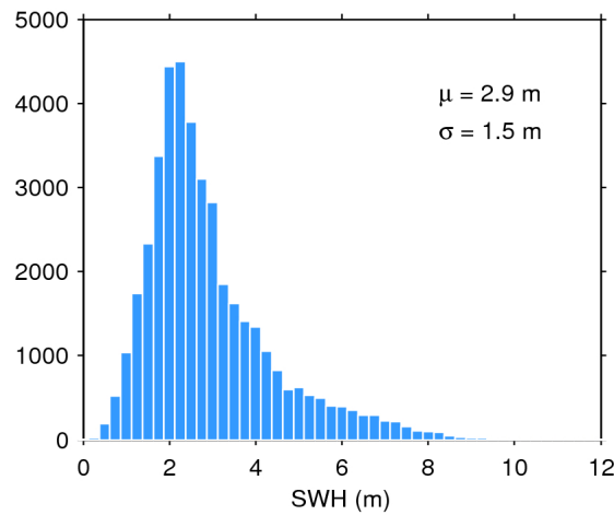
Figure 17. Histogram of flag-valid SWH over oceans and lakes for 12/05/2018. The mean ( \mu ) and standard deviation ( \sigma ) are also shown. Note that values larger than 12 m are excluded from the histogram for the sake of readability but not from the computation of \mu and \sigma .
