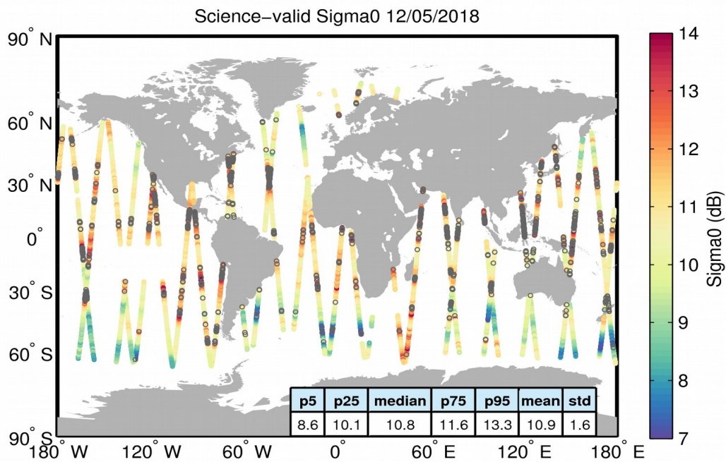
Figure 27. Geographical distribution of science-valid sigma0 data over oceans and lakes for 12/05/2018. The statistical values shown in the table refer to the sigma0 in dB and are calculated over all measurements shown in the figure. Gray circles denote records that have been rejected based on the editing criteria described in Table 4.
