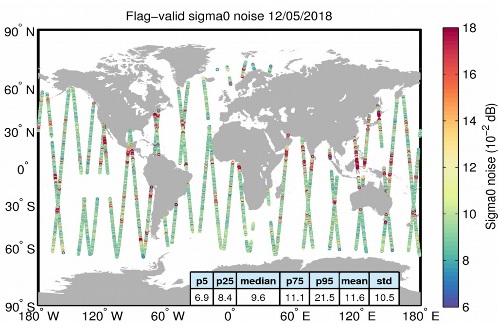
Figure 26. Geographical distribution of flag-valid 20-Hz sigma0 measurement noise over oceans and lakes for 12/05/2018. The statistical values shown in the table refer to the sigma0 noise and are calculated over all measurements shown in the figure.
