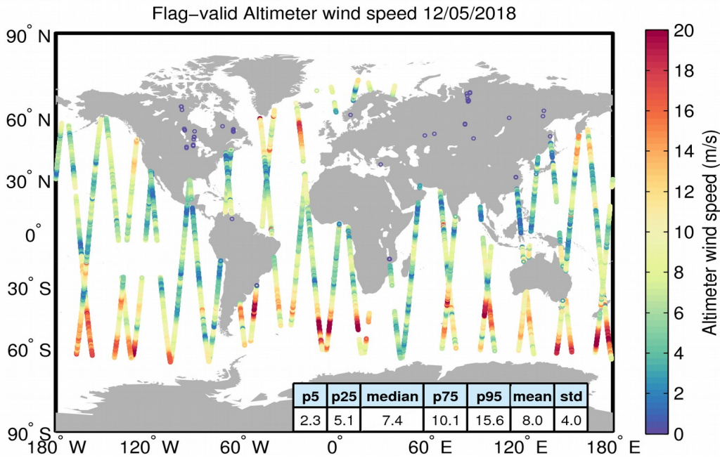
Figure 31. Geographical distribution of flag-valid wind data over oceans and lakes for 12/05/2018. The statistical values shown in the table refer to the wind in m/s and are calculated over all measurements shown in the figure.
