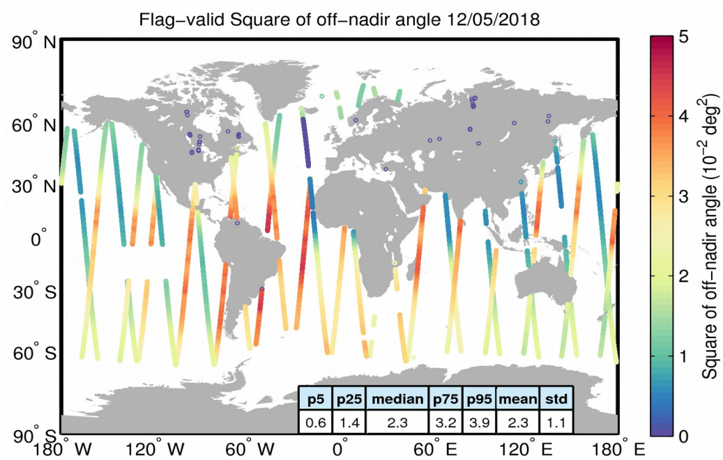
Figure 37. Geographical distribution of flag-valid mispointing data over oceans and lakes for 12/05/2018. The statistical values shown in the table refer to the mispointing in 10^{-2} \text{ deg}^2 and are calculated over all measurements shown in the figure.
