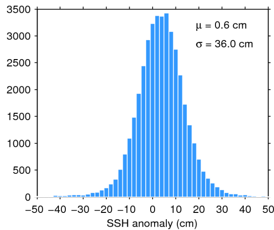
Figure 7. Histogram of flag-valid SSH anomaly over oceans and lakes for 12/05/2018. The mean ( \mu ) and standard deviation ( \sigma ) are also shown. Note that values outside [-50 50] cm are excluded from the histogram for the sake of readability but not from the computation of \mu and \sigma .
