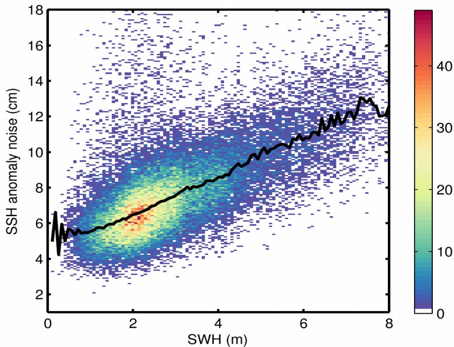
Figure 9. 2D histogram showing flag-valid SSH anomaly noise as a function of SWH for 12/05/2018. The black line denotes the median SSH anomaly noise as a function of SWH.
