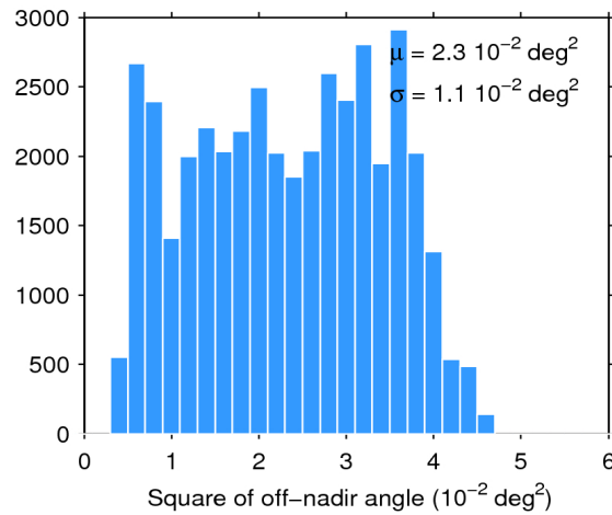
Figure 39. Histogram of flag-valid mispointing over oceans and lakes for 12/05/2018. The mean ( \mu ) and standard deviation ( \sigma ) are also shown. Note that values larger than 6 \cdot 10^{-2} \text{ deg}^2 are excluded from the histogram for the sake of readability but not from the computation of \mu and \sigma .
