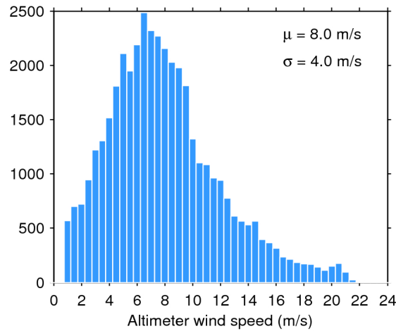
Figure 33. Histogram of flag-valid wind over oceans and lakes for 12/05/2018. The mean ( \mu ) and standard deviation ( \sigma ) are also shown. Note that values larger than 24 m/s are excluded from the histogram for the sake of readability but not from the computation of \mu and \sigma .
