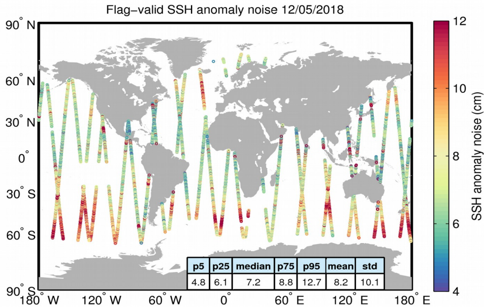
Figure 8. Geographical distribution of flag-valid 20-Hz SSH anomaly measurement noise over oceans and lakes for 12/05/2018. The statistical values shown in the table refer to the SSH anomaly noise and are calculated over all measurements shown in the figure.
