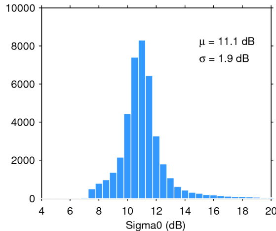
Figure 25. Histogram of flag-valid sigma0 over oceans and lakes for 11/05/2018. The mean ( \mu ) and standard deviation ( \sigma ) are also shown. Note that values outside [4 20] dB are excluded from the histogram for the sake of readability but not from the computation of \mu and \sigma .
