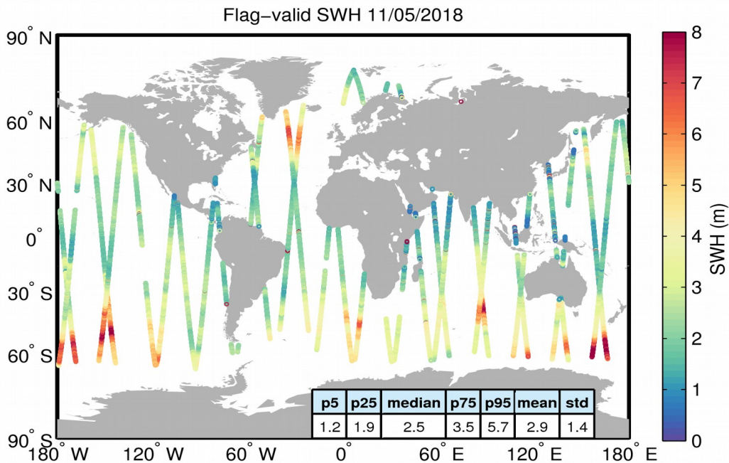
Figure 15. Geographical distribution of flag-valid SWH data over oceans and lakes for 11/05/2018. The statistical values shown in the table refer to the SWH in m and are calculated over all measurements shown in the figure.
