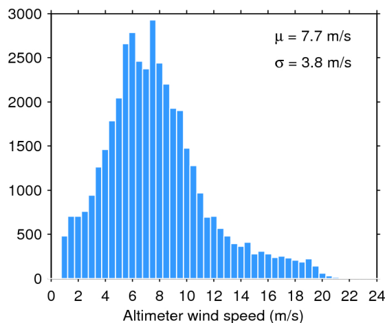
Figure 35. Histogram of science-valid wind over oceans and lakes for 11/05/2018. The mean ( \mu ) and standard deviation ( \sigma ) are also shown. Note that values larger than 24 m/s are excluded from the histogram for the sake of readability but not from the computation of \mu and \sigma .
