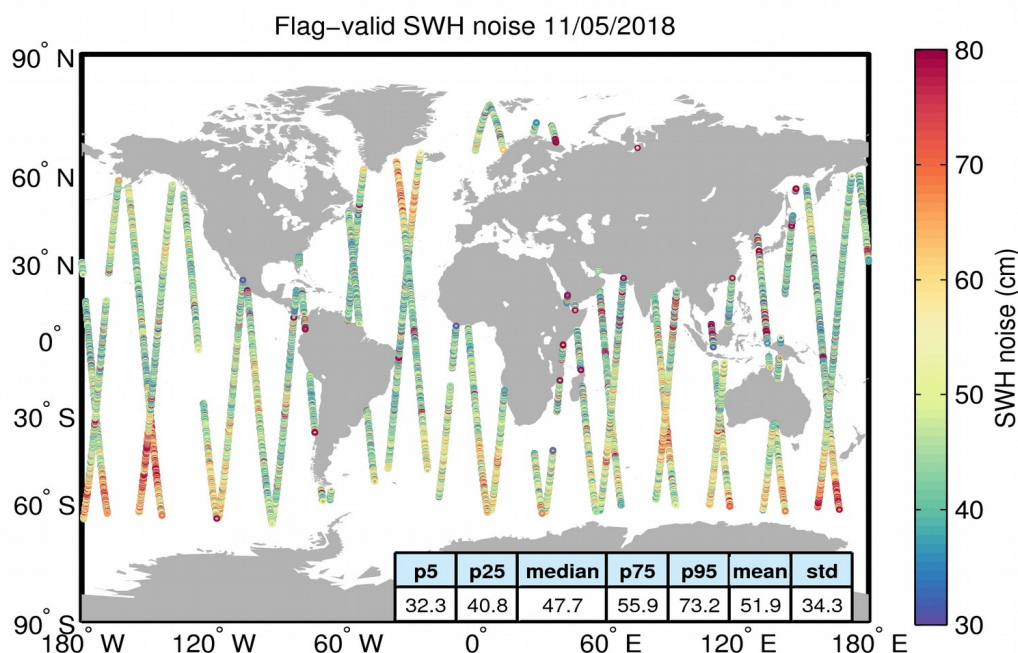
Figure 18. Geographical distribution of flag-valid 20-Hz SWH measurement noise over oceans and lakes for 11/05/2018. The statistical values shown in the figure refer to the SWH noise and are calculated over all measurements shown in the figure.
