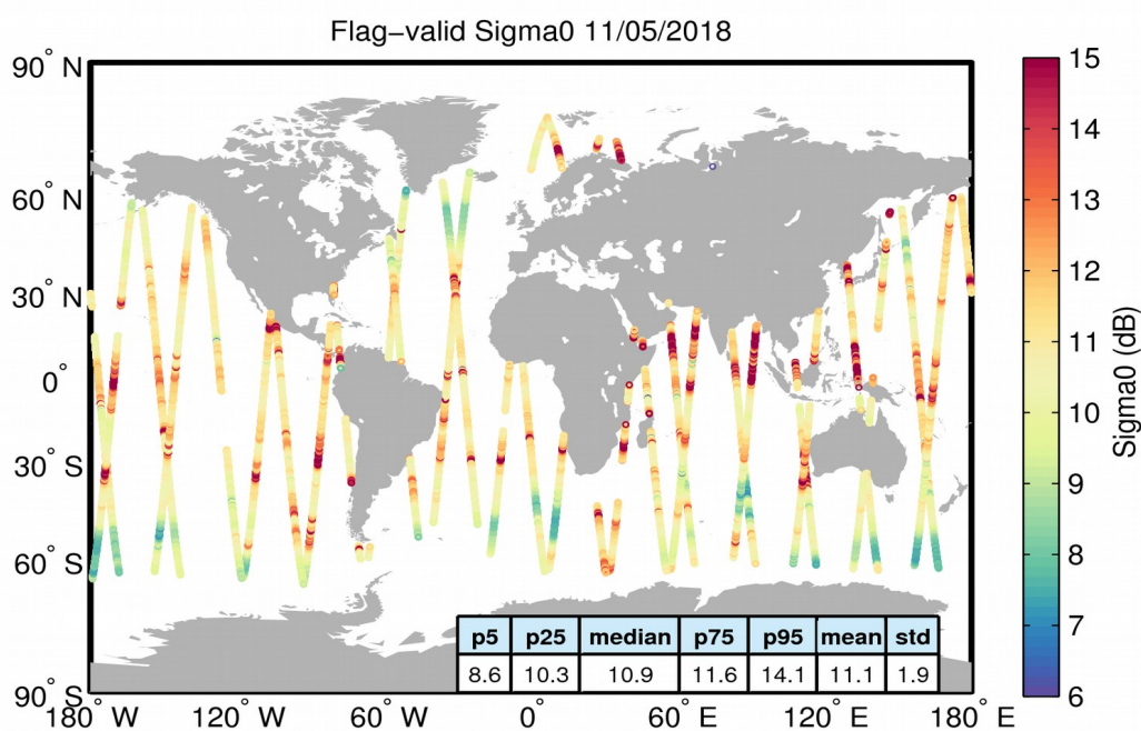
Figure 23. Geographical distribution of flag-valid sigma0 data over oceans and lakes for 11/05/2018. The statistical values shown in the table refer to the sigma0 in dB and are calculated over all measurements shown in the figure.
