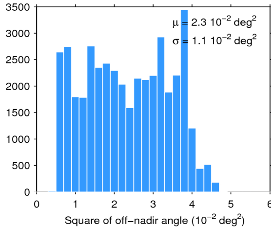
Figure 39. Histogram of flag-valid mispointing over oceans and lakes for 11/05/2018. The mean ( \mu ) and standard deviation ( \sigma ) are also shown. Note that values larger than 6 \cdot 10^{-2} \text{ deg}^2 are excluded from the histogram for the sake of readability but not from the computation of \mu and \sigma .
