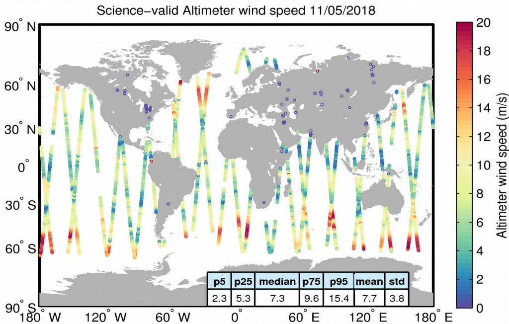
Figure 34. Geographical distribution of science-valid wind data over oceans and lakes for 11/05/2018. The statistical values shown in the table refer to the wind in m/s and are calculated over all measurements shown in the figure. Gray circles denote records that have been rejected based on the editing criteria described in Table 5.
