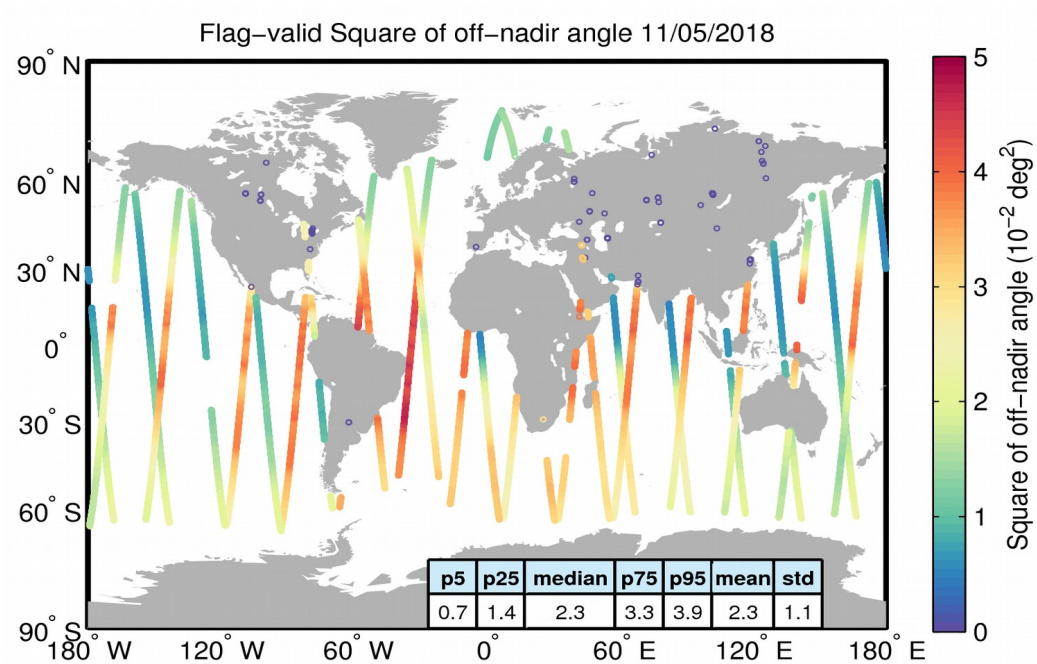
Figure 37. Geographical distribution of flag-valid mispointing data over oceans and lakes for 11/05/2018. The statistical values shown in the table refer to the mispointing in 10^{-2} \text{deg}^2 and are calculated over all measurements shown in the figure.
