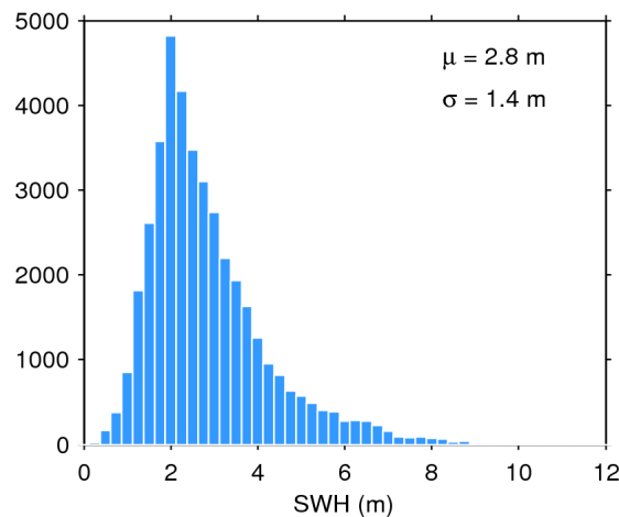
Figure 20. Histogram of science-valid SWH over oceans and lakes for 11/05/2018. The mean ( \mu ) and standard deviation ( \sigma ) are also shown. Note that values larger than 12 m are excluded from the histogram for the sake of readability but not from the computation of \mu and \sigma .
