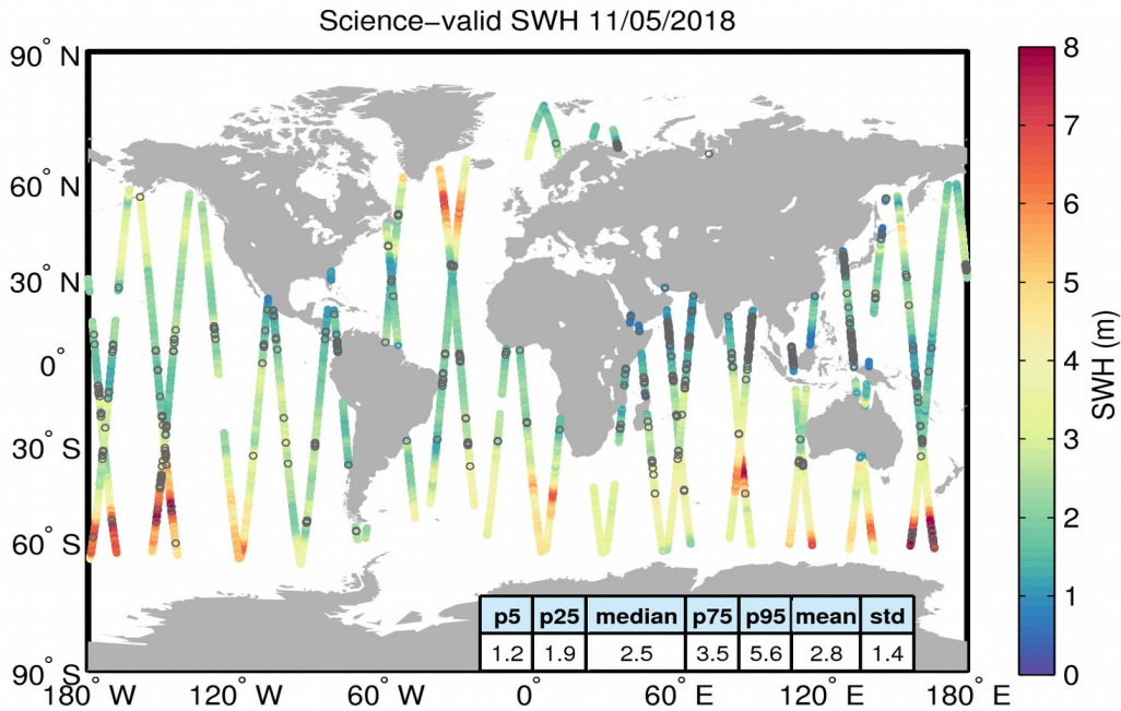
Figure 19. Geographical distribution of science-valid SWH data over oceans and lakes for 11/05/2018. The statistical values shown in the table refer to the SWH in m and are calculated over all measurements shown in the figure. Gray circles denote records that have been rejected based on the editing criteria described in Table 3.
