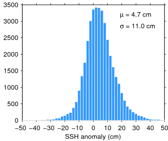
Figure 11. Histogram of science-valid SSH anomaly over oceans and lakes for 11/05/2018. The mean ( \mu ) and standard deviation ( \sigma ) are also shown. Note that values outside [-50 50] cm are excluded from the histogram for the sake of readability but not from the computation of \mu and \sigma .
