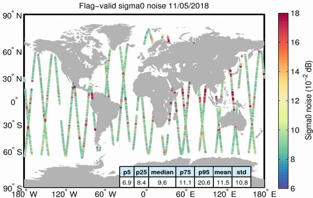
Figure 26. Geographical distribution of flag-valid 20-Hz sigma0 measurement noise over oceans and lakes for 11/05/2018. The statistical values shown in the table refer to the sigma0 noise and are calculated over all measurements shown in the figure.
