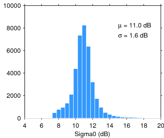
Figure 28. Histogram of science-valid sigma0 over oceans and lakes for 11/05/2018. The mean ( \mu ) and standard deviation ( \sigma ) are also shown. Note that values outside [4 20] dB are excluded from the histogram for the sake of readability but not from the computation of \mu and \sigma .
