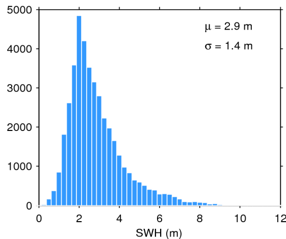
Figure 17. Histogram of flag-valid SWH over oceans and lakes for 11/05/2018. The mean ( \mu ) and standard deviation ( \sigma ) are also shown. Note that values larger than 12 m are excluded from the histogram for the sake of readability but not from the computation of \mu and \sigma .
