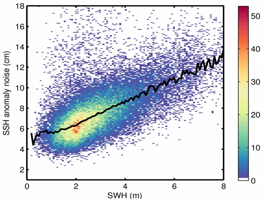
Figure 9. 2D histogram showing flag-valid SSH anomaly noise as a function of SWH for 11/05/2018. The black line denotes the median SSH anomaly noise as a function of SWH.
