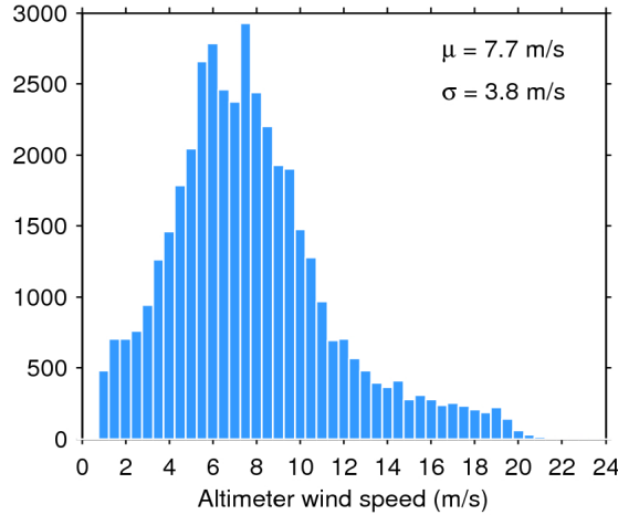
Figure 33. Histogram of flag-valid wind over oceans and lakes for 11/05/2018. The mean ( \mu ) and standard deviation ( \sigma ) are also shown. Note that values larger than 24 m/s are excluded from the histogram for the sake of readability but not from the computation of \mu and \sigma .
