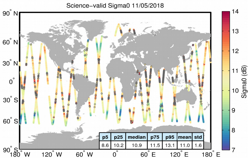
Figure 27. Geographical distribution of science-valid sigma0 data over oceans and lakes for 11/05/2018. The statistical values shown in the table refer to the sigma0 in dB and are calculated over all measurements shown in the figure. Gray circles denote records that have been rejected based on the editing criteria described in Table 4.
