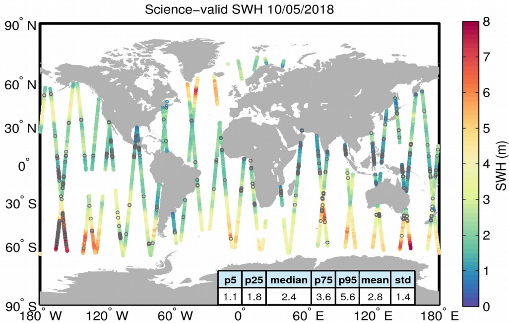
Figure 19. Geographical distribution of science-valid SWH data over oceans and lakes for 10/05/2018. The statistical values shown in the table refer to the SWH in m and are calculated over all measurements shown in the figure. Gray circles denote records that have been rejected based on the editing criteria described in Table 3.
