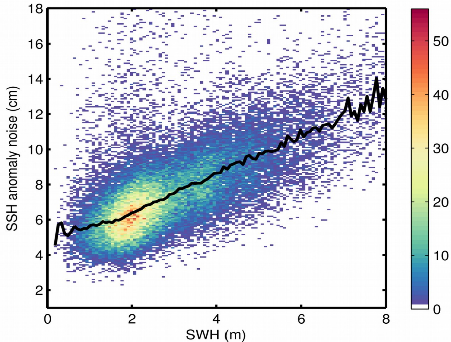
Figure 9. 2D histogram showing flag-valid SSH anomaly noise as a function of SWH for 10/05/2018. The black line denotes the median SSH anomaly noise as a function of SWH.
