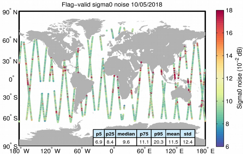
Figure 26. Geographical distribution of flag-valid 20-Hz sigma0 measurement noise over oceans and lakes for 10/05/2018. The statistical values shown in the table refer to the sigma0 noise and are calculated over all measurements shown in the figure.
