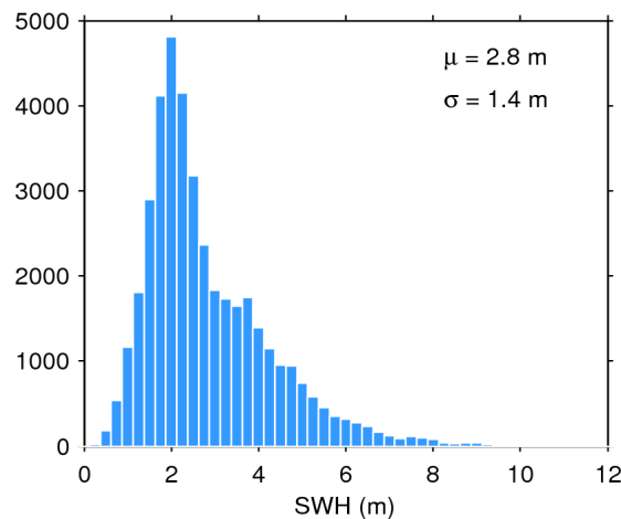
Figure 20. Histogram of science-valid SWH over oceans and lakes for 10/05/2018. The mean ( \mu ) and standard deviation ( \sigma ) are also shown. Note that values larger than 12 m are excluded from the histogram for the sake of readability but not from the computation of \mu and \sigma .
