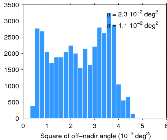
Figure 39. Histogram of flag-valid mispointing over oceans and lakes for 10/05/2018. The mean ( \mu ) and standard deviation ( \sigma ) are also shown. Note that values larger than 6 \cdot 10^{-2} \text{ deg}^2 are excluded from the histogram for the sake of readability but not from the computation of \mu and \sigma .
