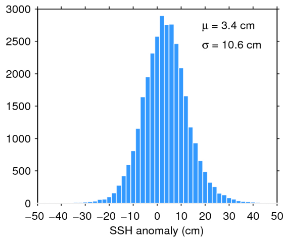
Figure 11. Histogram of science-valid SSH anomaly over oceans and lakes for 10/05/2018. The mean ( \mu ) and standard deviation ( \sigma ) are also shown. Note that values outside [-50 50] cm are excluded from the histogram for the sake of readability but not from the computation of \mu and \sigma .
