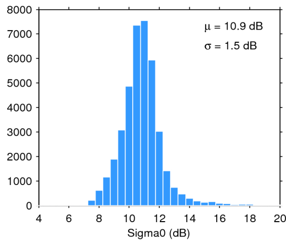
Figure 28. Histogram of science-valid sigma0 over oceans and lakes for 10/05/2018. The mean ( \mu ) and standard deviation ( \sigma ) are also shown. Note that values outside [4 20] dB are excluded from the histogram for the sake of readability but not from the computation of \mu and \sigma .
