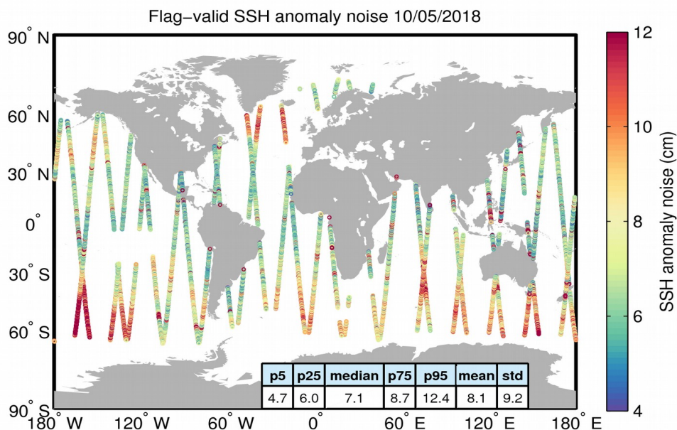
Figure 8. Geographical distribution of flag-valid 20-Hz SSH anomaly measurement noise over oceans and lakes for 10/05/2018. The statistical values shown in the table refer to the SSH anomaly noise and are calculated over all measurements shown in the figure.
