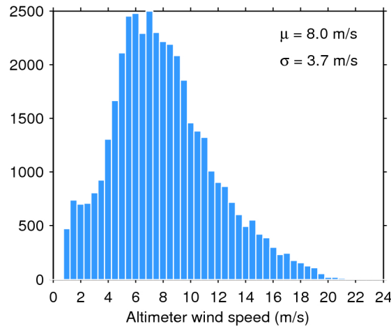
Figure 33. Histogram of flag-valid wind over oceans and lakes for 10/05/2018. The mean ( \mu ) and standard deviation ( \sigma ) are also shown. Note that values larger than 24 m/s are excluded from the histogram for the sake of readability but not from the computation of \mu and \sigma .
