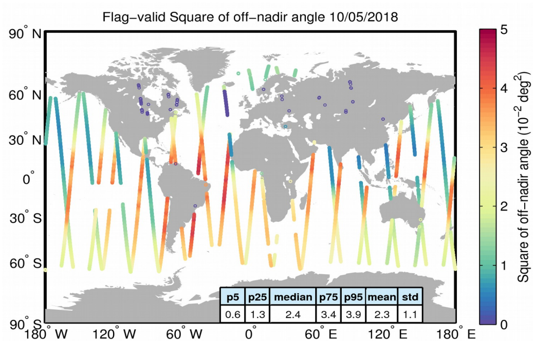
Figure 37. Geographical distribution of flag-valid mispointing data over oceans and lakes for 10/05/2018. The statistical values shown in the table refer to the mispointing in 10^{-2} \text{ deg}^2 and are calculated over all measurements shown in the figure.
