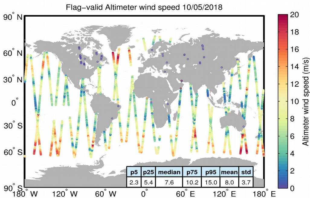
Figure 31. Geographical distribution of flag-valid wind data over oceans and lakes for 10/05/2018. The statistical values shown in the table refer to the wind in m/s and are calculated over all measurements shown in the figure.
