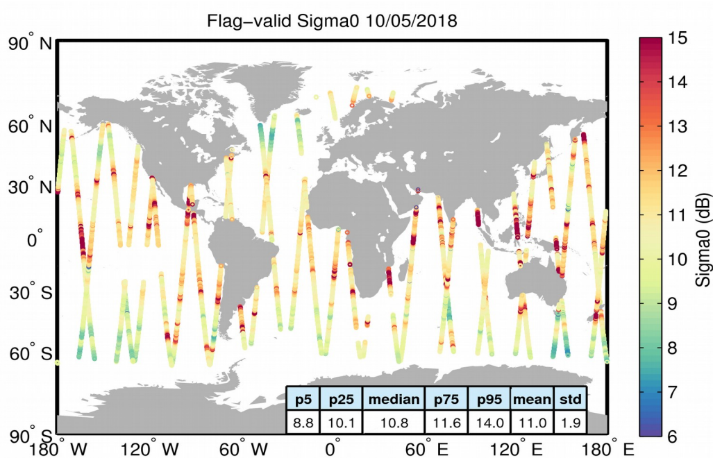
Figure 23. Geographical distribution of flag-valid sigma0 data over oceans and lakes for 10/05/2018. The statistical values shown in the table refer to the sigma0 in dB and are calculated over all measurements shown in the figure.
