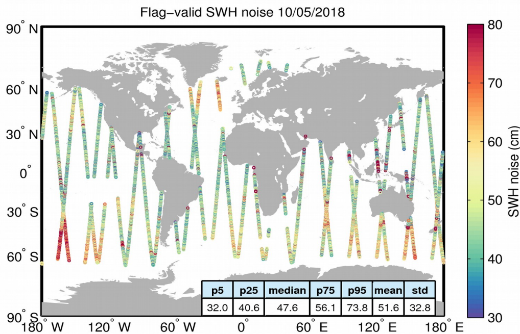
Figure 18. Geographical distribution of flag-valid 20-Hz SWH measurement noise over oceans and lakes for 10/05/2018. The statistical values shown in the table refer to the SWH noise and are calculated over all measurements shown in the figure.
