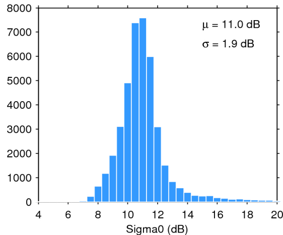
Figure 25. Histogram of flag-valid sigma0 over oceans and lakes for 10/05/2018. The mean ( \mu ) and standard deviation ( \sigma ) are also shown. Note that values outside [4 20] dB are excluded from the histogram for the sake of readability but not from the computation of \mu and \sigma .
