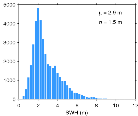
Figure 17. Histogram of flag-valid SWH over oceans and lakes for 10/05/2018. The mean ( \mu ) and standard deviation ( \sigma ) are also shown. Note that values larger than 12 m are excluded from the histogram for the sake of readability but not from the computation of \mu and \sigma .
