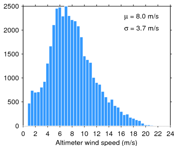
Figure 35. Histogram of science-valid wind over oceans and lakes for 10/05/2018. The mean ( \mu ) and standard deviation ( \sigma ) are also shown. Note that values larger than 24 m/s are excluded from the histogram for the sake of readability but not from the computation of \mu and \sigma .
