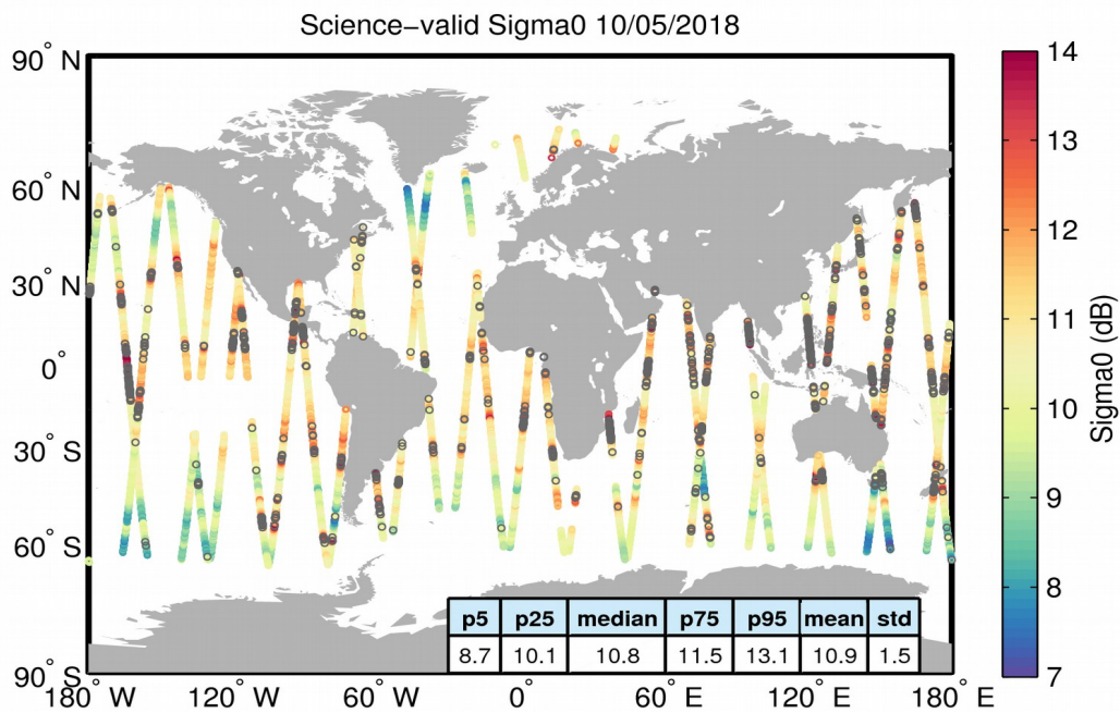
Figure 27. Geographical distribution of science-valid sigma0 data over oceans and lakes for 10/05/2018. The statistical values shown in the table refer to the sigma0 in dB and are calculated over all measurements shown in the figure. Gray circles denote records that have been rejected based on the editing criteria described in Table 4.
