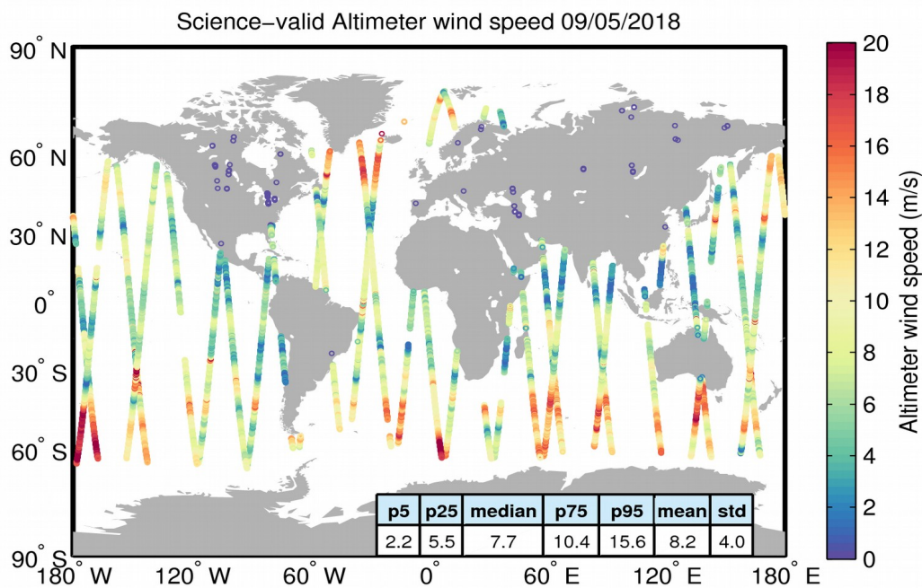
Figure 34. Geographical distribution of science-valid wind data over oceans and lakes for 09/05/2018. The statistical values shown in the table refer to the wind in m/s and are calculated over all measurements shown in the figure. Gray circles denote records that have been rejected based on the editing criteria described in Table 5.
