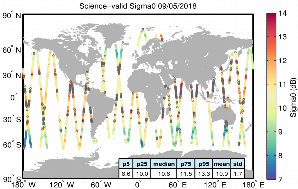
Figure 27. Geographical distribution of science-valid sigma0 data over oceans and lakes for 09/05/2018. The statistical values shown in the table refer to the sigma0 in dB and are calculated over all measurements shown in the figure. Gray circles denote records that have been rejected based on the editing criteria described in Table 4.
