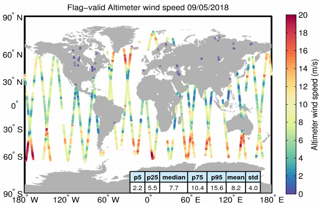
Figure 31. Geographical distribution of flag-valid wind data over oceans and lakes for 09/05/2018. The statistical values shown in the table refer to the wind in m/s and are calculated over all measurements shown in the figure.
