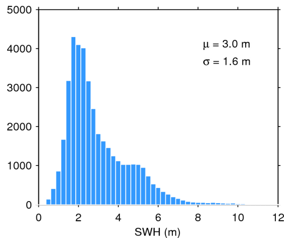
Figure 20. Histogram of science-valid SWH over oceans and lakes for 09/05/2018. The mean ( \mu ) and standard deviation ( \sigma ) are also shown. Note that values larger than 12 m are excluded from the histogram for the sake of readability but not from the computation of \mu and \sigma .
