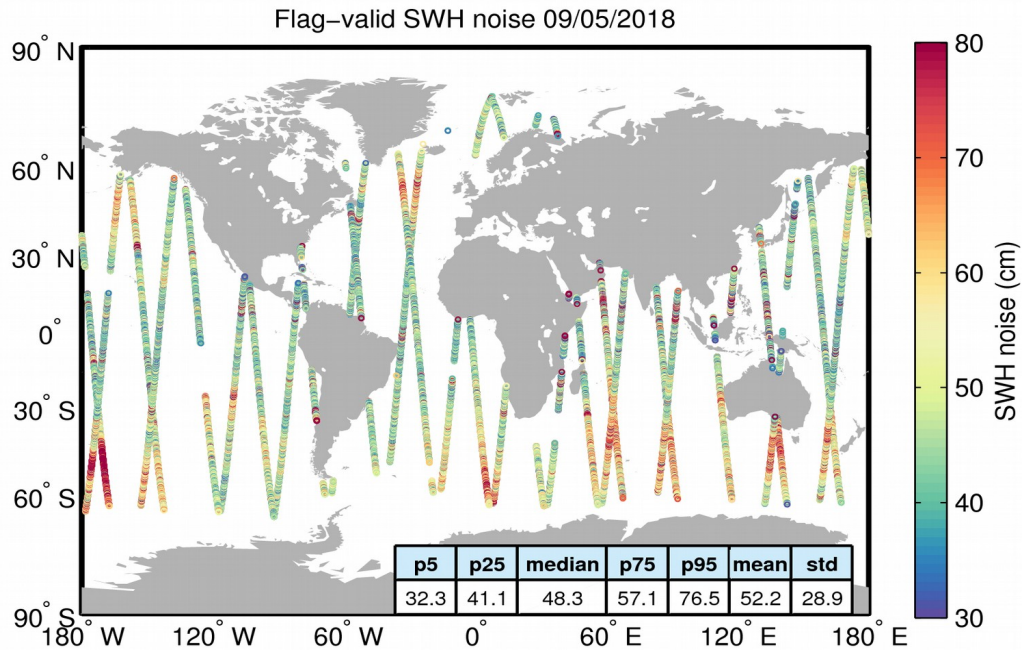
Figure 18. Geographical distribution of flag-valid 20-Hz SWH measurement noise over oceans and lakes for 09/05/2018. The statistical values shown in the figure refer to the SWH noise and are calculated over all measurements shown in the figure.
