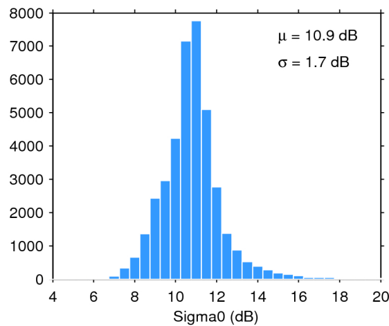
Figure 28. Histogram of science-valid sigma0 over oceans and lakes for 09/05/2018. The mean ( \mu ) and standard deviation ( \sigma ) are also shown. Note that values outside [4 20] dB are excluded from the histogram for the sake of readability but not from the computation of \mu and \sigma .
