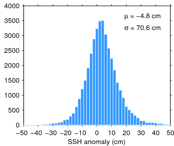
Figure 7. Histogram of flag-valid SSH anomaly over oceans and lakes for 09/05/2018. The mean ( \mu ) and standard deviation ( \sigma ) are also shown. Note that values outside [-50\ 50] cm are excluded from the histogram for the sake of readability but not from the computation of \mu and \sigma .
