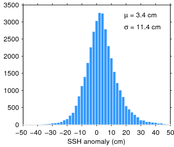
Figure 11. Histogram of science-valid SSH anomaly over oceans and lakes for 09/05/2018. The mean ( \mu ) and standard deviation ( \sigma ) are also shown. Note that values outside [-50 50] cm are excluded from the histogram for the sake of readability but not from the computation of \mu and \sigma .
