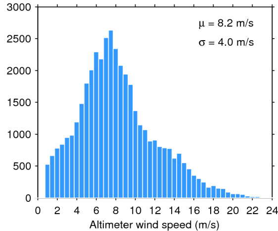
Figure 33. Histogram of flag-valid wind over oceans and lakes for 09/05/2018. The mean ( \mu ) and standard deviation ( \sigma ) are also shown. Note that values larger than 24 m/s are excluded from the histogram for the sake of readability but not from the computation of \mu and \sigma .
