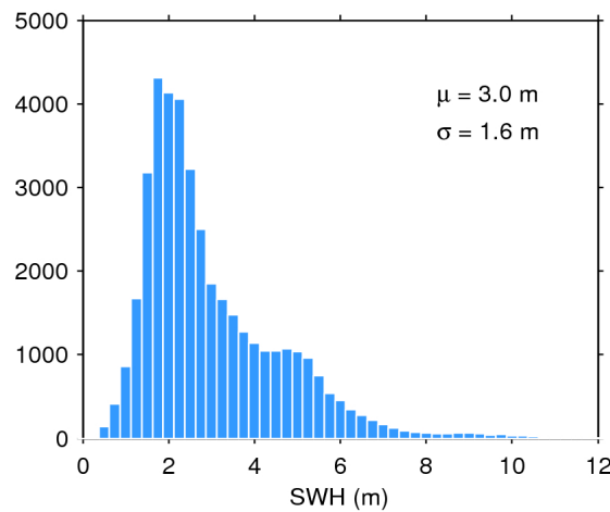
Figure 17. Histogram of flag-valid SWH over oceans and lakes for 09/05/2018. The mean ( \mu ) and standard deviation ( \sigma ) are also shown. Note that values larger than 12 m are excluded from the histogram for the sake of readability but not from the computation of \mu and \sigma .
