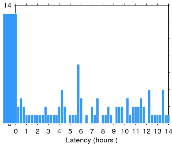
Figure 2. Histogram of the data latency for 09/05/2018. The y-axis denotes the number of files that are made available with a delay of x-hours with respect to the mean time of the records stored in the file.
