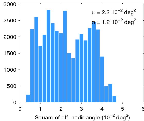
Figure 39. Histogram of flag-valid mispointing over oceans and lakes for 09/05/2018. The mean ( \mu ) and standard deviation ( \sigma ) are also shown. Note that values larger than 6 \cdot 10^{-2} \text{ deg}^2 are excluded from the histogram for the sake of readability but not from the computation of \mu and \sigma .
