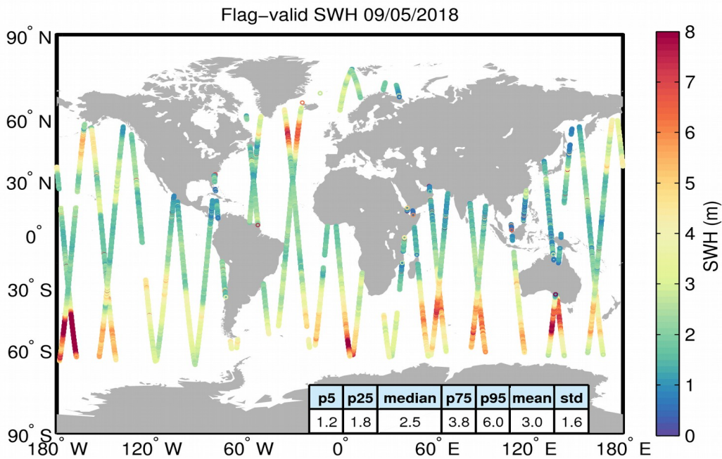
Figure 15. Geographical distribution of flag-valid SWH data over oceans and lakes for 09/05/2018. The statistical values shown in the table refer to the SWH in m and are calculated over all measurements shown in the figure.
