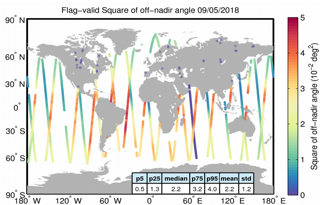
Figure 37. Geographical distribution of flag-valid mispointing data over oceans and lakes for 09/05/2018. The statistical values shown in the table refer to the mispointing in 10^{-2} deg 2 and are calculated over all measurements shown in the figure.
