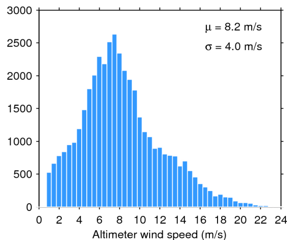
Figure 35. Histogram of science-valid wind over oceans and lakes for 09/05/2018. The mean ( \mu ) and standard deviation ( \sigma ) are also shown. Note that values larger than 24 m/s are excluded from the histogram for the sake of readability but not from the computation of \mu and \sigma .
