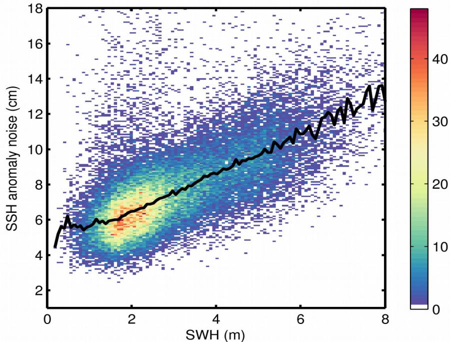
Figure 9. 2D histogram showing flag-valid SSH anomaly noise as a function of SWH for 09/05/2018. The black line denotes the median SSH anomaly noise as a function of SWH.
