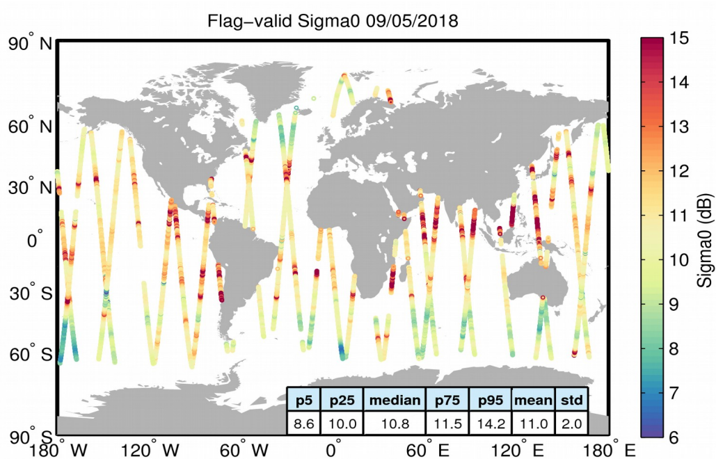
Figure 23. Geographical distribution of flag-valid sigma0 data over oceans and lakes for 09/05/2018. The statistical values shown in the table refer to the sigma0 in dB and are calculated over all measurements shown in the figure.
