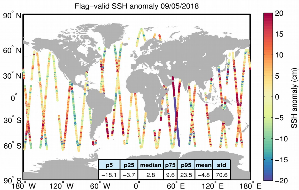
Figure 5. Geographical distribution of flag-valid 1-Hz SSH anomaly data over oceans and lakes for 09/05/2018. The statistical values shown in the table refer to the SSH anomaly in cm and are calculated over all measurements shown in the figure.
