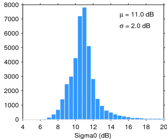
Figure 25. Histogram of flag-valid sigma0 over oceans and lakes for 09/05/2018. The mean ( \mu ) and standard deviation ( \sigma ) are also shown. Note that values outside [4 20] dB are excluded from the histogram for the sake of readability but not from the computation of \mu and \sigma .
