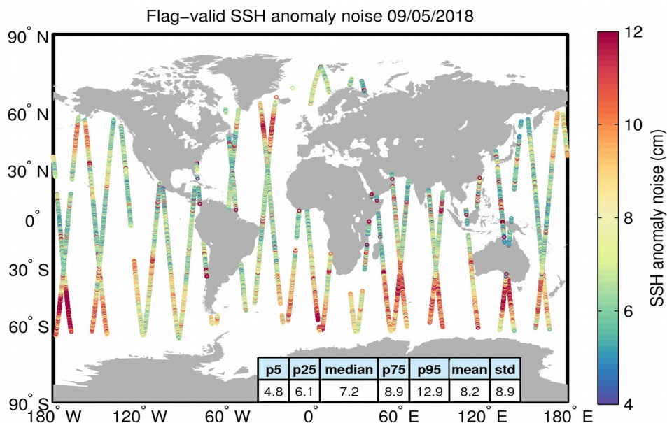
Figure 8. Geographical distribution of flag-valid 20-Hz SSH anomaly measurement noise over oceans and lakes for 09/05/2018. The statistical values shown in the table refer to the SSH anomaly noise and are calculated over all measurements shown in the figure.
