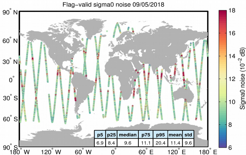
Figure 26. Geographical distribution of flag-valid 20-Hz sigma0 measurement noise over oceans and lakes for 09/05/2018. The statistical values shown in the table refer to the sigma0 noise and are calculated over all measurements shown in the figure.
