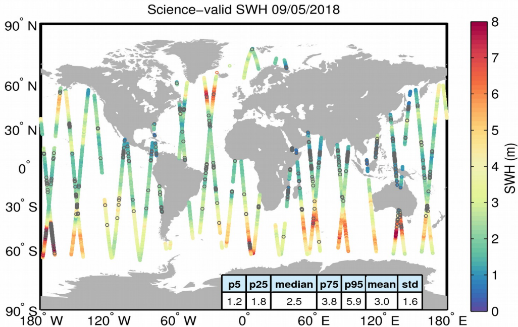
Figure 19. Geographical distribution of science-valid SWH data over oceans and lakes for 09/05/2018. The statistical values shown in the table refer to the SWH in m and are calculated over all measurements shown in the figure. Gray circles denote records that have been rejected based on the editing criteria described in Table 3.
