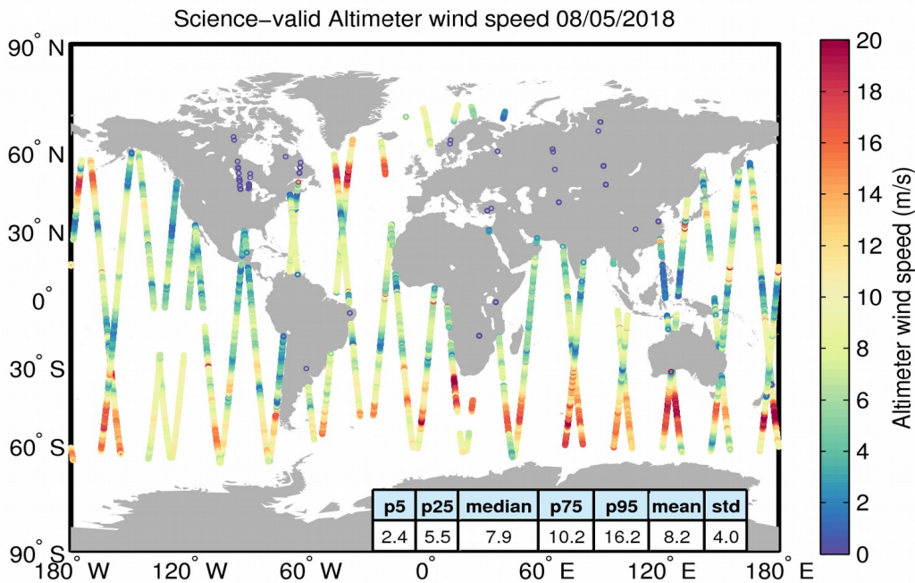
Figure 34. Geographical distribution of science-valid wind data over oceans and lakes for 08/05/2018. The statistical values shown in the table refer to the wind in m/s and are calculated over all measurements shown in the figure. Gray circles denote records that have been rejected based on the editing criteria described in Table 5.
