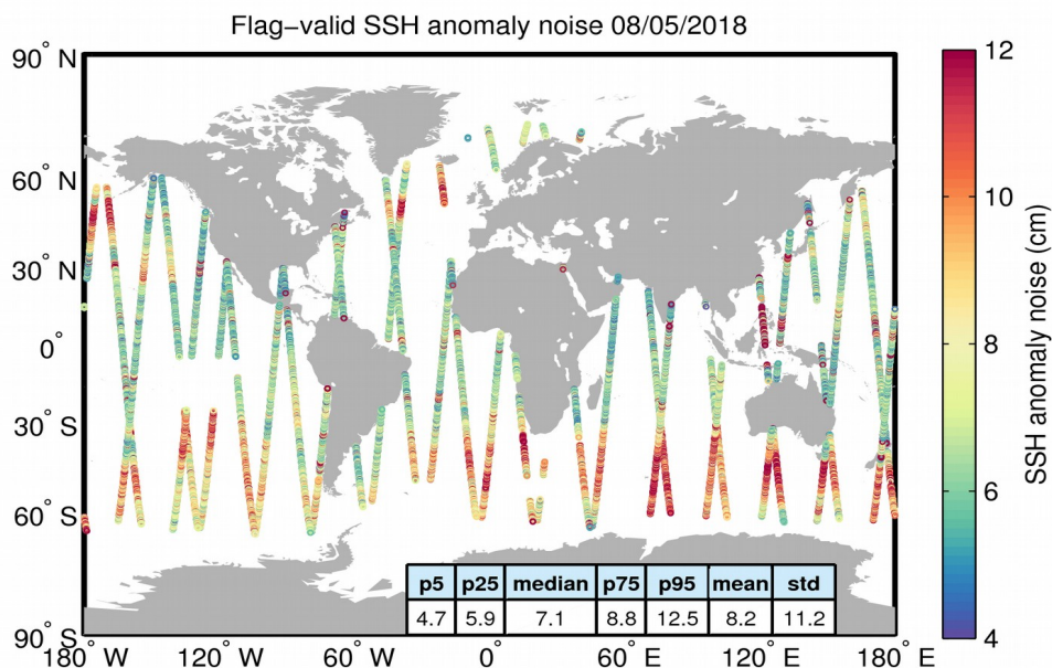
Figure 8. Geographical distribution of flag-valid 20-Hz SSH anomaly measurement noise over oceans and lakes for 08/05/2018. The statistical values shown in the table refer to the SSH anomaly noise and are calculated over all measurements shown in the figure.
