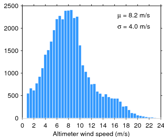
Figure 35. Histogram of science-valid wind over oceans and lakes for 08/05/2018. The mean ( \mu ) and standard deviation ( \sigma ) are also shown. Note that values larger than 24 m/s are excluded from the histogram for the sake of readability but not from the computation of \mu and \sigma .
