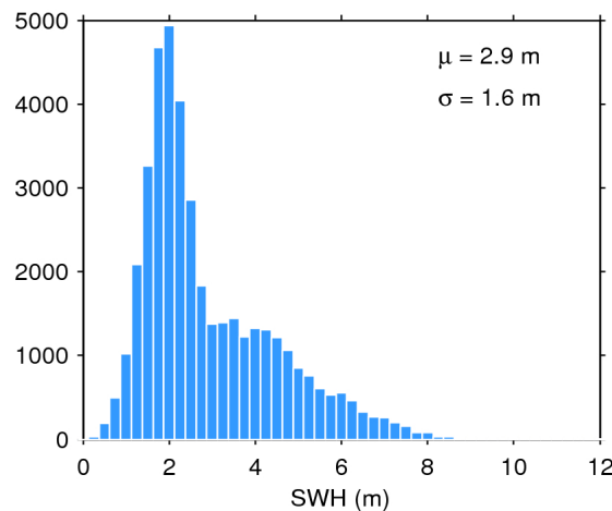
Figure 17. Histogram of flag-valid SWH over oceans and lakes for 08/05/2018. The mean ( \mu ) and standard deviation ( \sigma ) are also shown. Note that values larger than 12 m are excluded from the histogram for the sake of readability but not from the computation of \mu and \sigma .
