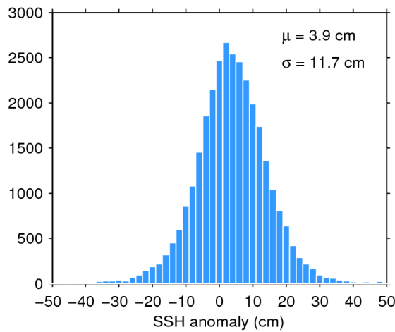
Figure 11. Histogram of science-valid SSH anomaly over oceans and lakes for 08/05/2018. The mean ( \mu ) and standard deviation ( \sigma ) are also shown. Note that values outside [-50 50] cm are excluded from the histogram for the sake of readability but not from the computation of \mu and \sigma .
