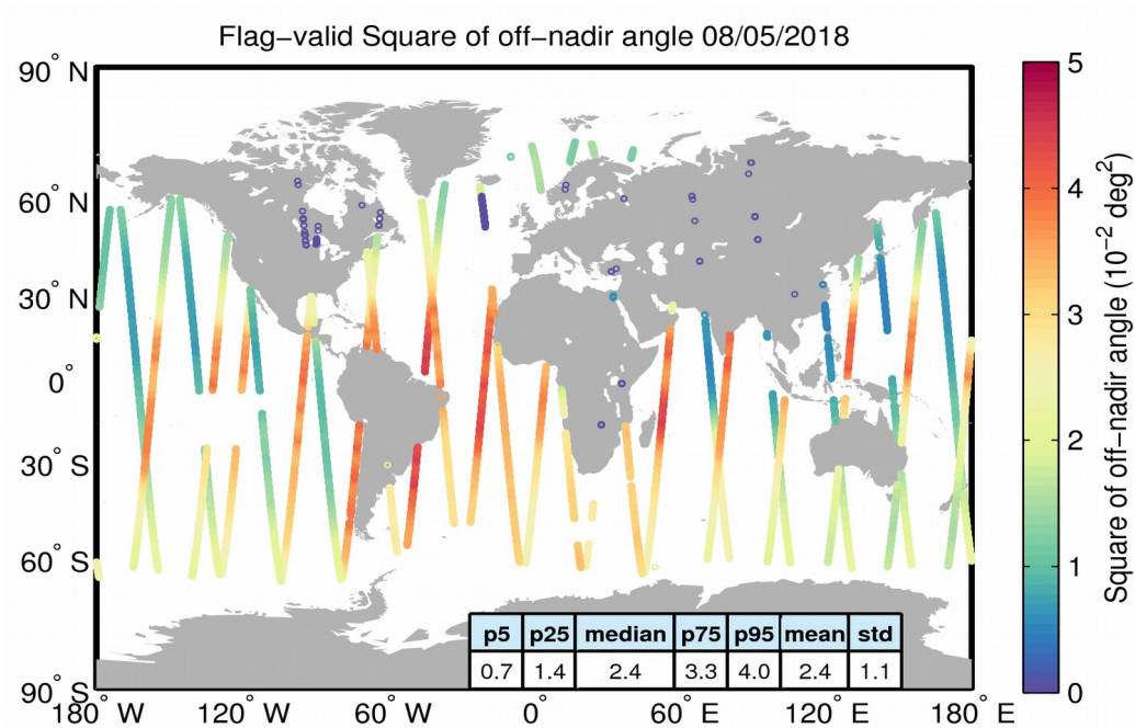
Figure 37. Geographical distribution of flag-valid mispointing data over oceans and lakes for 08/05/2018. The statistical values shown in the table refer to the mispointing in 10^{-2} \text{ deg}^2 and are calculated over all measurements shown in the figure.
