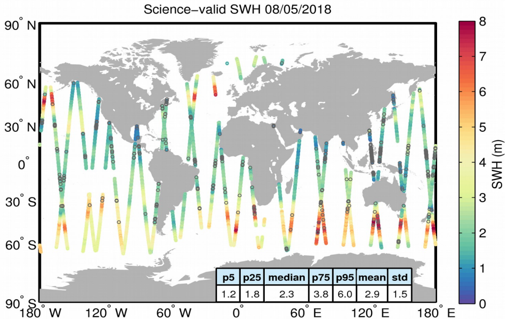
Figure 19. Geographical distribution of science-valid SWH data over oceans and lakes for 08/05/2018. The statistical values shown in the table refer to the SWH in m and are calculated over all measurements shown in the figure. Gray circles denote records that have been rejected based on the editing criteria described in Table 3.
