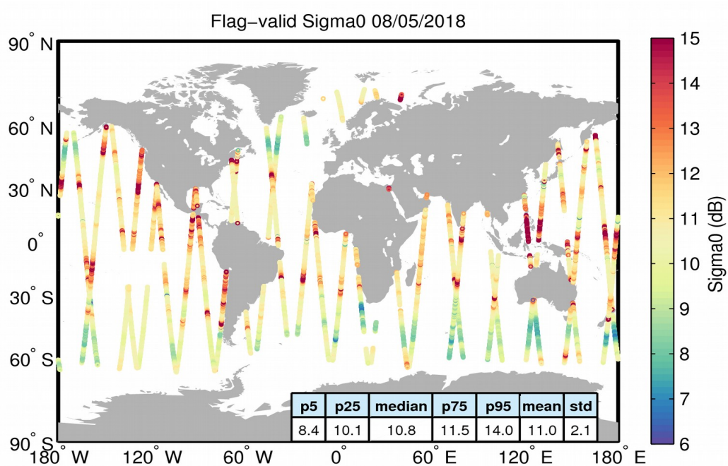
Figure 23. Geographical distribution of flag-valid sigma0 data over oceans and lakes for 08/05/2018. The statistical values shown in the table refer to the sigma0 in dB and are calculated over all measurements shown in the figure.
