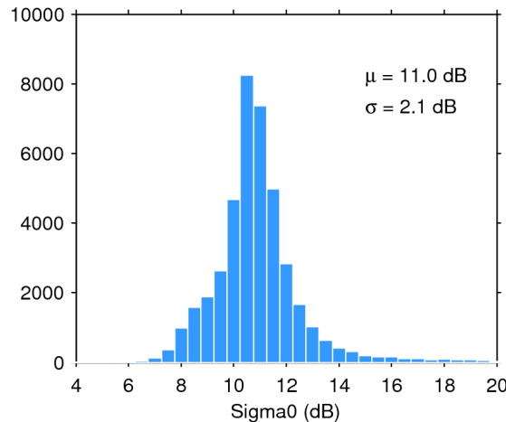
Figure 25. Histogram of flag-valid sigma0 over oceans and lakes for 08/05/2018. The mean ( \mu ) and standard deviation ( \sigma ) are also shown. Note that values outside [4 20] dB are excluded from the histogram for the sake of readability but not from the computation of \mu and \sigma .
