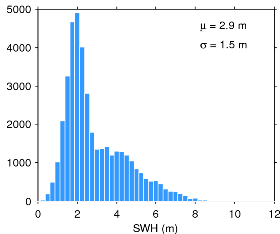
Figure 20. Histogram of science-valid SWH over oceans and lakes for 08/05/2018. The mean ( \mu ) and standard deviation ( \sigma ) are also shown. Note that values larger than 12 m are excluded from the histogram for the sake of readability but not from the computation of \mu and \sigma .
