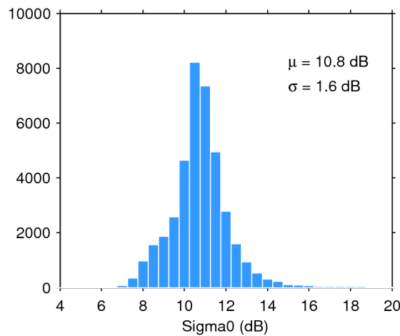
Figure 28. Histogram of science-valid sigma0 over oceans and lakes for 08/05/2018. The mean ( \mu ) and standard deviation ( \sigma ) are also shown. Note that values outside [4 20] dB are excluded from the histogram for the sake of readability but not from the computation of \mu and \sigma .
