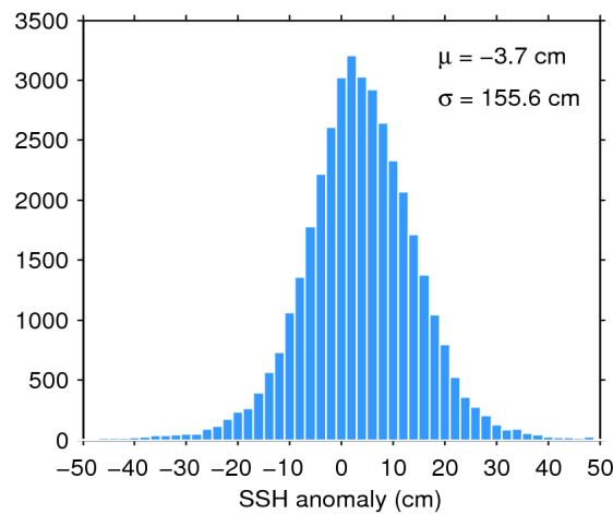
Figure 7. Histogram of flag-valid SSH anomaly over oceans and lakes for 08/05/2018. The mean ( \mu ) and standard deviation ( \sigma ) are also shown. Note that values outside [-50 50] cm are excluded from the histogram for the sake of readability but not from the computation of \mu and \sigma .
