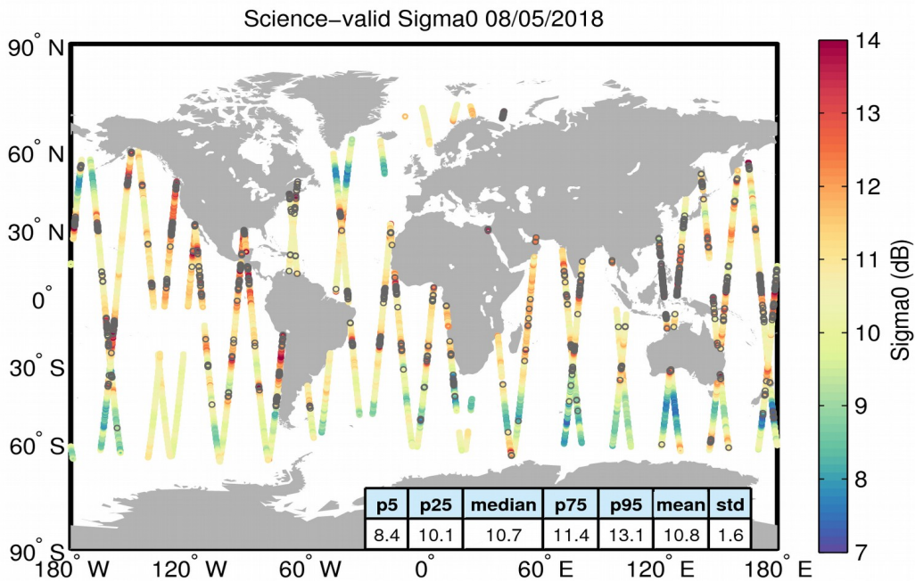
Figure 27. Geographical distribution of science-valid sigma0 data over oceans and lakes for 08/05/2018. The statistical values shown in the table refer to the sigma0 in dB and are calculated over all measurements shown in the figure. Gray circles denote records that have been rejected based on the editing criteria described in Table 4.
