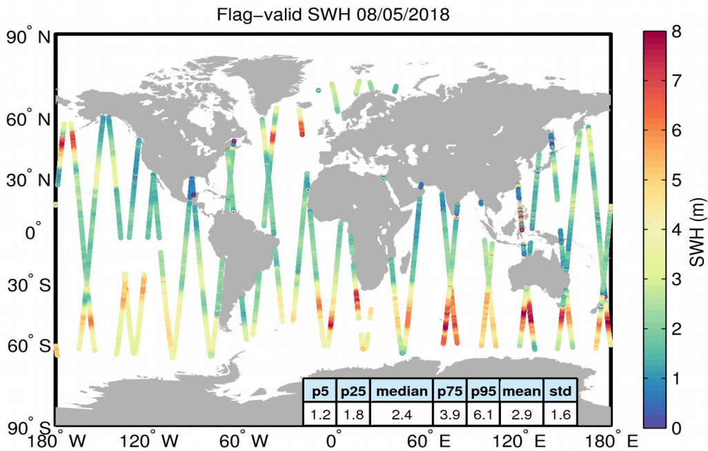
Figure 15. Geographical distribution of flag-valid SWH data over oceans and lakes for 08/05/2018. The statistical values shown in the table refer to the SWH in m and are calculated over all measurements shown in the figure.
