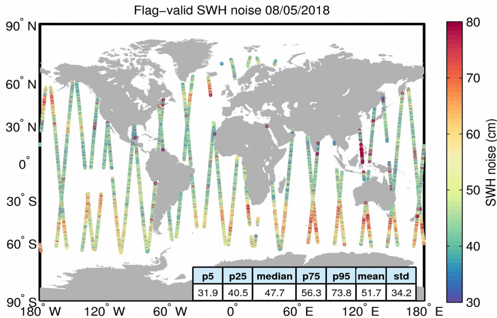
Figure 18. Geographical distribution of flag-valid 20-Hz SWH measurement noise over oceans and lakes for 08/05/2018. The statistical values shown in the table refer to the SWH noise and are calculated over all measurements shown in the figure.
