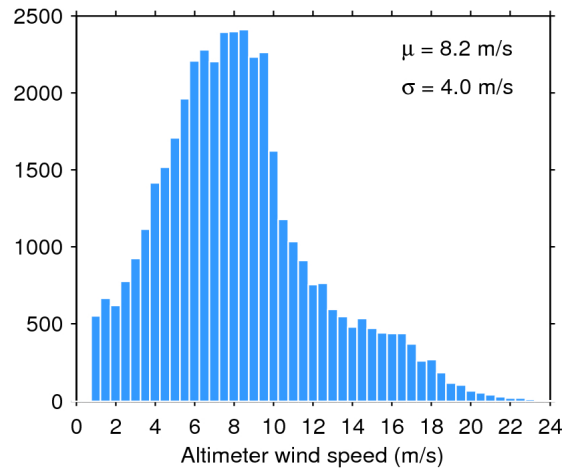
Figure 33. Histogram of flag-valid wind over oceans and lakes for 08/05/2018. The mean ( \mu ) and standard deviation ( \sigma ) are also shown. Note that values larger than 24 m/s are excluded from the histogram for the sake of readability but not from the computation of \mu and \sigma .
