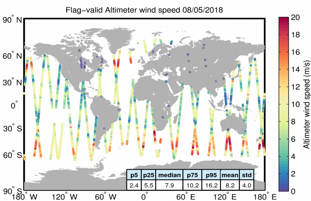
Figure 31. Geographical distribution of flag-valid wind data over oceans and lakes for 08/05/2018. The statistical values shown in the table refer to the wind in m/s and are calculated over all measurements shown in the figure.
