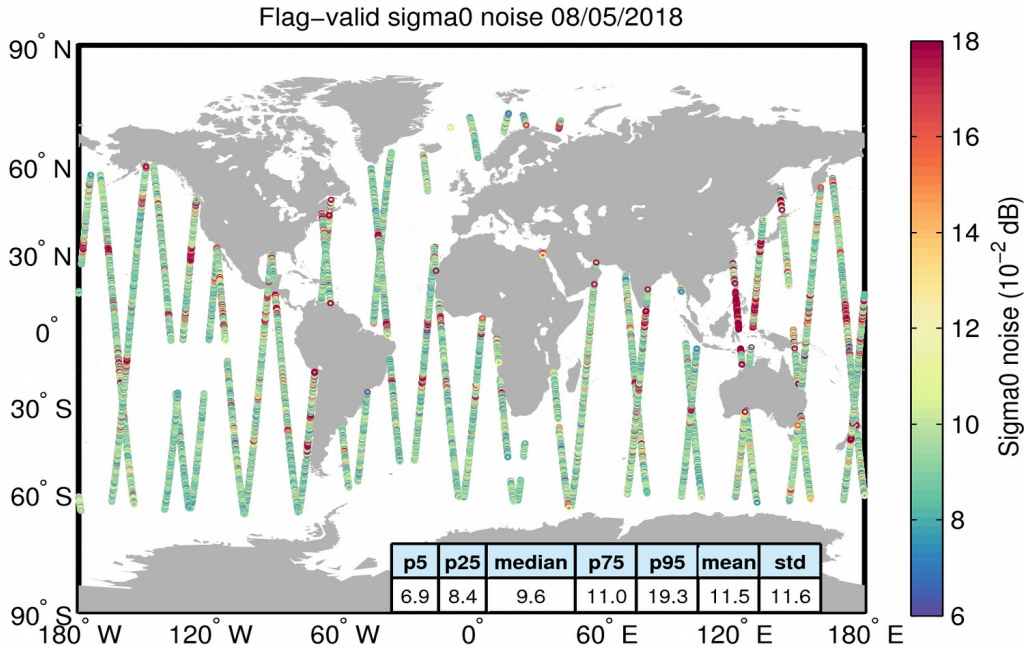
Figure 26. Geographical distribution of flag-valid 20-Hz sigma0 measurement noise over oceans and lakes for 08/05/2018. The statistical values shown in the table refer to the sigma0 noise and are calculated over all measurements shown in the figure.
