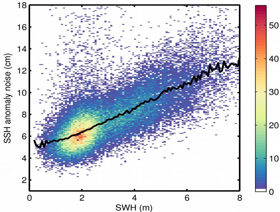
Figure 9. 2D histogram showing flag-valid SSH anomaly noise as a function of SWH for 08/05/2018. The black line denotes the median SSH anomaly noise as a function of SWH.
