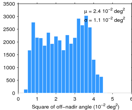
Figure 39. Histogram of flag-valid mispointing over oceans and lakes for 08/05/2018. The mean ( \mu ) and standard deviation ( \sigma ) are also shown. Note that values larger than 6 \cdot 10^{-2} \text{ deg}^2 are excluded from the histogram for the sake of readability but not from the computation of \mu and \sigma .
