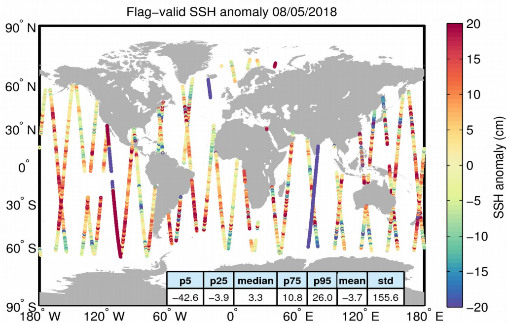
Figure 5. Geographical distribution of flag-valid 1-Hz SSH anomaly data over oceans and lakes for 08/05/2018. The statistical values shown in the table refer to the SSH anomaly in cm and are calculated over all measurements shown in the figure.
