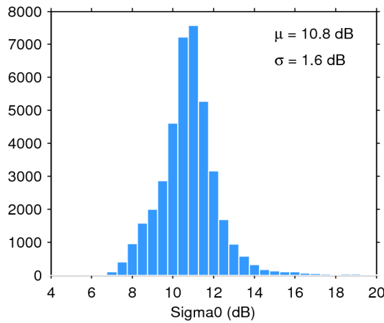
Figure 28. Histogram of science-valid sigma0 over oceans and lakes for 07/05/2018. The mean ( \mu ) and standard deviation ( \sigma ) are also shown. Note that values outside [4 20] dB are excluded from the histogram for the sake of readability but not from the computation of \mu and \sigma .
