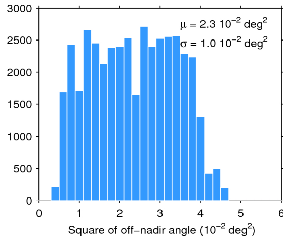
Figure 39. Histogram of flag-valid mispointing over oceans and lakes for 07/05/2018. The mean ( \mu ) and standard deviation ( \sigma ) are also shown. Note that values larger than 6 \cdot 10^{-2} \text{ deg}^2 are excluded from the histogram for the sake of readability but not from the computation of \mu and \sigma .
