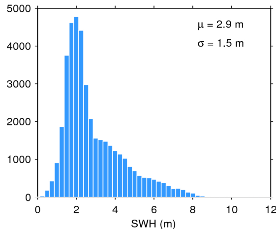
Figure 20. Histogram of science-valid SWH over oceans and lakes for 07/05/2018. The mean ( \mu ) and standard deviation ( \sigma ) are also shown. Note that values larger than 12 m are excluded from the histogram for the sake of readability but not from the computation of \mu and \sigma .
