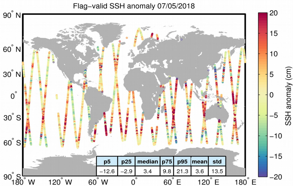
Figure 5. Geographical distribution of flag-valid 1-Hz SSH anomaly data over oceans and lakes for 07/05/2018. The statistical values shown in the table refer to the SSH anomaly in cm and are calculated over all measurements shown in the figure.
