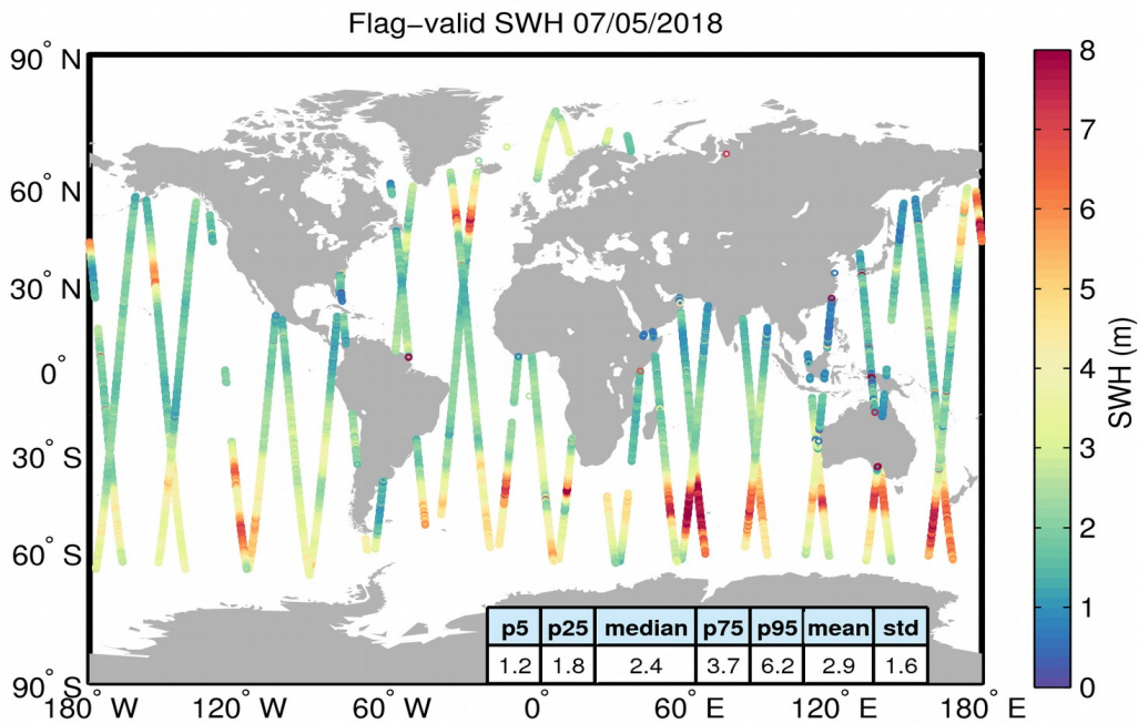
Figure 15. Geographical distribution of flag-valid SWH data over oceans and lakes for 07/05/2018. The statistical values shown in the table refer to the SWH in m and are calculated over all measurements shown in the figure.
