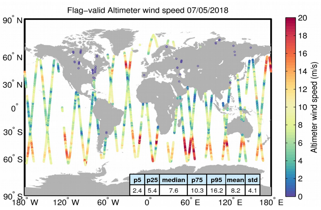
Figure 31. Geographical distribution of flag-valid wind data over oceans and lakes for 07/05/2018. The statistical values shown in the table refer to the wind in m/s and are calculated over all measurements shown in the figure.
