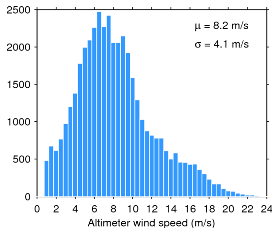
Figure 35. Histogram of science-valid wind over oceans and lakes for 07/05/2018. The mean ( \mu ) and standard deviation ( \sigma ) are also shown. Note that values larger than 24 m/s are excluded from the histogram for the sake of readability but not from the computation of \mu and \sigma .
