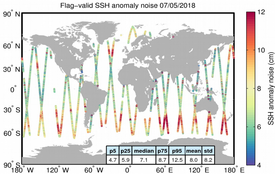
Figure 8. Geographical distribution of flag-valid 20-Hz SSH anomaly measurement noise over oceans and lakes for 07/05/2018. The statistical values shown in the table refer to the SSH anomaly noise and are calculated over all measurements shown in the figure.
