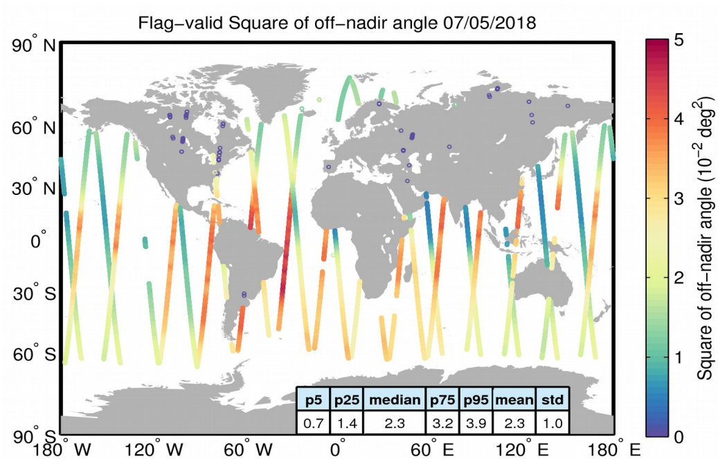
Figure 37. Geographical distribution of flag-valid mispointing data over oceans and lakes for 07/05/2018. The statistical values shown in the table refer to the mispointing in 10^{-2} deg 2 and are calculated over all measurements shown in the figure.
