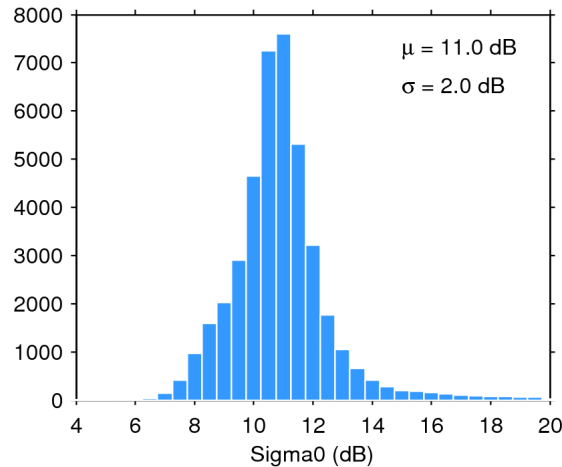
Figure 25. Histogram of flag-valid sigma0 over oceans and lakes for 07/05/2018. The mean ( \mu ) and standard deviation ( \sigma ) are also shown. Note that values outside [4 20] dB are excluded from the histogram for the sake of readability but not from the computation of \mu and \sigma .
