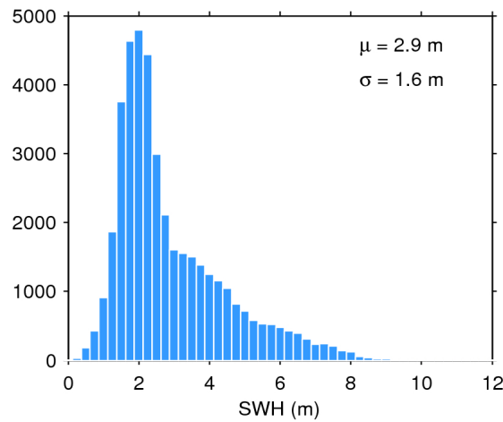
Figure 17. Histogram of flag-valid SWH over oceans and lakes for 07/05/2018. The mean ( \mu ) and standard deviation ( \sigma ) are also shown. Note that values larger than 12 m are excluded from the histogram for the sake of readability but not from the computation of \mu and \sigma .
