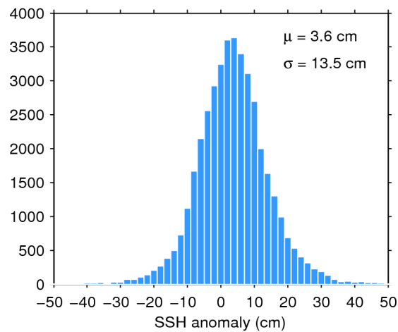
Figure 7. Histogram of flag-valid SSH anomaly over oceans and lakes for 07/05/2018. The mean ( \mu ) and standard deviation ( \sigma ) are also shown. Note that values outside [-50\ 50] cm are excluded from the histogram for the sake of readability but not from the computation of \mu and \sigma .
