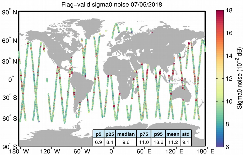
Figure 26. Geographical distribution of flag-valid 20-Hz sigma0 measurement noise over oceans and lakes for 07/05/2018. The statistical values shown in the table refer to the sigma0 noise and are calculated over all measurements shown in the figure.
