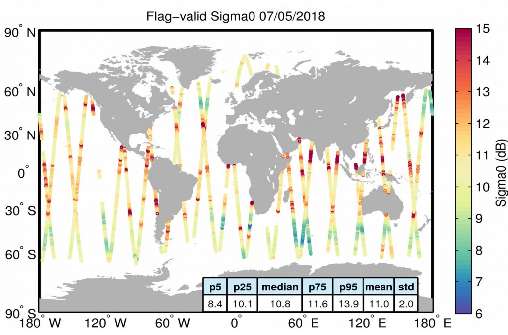
Figure 23. Geographical distribution of flag-valid sigma0 data over oceans and lakes for 07/05/2018. The statistical values shown in the table refer to the sigma0 in dB and are calculated over all measurements shown in the figure.
