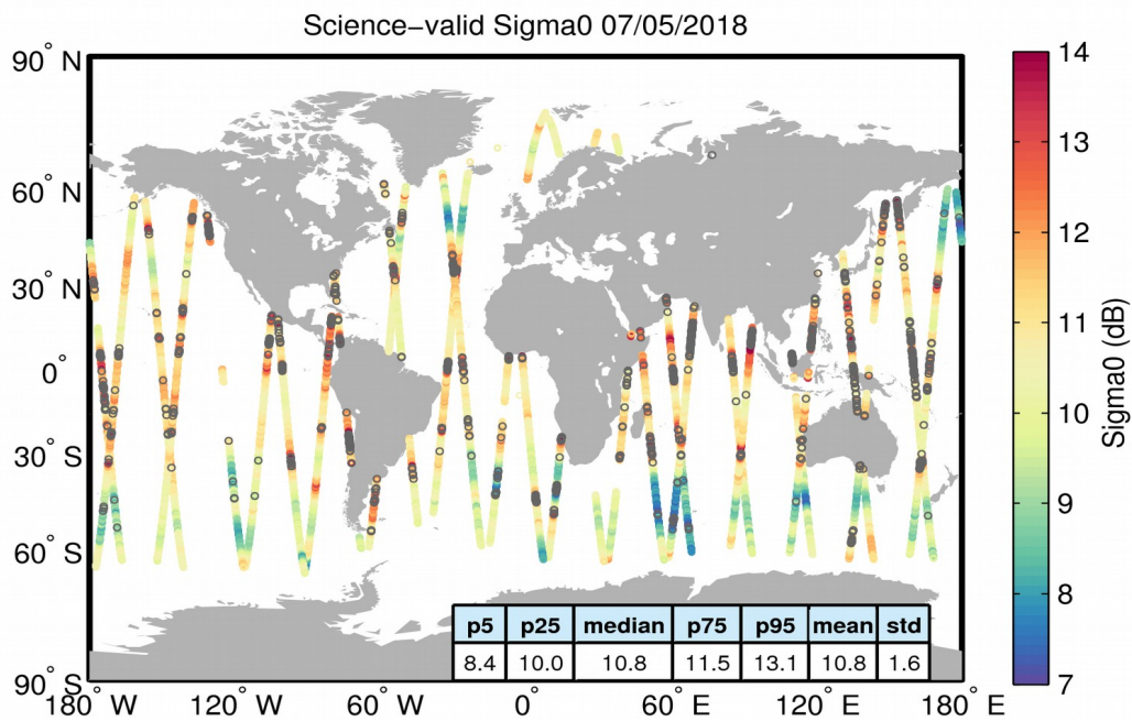
Figure 27. Geographical distribution of science-valid sigma0 data over oceans and lakes for 07/05/2018. The statistical values shown in the table refer to the sigma0 in dB and are calculated over all measurements shown in the figure. Gray circles denote records that have been rejected based on the editing criteria described in Table 4.
