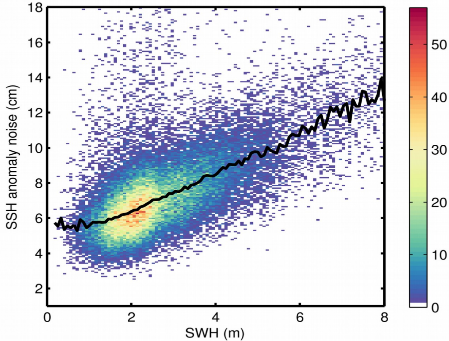
Figure 9. 2D histogram showing flag-valid SSH anomaly noise as a function of SWH for 06/05/2018. The black line denotes the median SSH anomaly noise as a function of SWH.
