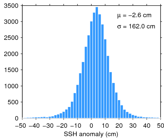
Figure 7. Histogram of flag-valid SSH anomaly over oceans and lakes for 06/05/2018. The mean ( \mu ) and standard deviation ( \sigma ) are also shown. Note that values outside [-50\ 50] cm are excluded from the histogram for the sake of readability but not from the computation of \mu and \sigma .
