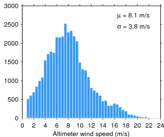
Figure 35. Histogram of science-valid wind over oceans and lakes for 06/05/2018. The mean ( \mu ) and standard deviation ( \sigma ) are also shown. Note that values larger than 24 m/s are excluded from the histogram for the sake of readability but not from the computation of \mu and \sigma .
