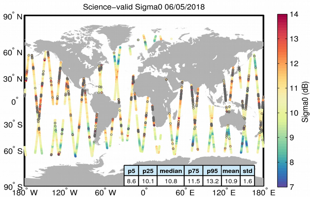
Figure 27. Geographical distribution of science-valid sigma0 data over oceans and lakes for 06/05/2018. The statistical values shown in the table refer to the sigma0 in dB and are calculated over all measurements shown in the figure. Gray circles denote records that have been rejected based on the editing criteria described in Table 4.
