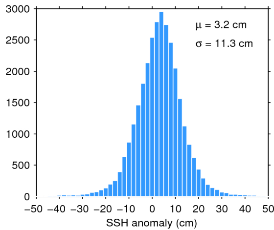
Figure 11. Histogram of science-valid SSH anomaly over oceans and lakes for 06/05/2018. The mean ( \mu ) and standard deviation ( \sigma ) are also shown. Note that values outside [-50 50] cm are excluded from the histogram for the sake of readability but not from the computation of \mu and \sigma .
