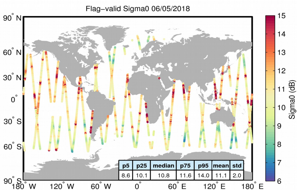
Figure 23. Geographical distribution of flag-valid sigma0 data over oceans and lakes for 06/05/2018. The statistical values shown in the table refer to the sigma0 in dB and are calculated over all measurements shown in the figure.
