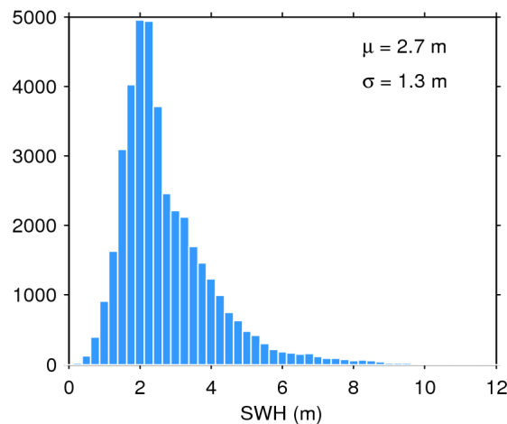
Figure 20. Histogram of science-valid SWH over oceans and lakes for 06/05/2018. The mean ( \mu ) and standard deviation ( \sigma ) are also shown. Note that values larger than 12 m are excluded from the histogram for the sake of readability but not from the computation of \mu and \sigma .
