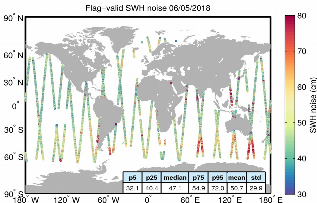
Figure 18. Geographical distribution of flag-valid 20-Hz SWH measurement noise over oceans and lakes for 06/05/2018. The statistical values shown in the figure refer to the SWH noise and are calculated over all measurements shown in the figure.
