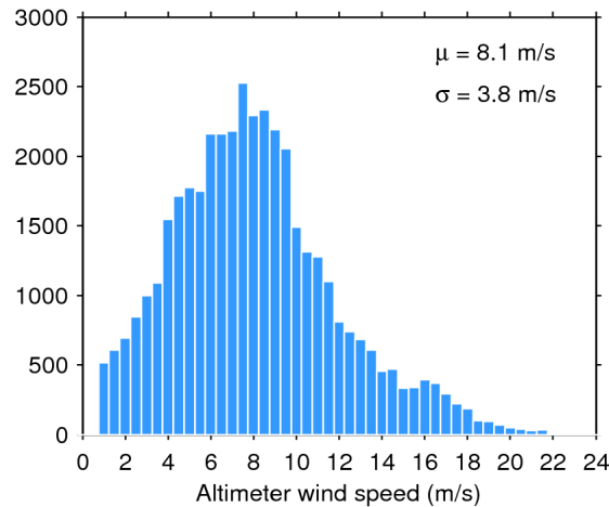
Figure 33. Histogram of flag-valid wind over oceans and lakes for 06/05/2018. The mean ( \mu ) and standard deviation ( \sigma ) are also shown. Note that values larger than 24 m/s are excluded from the histogram for the sake of readability but not from the computation of \mu and \sigma .
