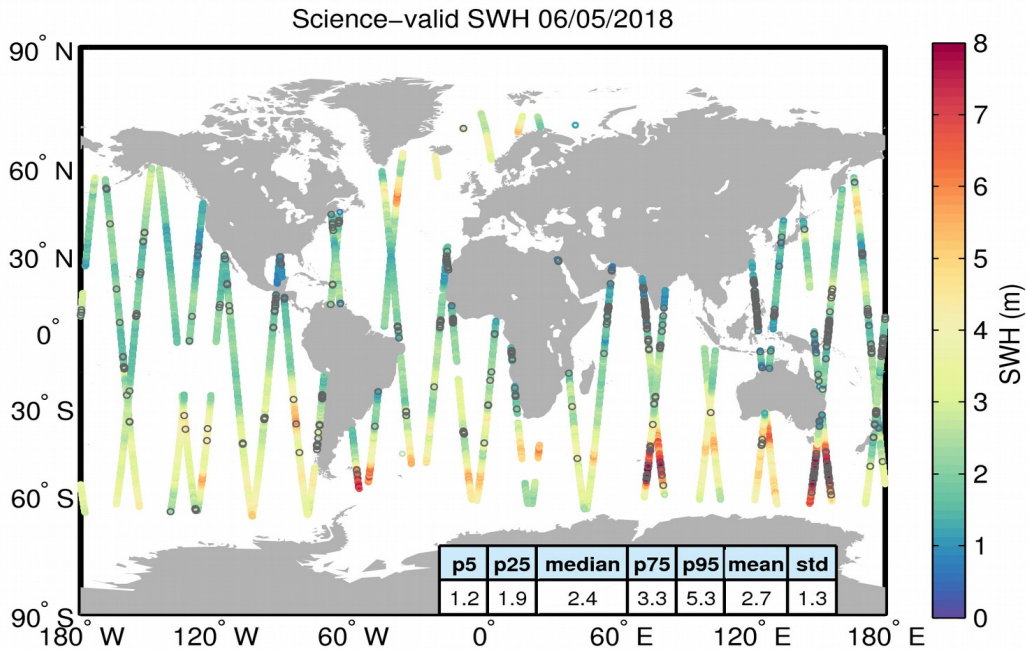
Figure 19. Geographical distribution of science-valid SWH data over oceans and lakes for 06/05/2018. The statistical values shown in the table refer to the SWH in m and are calculated over all measurements shown in the figure. Gray circles denote records that have been rejected based on the editing criteria described in Table 3.
