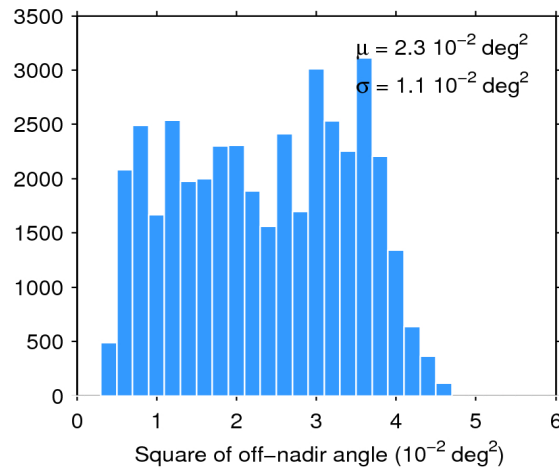
Figure 39. Histogram of flag-valid mispointing over oceans and lakes for 06/05/2018. The mean ( \mu ) and standard deviation ( \sigma ) are also shown. Note that values larger than 6 \cdot 10^{-2} \text{ deg}^2 are excluded from the histogram for the sake of readability but not from the computation of \mu and \sigma .
