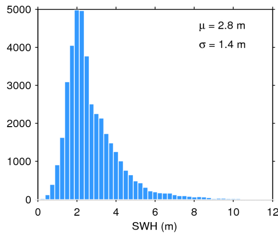
Figure 17. Histogram of flag-valid SWH over oceans and lakes for 06/05/2018. The mean ( \mu ) and standard deviation ( \sigma ) are also shown. Note that values larger than 12 m are excluded from the histogram for the sake of readability but not from the computation of \mu and \sigma .
