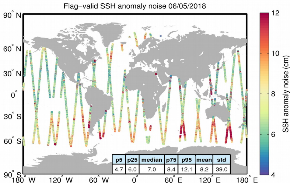
Figure 8. Geographical distribution of flag-valid 20-Hz SSH anomaly measurement noise over oceans and lakes for 06/05/2018. The statistical values shown in the table refer to the SSH anomaly noise and are calculated over all measurements shown in the figure.
