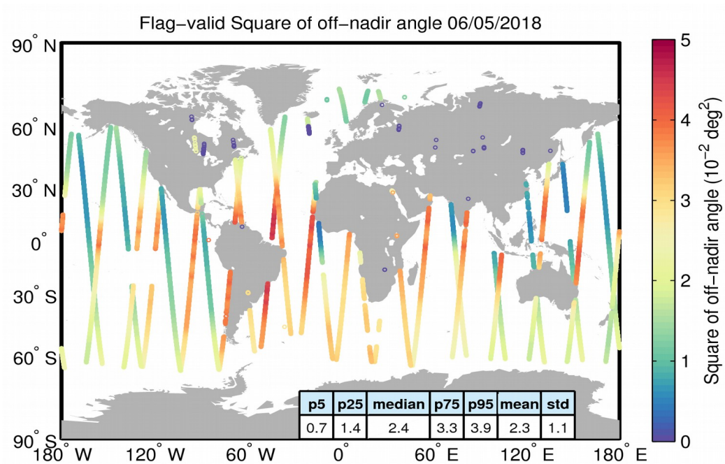
Figure 37. Geographical distribution of flag-valid mispointing data over oceans and lakes for 06/05/2018. The statistical values shown in the table refer to the mispointing in 10^{-2} deg 2 and are calculated over all measurements shown in the figure.
