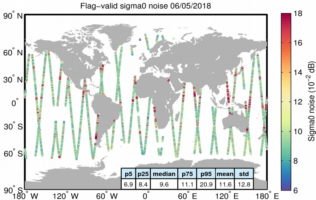
Figure 26. Geographical distribution of flag-valid 20-Hz sigma0 measurement noise over oceans and lakes for 06/05/2018. The statistical values shown in the table refer to the sigma0 noise and are calculated over all measurements shown in the figure.
