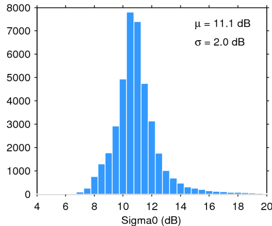
Figure 25. Histogram of flag-valid sigma0 over oceans and lakes for 06/05/2018. The mean ( \mu ) and standard deviation ( \sigma ) are also shown. Note that values outside [4 20] dB are excluded from the histogram for the sake of readability but not from the computation of \mu and \sigma .
