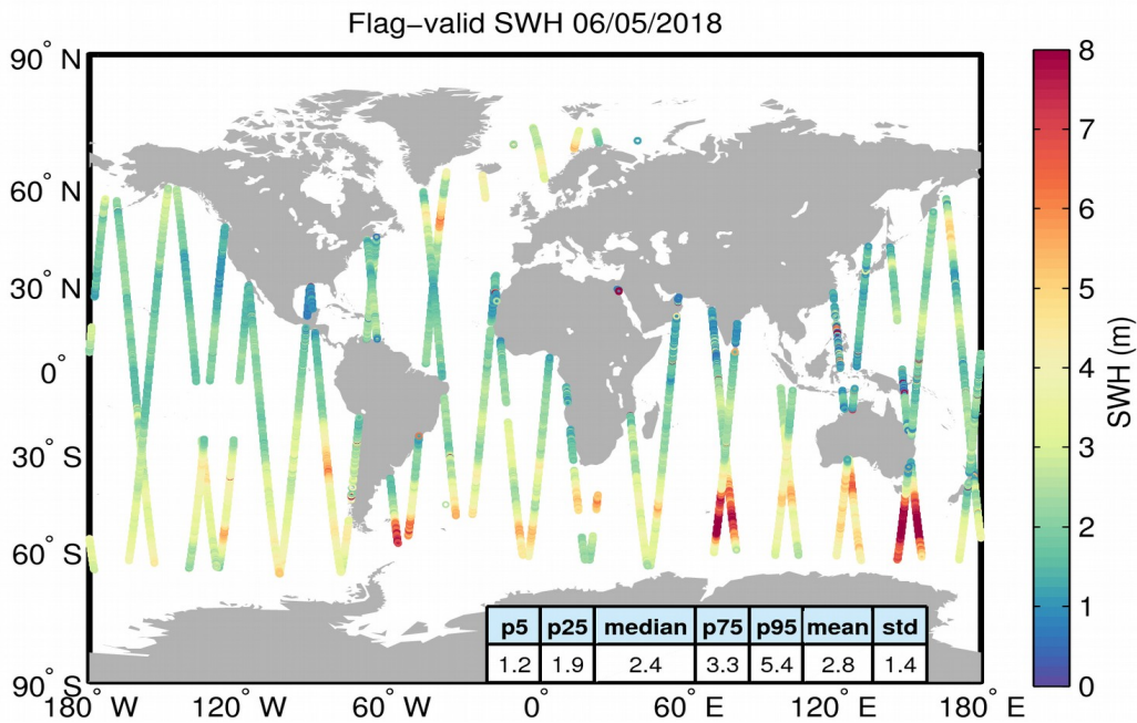
Figure 15. Geographical distribution of flag-valid SWH data over oceans and lakes for 06/05/2018. The statistical values shown in the table refer to the SWH in m and are calculated over all measurements shown in the figure.
