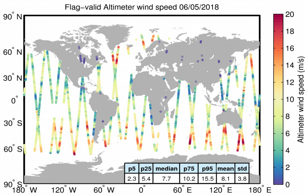
Figure 31. Geographical distribution of flag-valid wind data over oceans and lakes for 06/05/2018. The statistical values shown in the table refer to the wind in m/s and are calculated over all measurements shown in the figure.
