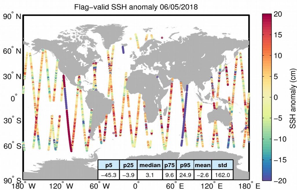
Figure 5. Geographical distribution of flag-valid 1-Hz SSH anomaly data over oceans and lakes for 06/05/2018. The statistical values shown in the table refer to the SSH anomaly in cm and are calculated over all measurements shown in the figure.
