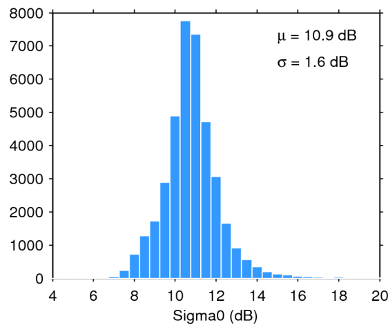
Figure 28. Histogram of science-valid sigma0 over oceans and lakes for 06/05/2018. The mean ( \mu ) and standard deviation ( \sigma ) are also shown. Note that values outside [4 20] dB are excluded from the histogram for the sake of readability but not from the computation of \mu and \sigma .
