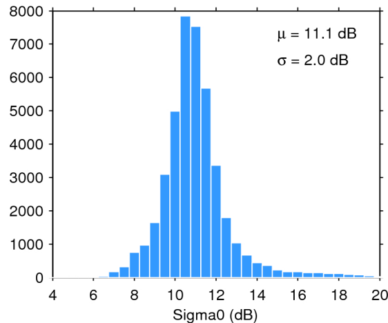
Figure 25. Histogram of flag-valid sigma0 over oceans and lakes for 05/05/2018. The mean ( \mu ) and standard deviation ( \sigma ) are also shown. Note that values outside [4 20] dB are excluded from the histogram for the sake of readability but not from the computation of \mu and \sigma .
