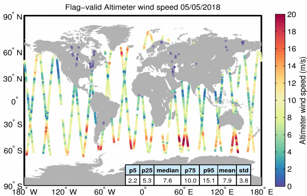
Figure 31. Geographical distribution of flag-valid wind data over oceans and lakes for 05/05/2018. The statistical values shown in the table refer to the wind in m/s and are calculated over all measurements shown in the figure.
