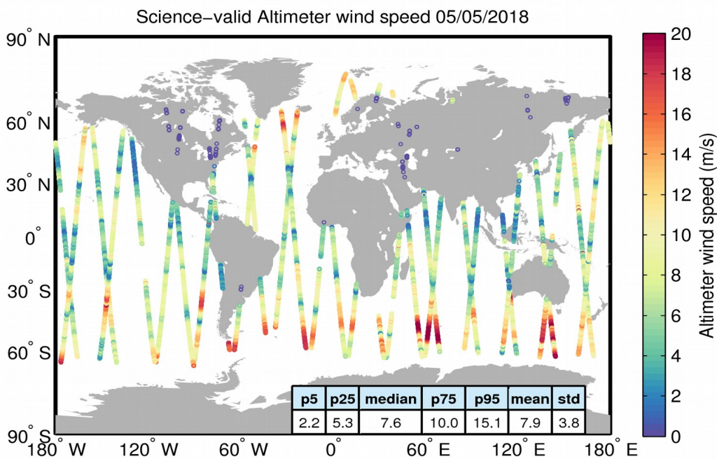
Figure 34. Geographical distribution of science-valid wind data over oceans and lakes for 05/05/2018. The statistical values shown in the table refer to the wind in m/s and are calculated over all measurements shown in the figure. Gray circles denote records that have been rejected based on the editing criteria described in Table 5.
