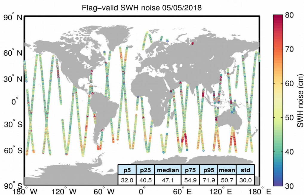
Figure 18. Geographical distribution of flag-valid 20-Hz SWH measurement noise over oceans and lakes for 05/05/2018. The statistical values shown in the figure refer to the SWH noise and are calculated over all measurements shown in the figure.
