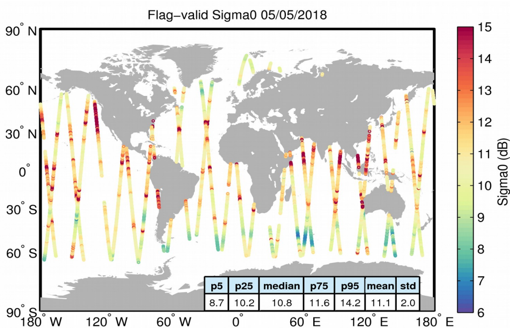
Figure 23. Geographical distribution of flag-valid sigma0 data over oceans and lakes for 05/05/2018. The statistical values shown in the table refer to the sigma0 in dB and are calculated over all measurements shown in the figure.
