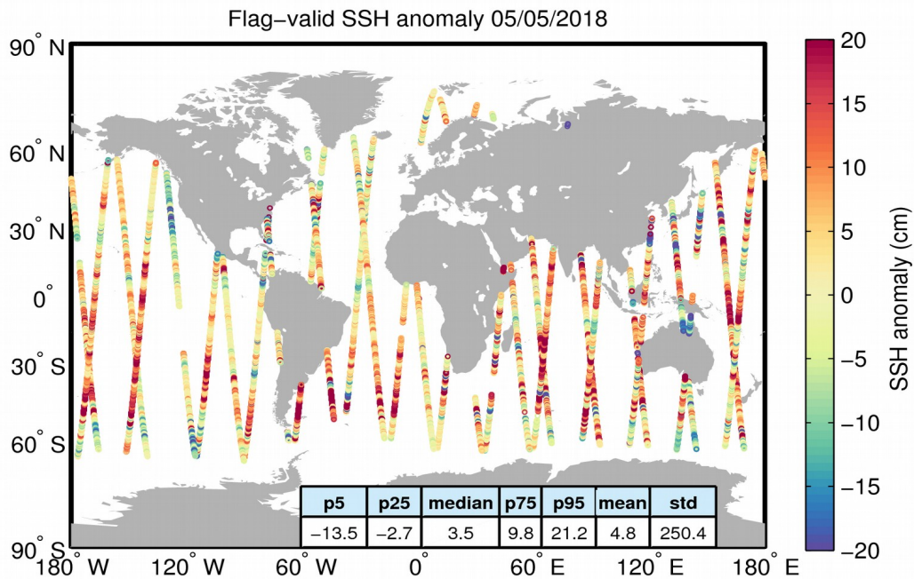
Figure 5. Geographical distribution of flag-valid 1-Hz SSH anomaly data over oceans and lakes for 05/05/2018. The statistical values shown in the table refer to the SSH anomaly in cm and are calculated over all measurements shown in the figure.
