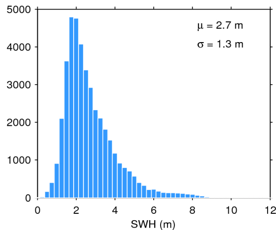
Figure 20. Histogram of science-valid SWH over oceans and lakes for 05/05/2018. The mean ( \mu ) and standard deviation ( \sigma ) are also shown. Note that values larger than 12 m are excluded from the histogram for the sake of readability but not from the computation of \mu and \sigma .
