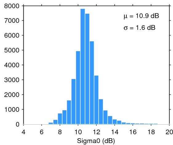
Figure 28. Histogram of science-valid sigma0 over oceans and lakes for 05/05/2018. The mean ( \mu ) and standard deviation ( \sigma ) are also shown. Note that values outside [4 20] dB are excluded from the histogram for the sake of readability but not from the computation of \mu and \sigma .
