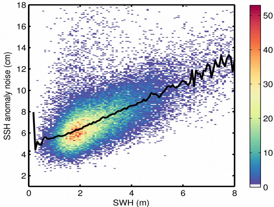
Figure 9. 2D histogram showing flag-valid SSH anomaly noise as a function of SWH for 05/05/2018. The black line denotes the median SSH anomaly noise as a function of SWH.
