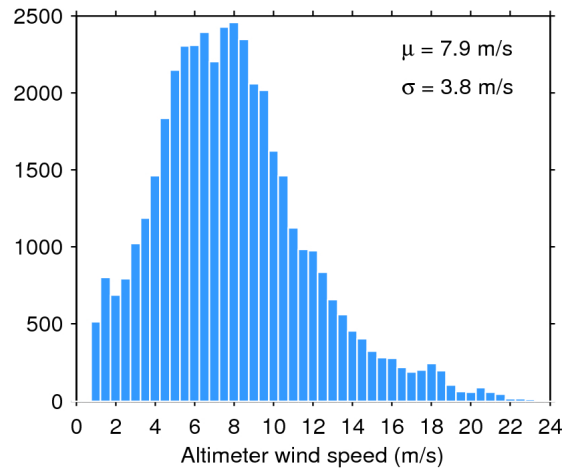
Figure 33. Histogram of flag-valid wind over oceans and lakes for 05/05/2018. The mean ( \mu ) and standard deviation ( \sigma ) are also shown. Note that values larger than 24 m/s are excluded from the histogram for the sake of readability but not from the computation of \mu and \sigma .
