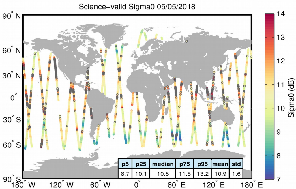
Figure 27. Geographical distribution of science-valid sigma0 data over oceans and lakes for 05/05/2018. The statistical values shown in the table refer to the sigma0 in dB and are calculated over all measurements shown in the figure. Gray circles denote records that have been rejected based on the editing criteria described in Table 4.
