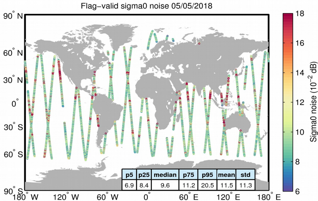
Figure 26. Geographical distribution of flag-valid 20-Hz sigma0 measurement noise over oceans and lakes for 05/05/2018. The statistical values shown in the table refer to the sigma0 noise and are calculated over all measurements shown in the figure.
