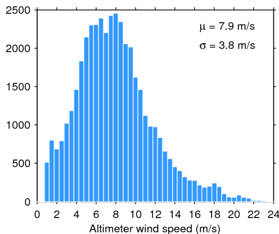
Figure 35. Histogram of science-valid wind over oceans and lakes for 05/05/2018. The mean ( \mu ) and standard deviation ( \sigma ) are also shown. Note that values larger than 24 m/s are excluded from the histogram for the sake of readability but not from the computation of \mu and \sigma .
