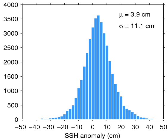
Figure 11. Histogram of science-valid SSH anomaly over oceans and lakes for 05/05/2018. The mean ( \mu ) and standard deviation ( \sigma ) are also shown. Note that values outside [-50 50] cm are excluded from the histogram for the sake of readability but not from the computation of \mu and \sigma .
