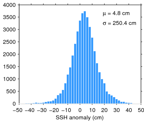
Figure 7. Histogram of flag-valid SSH anomaly over oceans and lakes for 05/05/2018. The mean ( \mu ) and standard deviation ( \sigma ) are also shown. Note that values outside [-50\ 50] cm are excluded from the histogram for the sake of readability but not from the computation of \mu and \sigma .
