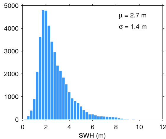
Figure 17. Histogram of flag-valid SWH over oceans and lakes for 05/05/2018. The mean ( \mu ) and standard deviation ( \sigma ) are also shown. Note that values larger than 12 m are excluded from the histogram for the sake of readability but not from the computation of \mu and \sigma .
