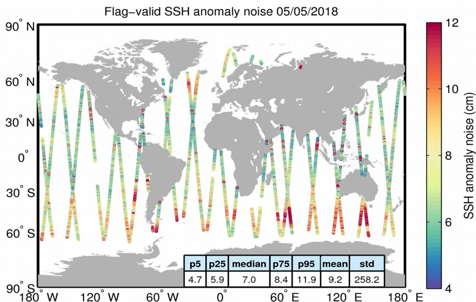
Figure 8. Geographical distribution of flag-valid 20-Hz SSH anomaly measurement noise over oceans and lakes for 05/05/2018. The statistical values shown in the table refer to the SSH anomaly noise and are calculated over all measurements shown in the figure.
