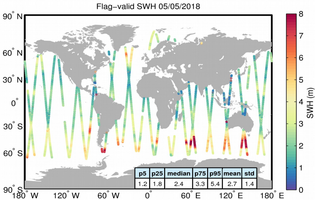
Figure 15. Geographical distribution of flag-valid SWH data over oceans and lakes for 05/05/2018. The statistical values shown in the table refer to the SWH in m and are calculated over all measurements shown in the figure.
