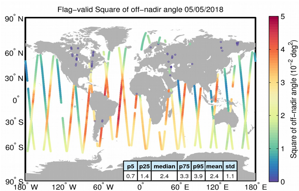
Figure 37. Geographical distribution of flag-valid mispointing data over oceans and lakes for 05/05/2018. The statistical values shown in the table refer to the mispointing in 10^{-2} deg 2 and are calculated over all measurements shown in the figure.
