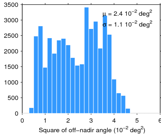
Figure 39. Histogram of flag-valid mispointing over oceans and lakes for 05/05/2018. The mean ( \mu ) and standard deviation ( \sigma ) are also shown. Note that values larger than 6 \cdot 10^{-2} \text{ deg}^2 are excluded from the histogram for the sake of readability but not from the computation of \mu and \sigma .
