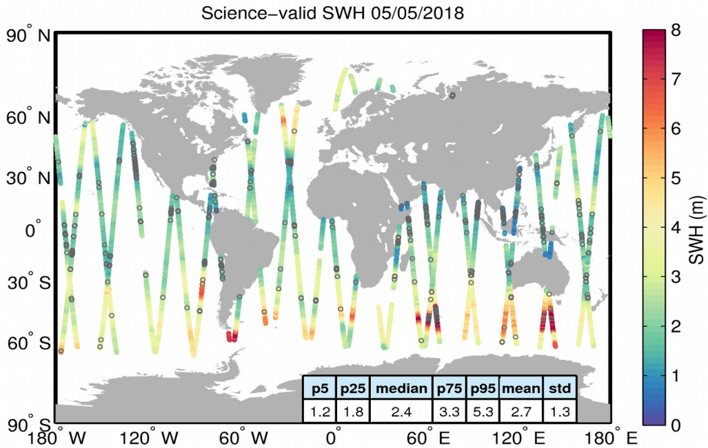
Figure 19. Geographical distribution of science-valid SWH data over oceans and lakes for 05/05/2018. The statistical values shown in the table refer to the SWH in m and are calculated over all measurements shown in the figure. Gray circles denote records that have been rejected based on the editing criteria described in Table 3.
