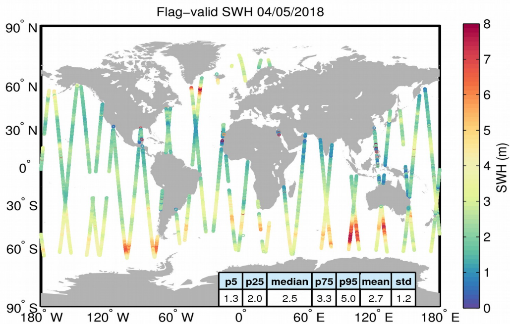
Figure 15. Geographical distribution of flag-valid SWH data over oceans and lakes for 04/05/2018. The statistical values shown in the table refer to the SWH in m and are calculated over all measurements shown in the figure.
