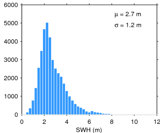
Figure 20. Histogram of science-valid SWH over oceans and lakes for 04/05/2018. The mean ( \mu ) and standard deviation ( \sigma ) are also shown. Note that values larger than 12 m are excluded from the histogram for the sake of readability but not from the computation of \mu and \sigma .
