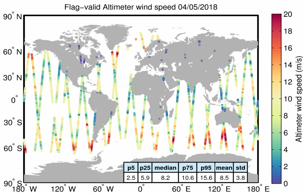
Figure 31. Geographical distribution of flag-valid wind data over oceans and lakes for 04/05/2018. The statistical values shown in the table refer to the wind in m/s and are calculated over all measurements shown in the figure.
