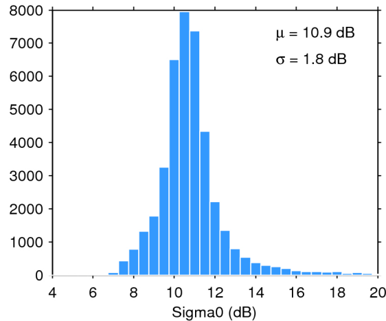
Figure 25. Histogram of flag-valid sigma0 over oceans and lakes for 04/05/2018. The mean ( \mu ) and standard deviation ( \sigma ) are also shown. Note that values outside [4 20] dB are excluded from the histogram for the sake of readability but not from the computation of \mu and \sigma .
