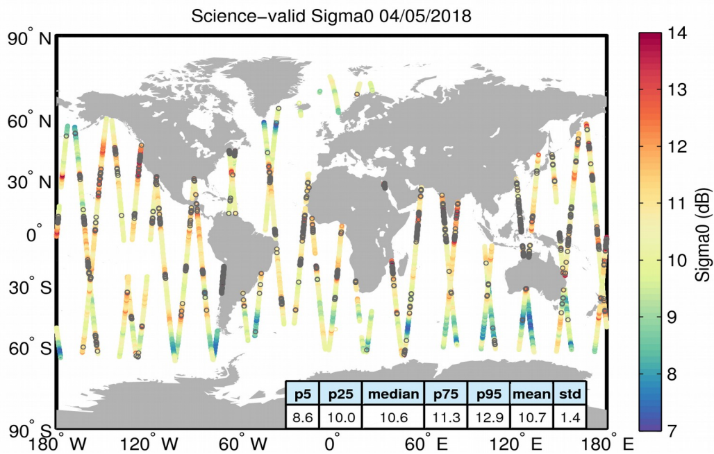
Figure 27. Geographical distribution of science-valid sigma0 data over oceans and lakes for 04/05/2018. The statistical values shown in the table refer to the sigma0 in dB and are calculated over all measurements shown in the figure. Gray circles denote records that have been rejected based on the editing criteria described in Table 4.
