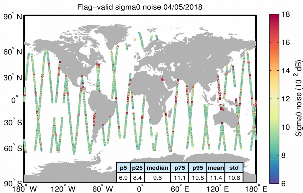
Figure 26. Geographical distribution of flag-valid 20-Hz sigma0 measurement noise over oceans and lakes for 04/05/2018. The statistical values shown in the table refer to the sigma0 noise and are calculated over all measurements shown in the figure.
