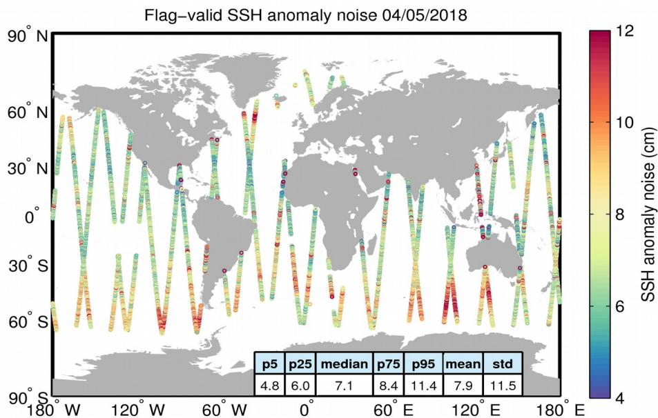
Figure 8. Geographical distribution of flag-valid 20-Hz SSH anomaly measurement noise over oceans and lakes for 04/05/2018. The statistical values shown in the table refer to the SSH anomaly noise and are calculated over all measurements shown in the figure.
