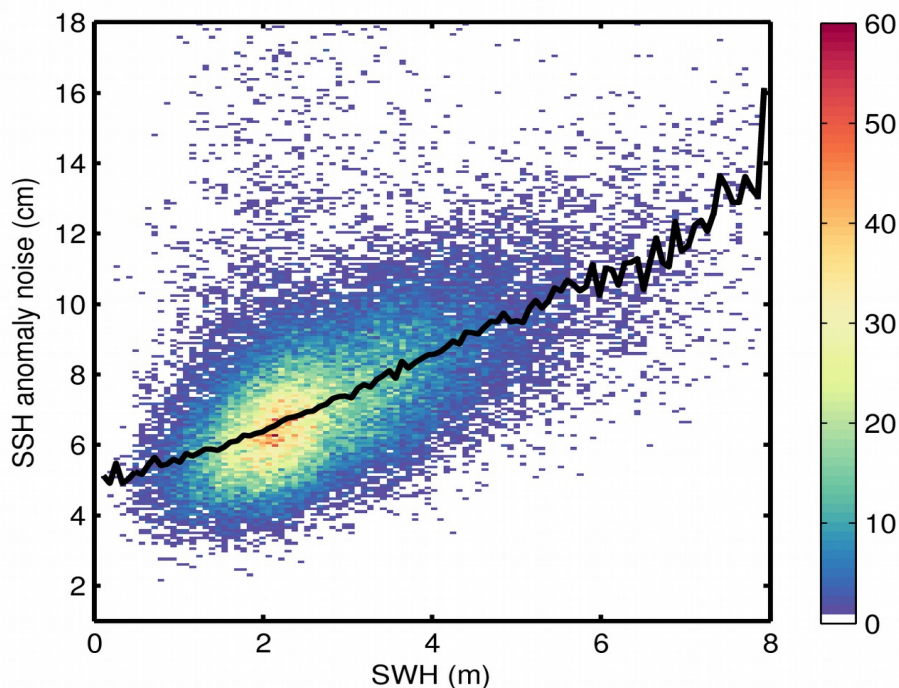
Figure 9. 2D histogram showing flag-valid SSH anomaly noise as a function of SWH for 04/05/2018. The black line denotes the median SSH anomaly noise as a function of SWH.
