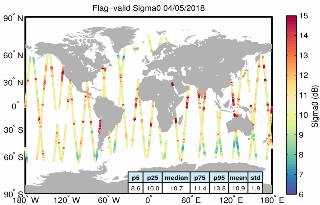
Figure 23. Geographical distribution of flag-valid sigma0 data over oceans and lakes for 04/05/2018. The statistical values shown in the table refer to the sigma0 in dB and are calculated over all measurements shown in the figure.
