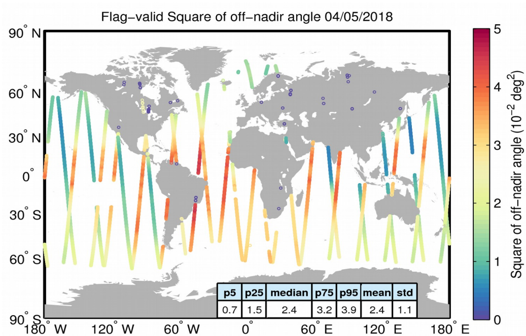
Figure 37. Geographical distribution of flag-valid mispointing data over oceans and lakes for 04/05/2018. The statistical values shown in the table refer to the mispointing in 10^{-2} \text{ deg}^2 and are calculated over all measurements shown in the figure.
