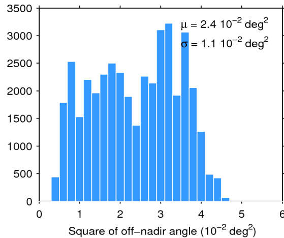
Figure 39. Histogram of flag-valid mispointing over oceans and lakes for 04/05/2018. The mean ( \mu ) and standard deviation ( \sigma ) are also shown. Note that values larger than 6 \cdot 10^{-2} \text{ deg}^2 are excluded from the histogram for the sake of readability but not from the computation of \mu and \sigma .
