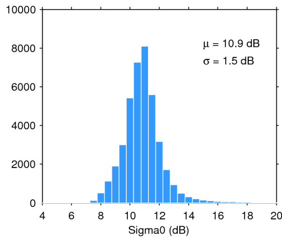
Figure 28. Histogram of science-valid sigma0 over oceans and lakes for 03/05/2018. The mean ( \mu ) and standard deviation ( \sigma ) are also shown. Note that values outside [4 20] dB are excluded from the histogram for the sake of readability but not from the computation of \mu and \sigma .
