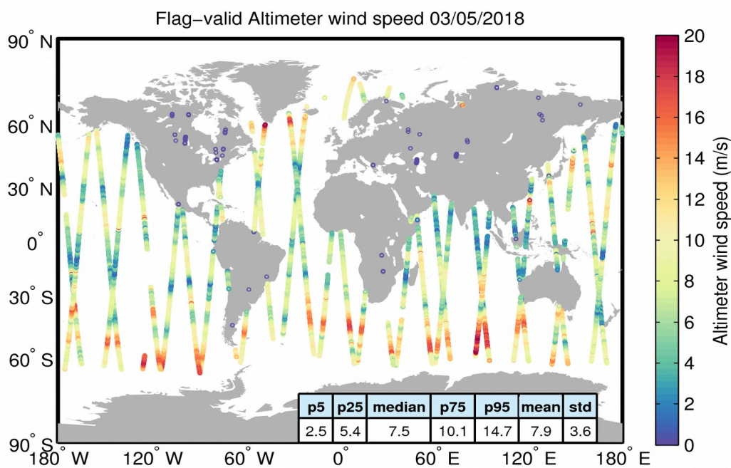
Figure 31. Geographical distribution of flag-valid wind data over oceans and lakes for 03/05/2018. The statistical values shown in the table refer to the wind in m/s and are calculated over all measurements shown in the figure.
