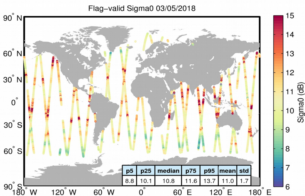
Figure 23. Geographical distribution of flag-valid sigma0 data over oceans and lakes for 03/05/2018. The statistical values shown in the table refer to the sigma0 in dB and are calculated over all measurements shown in the figure.
