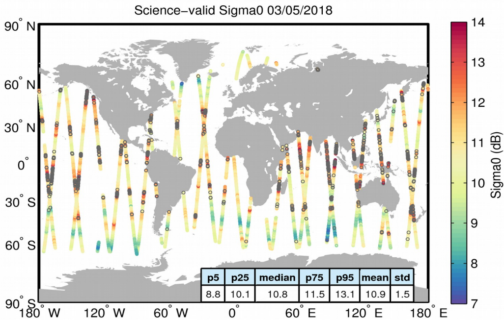
Figure 27. Geographical distribution of science-valid sigma0 data over oceans and lakes for 03/05/2018. The statistical values shown in the table refer to the sigma0 in dB and are calculated over all measurements shown in the figure. Gray circles denote records that have been rejected based on the editing criteria described in Table 4.
