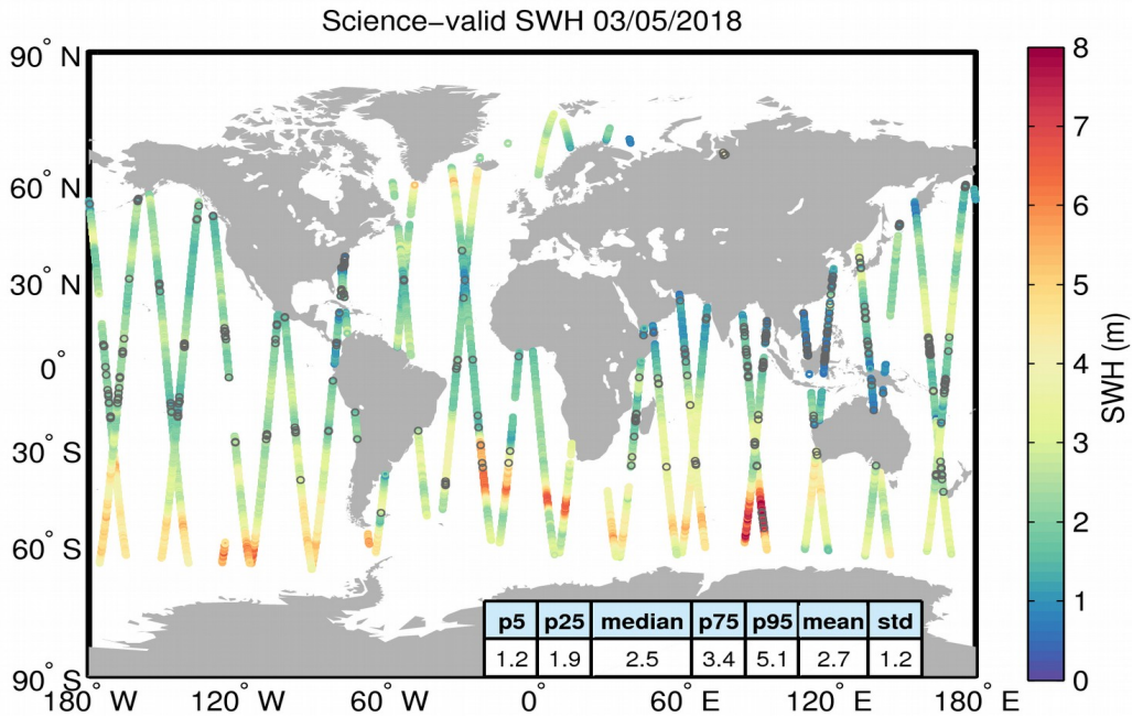
Figure 19. Geographical distribution of science-valid SWH data over oceans and lakes for 03/05/2018. The statistical values shown in the table refer to the SWH in m and are calculated over all measurements shown in the figure. Gray circles denote records that have been rejected based on the editing criteria described in Table 3.
