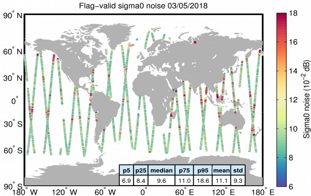
Figure 26. Geographical distribution of flag-valid 20-Hz sigma0 measurement noise over oceans and lakes for 03/05/2018. The statistical values shown in the table refer to the sigma0 noise and are calculated over all measurements shown in the figure.
