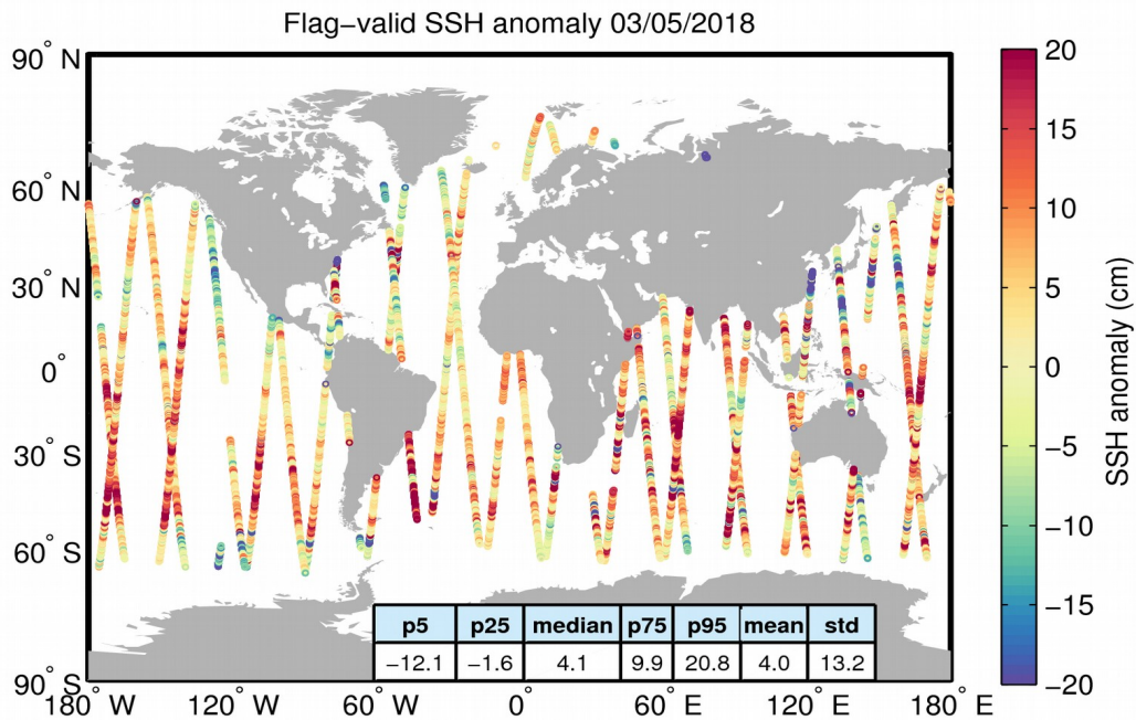
Figure 5. Geographical distribution of flag-valid 1-Hz SSH anomaly data over oceans and lakes for 03/05/2018. The statistical values shown in the table refer to the SSH anomaly in cm and are calculated over all measurements shown in the figure.
