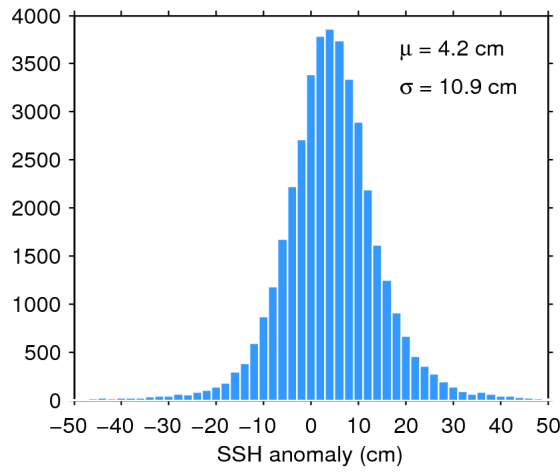
Figure 11. Histogram of science-valid SSH anomaly over oceans and lakes for 03/05/2018. The mean ( \mu ) and standard deviation ( \sigma ) are also shown. Note that values outside [-50 50] cm are excluded from the histogram for the sake of readability but not from the computation of \mu and \sigma .
