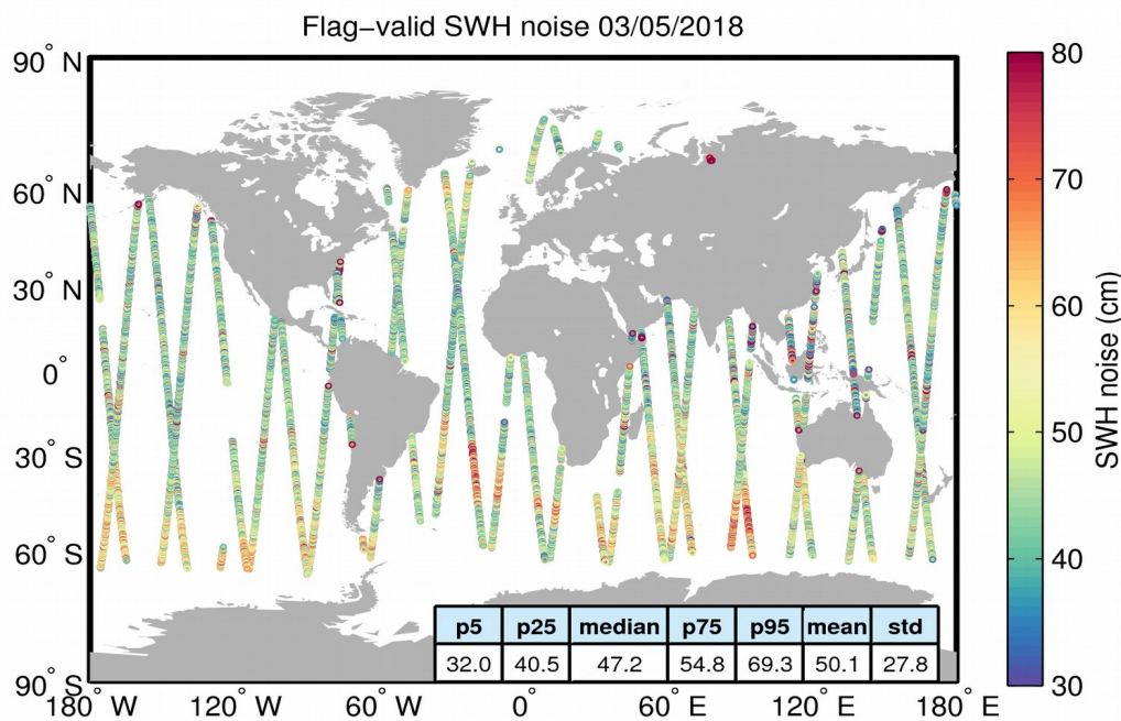
Figure 18. Geographical distribution of flag-valid 20-Hz SWH measurement noise over oceans and lakes for 03/05/2018. The statistical values shown in the figure refer to the SWH noise and are calculated over all measurements shown in the figure.
