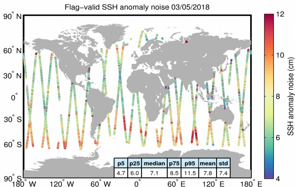
Figure 8. Geographical distribution of flag-valid 20-Hz SSH anomaly measurement noise over oceans and lakes for 03/05/2018. The statistical values shown in the table refer to the SSH anomaly noise and are calculated over all measurements shown in the figure.
