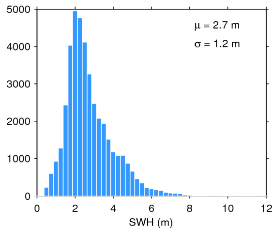
Figure 20. Histogram of science-valid SWH over oceans and lakes for 03/05/2018. The mean ( \mu ) and standard deviation ( \sigma ) are also shown. Note that values larger than 12 m are excluded from the histogram for the sake of readability but not from the computation of \mu and \sigma .
