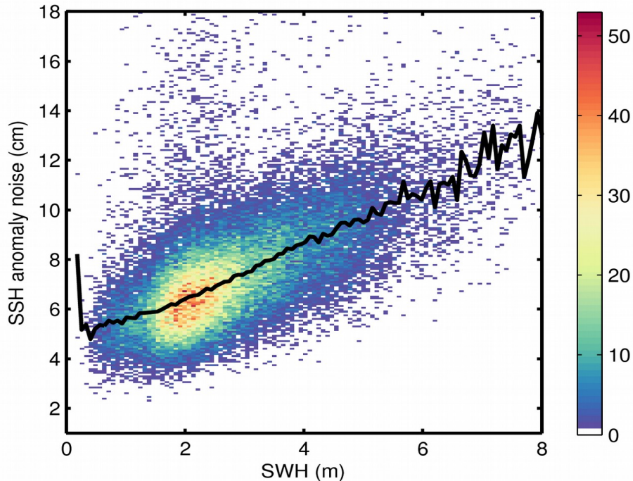
Figure 9. 2D histogram showing flag-valid SSH anomaly noise as a function of SWH for 03/05/2018. The black line denotes the median SSH anomaly noise as a function of SWH.
