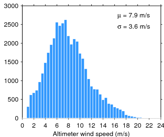
Figure 35. Histogram of science-valid wind over oceans and lakes for 03/05/2018. The mean ( \mu ) and standard deviation ( \sigma ) are also shown. Note that values larger than 24 m/s are excluded from the histogram for the sake of readability but not from the computation of \mu and \sigma .
