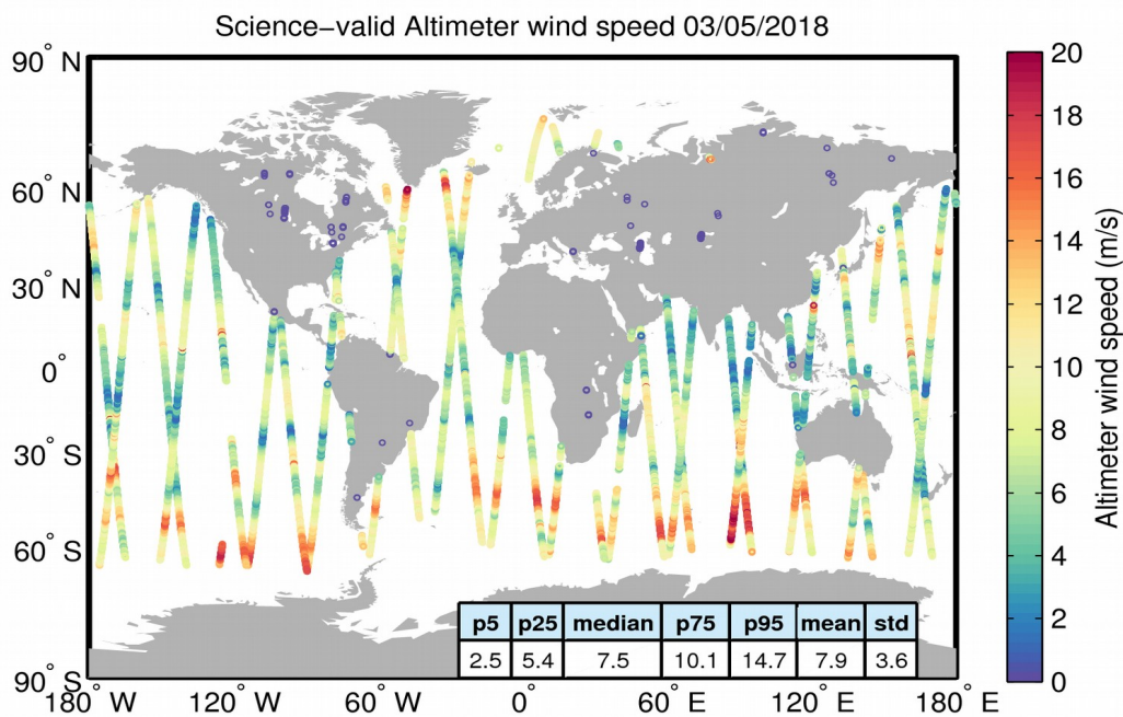
Figure 34. Geographical distribution of science-valid wind data over oceans and lakes for 03/05/2018. The statistical values shown in the table refer to the wind in m/s and are calculated over all measurements shown in the figure. Gray circles denote records that have been rejected based on the editing criteria described in Table 5.
