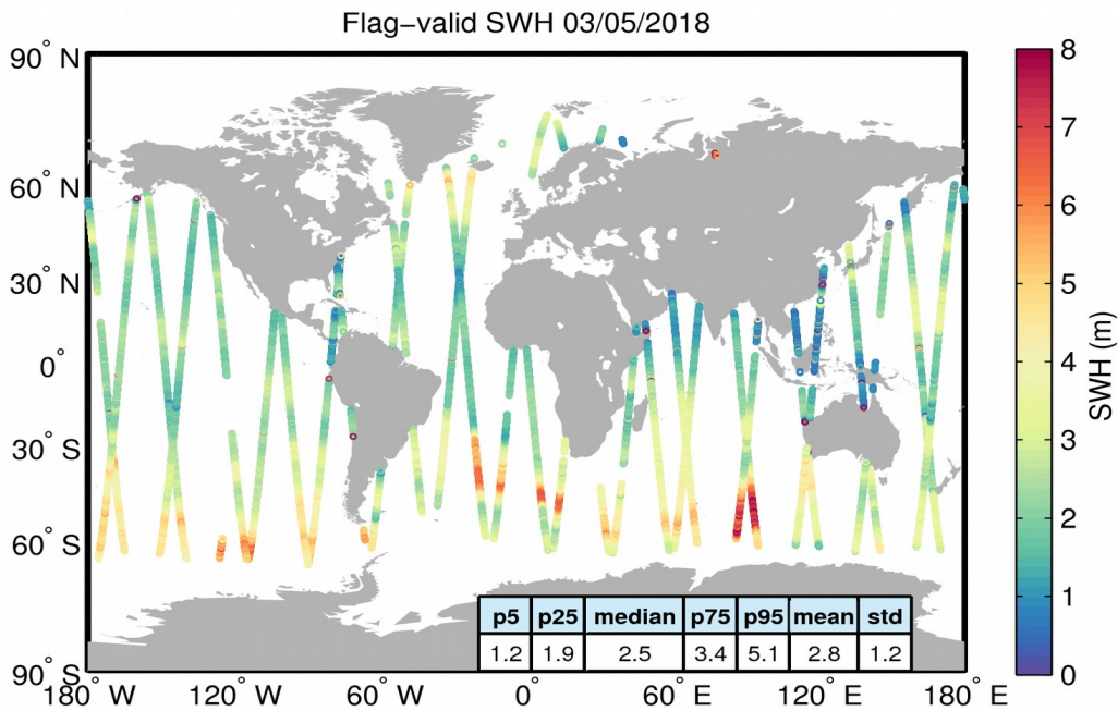
Figure 15. Geographical distribution of flag-valid SWH data over oceans and lakes for 03/05/2018. The statistical values shown in the table refer to the SWH in m and are calculated over all measurements shown in the figure.
