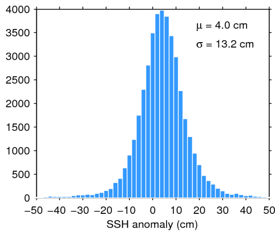
Figure 7. Histogram of flag-valid SSH anomaly over oceans and lakes for 03/05/2018. The mean ( \mu ) and standard deviation ( \sigma ) are also shown. Note that values outside [-50\ 50] cm are excluded from the histogram for the sake of readability but not from the computation of \mu and \sigma .
