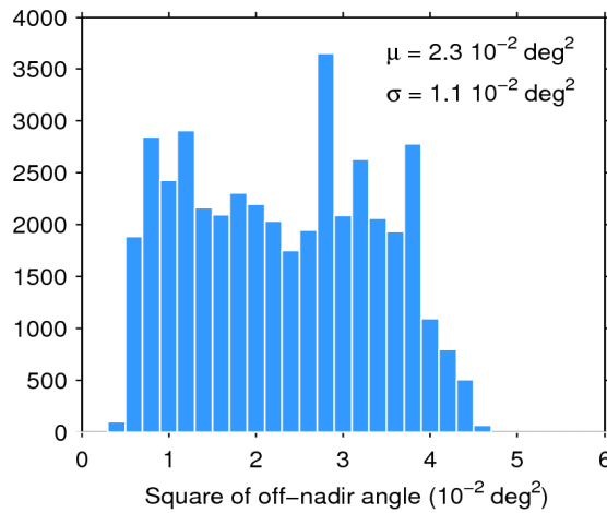
Figure 39. Histogram of flag-valid mispointing over oceans and lakes for 03/05/2018. The mean ( \mu ) and standard deviation ( \sigma ) are also shown. Note that values larger than 6 \cdot 10^{-2} \text{ deg}^2 are excluded from the histogram for the sake of readability but not from the computation of \mu and \sigma .
