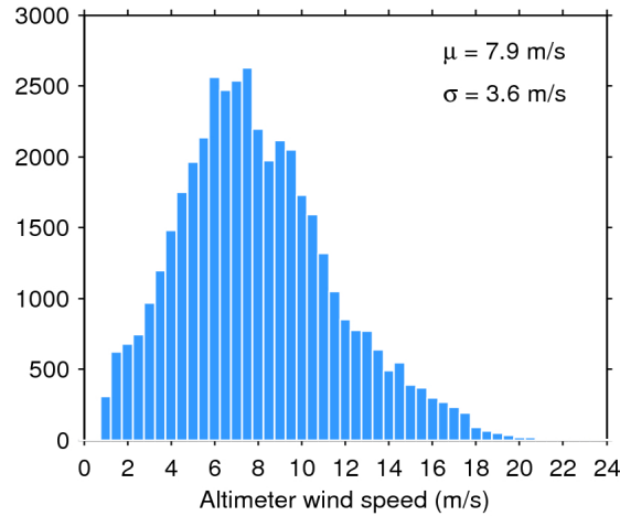
Figure 33. Histogram of flag-valid wind over oceans and lakes for 03/05/2018. The mean ( \mu ) and standard deviation ( \sigma ) are also shown. Note that values larger than 24 m/s are excluded from the histogram for the sake of readability but not from the computation of \mu and \sigma .
