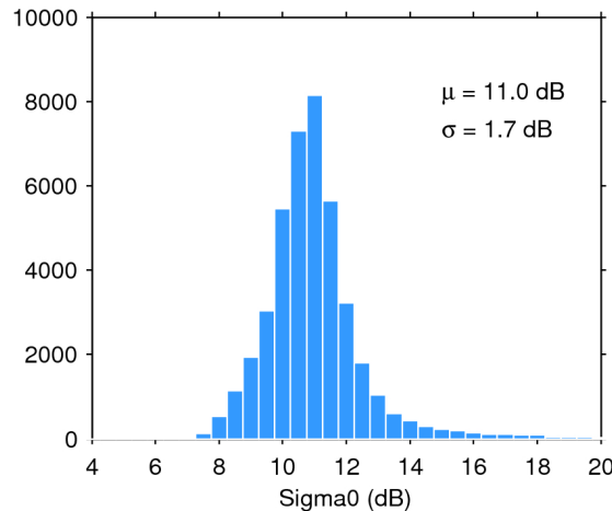
Figure 25. Histogram of flag-valid sigma0 over oceans and lakes for 03/05/2018. The mean ( \mu ) and standard deviation ( \sigma ) are also shown. Note that values outside [4 20] dB are excluded from the histogram for the sake of readability but not from the computation of \mu and \sigma .
