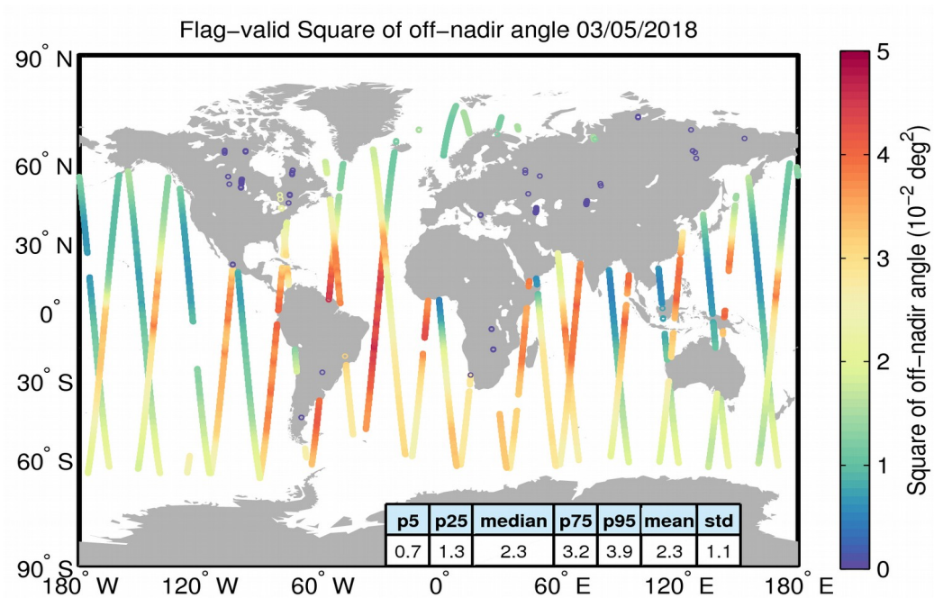
Figure 37. Geographical distribution of flag-valid mispointing data over oceans and lakes for 03/05/2018. The statistical values shown in the table refer to the mispointing in 10^{-2} \text{deg}^2 and are calculated over all measurements shown in the figure.
