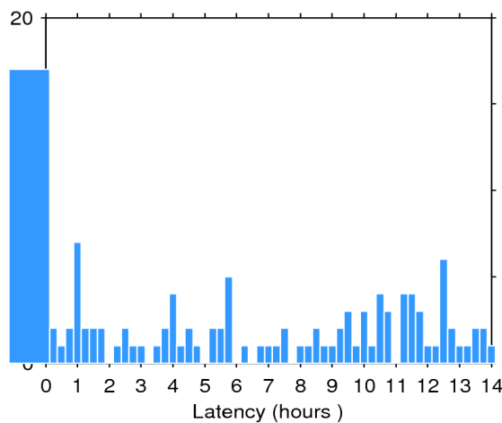
Figure 2. Histogram of the data latency for 03/05/2018. The y-axis denotes the number of files that are made available with a delay of x-hours with respect to the mean time of the records stored in the file.
