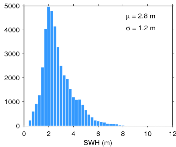
Figure 17. Histogram of flag-valid SWH over oceans and lakes for 03/05/2018. The mean ( \mu ) and standard deviation ( \sigma ) are also shown. Note that values larger than 12 m are excluded from the histogram for the sake of readability but not from the computation of \mu and \sigma .
