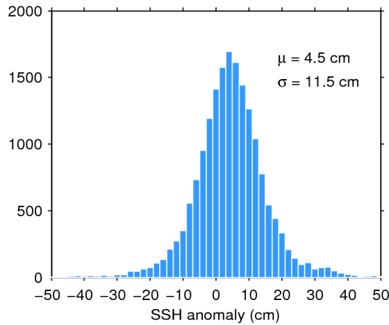
Figure 11. Histogram of science-valid SSH anomaly over oceans and lakes for 02/05/2018. The mean ( \mu ) and standard deviation ( \sigma ) are also shown. Note that values outside [-50 50] cm are excluded from the histogram for the sake of readability but not from the computation of \mu and \sigma .
