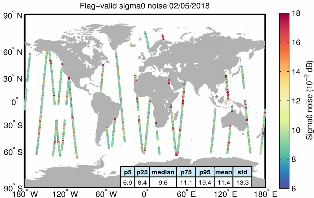
Figure 26. Geographical distribution of flag-valid 20-Hz sigma0 measurement noise over oceans and lakes for 02/05/2018. The statistical values shown in the table refer to the sigma0 noise and are calculated over all measurements shown in the figure.
