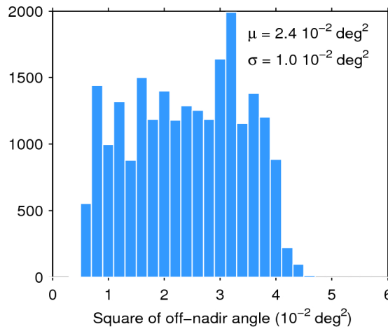
Figure 39. Histogram of flag-valid mispointing over oceans and lakes for 02/05/2018. The mean ( \mu ) and standard deviation ( \sigma ) are also shown. Note that values larger than 6 \cdot 10^{-2} \text{ deg}^2 are excluded from the histogram for the sake of readability but not from the computation of \mu and \sigma .
