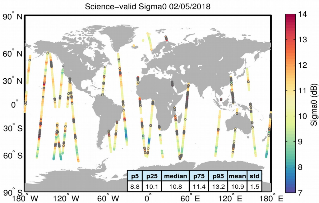
Figure 27. Geographical distribution of science-valid sigma0 data over oceans and lakes for 02/05/2018. The statistical values shown in the table refer to the sigma0 in dB and are calculated over all measurements shown in the figure. Gray circles denote records that have been rejected based on the editing criteria described in Table 4.
