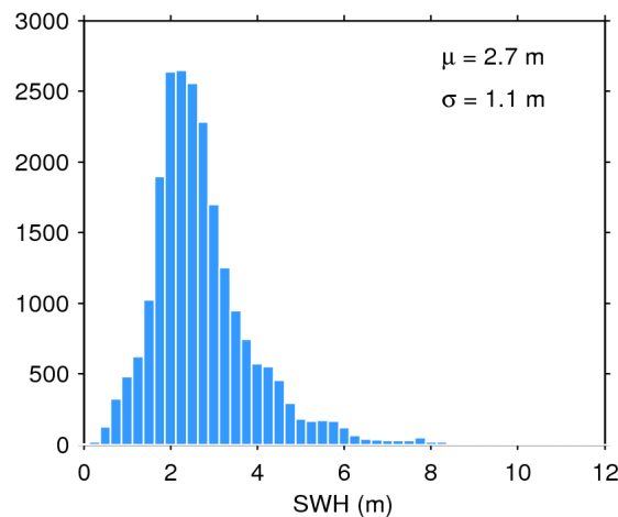
Figure 20. Histogram of science-valid SWH over oceans and lakes for 02/05/2018. The mean ( \mu ) and standard deviation ( \sigma ) are also shown. Note that values larger than 12 m are excluded from the histogram for the sake of readability but not from the computation of \mu and \sigma .
