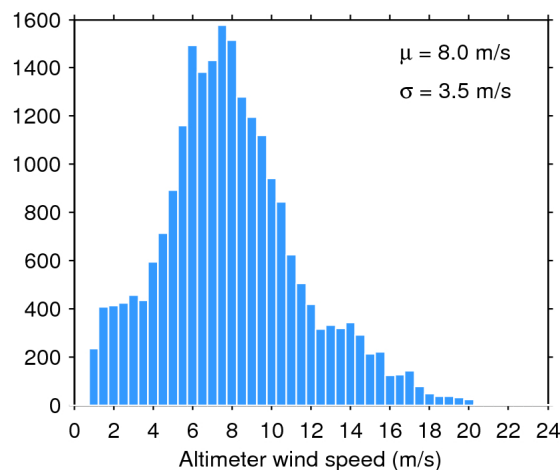
Figure 35. Histogram of science-valid wind over oceans and lakes for 02/05/2018. The mean ( \mu ) and standard deviation ( \sigma ) are also shown. Note that values larger than 24 m/s are excluded from the histogram for the sake of readability but not from the computation of \mu and \sigma .
