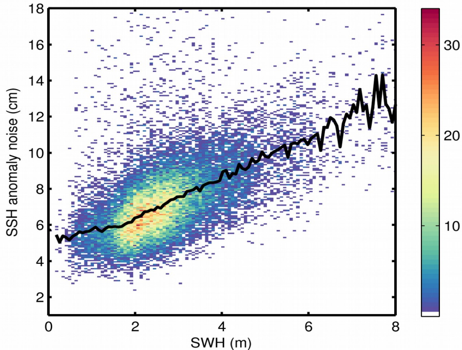
Figure 9. 2D histogram showing flag-valid SSH anomaly noise as a function of SWH for 02/05/2018. The black line denotes the median SSH anomaly noise as a function of SWH.
