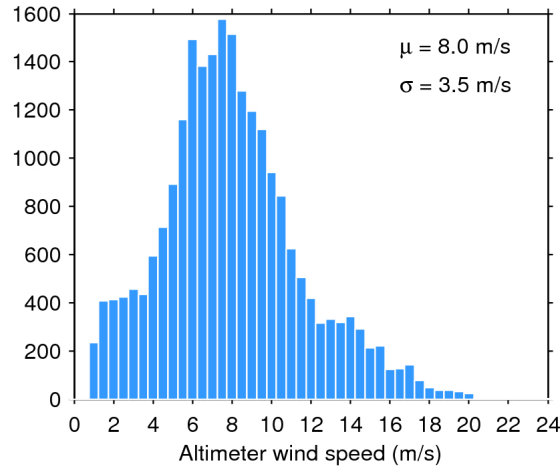
Figure 33. Histogram of flag-valid wind over oceans and lakes for 02/05/2018. The mean ( \mu ) and standard deviation ( \sigma ) are also shown. Note that values larger than 24 m/s are excluded from the histogram for the sake of readability but not from the computation of \mu and \sigma .
