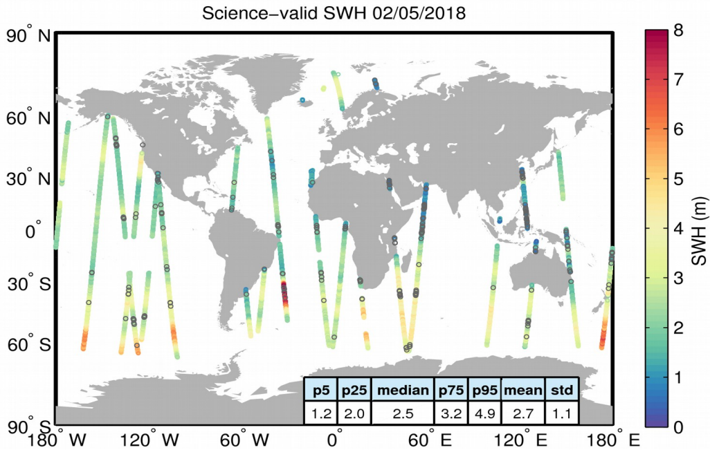
Figure 19. Geographical distribution of science-valid SWH data over oceans and lakes for 02/05/2018. The statistical values shown in the table refer to the SWH in m and are calculated over all measurements shown in the figure. Gray circles denote records that have been rejected based on the editing criteria described in Table 3.
