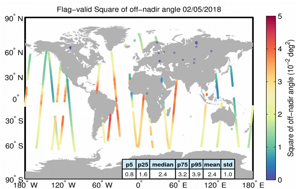
Figure 37. Geographical distribution of flag-valid mispointing data over oceans and lakes for 02/05/2018. The statistical values shown in the table refer to the mispointing in 10^{-2} \text{ deg}^2 and are calculated over all measurements shown in the figure.
