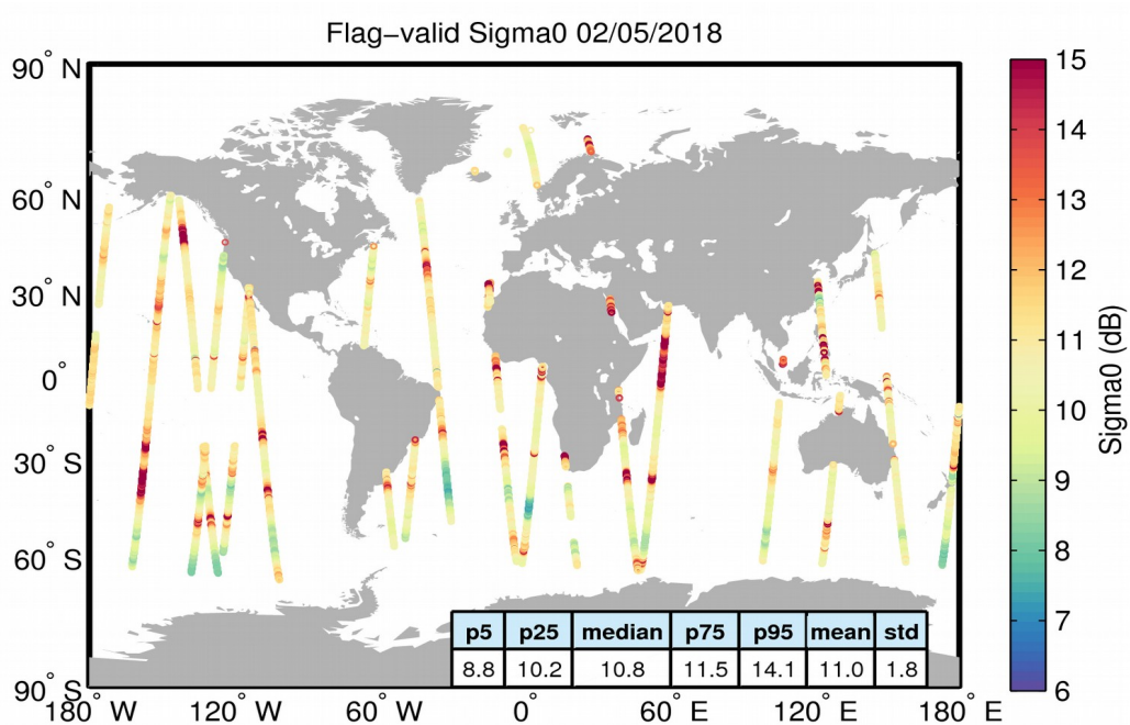
Figure 23. Geographical distribution of flag-valid sigma0 data over oceans and lakes for 02/05/2018. The statistical values shown in the table refer to the sigma0 in dB and are calculated over all measurements shown in the figure.
