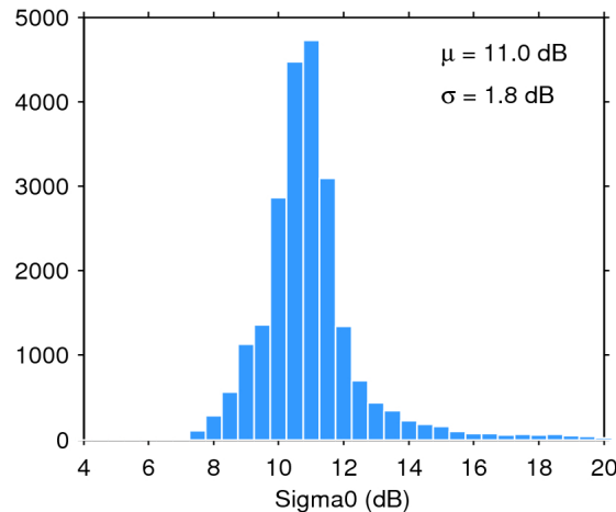
Figure 25. Histogram of flag-valid sigma0 over oceans and lakes for 02/05/2018. The mean ( \mu ) and standard deviation ( \sigma ) are also shown. Note that values outside [4 20] dB are excluded from the histogram for the sake of readability but not from the computation of \mu and \sigma .
