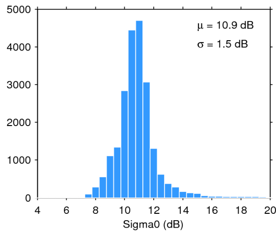
Figure 28. Histogram of science-valid sigma0 over oceans and lakes for 02/05/2018. The mean ( \mu ) and standard deviation ( \sigma ) are also shown. Note that values outside [4 20] dB are excluded from the histogram for the sake of readability but not from the computation of \mu and \sigma .
