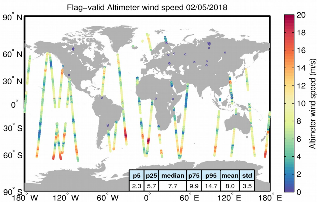
Figure 31. Geographical distribution of flag-valid wind data over oceans and lakes for 02/05/2018. The statistical values shown in the table refer to the wind in m/s and are calculated over all measurements shown in the figure.
