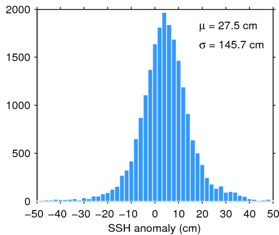
Figure 7. Histogram of flag-valid SSH anomaly over oceans and lakes for 02/05/2018. The mean ( \mu ) and standard deviation ( \sigma ) are also shown. Note that values outside [-50\ 50] cm are excluded from the histogram for the sake of readability but not from the computation of \mu and \sigma .
