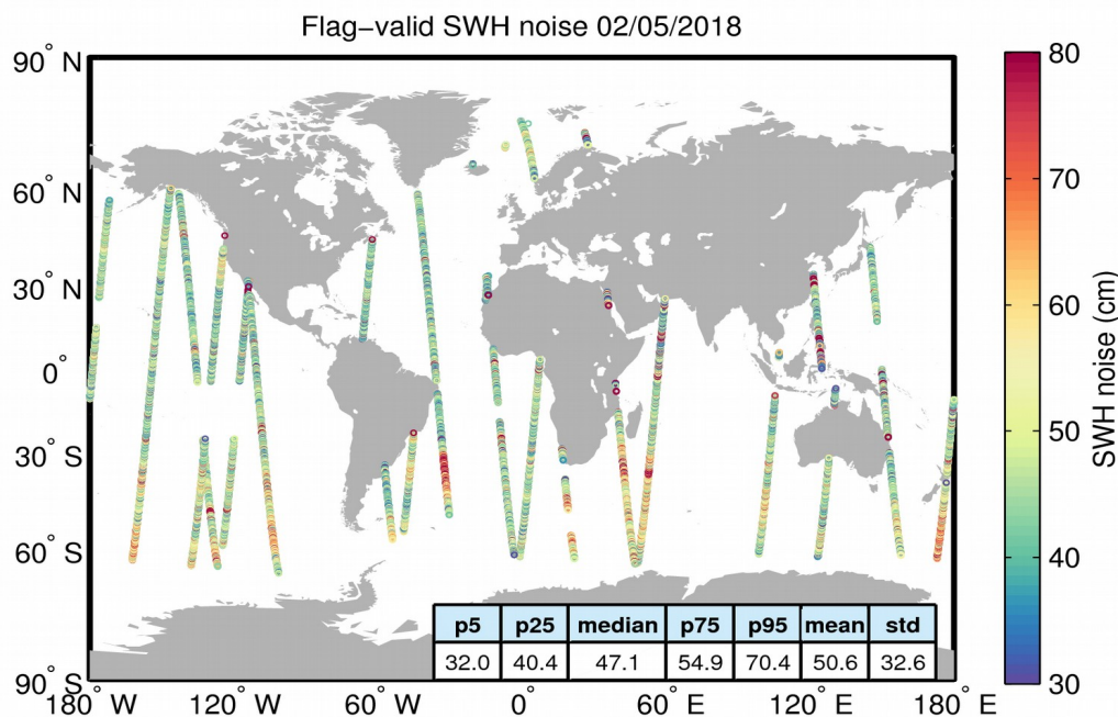
Figure 18. Geographical distribution of flag-valid 20-Hz SWH measurement noise over oceans and lakes for 02/05/2018. The statistical values shown in the figure refer to the SWH noise and are calculated over all measurements shown in the figure.
