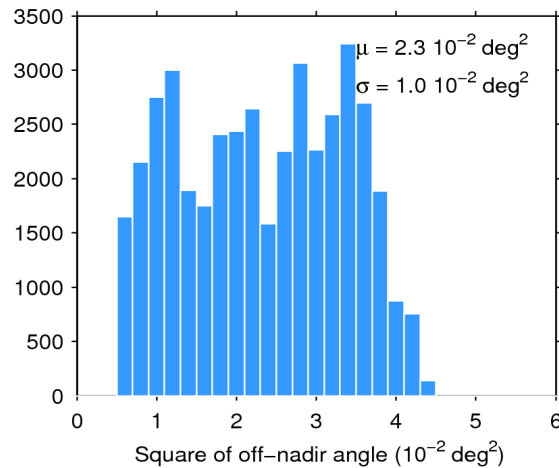
Figure 39. Histogram of flag-valid mispointing over oceans and lakes for 01/05/2018. The mean ( \mu ) and standard deviation ( \sigma ) are also shown. Note that values larger than 6 \cdot 10^{-2} \text{ deg}^2 are excluded from the histogram for the sake of readability but not from the computation of \mu and \sigma .
