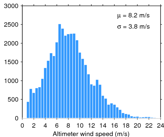
Figure 35. Histogram of science-valid wind over oceans and lakes for 01/05/2018. The mean ( \mu ) and standard deviation ( \sigma ) are also shown. Note that values larger than 24 m/s are excluded from the histogram for the sake of readability but not from the computation of \mu and \sigma .
