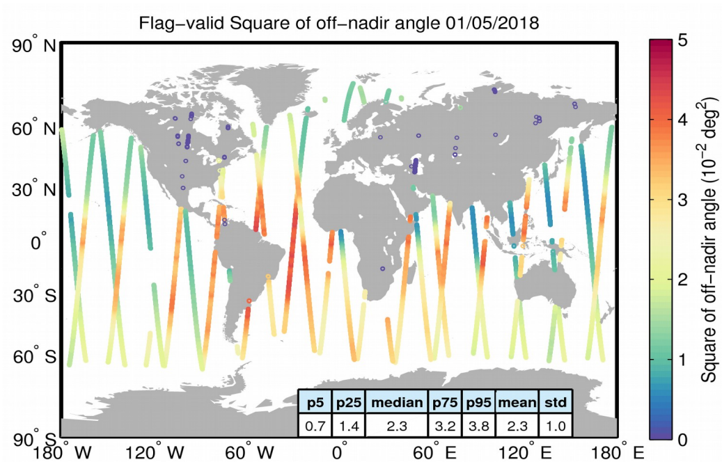
Figure 37. Geographical distribution of flag-valid mispointing data over oceans and lakes for 01/05/2018. The statistical values shown in the table refer to the mispointing in 10^{-2} \text{deg}^2 and are calculated over all measurements shown in the figure.
