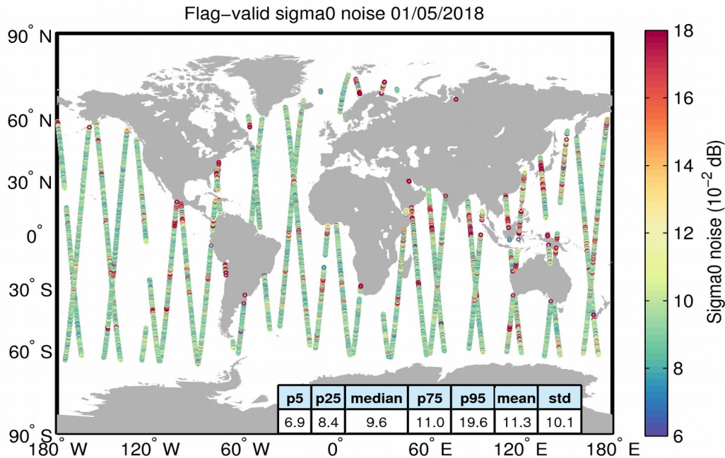
Figure 26. Geographical distribution of flag-valid 20-Hz sigma0 measurement noise over oceans and lakes for 01/05/2018. The statistical values shown in the table refer to the sigma0 noise and are calculated over all measurements shown in the figure.
