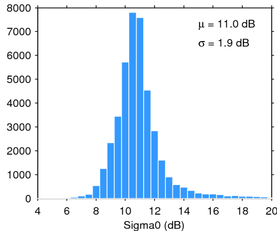
Figure 25. Histogram of flag-valid sigma0 over oceans and lakes for 01/05/2018. The mean ( \mu ) and standard deviation ( \sigma ) are also shown. Note that values outside [4 20] dB are excluded from the histogram for the sake of readability but not from the computation of \mu and \sigma .
