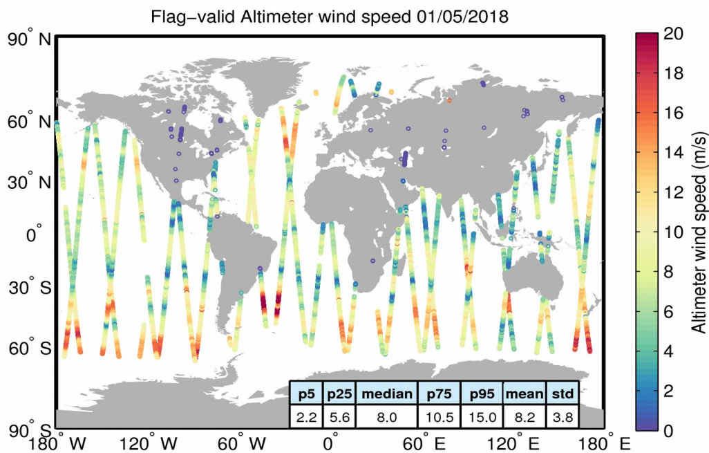
Figure 31. Geographical distribution of flag-valid wind data over oceans and lakes for 01/05/2018. The statistical values shown in the table refer to the wind in m/s and are calculated over all measurements shown in the figure.
