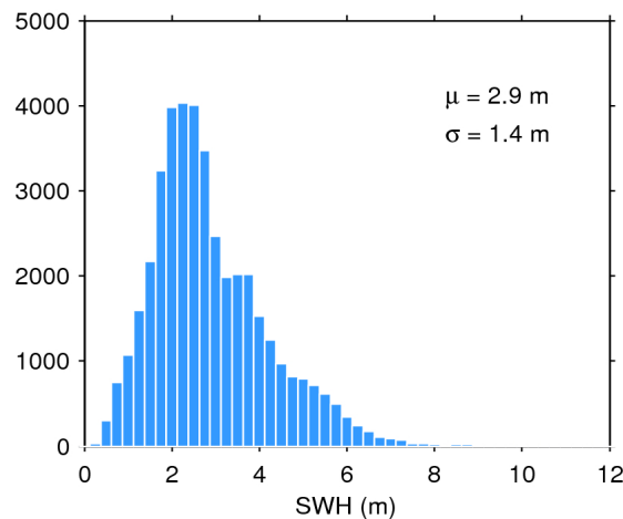
Figure 17. Histogram of flag-valid SWH over oceans and lakes for 01/05/2018. The mean ( \mu ) and standard deviation ( \sigma ) are also shown. Note that values larger than 12 m are excluded from the histogram for the sake of readability but not from the computation of \mu and \sigma .
