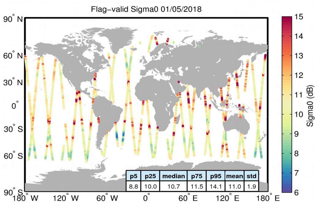
Figure 23. Geographical distribution of flag-valid sigma0 data over oceans and lakes for 01/05/2018. The statistical values shown in the table refer to the sigma0 in dB and are calculated over all measurements shown in the figure.
