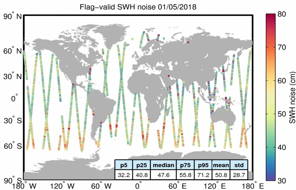
Figure 18. Geographical distribution of flag-valid 20-Hz SWH measurement noise over oceans and lakes for 01/05/2018. The statistical values shown in the figure refer to the SWH noise and are calculated over all measurements shown in the figure.
