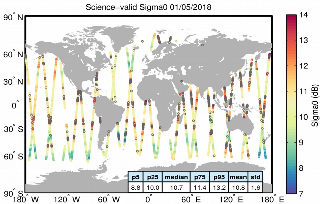
Figure 27. Geographical distribution of science-valid sigma0 data over oceans and lakes for 01/05/2018. The statistical values shown in the table refer to the sigma0 in dB and are calculated over all measurements shown in the figure. Gray circles denote records that have been rejected based on the editing criteria described in Table 4.
