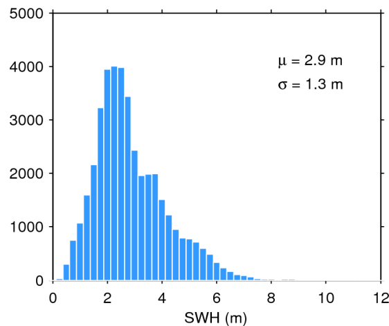
Figure 20. Histogram of science-valid SWH over oceans and lakes for 01/05/2018. The mean ( \mu ) and standard deviation ( \sigma ) are also shown. Note that values larger than 12 m are excluded from the histogram for the sake of readability but not from the computation of \mu and \sigma .
