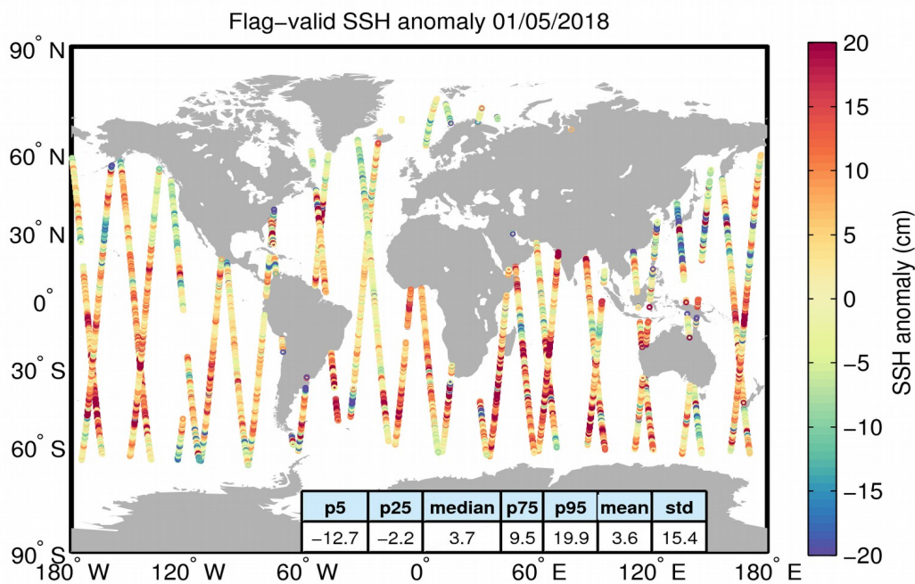
Figure 5. Geographical distribution of flag-valid 1-Hz SSH anomaly data over oceans and lakes for 01/05/2018. The statistical values shown in the table refer to the SSH anomaly in cm and are calculated over all measurements shown in the figure.
