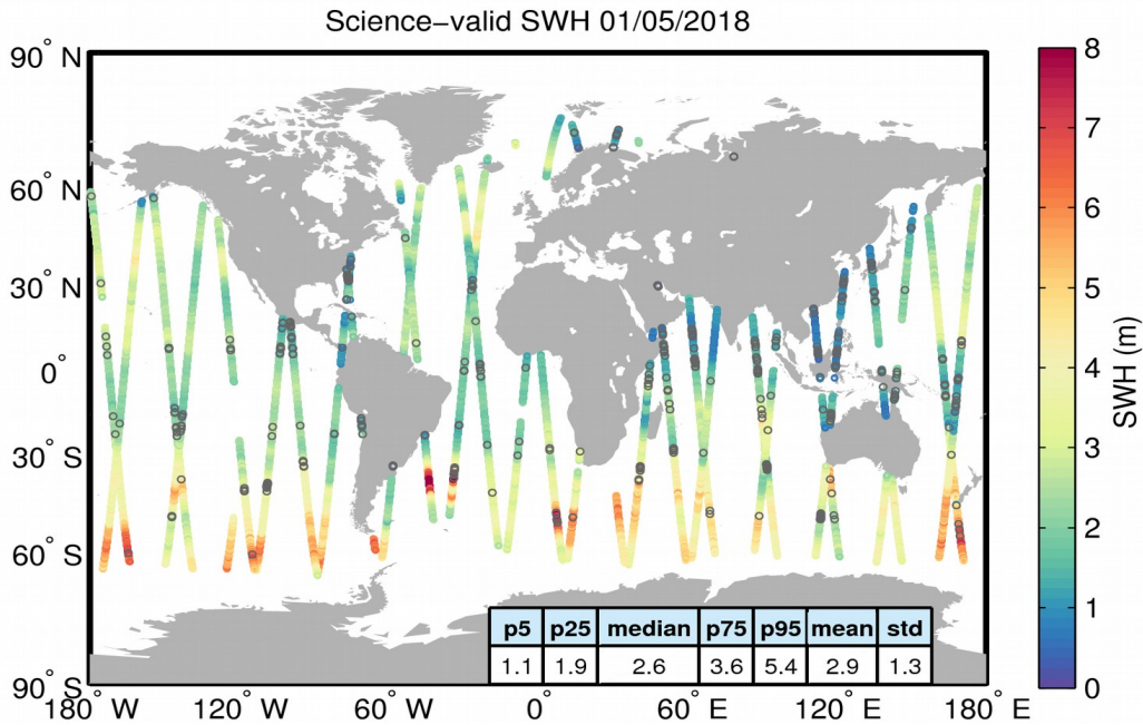
Figure 19. Geographical distribution of science-valid SWH data over oceans and lakes for 01/05/2018. The statistical values shown in the table refer to the SWH in m and are calculated over all measurements shown in the figure. Gray circles denote records that have been rejected based on the editing criteria described in Table 3.
