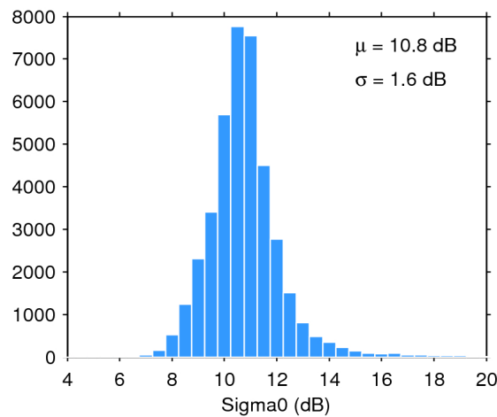
Figure 28. Histogram of science-valid sigma0 over oceans and lakes for 01/05/2018. The mean ( \mu ) and standard deviation ( \sigma ) are also shown. Note that values outside [4 20] dB are excluded from the histogram for the sake of readability but not from the computation of \mu and \sigma .
