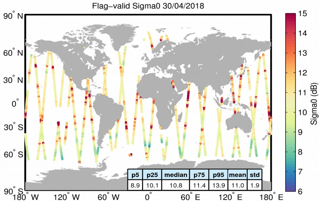
Figure 23. Geographical distribution of flag-valid sigma0 data over oceans and lakes for 30/04/2018. The statistical values shown in the table refer to the sigma0 in dB and are calculated over all measurements shown in the figure.
