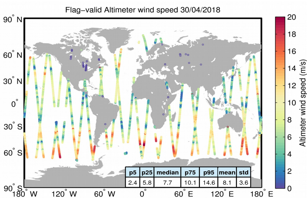
Figure 31. Geographical distribution of flag-valid wind data over oceans and lakes for 30/04/2018. The statistical values shown in the table refer to the wind in m/s and are calculated over all measurements shown in the figure.
