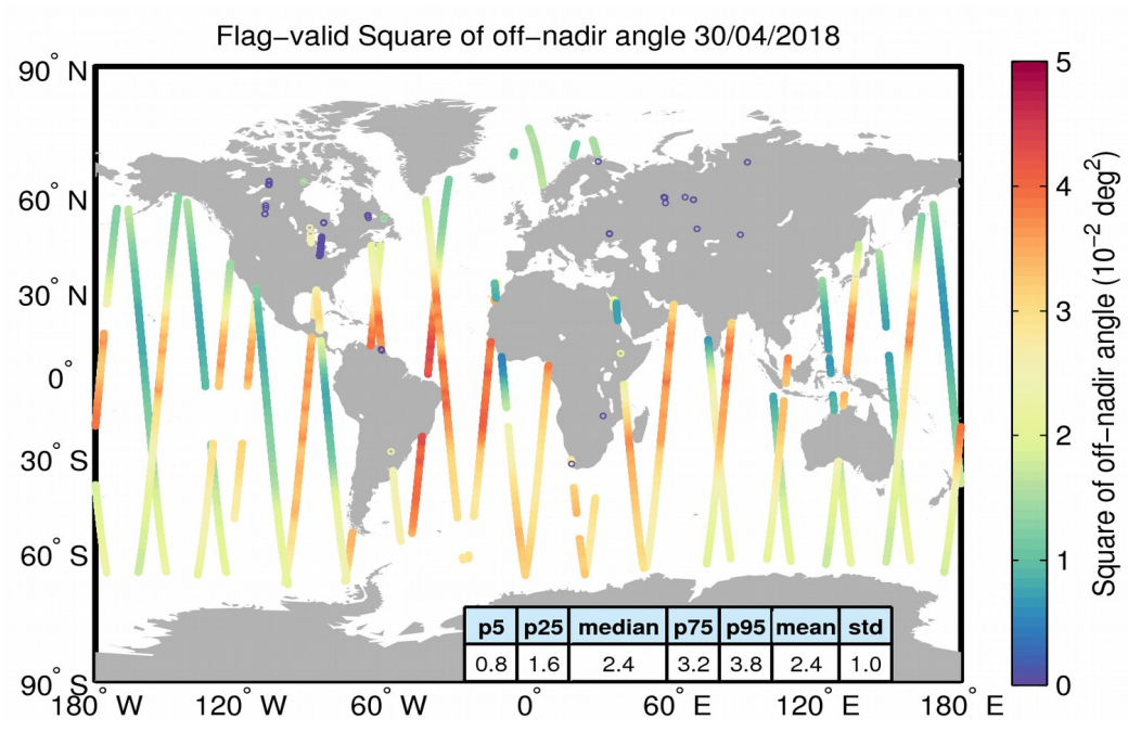
Figure 37. Geographical distribution of flag-valid mispointing data over oceans and lakes for 30/04/2018. The statistical values shown in the table refer to the mispointing in 10^{-2} deg 2 and are calculated over all measurements shown in the figure.
