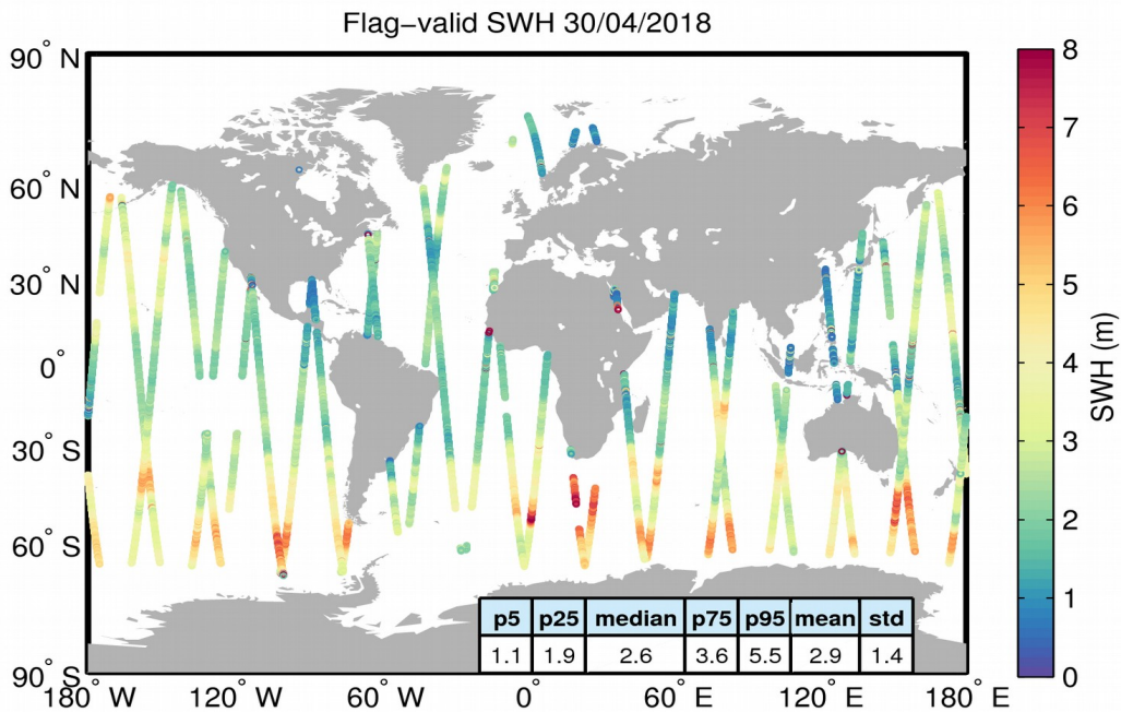
Figure 15. Geographical distribution of flag-valid SWH data over oceans and lakes for 30/04/2018. The statistical values shown in the table refer to the SWH in m and are calculated over all measurements shown in the figure.
