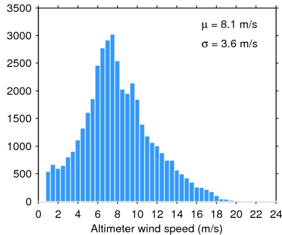
Figure 33. Histogram of flag-valid wind over oceans and lakes for 30/04/2018. The mean ( \mu ) and standard deviation ( \sigma ) are also shown. Note that values larger than 24 m/s are excluded from the histogram for the sake of readability but not from the computation of \mu and \sigma .
