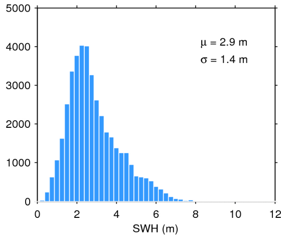
Figure 17. Histogram of flag-valid SWH over oceans and lakes for 30/04/2018. The mean ( \mu ) and standard deviation ( \sigma ) are also shown. Note that values larger than 12 m are excluded from the histogram for the sake of readability but not from the computation of \mu and \sigma .
