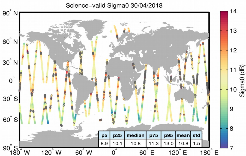
Figure 27. Geographical distribution of science-valid sigma0 data over oceans and lakes for 30/04/2018. The statistical values shown in the table refer to the sigma0 in dB and are calculated over all measurements shown in the figure. Gray circles denote records that have been rejected based on the editing criteria described in Table 4.
