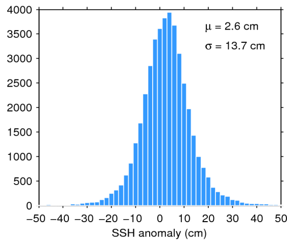
Figure 7. Histogram of flag-valid SSH anomaly over oceans and lakes for 29/04/2018. The mean ( \mu ) and standard deviation ( \sigma ) are also shown. Note that values outside [-50\ 50] cm are excluded from the histogram for the sake of readability but not from the computation of \mu and \sigma .
