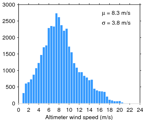
Figure 33. Histogram of flag-valid wind over oceans and lakes for 29/04/2018. The mean ( \mu ) and standard deviation ( \sigma ) are also shown. Note that values larger than 24 m/s are excluded from the histogram for the sake of readability but not from the computation of \mu and \sigma .
