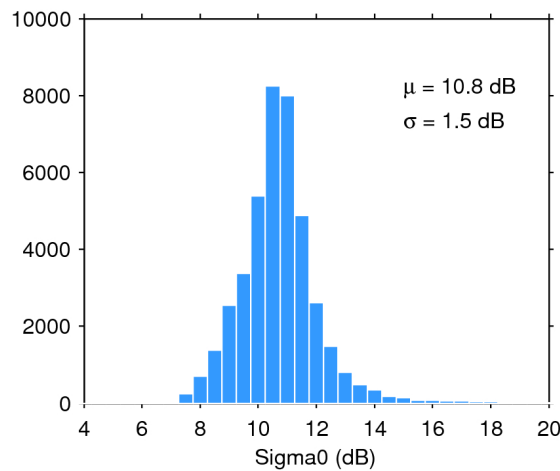
Figure 28. Histogram of science-valid sigma0 over oceans and lakes for 29/04/2018. The mean ( \mu ) and standard deviation ( \sigma ) are also shown. Note that values outside [4 20] dB are excluded from the histogram for the sake of readability but not from the computation of \mu and \sigma .
