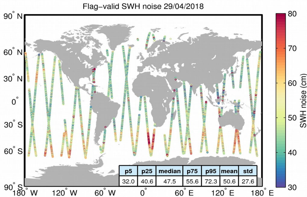
Figure 18. Geographical distribution of flag-valid 20-Hz SWH measurement noise over oceans and lakes for 29/04/2018. The statistical values shown in the figure refer to the SWH noise and are calculated over all measurements shown in the figure.
