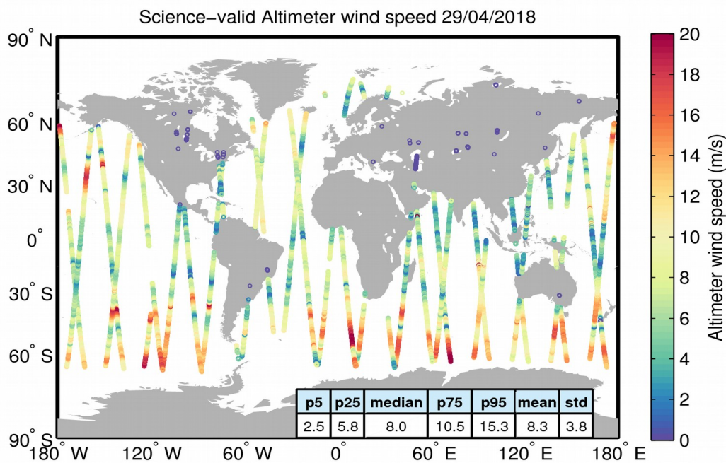
Figure 34. Geographical distribution of science-valid wind data over oceans and lakes for 29/04/2018. The statistical values shown in the table refer to the wind in m/s and are calculated over all measurements shown in the figure. Gray circles denote records that have been rejected based on the editing criteria described in Table 5.
