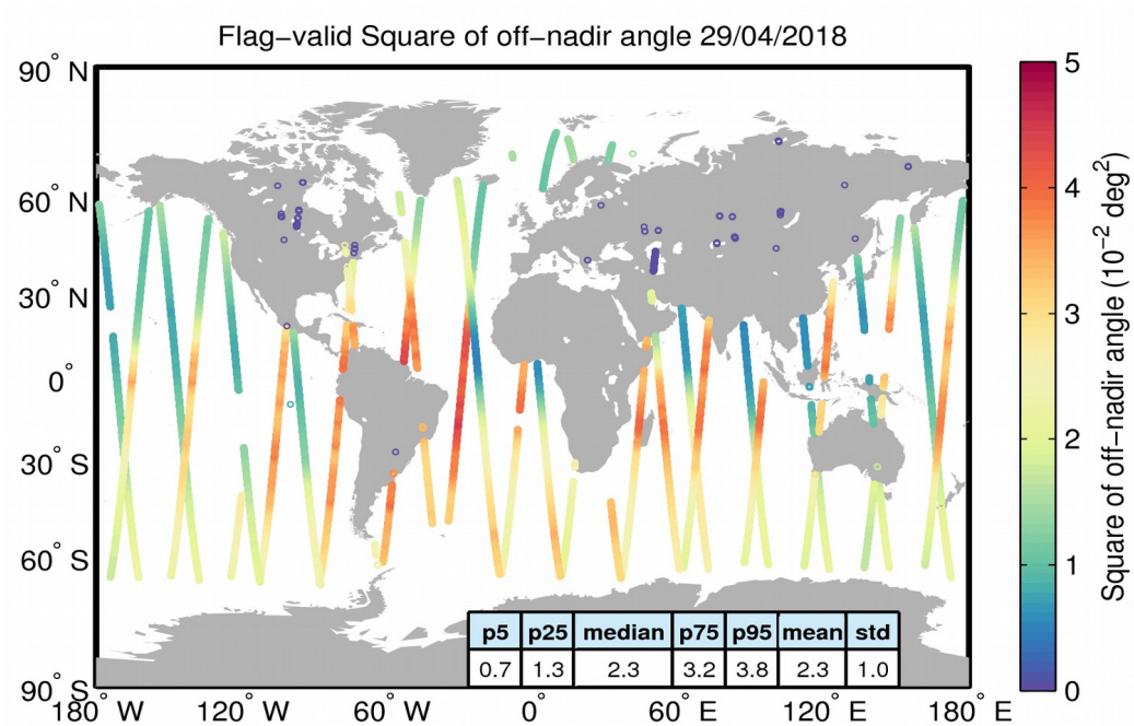
Figure 37. Geographical distribution of flag-valid mispointing data over oceans and lakes for 29/04/2018. The statistical values shown in the table refer to the mispointing in 10^{-2} deg 2 and are calculated over all measurements shown in the figure.
