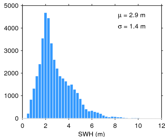
Figure 20. Histogram of science-valid SWH over oceans and lakes for 29/04/2018. The mean ( \mu ) and standard deviation ( \sigma ) are also shown. Note that values larger than 12 m are excluded from the histogram for the sake of readability but not from the computation of \mu and \sigma .
