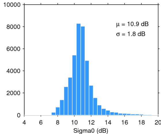
Figure 25. Histogram of flag-valid sigma0 over oceans and lakes for 29/04/2018. The mean ( \mu ) and standard deviation ( \sigma ) are also shown. Note that values outside [4 20] dB are excluded from the histogram for the sake of readability but not from the computation of \mu and \sigma .
