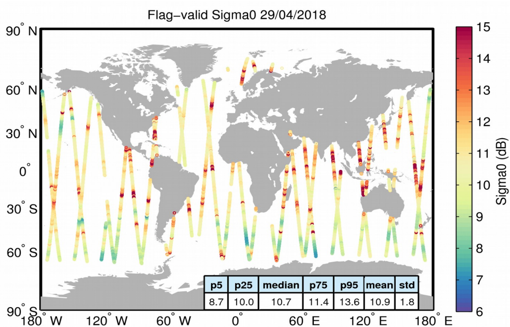
Figure 23. Geographical distribution of flag-valid sigma0 data over oceans and lakes for 29/04/2018. The statistical values shown in the table refer to the sigma0 in dB and are calculated over all measurements shown in the figure.
