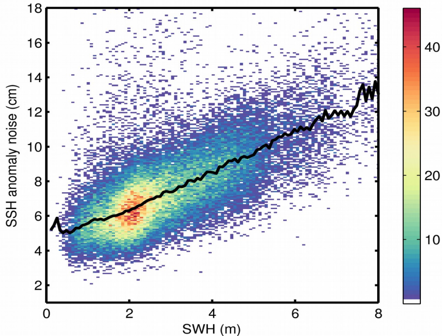
Figure 9. 2D histogram showing flag-valid SSH anomaly noise as a function of SWH for 29/04/2018. The black line denotes the median SSH anomaly noise as a function of SWH.
