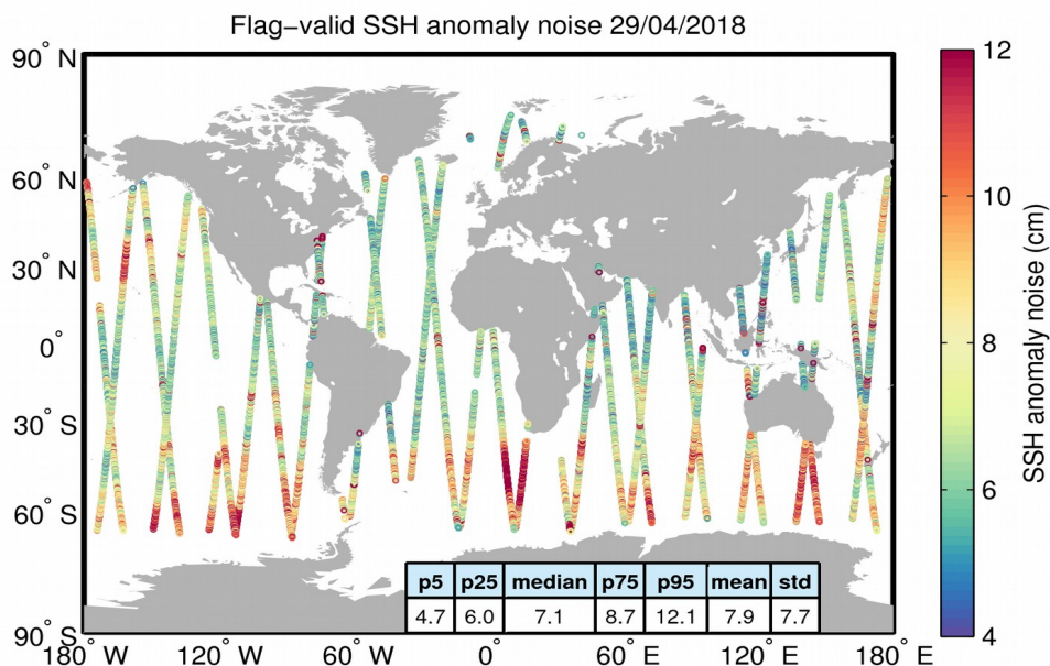
Figure 8. Geographical distribution of flag-valid 20-Hz SSH anomaly measurement noise over oceans and lakes for 29/04/2018. The statistical values shown in the table refer to the SSH anomaly noise and are calculated over all measurements shown in the figure.
