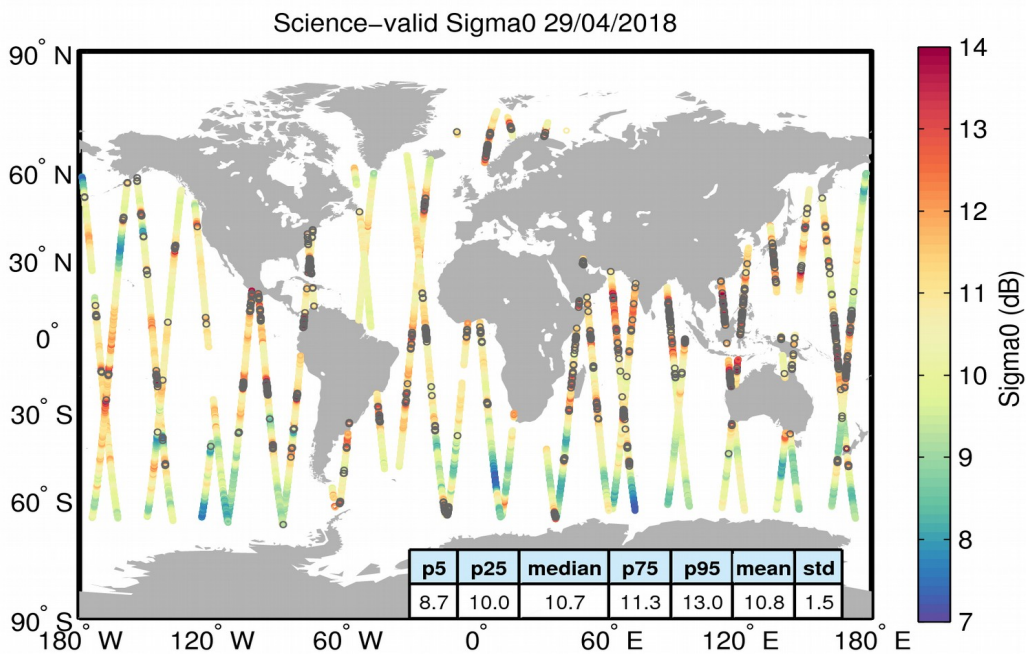
Figure 27. Geographical distribution of science-valid sigma0 data over oceans and lakes for 29/04/2018. The statistical values shown in the table refer to the sigma0 in dB and are calculated over all measurements shown in the figure. Gray circles denote records that have been rejected based on the editing criteria described in Table 4.
