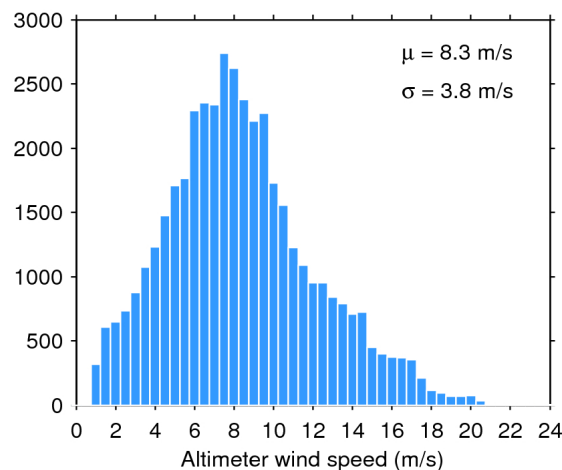
Figure 35. Histogram of science-valid wind over oceans and lakes for 29/04/2018. The mean ( \mu ) and standard deviation ( \sigma ) are also shown. Note that values larger than 24 m/s are excluded from the histogram for the sake of readability but not from the computation of \mu and \sigma .
