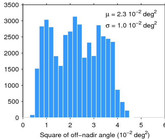
Figure 39. Histogram of flag-valid mispointing over oceans and lakes for 29/04/2018. The mean ( \mu ) and standard deviation ( \sigma ) are also shown. Note that values larger than 6 \cdot 10^{-2} \text{ deg}^2 are excluded from the histogram for the sake of readability but not from the computation of \mu and \sigma .
