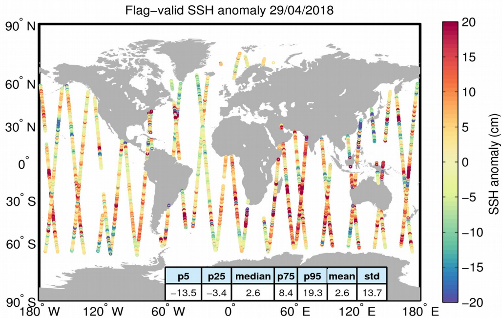
Figure 5. Geographical distribution of flag-valid 1-Hz SSH anomaly data over oceans and lakes for 29/04/2018. The statistical values shown in the table refer to the SSH anomaly in cm and are calculated over all measurements shown in the figure.
