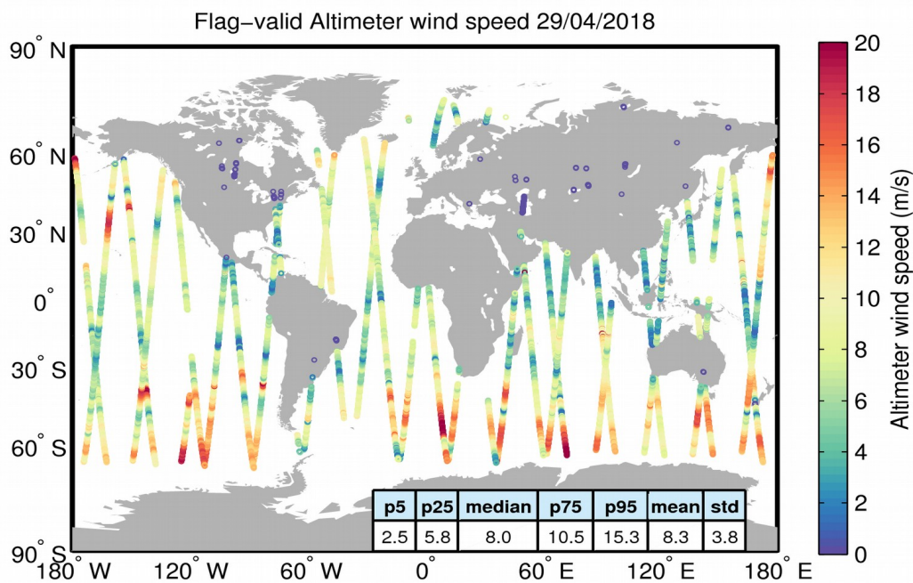
Figure 31. Geographical distribution of flag-valid wind data over oceans and lakes for 29/04/2018. The statistical values shown in the table refer to the wind in m/s and are calculated over all measurements shown in the figure.
