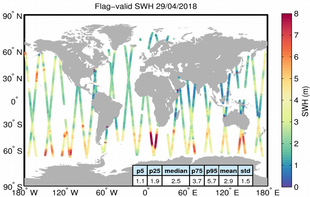
Figure 15. Geographical distribution of flag-valid SWH data over oceans and lakes for 29/04/2018. The statistical values shown in the table refer to the SWH in m and are calculated over all measurements shown in the figure.
