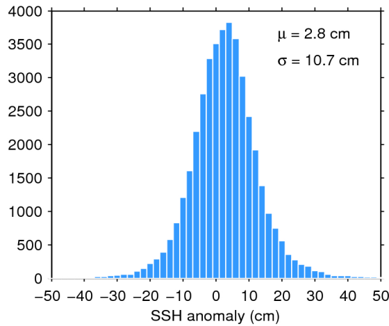
Figure 11. Histogram of science-valid SSH anomaly over oceans and lakes for 29/04/2018. The mean ( \mu ) and standard deviation ( \sigma ) are also shown. Note that values outside [-50 50] cm are excluded from the histogram for the sake of readability but not from the computation of \mu and \sigma .
