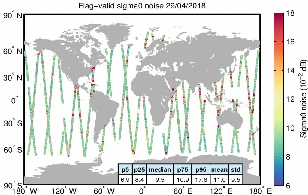
Figure 26. Geographical distribution of flag-valid 20-Hz sigma0 measurement noise over oceans and lakes for 29/04/2018. The statistical values shown in the table refer to the sigma0 noise and are calculated over all measurements shown in the figure.
