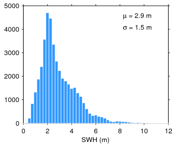
Figure 17. Histogram of flag-valid SWH over oceans and lakes for 29/04/2018. The mean ( \mu ) and standard deviation ( \sigma ) are also shown. Note that values larger than 12 m are excluded from the histogram for the sake of readability but not from the computation of \mu and \sigma .
