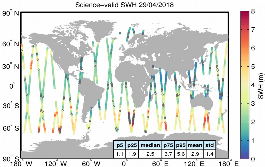
Figure 19. Geographical distribution of science-valid SWH data over oceans and lakes for 29/04/2018. The statistical values shown in the table refer to the SWH in m and are calculated over all measurements shown in the figure. Gray circles denote records that have been rejected based on the editing criteria described in Table 3.
