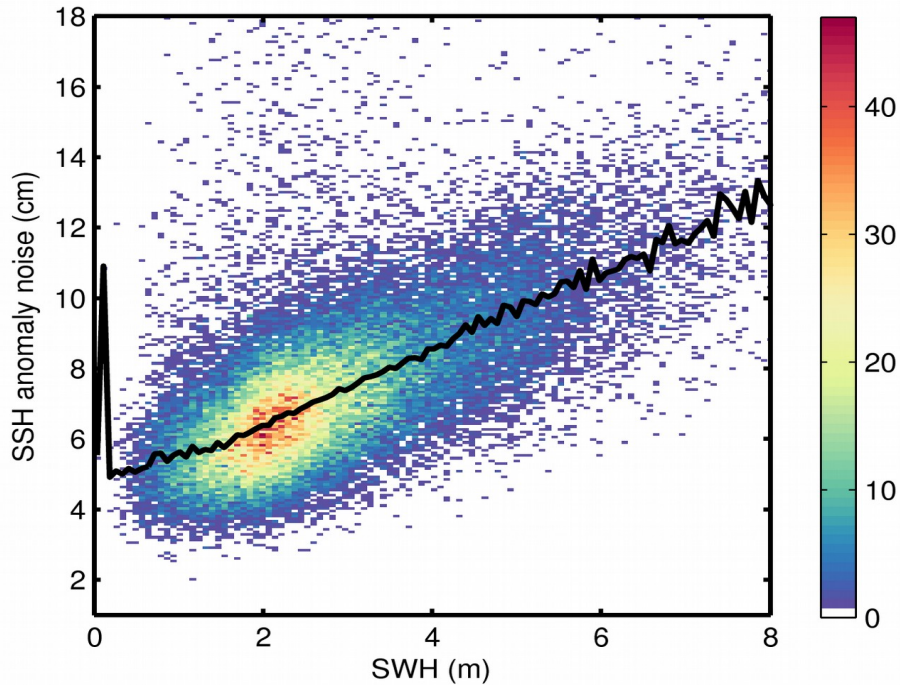
Figure 9. 2D histogram showing flag-valid SSH anomaly noise as a function of SWH for 28/04/2018. The black line denotes the median SSH anomaly noise as a function of SWH.
