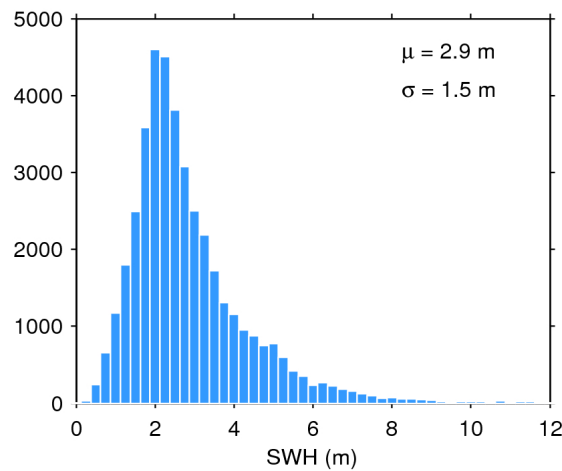
Figure 17. Histogram of flag-valid SWH over oceans and lakes for 28/04/2018. The mean ( \mu ) and standard deviation ( \sigma ) are also shown. Note that values larger than 12 m are excluded from the histogram for the sake of readability but not from the computation of \mu and \sigma .
