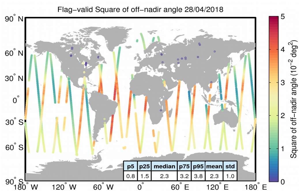
Figure 37. Geographical distribution of flag-valid mispointing data over oceans and lakes for 28/04/2018. The statistical values shown in the table refer to the mispointing in 10^{-2} \text{ deg}^2 and are calculated over all measurements shown in the figure.
