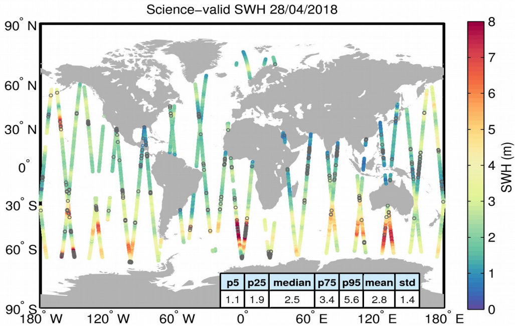
Figure 19. Geographical distribution of science-valid SWH data over oceans and lakes for 28/04/2018. The statistical values shown in the table refer to the SWH in m and are calculated over all measurements shown in the figure. Gray circles denote records that have been rejected based on the editing criteria described in Table 3.
