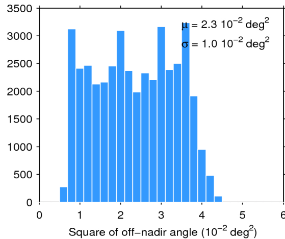
Figure 39. Histogram of flag-valid mispointing over oceans and lakes for 28/04/2018. The mean ( \mu ) and standard deviation ( \sigma ) are also shown. Note that values larger than 6 \cdot 10^{-2} \text{ deg}^2 are excluded from the histogram for the sake of readability but not from the computation of \mu and \sigma .
