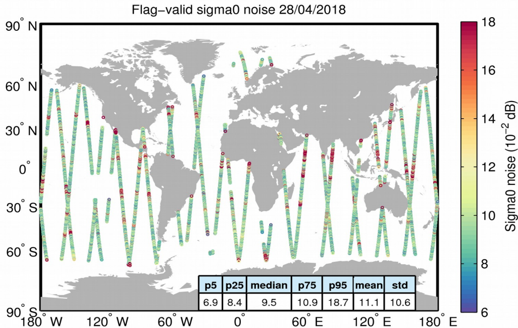
Figure 26. Geographical distribution of flag-valid 20-Hz sigma0 measurement noise over oceans and lakes for 28/04/2018. The statistical values shown in the table refer to the sigma0 noise and are calculated over all measurements shown in the figure.
