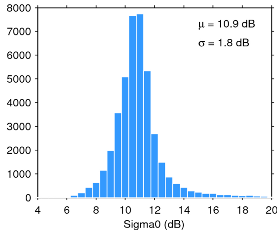
Figure 25. Histogram of flag-valid sigma0 over oceans and lakes for 28/04/2018. The mean ( \mu ) and standard deviation ( \sigma ) are also shown. Note that values outside [4 20] dB are excluded from the histogram for the sake of readability but not from the computation of \mu and \sigma .
