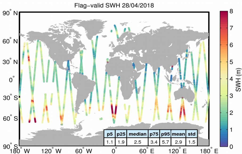
Figure 15. Geographical distribution of flag-valid SWH data over oceans and lakes for 28/04/2018. The statistical values shown in the table refer to the SWH in m and are calculated over all measurements shown in the figure.
