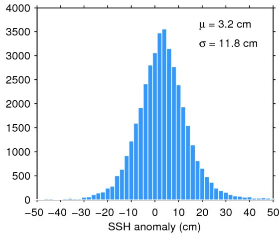
Figure 11. Histogram of science-valid SSH anomaly over oceans and lakes for 28/04/2018. The mean ( \mu ) and standard deviation ( \sigma ) are also shown. Note that values outside [-50 50] cm are excluded from the histogram for the sake of readability but not from the computation of \mu and \sigma .
