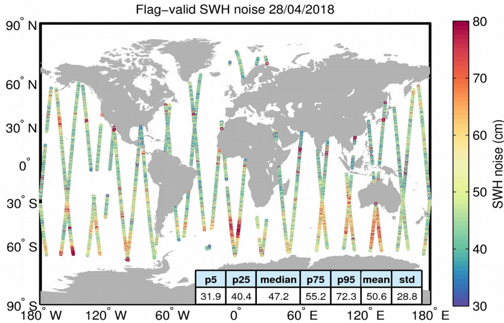
Figure 18. Geographical distribution of flag-valid 20-Hz SWH measurement noise over oceans and lakes for 28/04/2018. The statistical values shown in the figure refer to the SWH noise and are calculated over all measurements shown in the figure.
