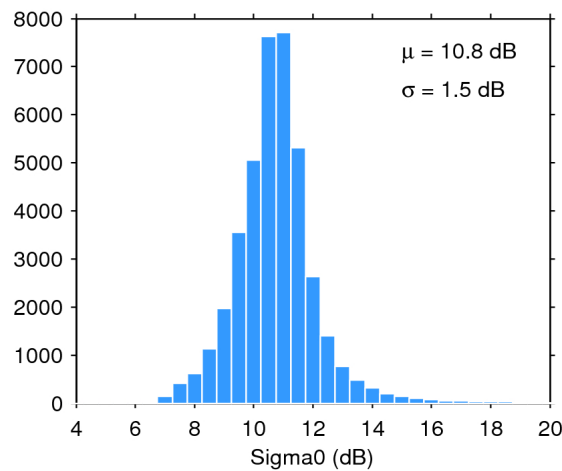
Figure 28. Histogram of science-valid sigma0 over oceans and lakes for 28/04/2018. The mean ( \mu ) and standard deviation ( \sigma ) are also shown. Note that values outside [4 20] dB are excluded from the histogram for the sake of readability but not from the computation of \mu and \sigma .
