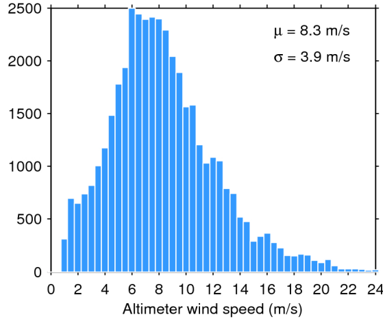
Figure 33. Histogram of flag-valid wind over oceans and lakes for 28/04/2018. The mean ( \mu ) and standard deviation ( \sigma ) are also shown. Note that values larger than 24 m/s are excluded from the histogram for the sake of readability but not from the computation of \mu and \sigma .
