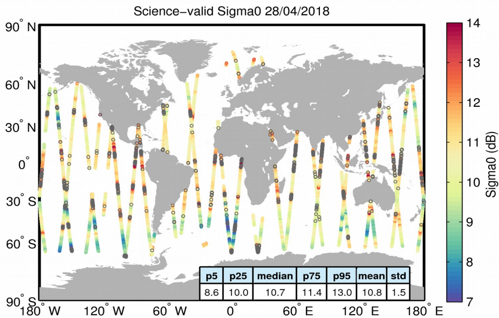
Figure 27. Geographical distribution of science-valid sigma0 data over oceans and lakes for 28/04/2018. The statistical values shown in the table refer to the sigma0 in dB and are calculated over all measurements shown in the figure. Gray circles denote records that have been rejected based on the editing criteria described in Table 4.
