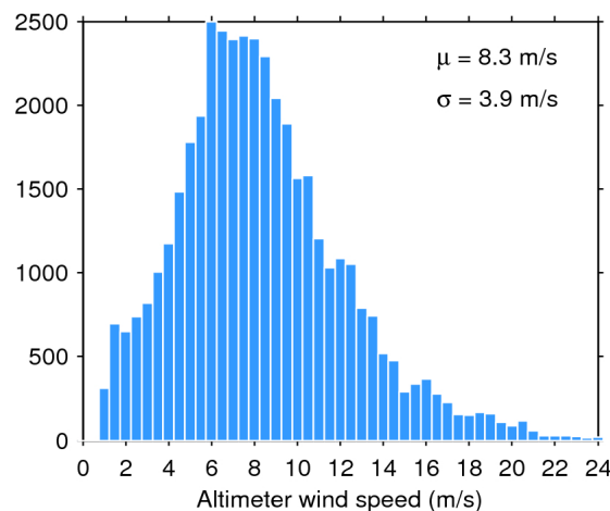
Figure 35. Histogram of science-valid wind over oceans and lakes for 28/04/2018. The mean ( \mu ) and standard deviation ( \sigma ) are also shown. Note that values larger than 24 m/s are excluded from the histogram for the sake of readability but not from the computation of \mu and \sigma .
