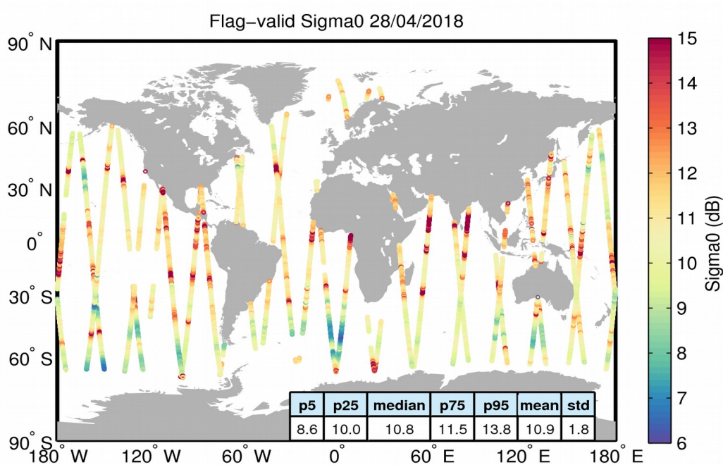
Figure 23. Geographical distribution of flag-valid sigma0 data over oceans and lakes for 28/04/2018. The statistical values shown in the table refer to the sigma0 in dB and are calculated over all measurements shown in the figure.
