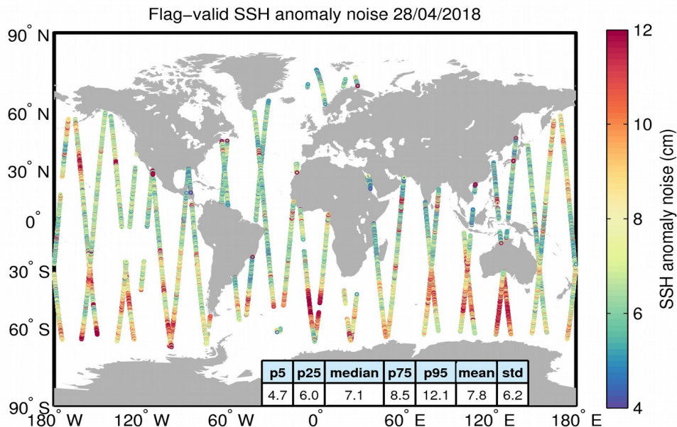
Figure 8. Geographical distribution of flag-valid 20-Hz SSH anomaly measurement noise over oceans and lakes for 28/04/2018. The statistical values shown in the table refer to the SSH anomaly noise and are calculated over all measurements shown in the figure.
