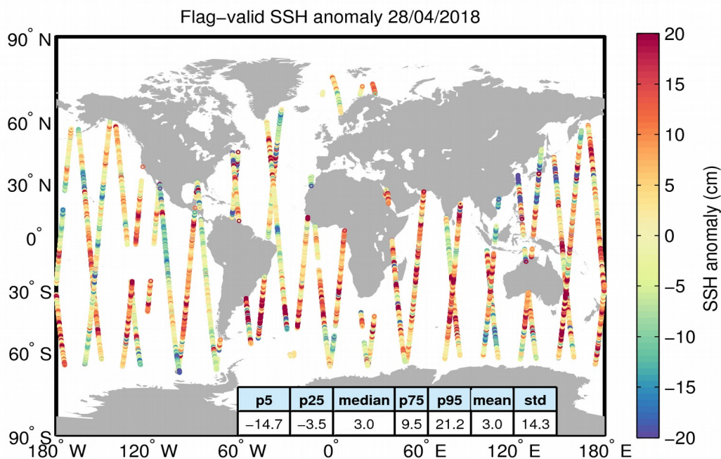
Figure 5. Geographical distribution of flag-valid 1-Hz SSH anomaly data over oceans and lakes for 28/04/2018. The statistical values shown in the table refer to the SSH anomaly in cm and are calculated over all measurements shown in the figure.
